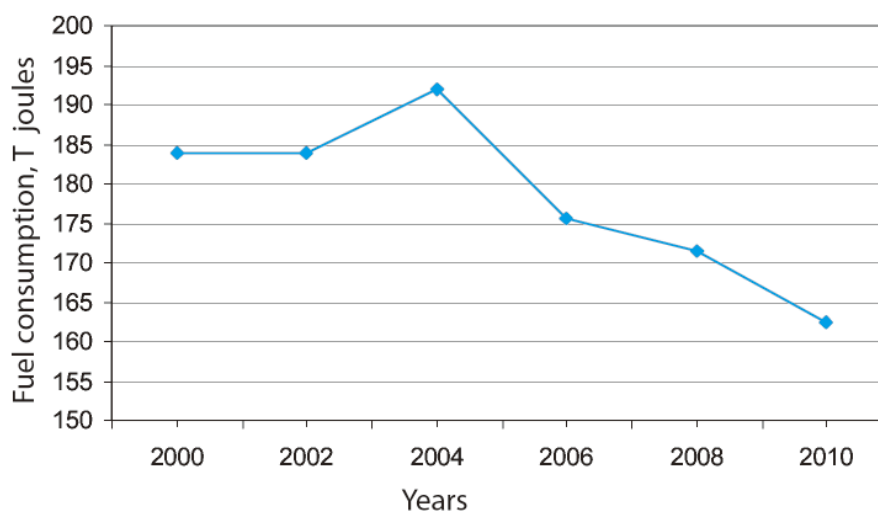
Figure 3.8. Reduction of fuel consumption over the whole power supply system due to phased upgrading of SRPS and HPP
