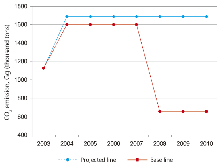
Figure 3.3. Dynamics of reduction of CO 2 emission due to upgrading of Abadan SRPS, thousand tons
