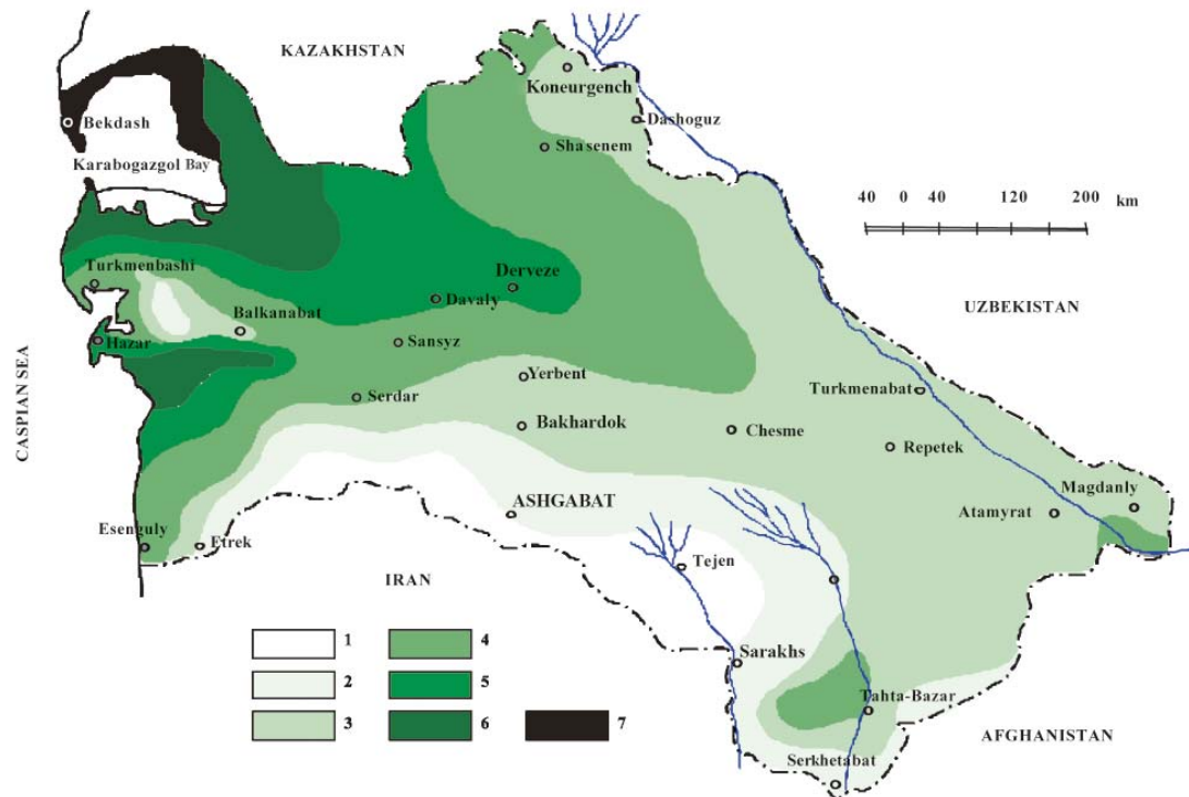
Figure 1.13. Wind - energy resources of Turkmenistan
