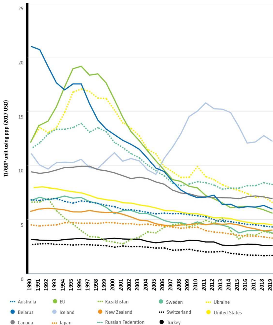
Figure 24 Trends in total primary energy supply per unit of gross domestic product using purchasing power parity for Annex I Parties in 1990–2019
