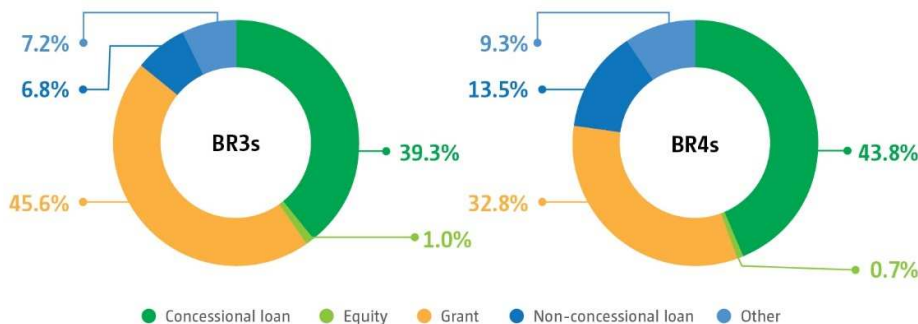
Figure 31 Shares of bilateral, regional and other support by financial instrument as reported in third (2015–2016) and fourth (2017–2018) biennial reports
