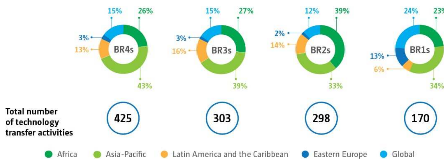
Distribution by region of technology transfer activities reported by Annex II Parties in their biennial reports
