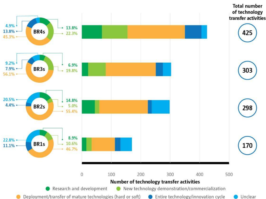
Figure 36 Distribution of technology support by stage of technology cycle reported by Annex II Parties in their biennial reports
