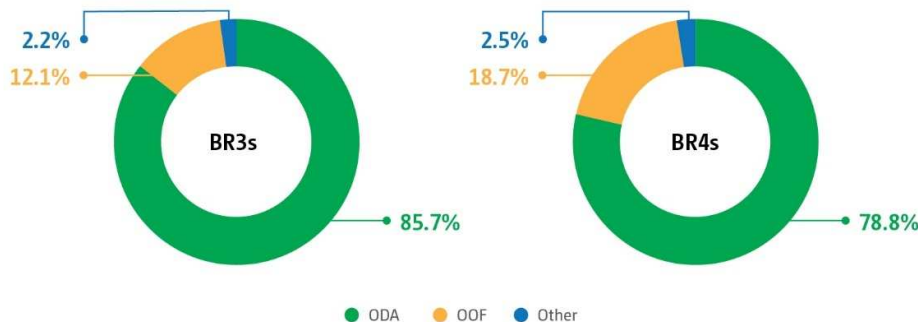
Figure 33 Shares of bilateral, regional and other support by source of funding as reported in third (2015–2016) and fourth (2017–2018) biennial reports
