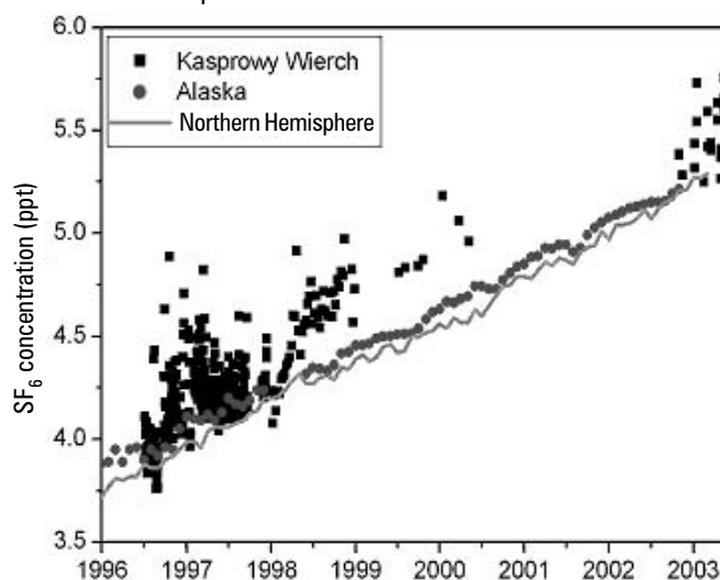
Figure 16. Measurements of SF 6 concentrations at station KASLAB on the Kasprowy Wierch Mountain between June 1996 and April 2003
