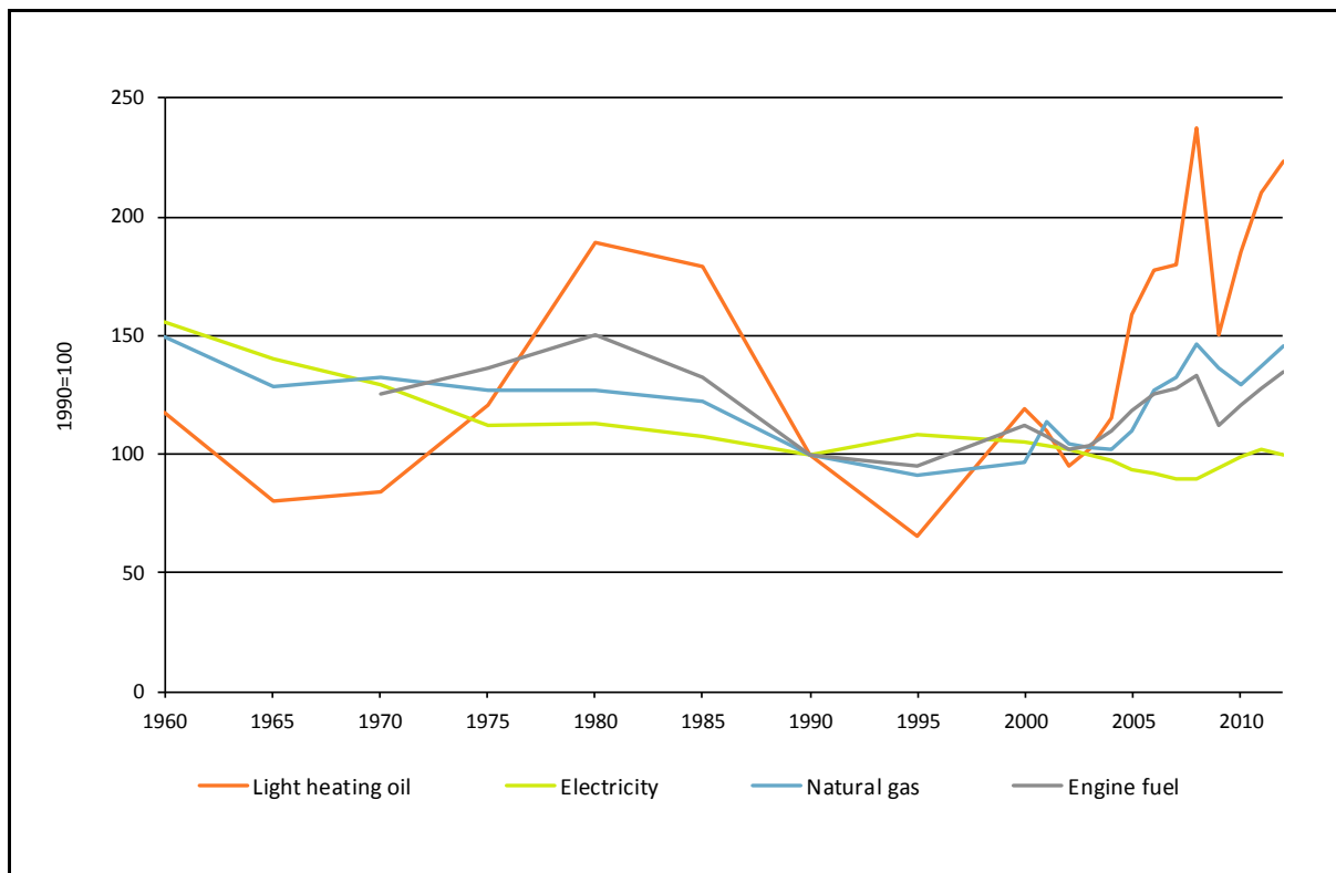
Figure 2-7 Real energy prices of the most important energy sources 1960-2012, Index 1990=100 (SFOE 2012)
