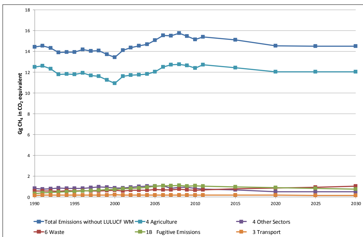
Figure 5-2 CH 4 emissions by sector (excl. LULUCF) from 1990 to 2030 for the scenario WM.
