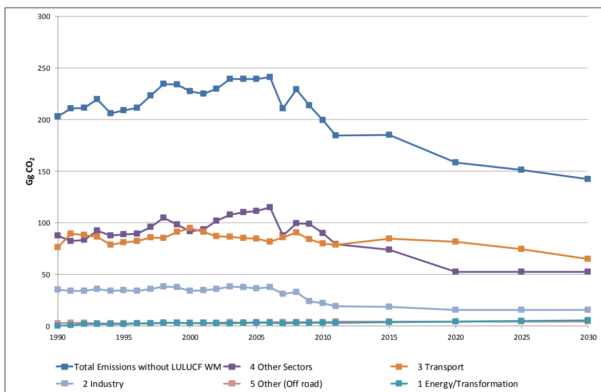
Figure 5-1 CO 2 emissions by sector (excl. LULUCF) from 1990 to 2030 for the scenario WM.
