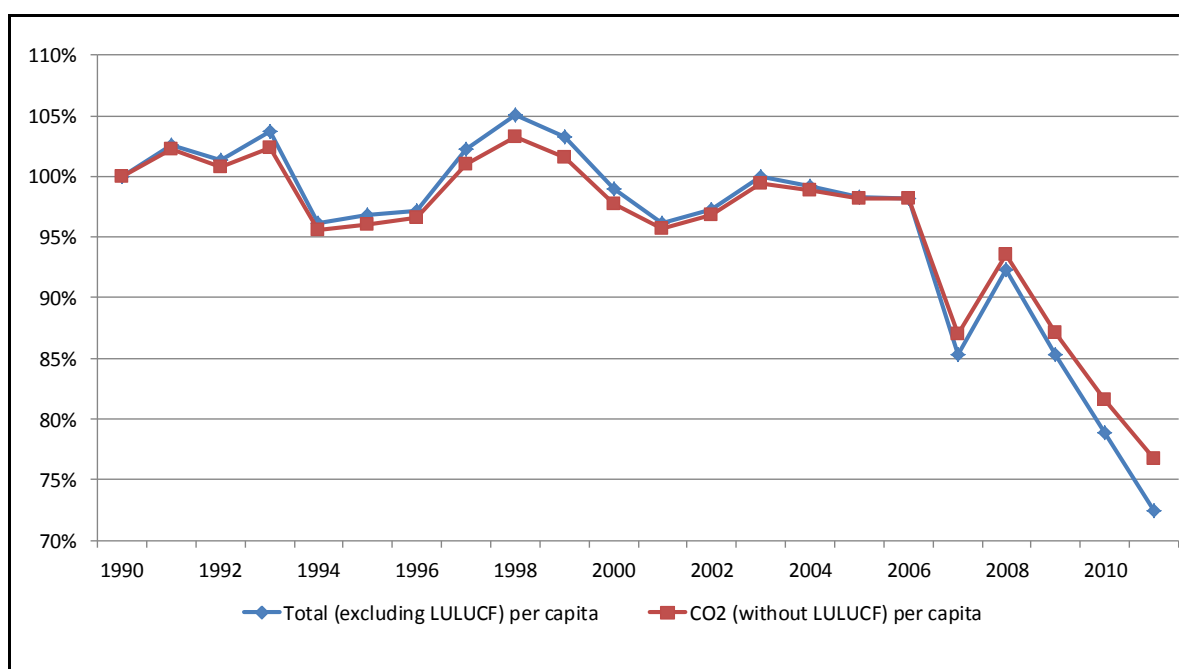
Figure 3-7 Relative CO 2 eq. emissions per capita (excl. LULUCF) and CO 2 emissions per capita (excl. LULUCF) between 1990 and 2011.
