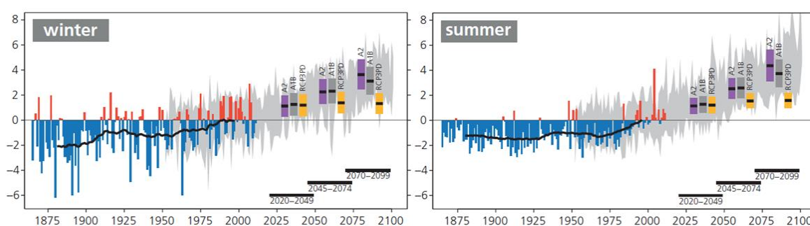
Figure 6-1 Past and future changes in seasonal temperature (°C) over northeastern Switzerland (including the Principality of Liechtenstein). The changes are relative to the reference period 1980–2009. The thin colored bars display the year-to-year differences with respect to the average of observations over the reference period, the heavy black lines are the corresponding smoothed 30-year averages. The grey shading indicates the range of year-to-year differences as projected by climate models for the A1B scenario (specifically, the 5–95 percentile range for each year across the available model set). The thick colored bars show best estimates of the future projections, and the associated uncertainty ranges, for selected 30-year time-periods and for three greenhouse gas emission scenarios (from CH2011 2011).
