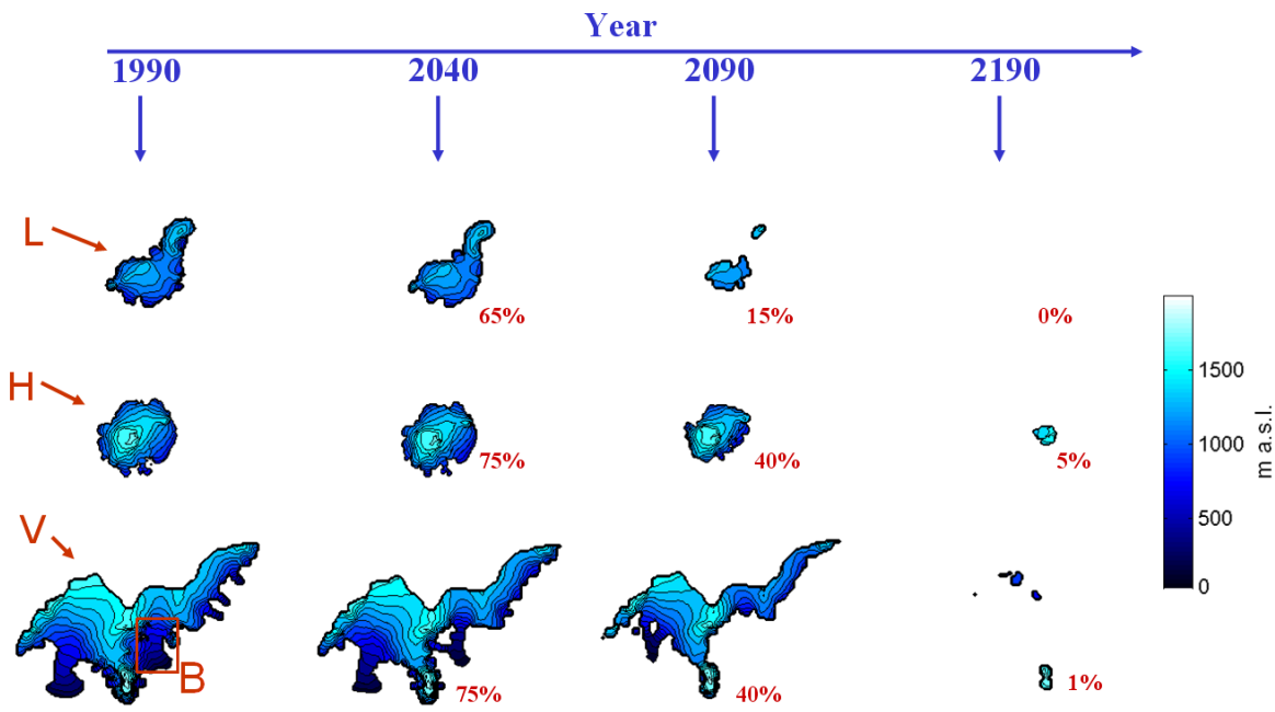
Figure 6.6: Response of Langjökull (L), Hofsjökull (H) and Southern Vatnajökull (V) to a climate warming scenario. The outlet glacier Breiðármerkurjökull on the south flank of Vatnajökull is indicated with a rectangle marked B in the left most map of Vatnajökull. The inset numbers are projected volumes relative to the initial stable glacier geometries in 1990. Note that Vatnajökull is only modeled south of the main east-west ice divide.
