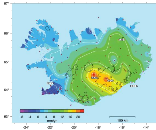
Figure 6.5: Vertical movement of land in Iceland. Much of the interior and the south eastern coast are experiencing uplift due to glacier thinning.
