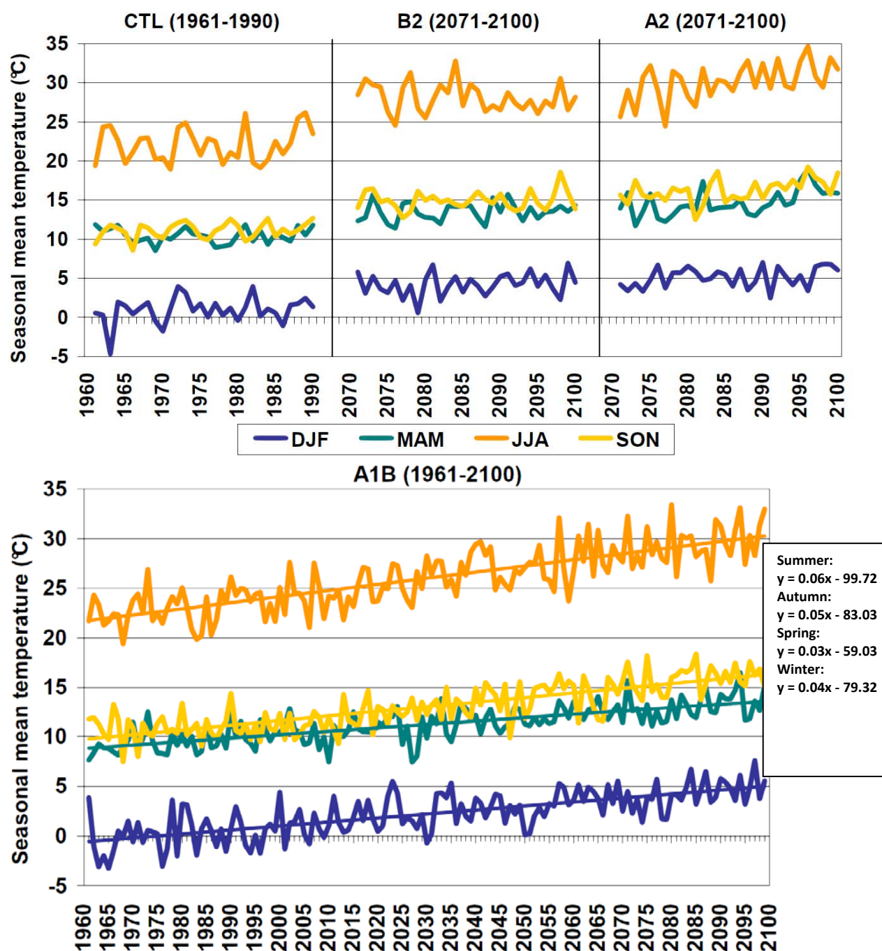
Figure 6.1. Year-to-year variation of seasonal mean temperature (°C) for Hungary. For the A1B simulation the fitted linear trends are also shown for 1961–2100. Source: Pieczka et al.
