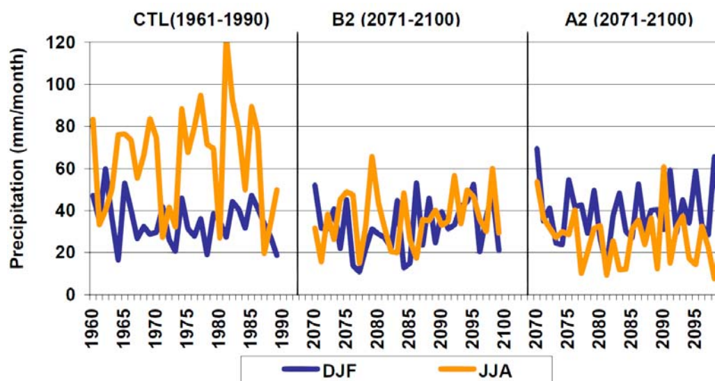
Figure 6.5a. Year-to-year variation of seasonal mean precipitation (mm/month) for Hungary in winter and summer.
