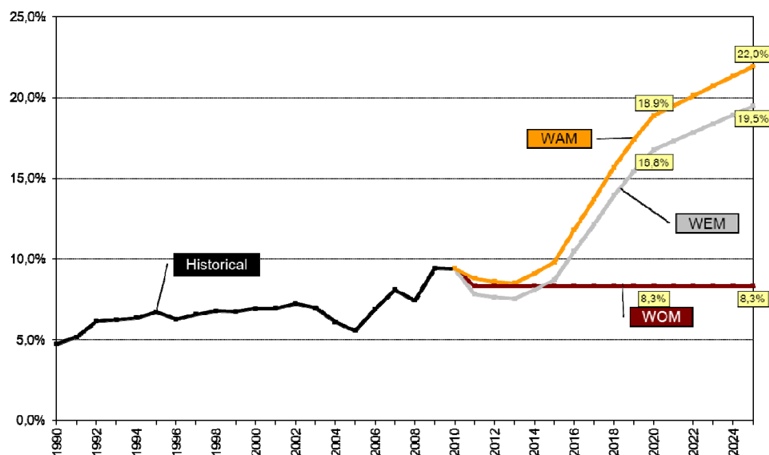
Figure 5.7. Historical and forecasted RES share in heat energy consumption in the three scenarios
