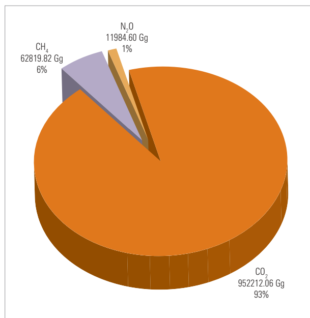
Figure 2.8: Greenhouse gas emission distribution in the energy sector in 2000. (Gg CO 2 eq.)
