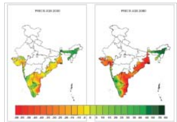
Figure 3.28: Impact of climate change on coconut production in India in PRECIS A1B-2030 and -2080 scenarios (percentage change from current yields)
