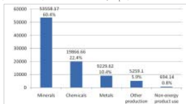
Figure 2.10: Distribution of CO 2 eq. emissions across the categories of the industrial processes and product use sector in 2000 (in Gg CO 2 eq.)
