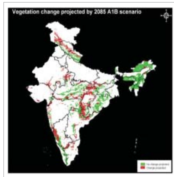
Figure 3.24: All forested grids in India (as per FSI, 2001) are depicted in colour (red or green): red indicates that a change in vegetation is projected at that grid in the time period of 2071–2100, and green indicates that no change in vegetation is projected by that period.
