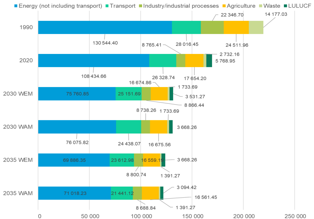
Greenhouse gas emission projections for the Kingdom of the Netherlands presented by sector (kt CO 2 eq)
