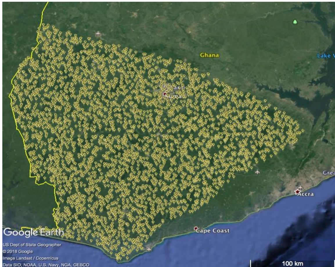
Figure 67: Spatial distribution of the 4000-validation point displayed in Google Earth Pro
