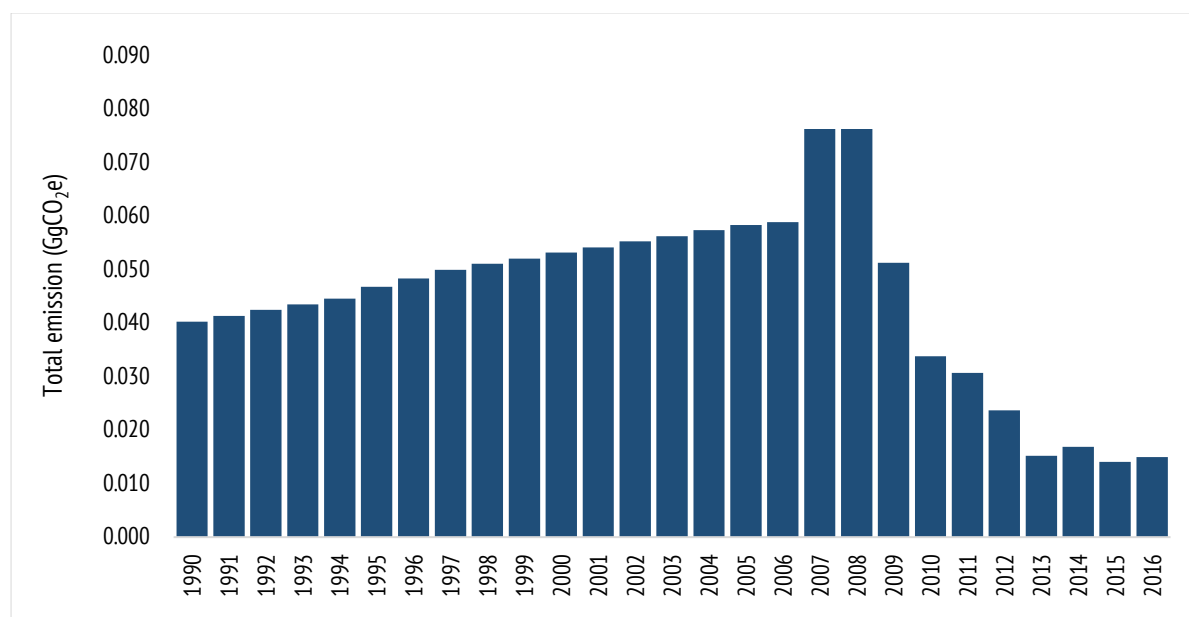
Figure 39: Soda Ash use emissions for the period 1990-2016
