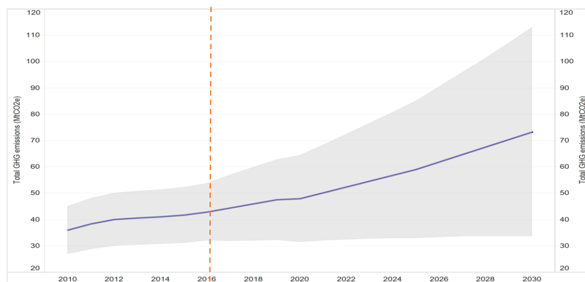
Figure 7: Projected Business-as-Usual emissions trajectory up to 2030 showing the uncertainty band
