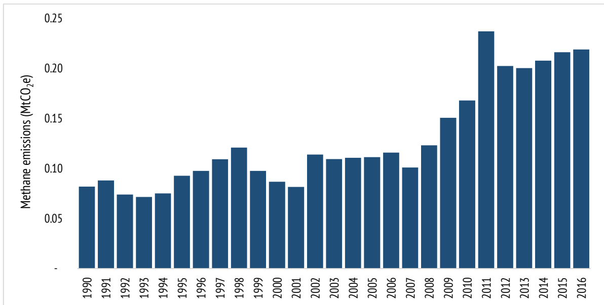
Figure 80: Methane emission trend from rice cultivation
