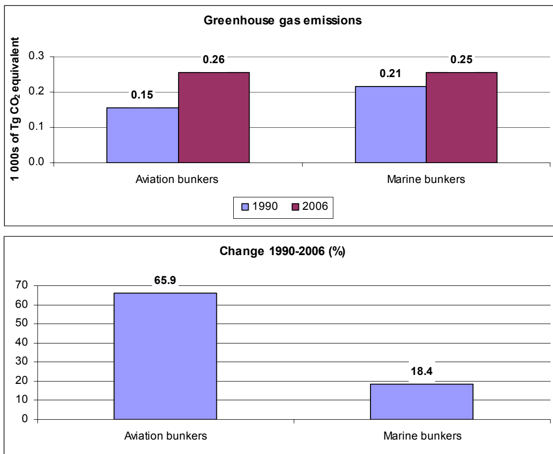
Figure 8. Greenhouse gas emissions from Annex I Parties from international bunker fuels, 1990 and 2006
