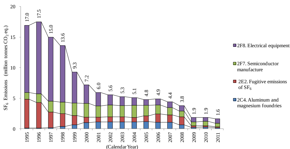
Figure 1-13 Trends in SF 6 Emissions
