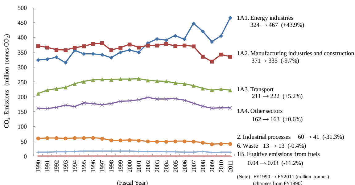
Figure 1-3 Trends in CO 2 Emissions in Each Sector
