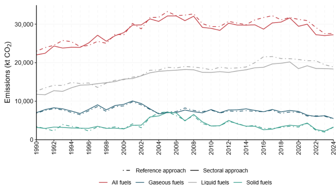
Figure A3.2.1 Reference and sectoral approaches to carbon dioxide by fuel type
