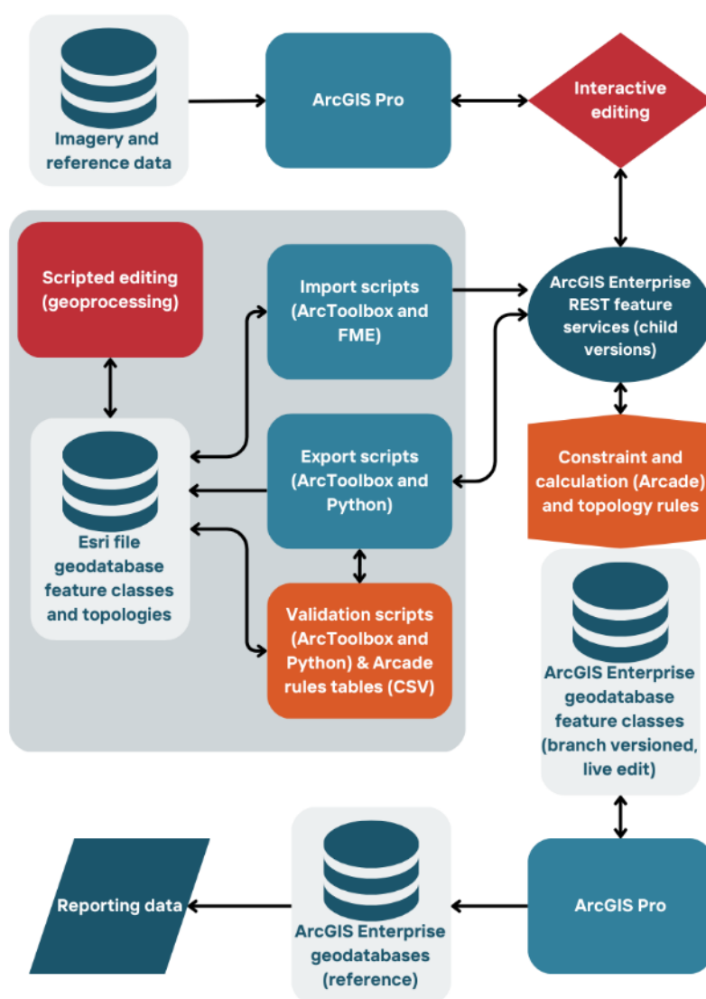
Figure A5.2.21 New Zealand's Geospatial System components
