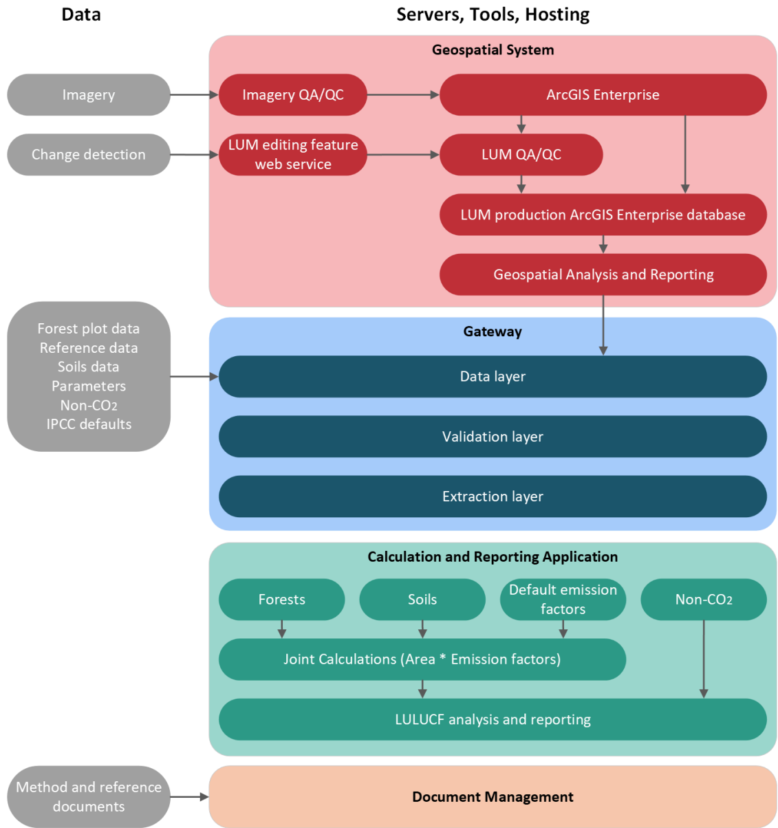
Figure A5.2.20 New Zealand’s LUCAS data management system
