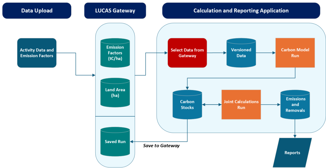
Figure A5.2.22 LUCAS Management Studio
