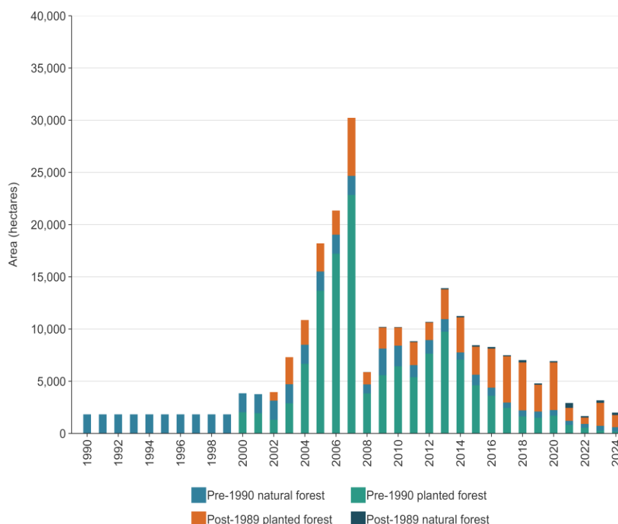
Figure A9.3.1 New Zealand's annual areas of deforestation, from 1990 to 2024
