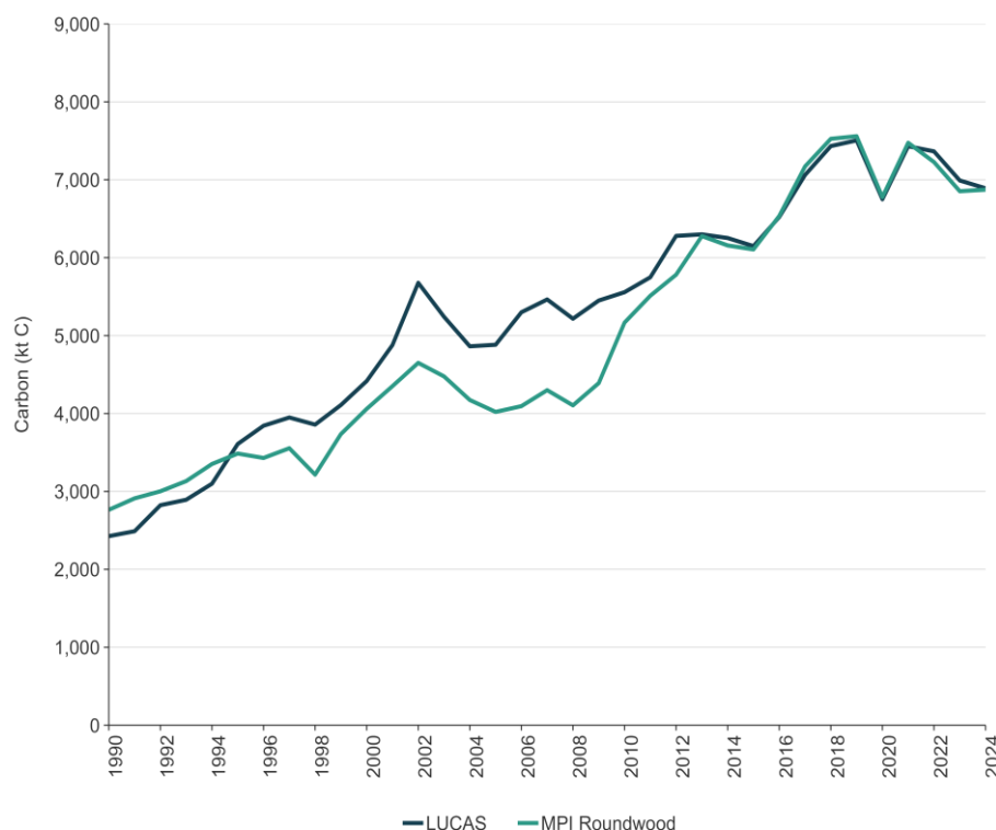
Figure A5.2.13 Comparison of the LUCAS estimate for above-ground biomass removed on planted forest destocking and carbon stored in roundwood production from 1990 to 2024
