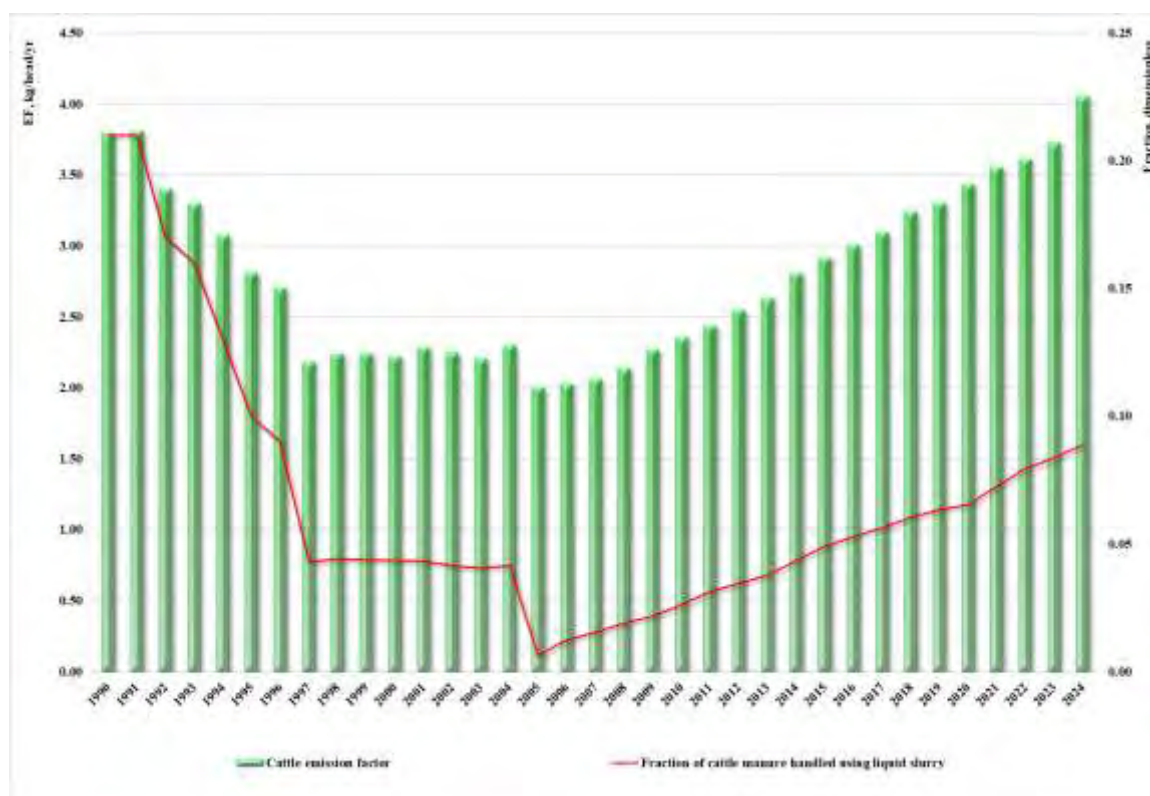
Fig. 5.9. Comparison of cattle emission factors and the shares of manure in MMS
