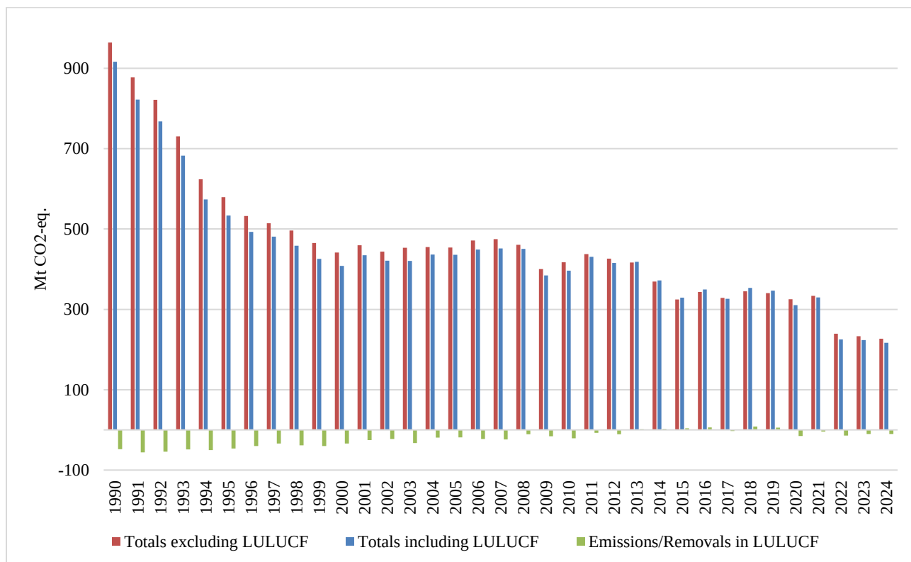
Fig. ES.3.2. Total GHG emissions (+) and removals (-) with and without the LULUCF sector, Mt CO 2 -eq.
