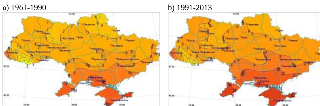
Fig.1.3. Average annual air temperatures: a) 1961-1990; b) 1991-2013
