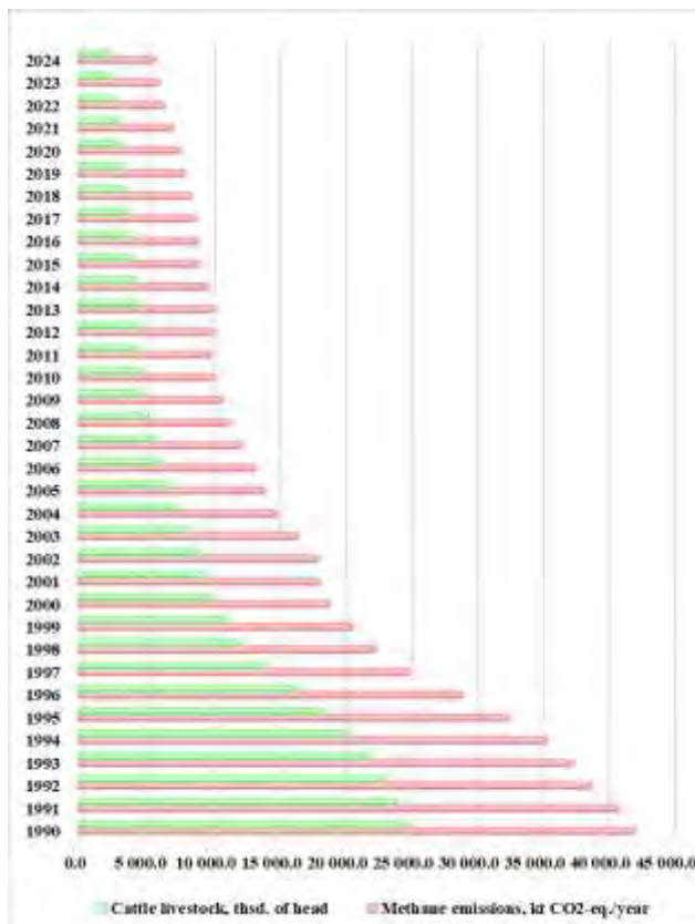
Fig. 5.5 Dependence of methane emission trends in category 3.A Enteric Fermentation on cattle population
