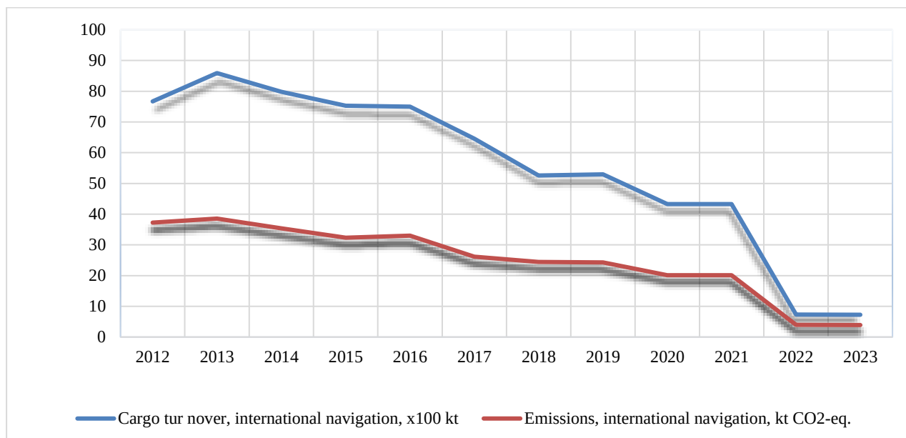
Fig 3.4 The correlation between cargo turnover and GHG emissions for international navigation
