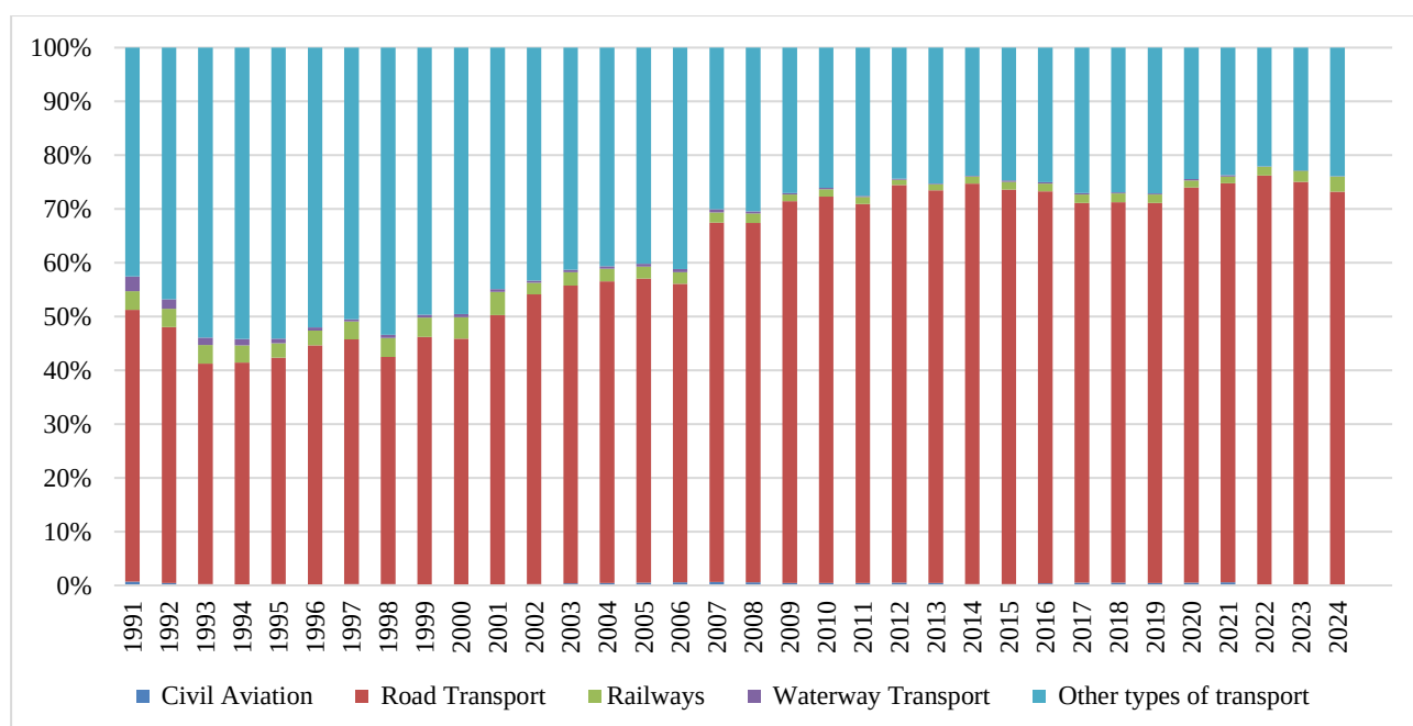
Fig.3.8. Changes in the structure of emissions from fuel combustion in category 1.A.3 Transport, %
