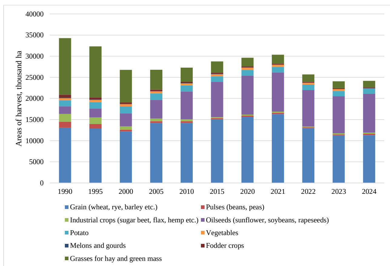
Fig. 6.2. Structure of areas of crops grown on Croplands
