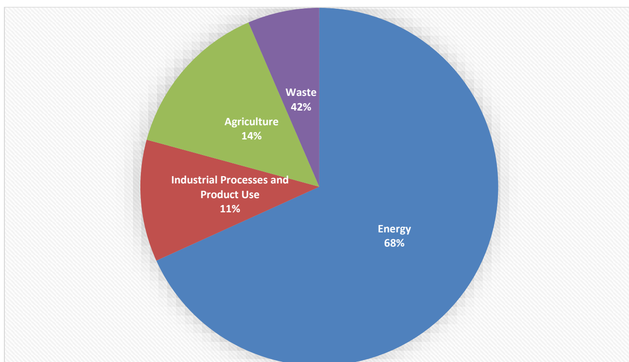
Fig. ES.3.1. The GHG emission structure by sources in 2024
