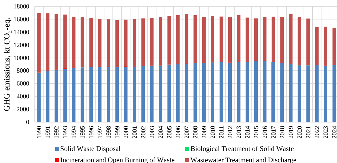
Fig. 7.1. GHG emissions in the “Waste” sector, 1990-2024
