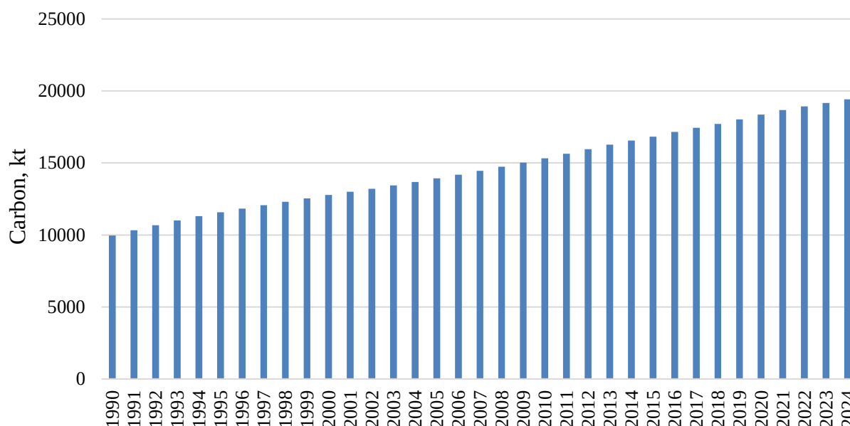
Fig. 7.5. Accumulated long-term storage carbon at MSW dumps, 1990-2024
