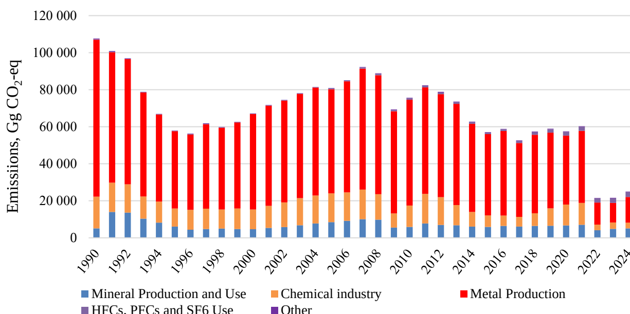
Fig. 4.2. Direct action greenhouse gas emissions in the major categories of the sector Industrial Processes and Product Use, kt CO 2 -eq
