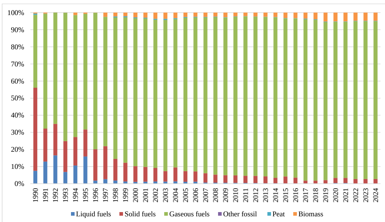
Fig. 3.14. Changes in the structure of fuel consumption in subcategory 1.A.4.b Residential Sector
