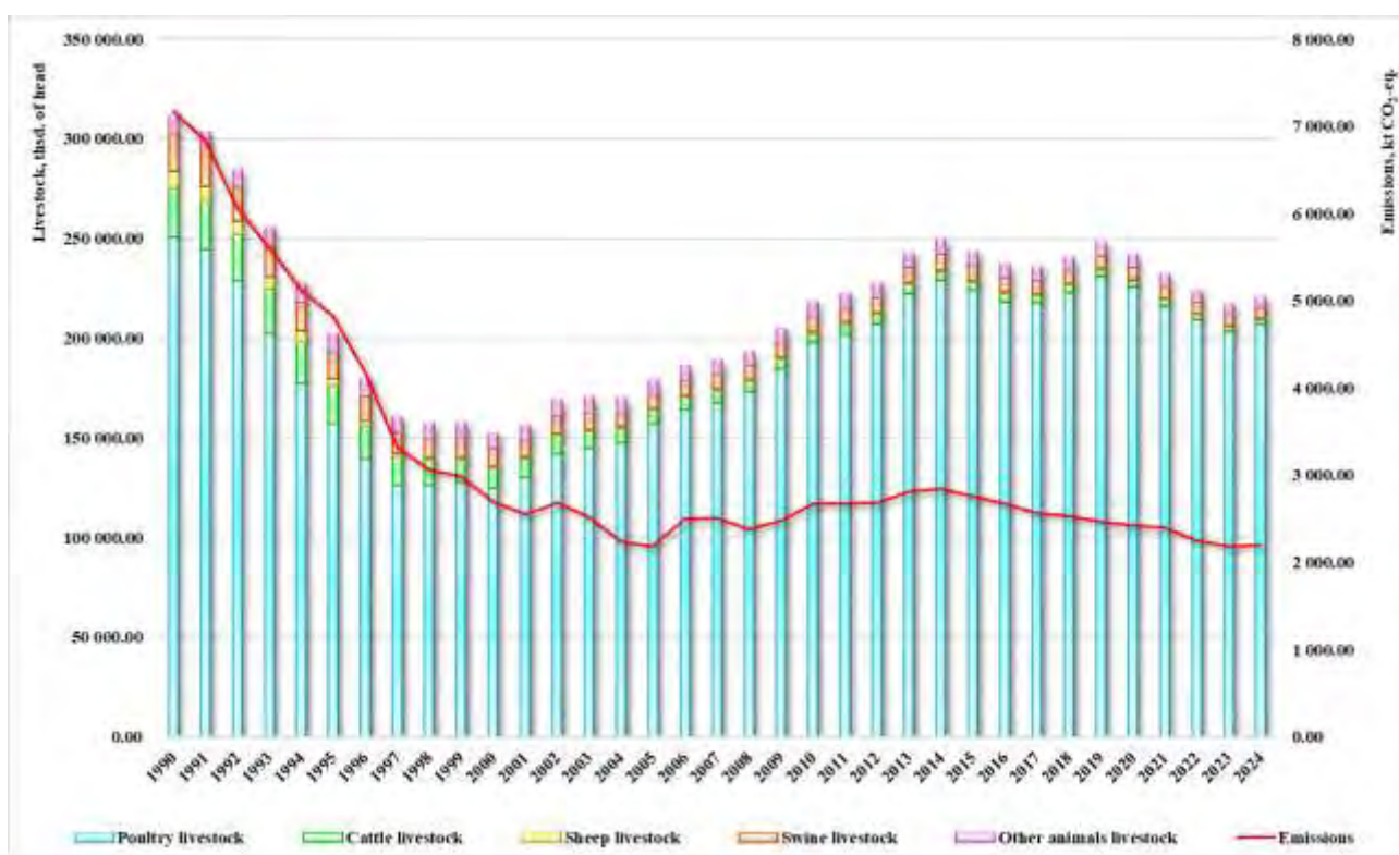
Fig. 5.8. Emission trends in category 3.B Manure Management, and those of cattle, swine, poultry and other animals' livestock
