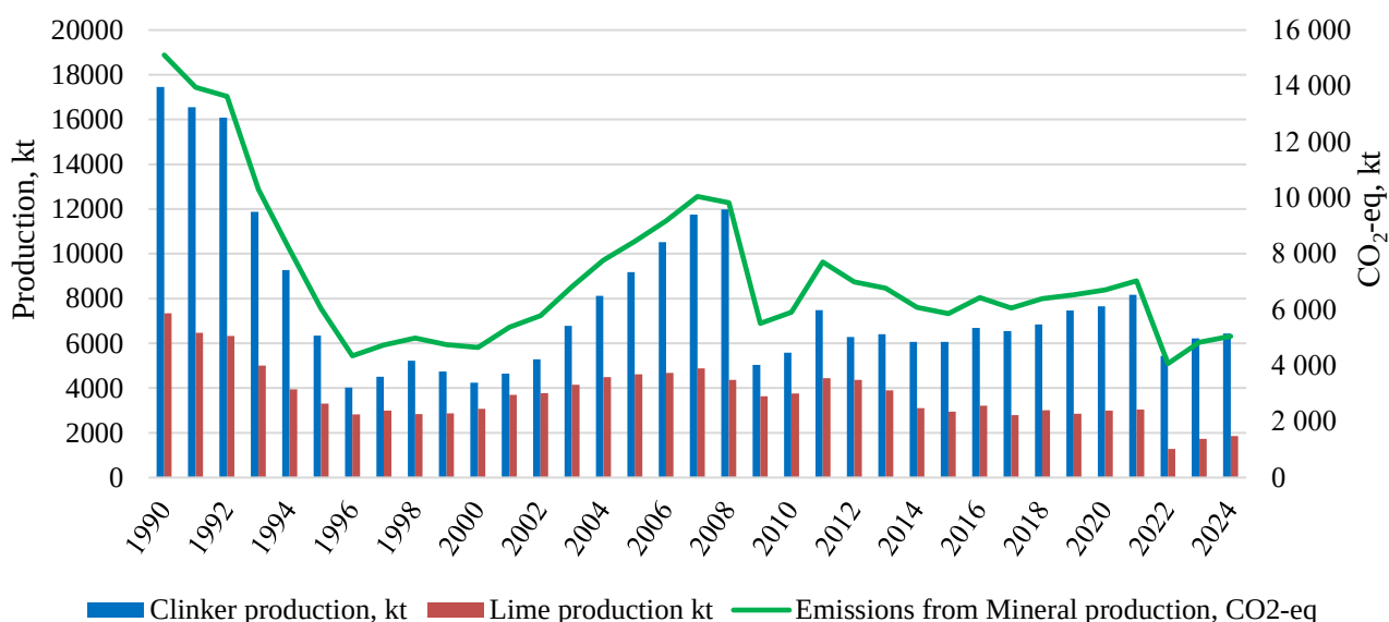
Fig. 4.4. CO 2 emissions from key categories in Mineral industry, kt
