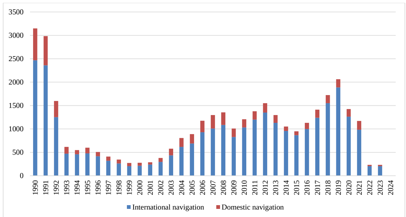
Fig. 3.11. GHG emissions from domestic and international navigation
