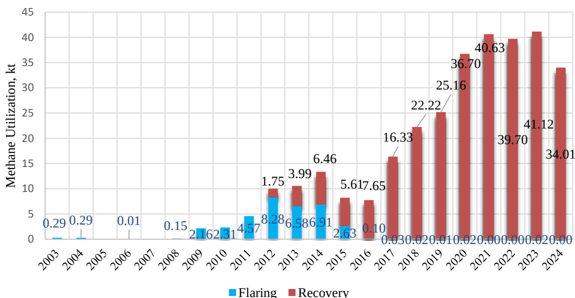
Fig. 7.4. Methane utilization at MSW landfills in Ukraine, 2003-2024
