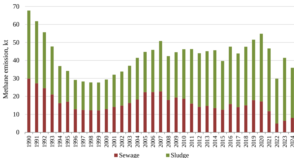
Fig. 7.14. Methane emissions from industrial sewage and sludge treatment in Ukraine, 1990-2024
