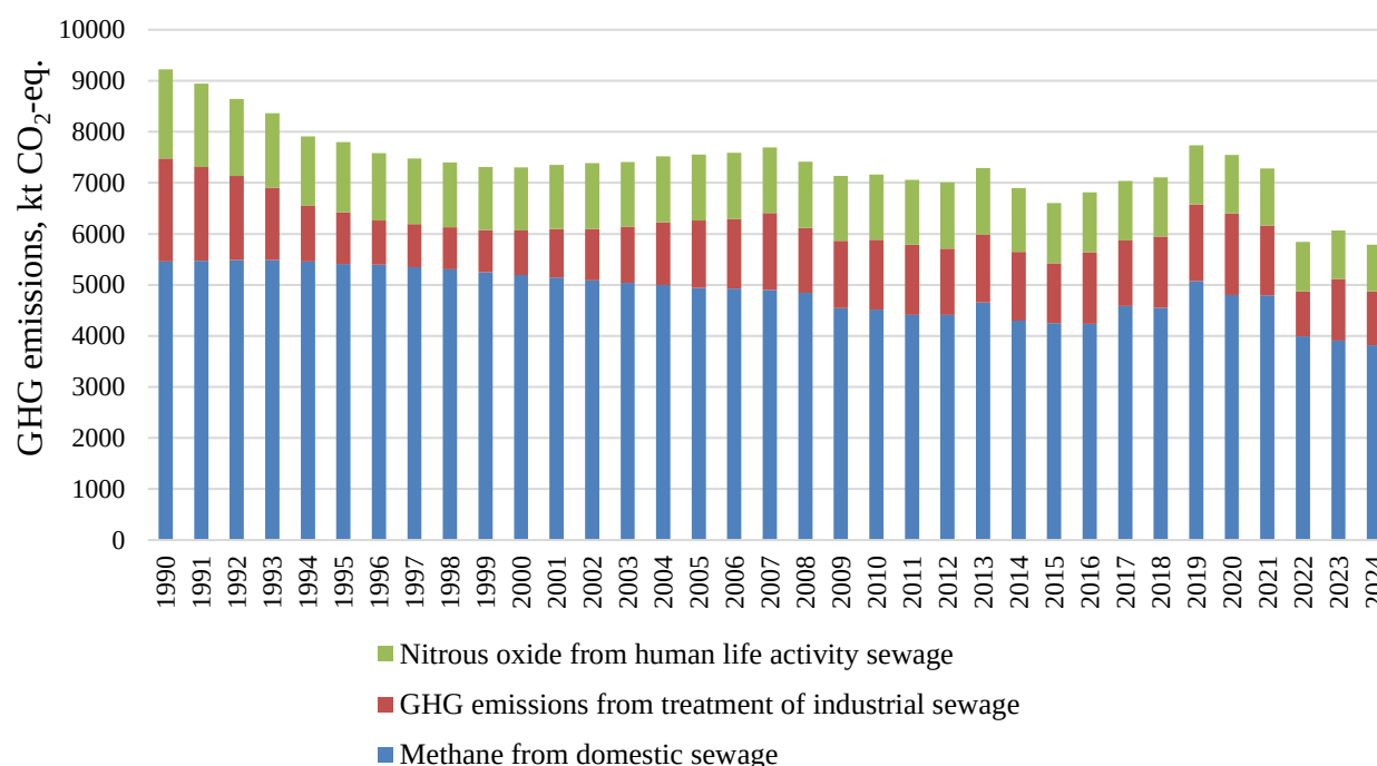
Fig. 7.8. Greenhouse gas emissions from wastewater treatment in Ukraine, 1990-2024
