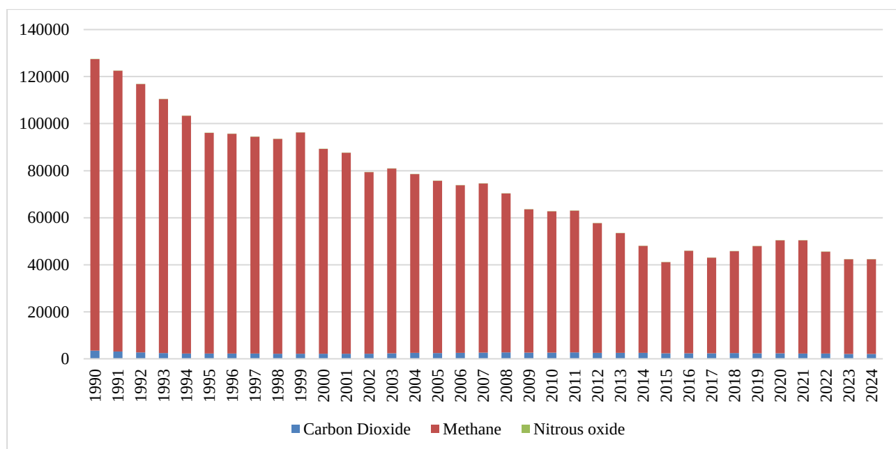
Fig. 3.15. Greenhouse gas emissions in category 1.B Fugitive Emissions from Fuels (sectoral approach), kt CO 2 -eq
