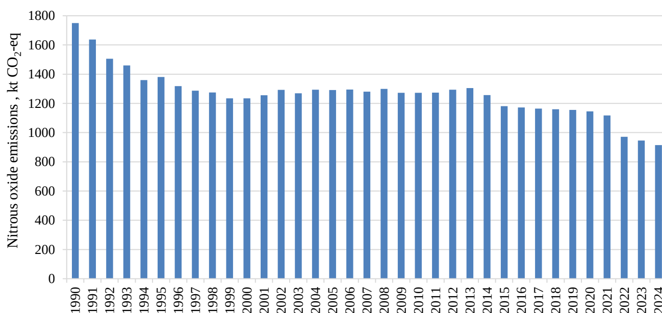
Fig. 7.11. Nitrous oxide emissions from human wastewater in Ukraine, 1990-2024
