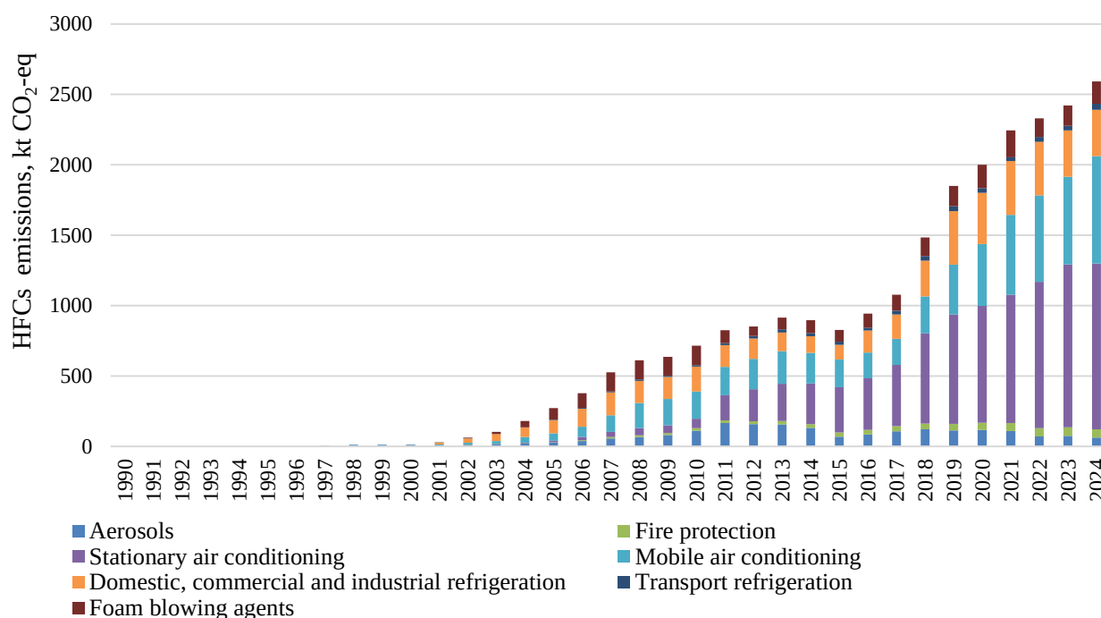
Figure 4.9 The emission trends of HFCs within the IPPU sector
