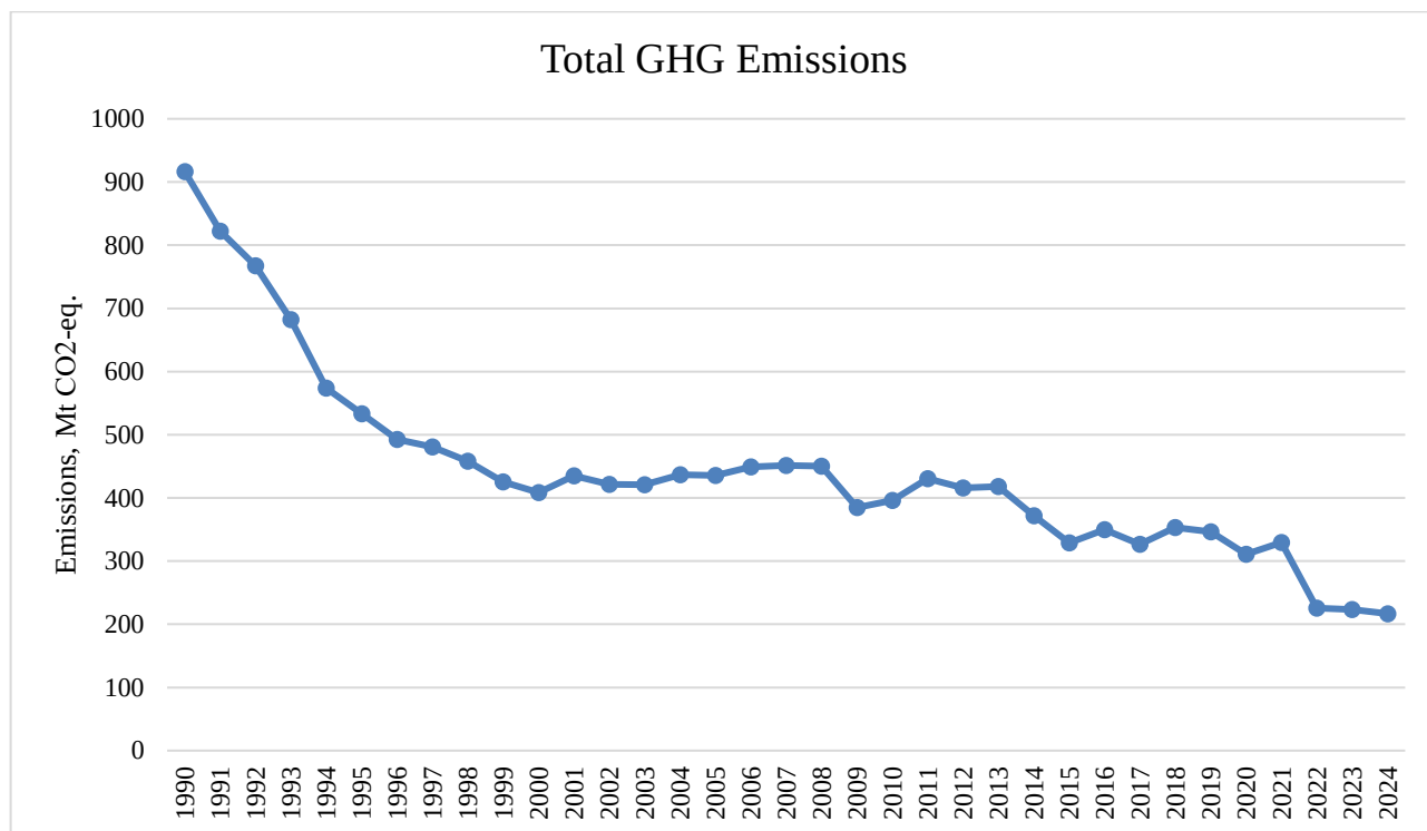
Fig. 2.1. GHG emissions in Ukraine (including LULUCF), Mt CO 2 -eq.
