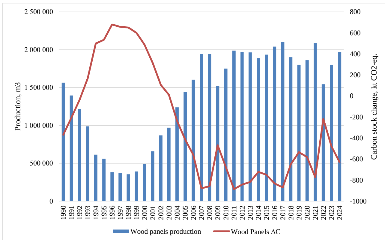
Fig. 6.9. Production and Carbon stock changes in the Wood-based Panels subcategory
