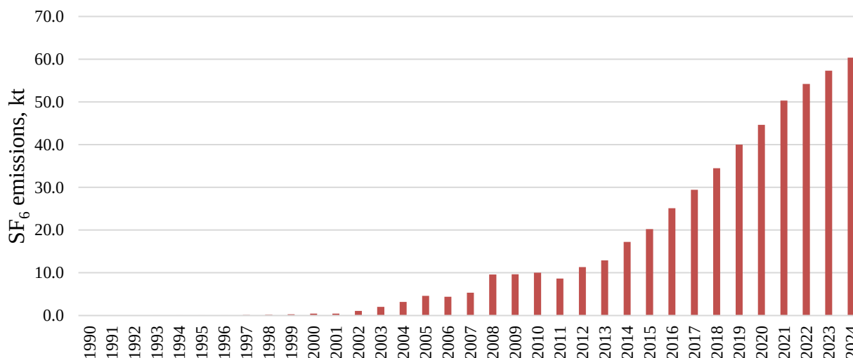
Figure 4.10. SF 6 emissions from category 2.G.1
