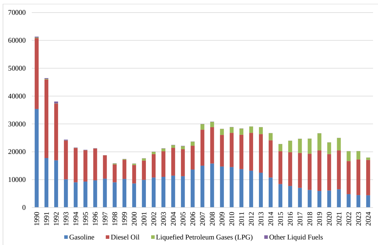
Fig. 3.10. GHG emissions in category 1.A.3.b Road Transport by fuels, for 1990-2024, kt of CO 2 -eq.
