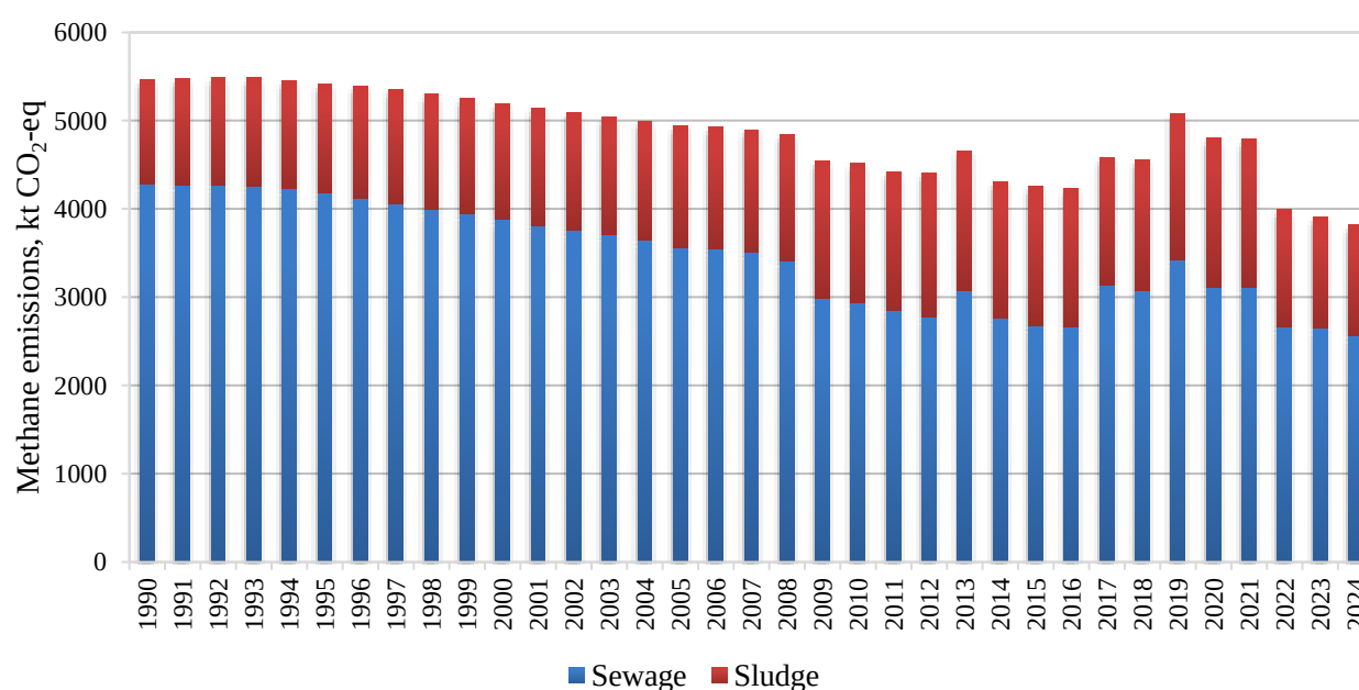
Fig. 7.9. Methane emissions from domestic sewage and sludge treatment in Ukraine, 1990-2024
