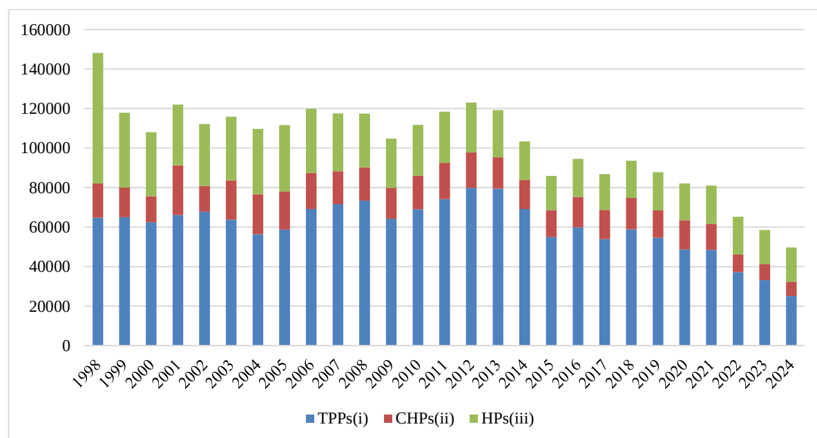
Fig.3.6. The structure of GHG emissions in the category 1.A.1.a “Electricity and Heat Production” by energy facilities, 2002-2024
