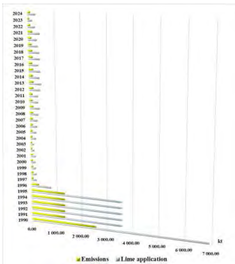
Fig. 5.13. Carbon dioxide emissions from liming of agricultural soils and their dependence on the amount of introduced liming materials
