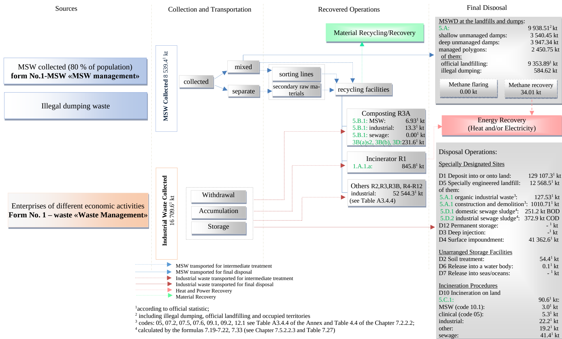
Figure A3.4.3. Waste management practices in Ukraine according to reporting forms No.1-wastes and No.1-MSW, 2024
