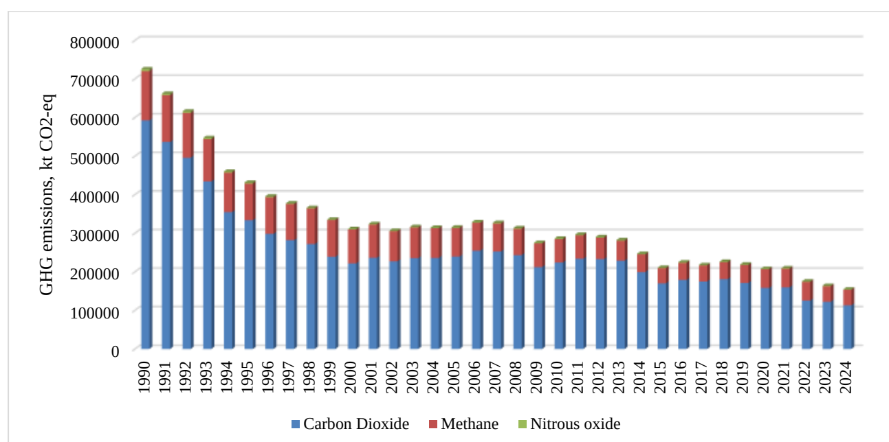
Fig. 3.1. GHG emissions in the "Energy" sector, 1990-2024
