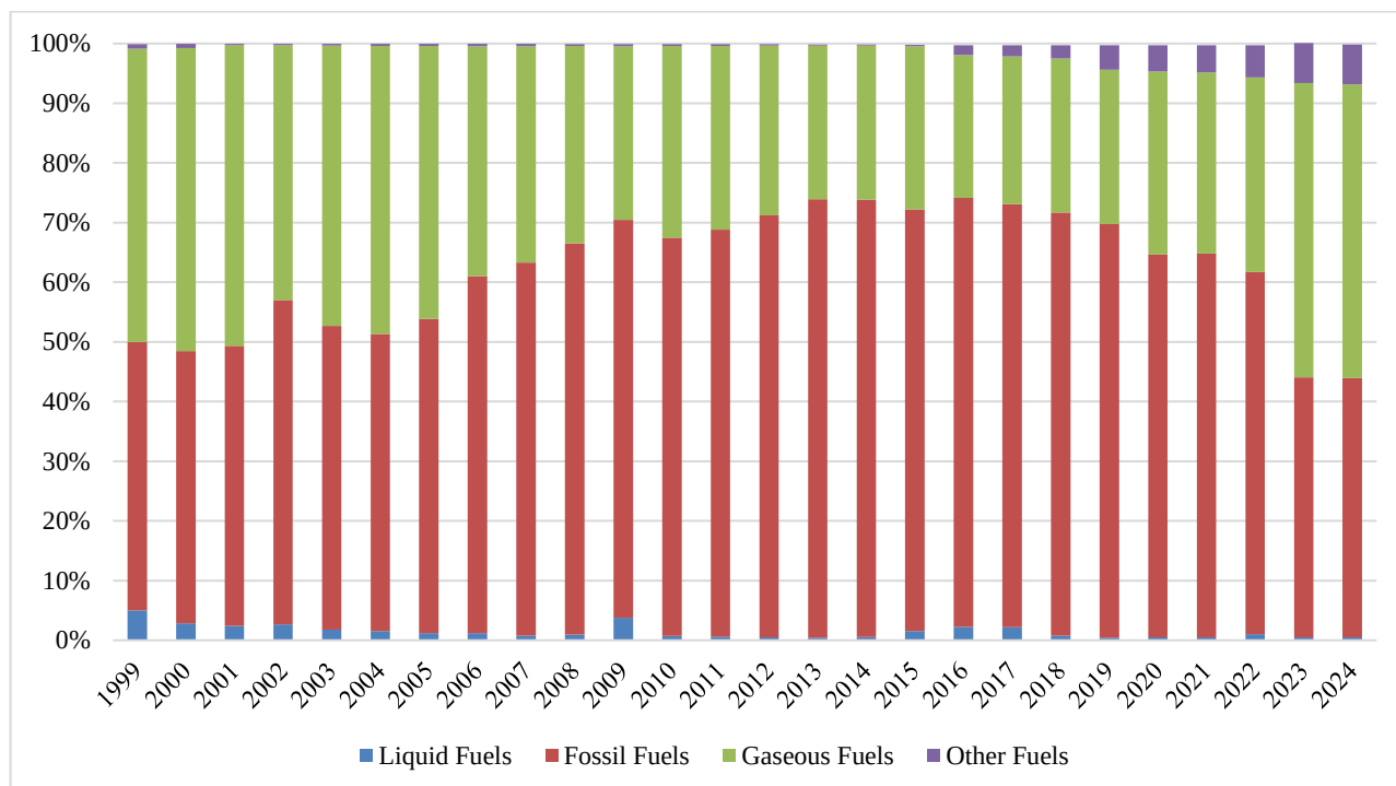
Fig. 3.5. GHG emissions in category 1.A.1.a by fuel groups, share of the category
