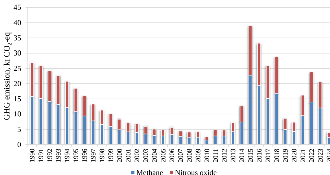
Fig. 7.6. GHG emissions from waste composting in Ukraine, 1990-2024
