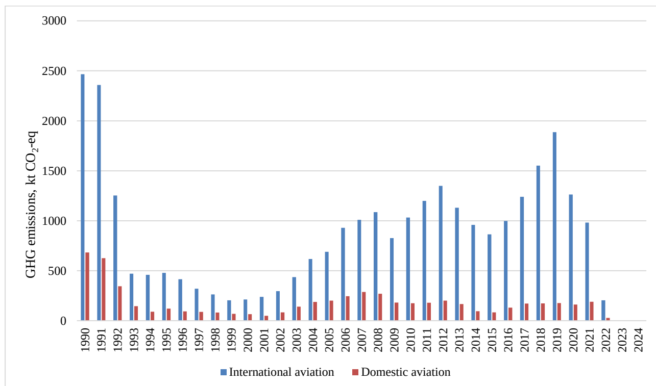
Fig. 3.9. GHG emissions from domestic and international aviation, 1990-2024
