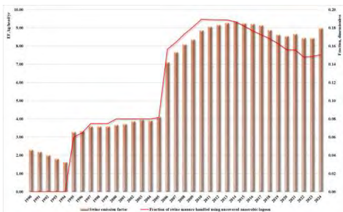
Fig. 5.10. Comparison of swine emission factors and the shares of manure in MMS
