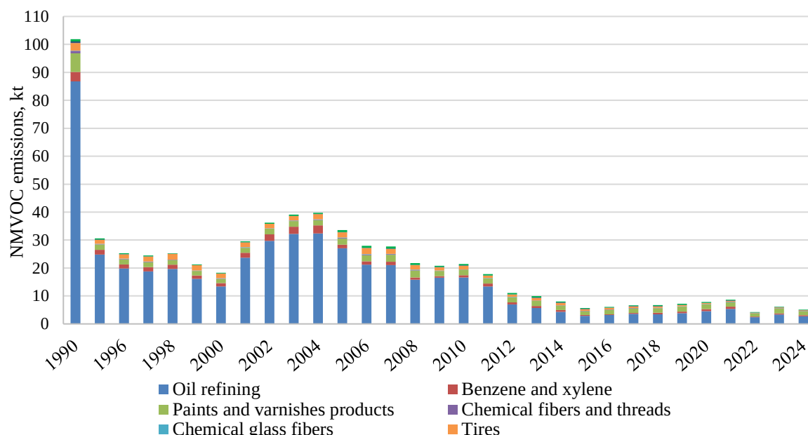
Figure 4.8. NMVOC emissions from chemical production and processing
