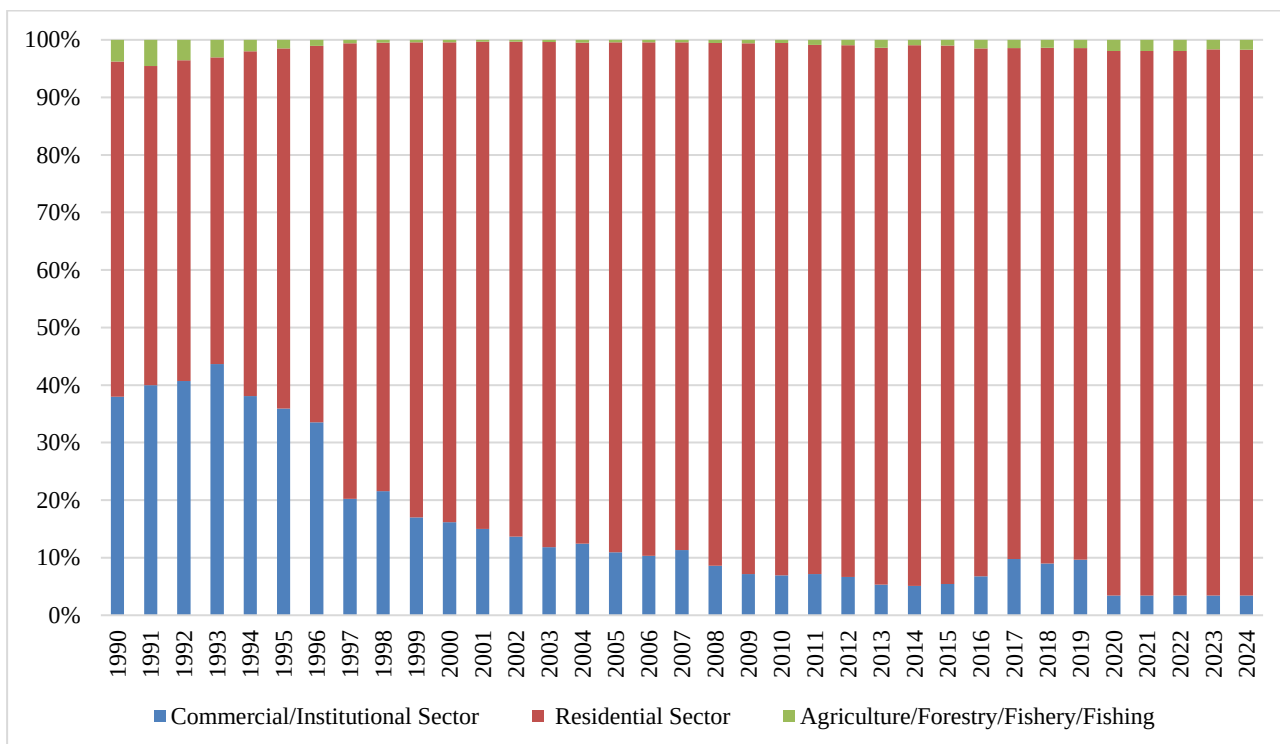
Fig. 3.13. Changes in the structure of emissions from fuel combustion in category 1.A.4 Other Sectors, %
