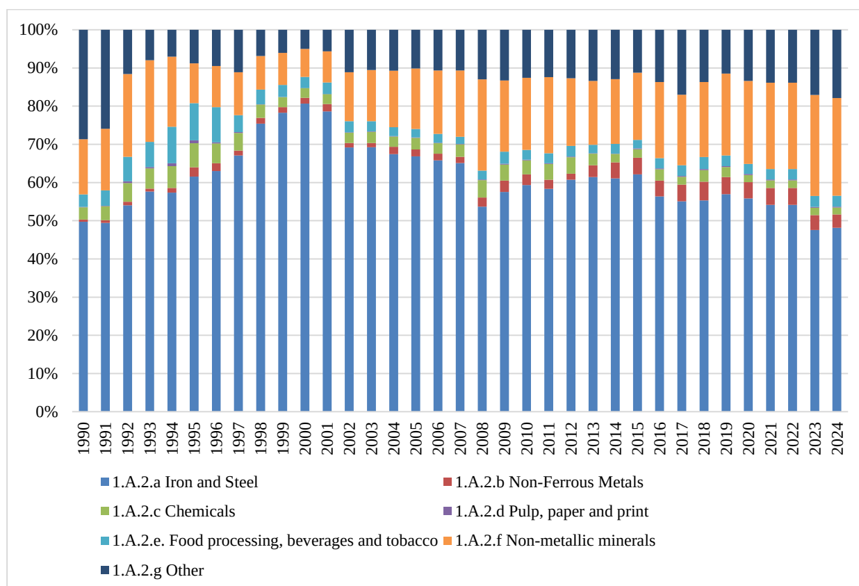
Fig.3.7. Changes in the structure of emissions from fuel combustion in category 1.A.2 "Manufacturing Industries and Construction", %
