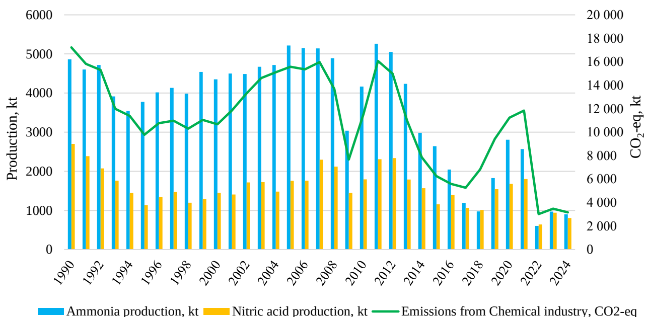
Fig. 4.5. CO 2 -eq emissions from Key categories in Chemical industry, kt
