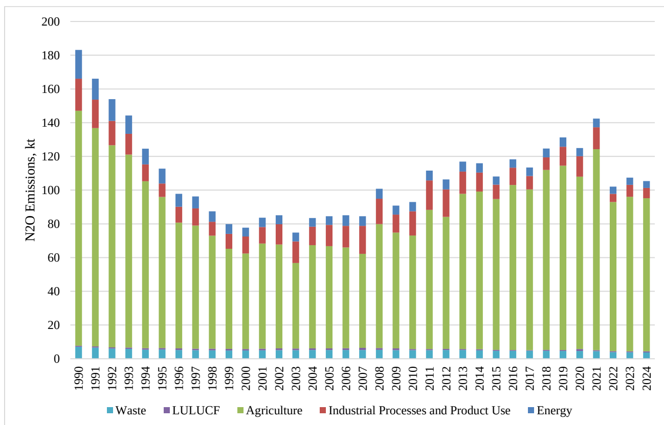
Fig. 2.4. Nitrous oxide emissions in Ukraine by sector, kt
