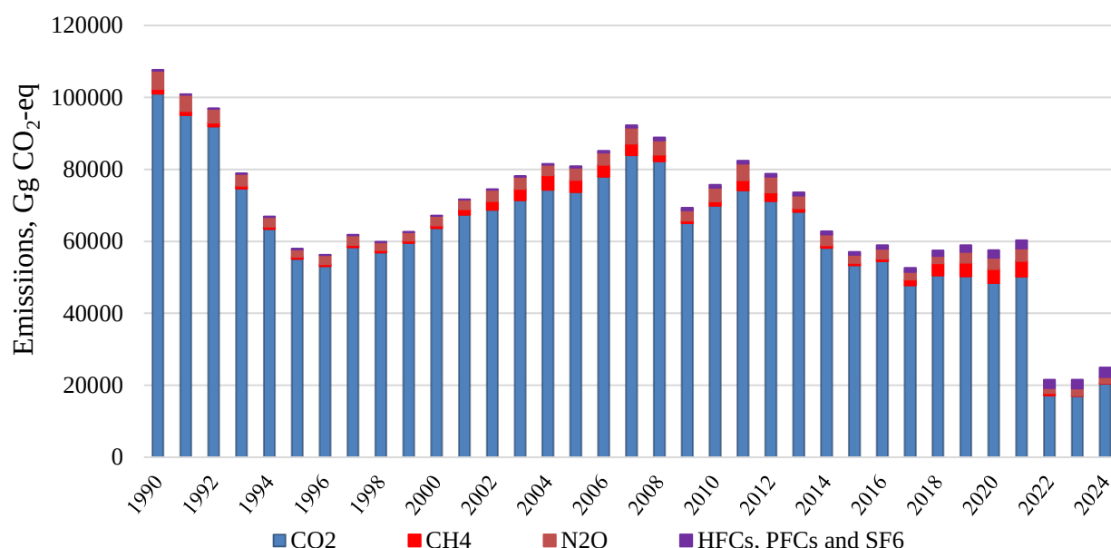
Fig. 4.1. Emissions of CO 2 , CH 4 , and N 2 O in the sector Industrial Processes and Product Use, kt CO 2 -eq
