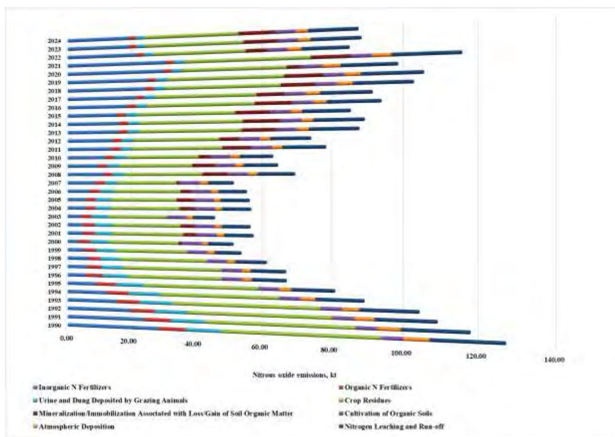
Fig. 5.12. Emission distribution in category 3.D Agricultural Soils
