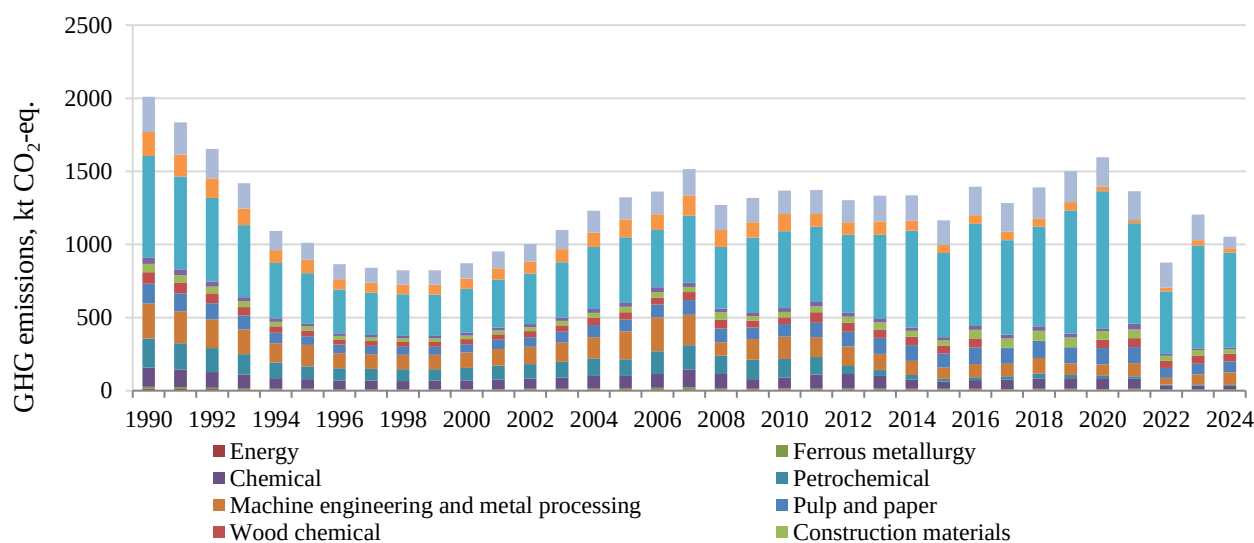
Fig. 7.15. GHG emissions from industrial sewage treatment by industries in Ukraine, 1990-2024
