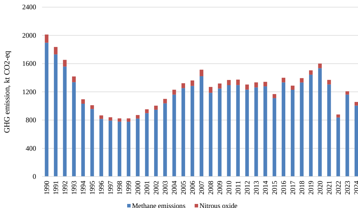
Fig. 7.13. GHG emissions from industrial sewage treatment in Ukraine, 1990-2024
