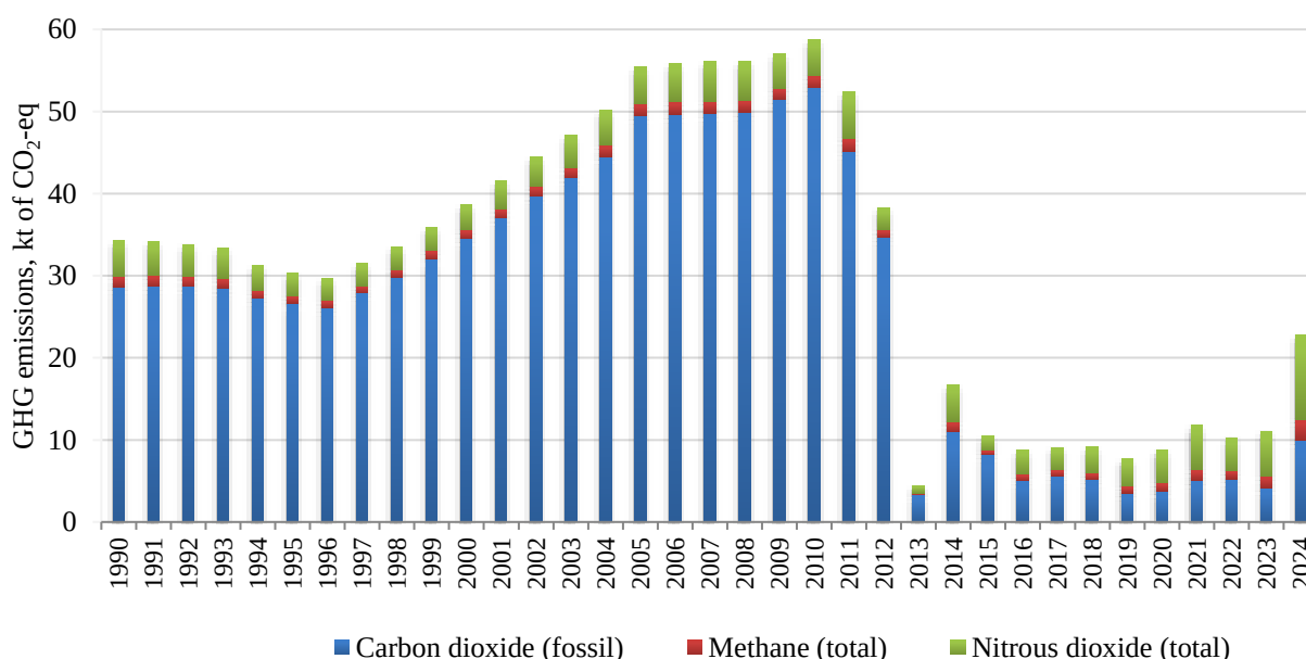
Fig. 7.7. GHG emissions from waste incineration without energy recovery in Ukraine, 1990-2024
