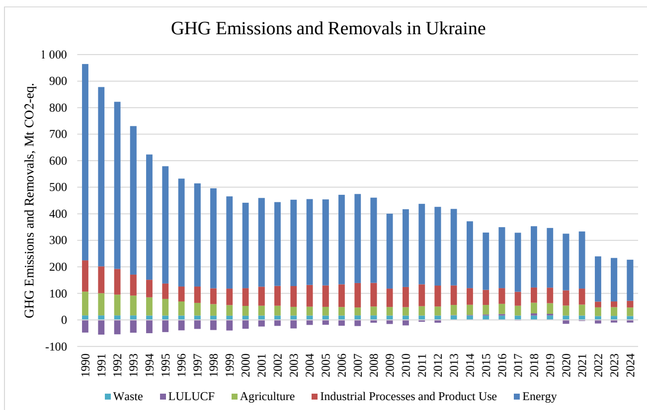
Fig. 2.7. GHG emissions and removals by sector in Ukraine, Mt CO 2 -eq.
