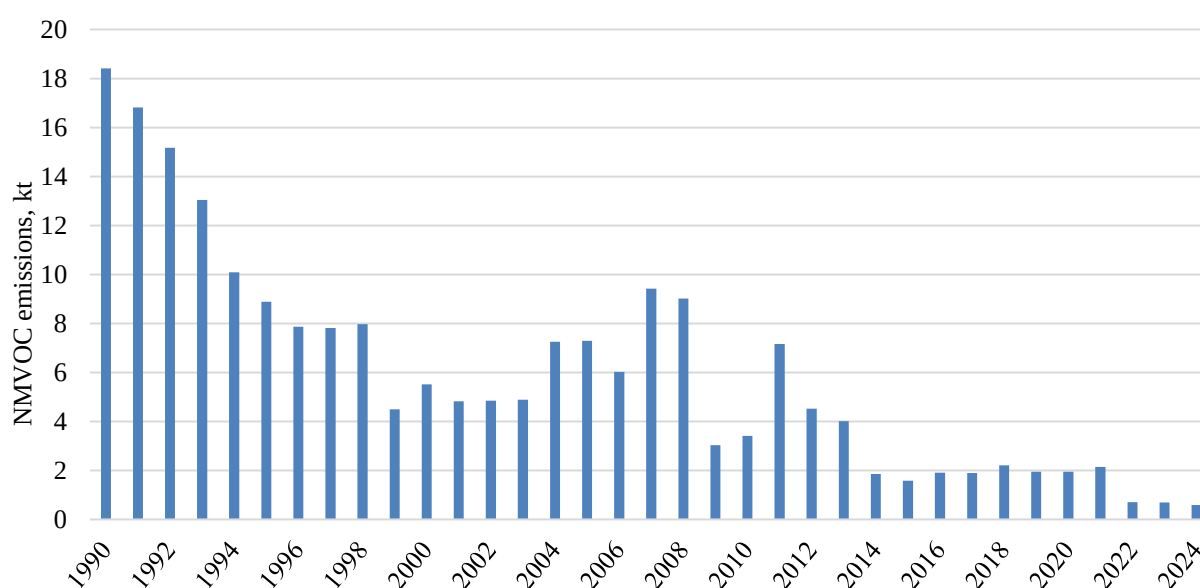
Figure 4.7. NMVOC emissions from degreasing and dry cleaning
