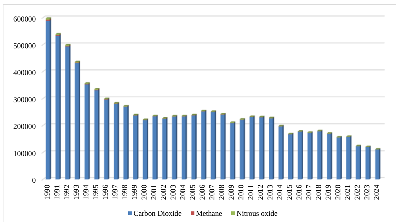
Fig. 3.2. GHG emissions in category 1.A Fuel Combustion Activities (sectoral approach, kt CO 2 -eq.), 1990-2024
