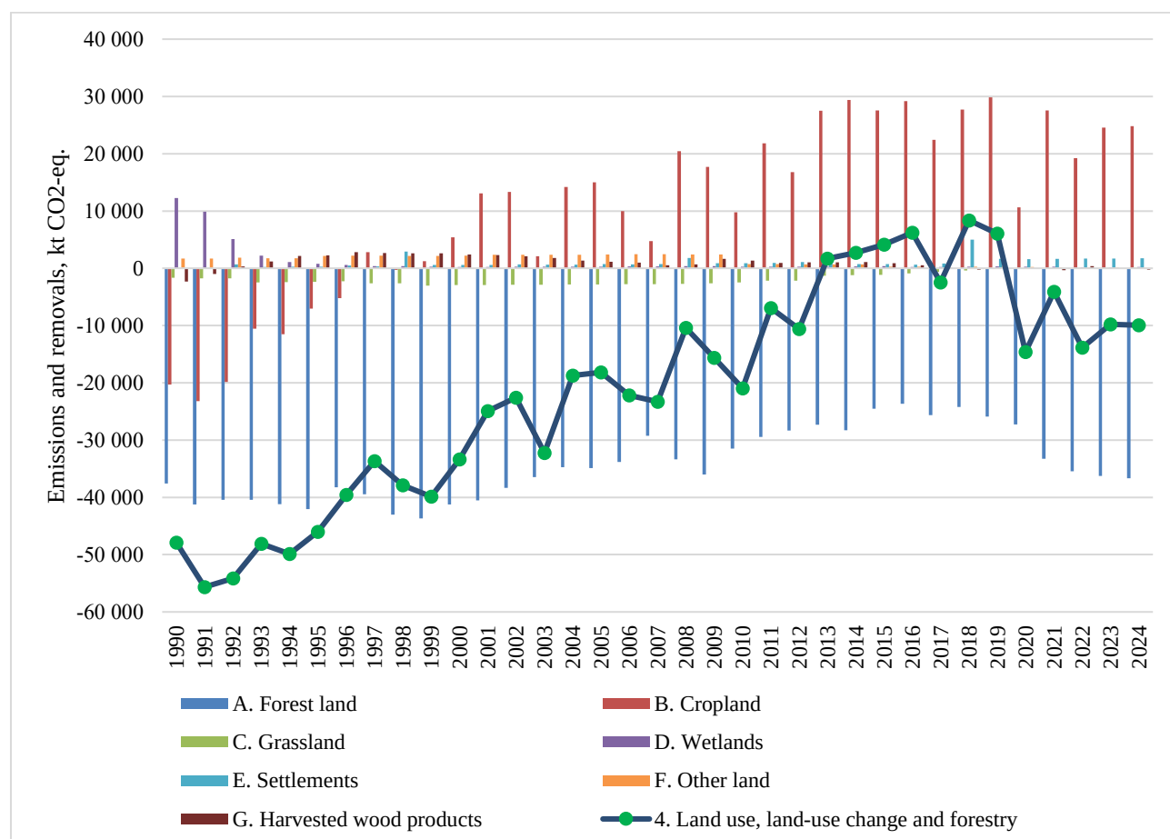
Fig. 6.1 Emissions and removals in the LULUCF sector in Ukraine in 1990-2024
