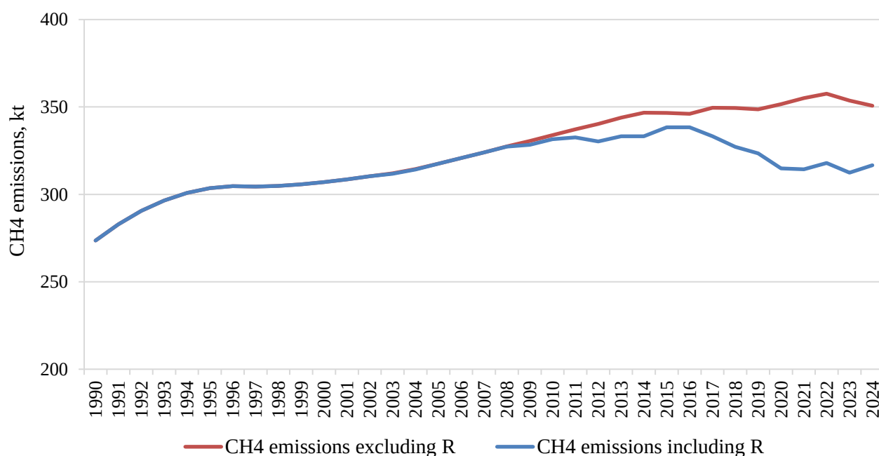
Fig. 7.2. Methane emissions from solid waste disposal, 1990-2024
