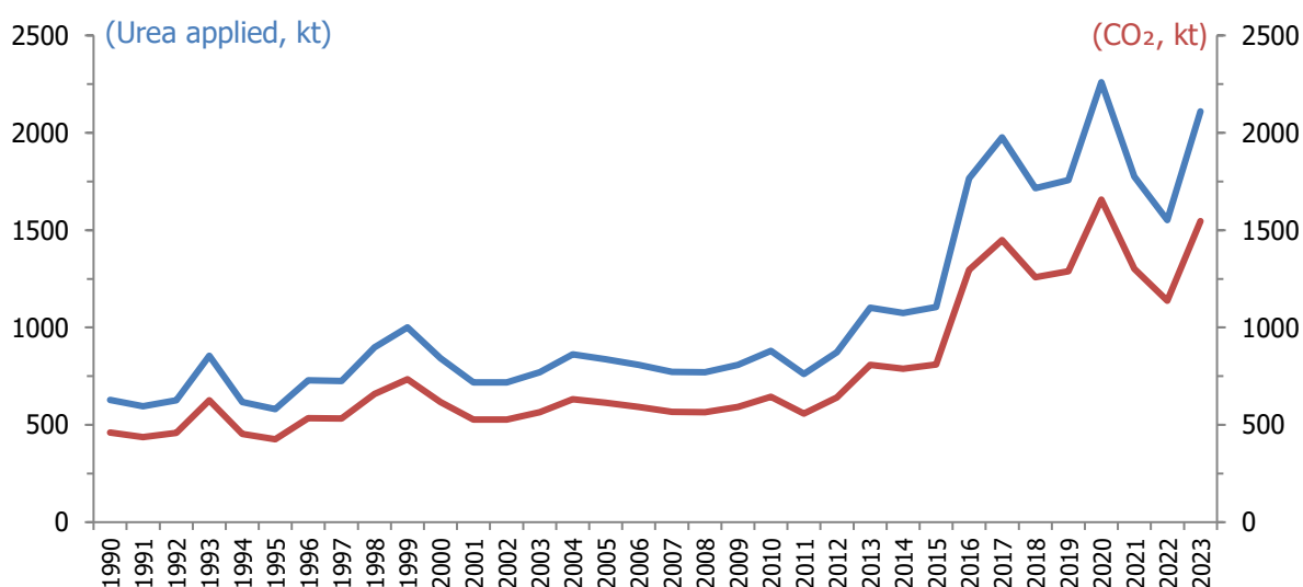
Figure 5.12 Urea application and emitted CO 2 , 1990–2023
