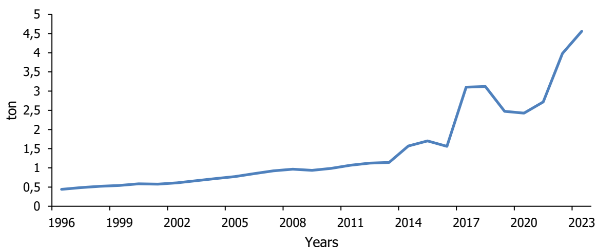
Figure 4.27 SF 6 emissions, 1996-2023
