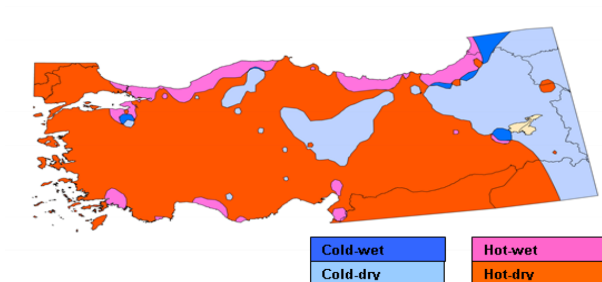
Figure 5.11 Climate Map of Türkiye
