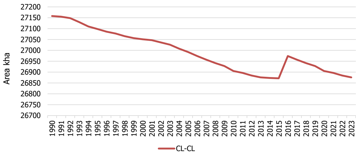
Figure 6.9 The change in area of CL-CL
