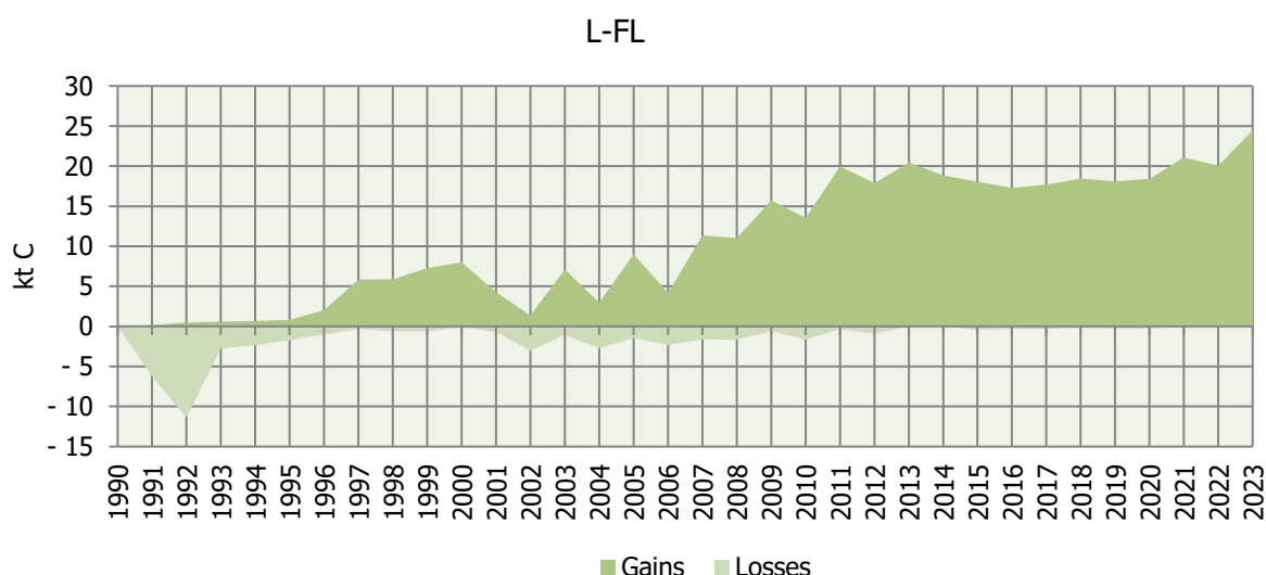
Figure 6.6 Gains and losses in Land Converted to Forest land subcategory (L-FL)
