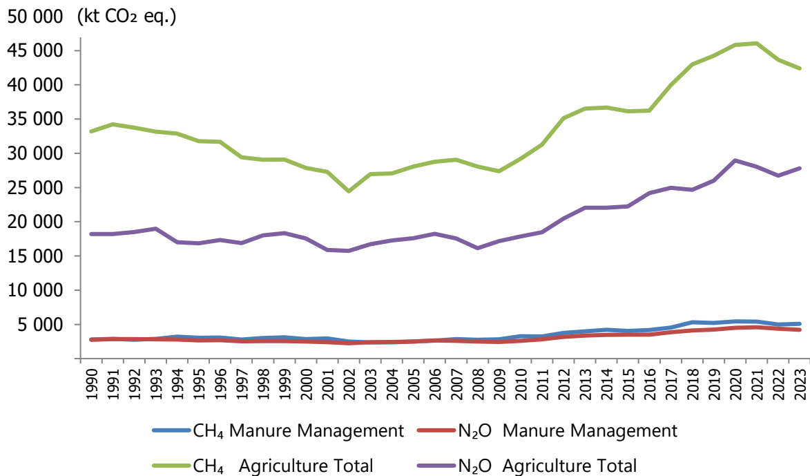
Figure 5.8 Comparing CH 4 and N 2 O emission trends, 1990–2023
