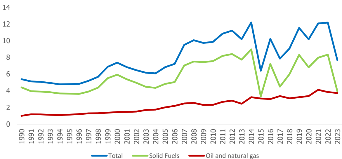
Figure 3.2 Fugitive emissions, 1990-2023
