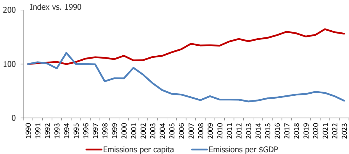
Figure 2.2 Trends in emissions per capita and dollar of GDP relative to 1990
