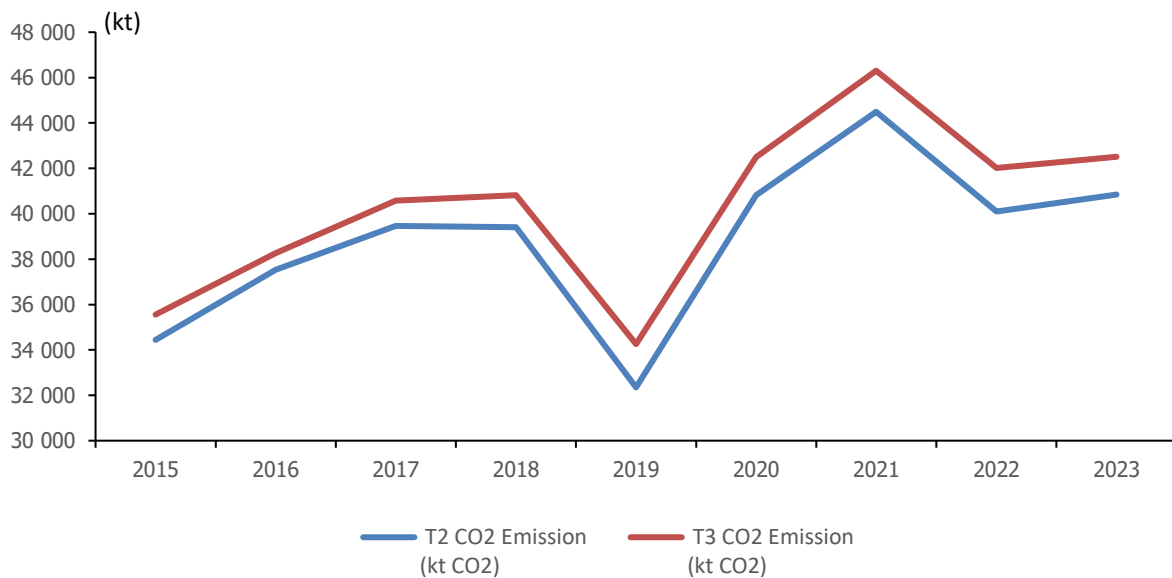
Figure 4.5 Consistent Overlap of T2 and T3 Estimations, 2015-2023
