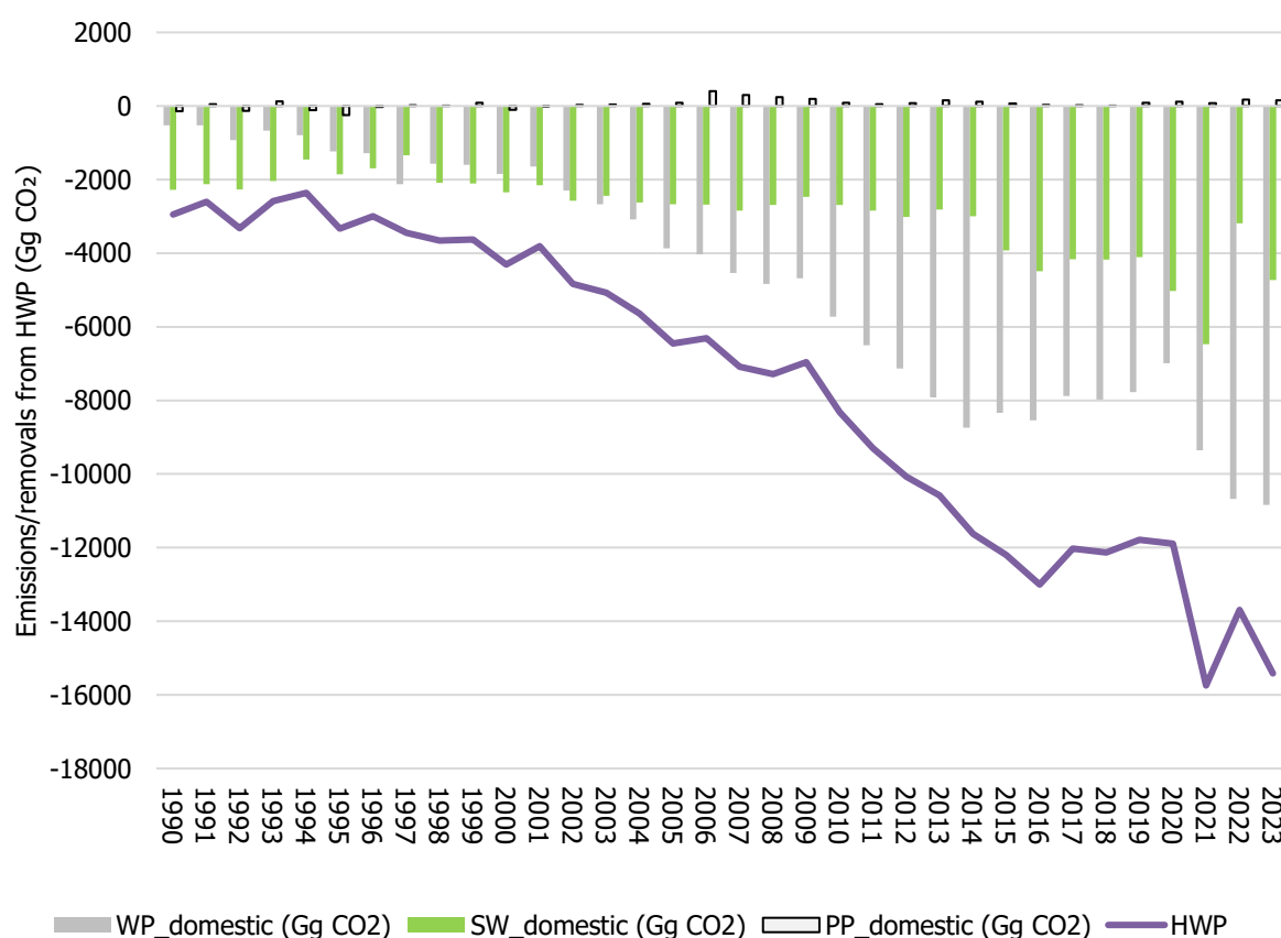
Figure 6.21 Emissions and removals in HWP pool
