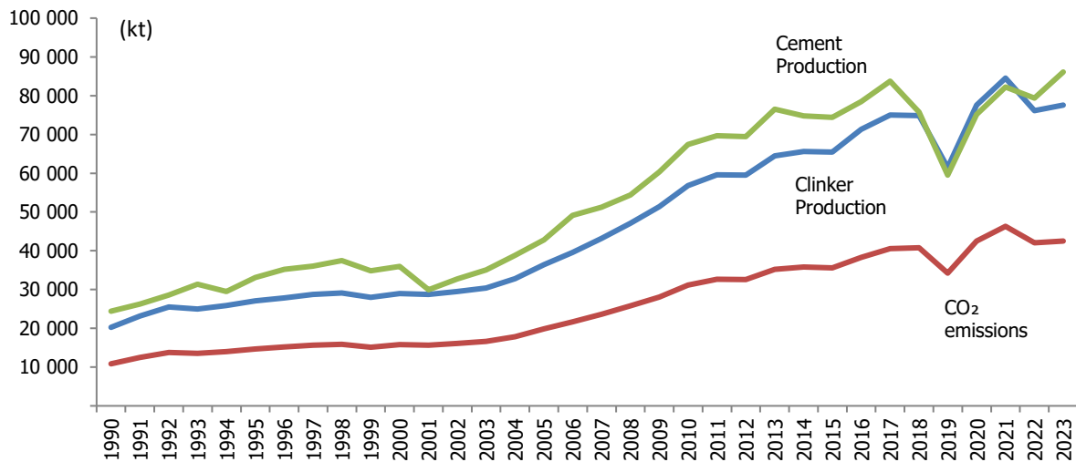
Figure 4.4 Trend at clinker, cement production and related CO 2 emissions, 1990-2023
