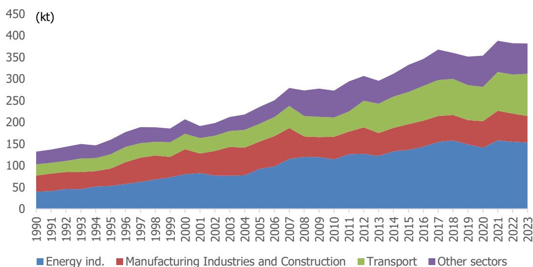
Figure 3.3 CO 2 emissions from fuel combustion, 1990-2023
