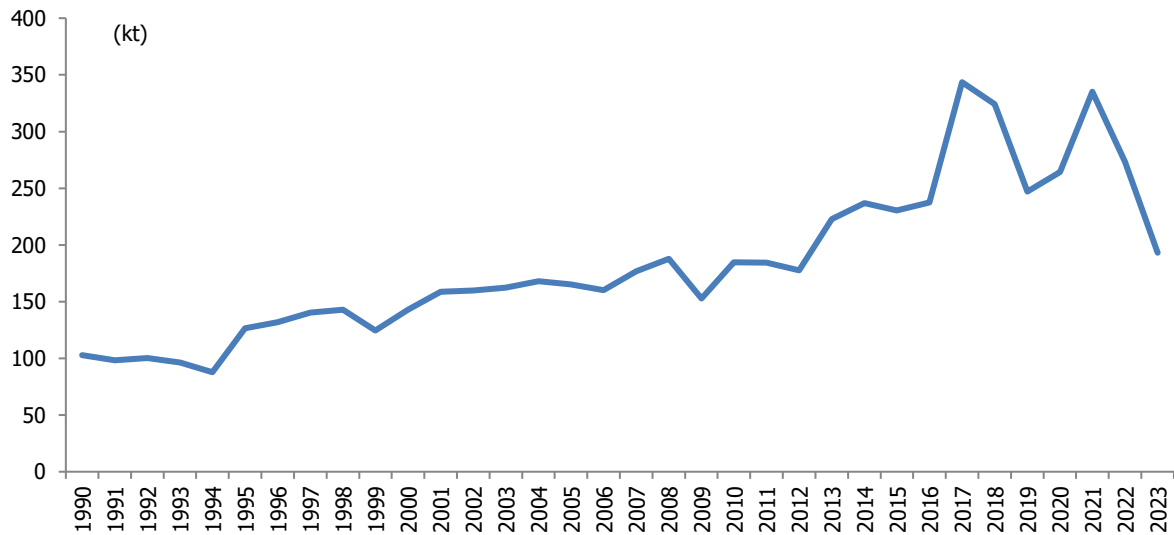
Figure 4.12 CO 2 emissions from magnesia production, 1990-2023
