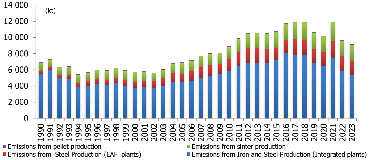
Figure 4.19 CO 2 emissions allocations within the 2.C.1 category, 1990-2023
