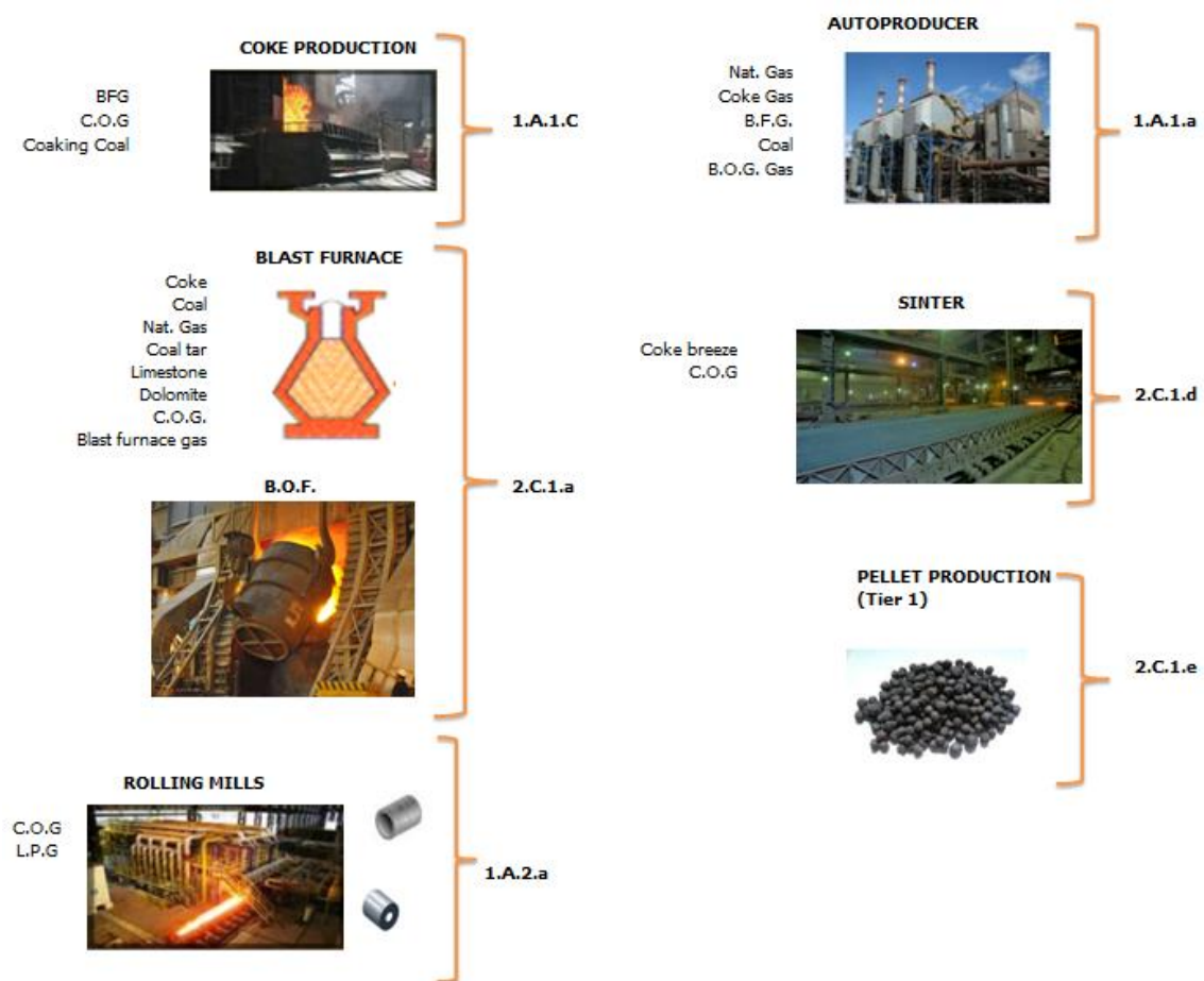
Figure 4.20 Allocations of the emissions from integrated iron and steel plants
