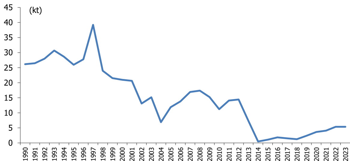
Figure 7.6 CO 2 emissions from open burning of waste, 1990-2023
