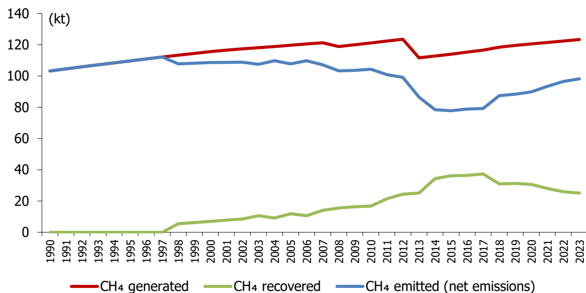
Figure 7.10 CH 4 emissions from domestic wastewater, 1990-2023
