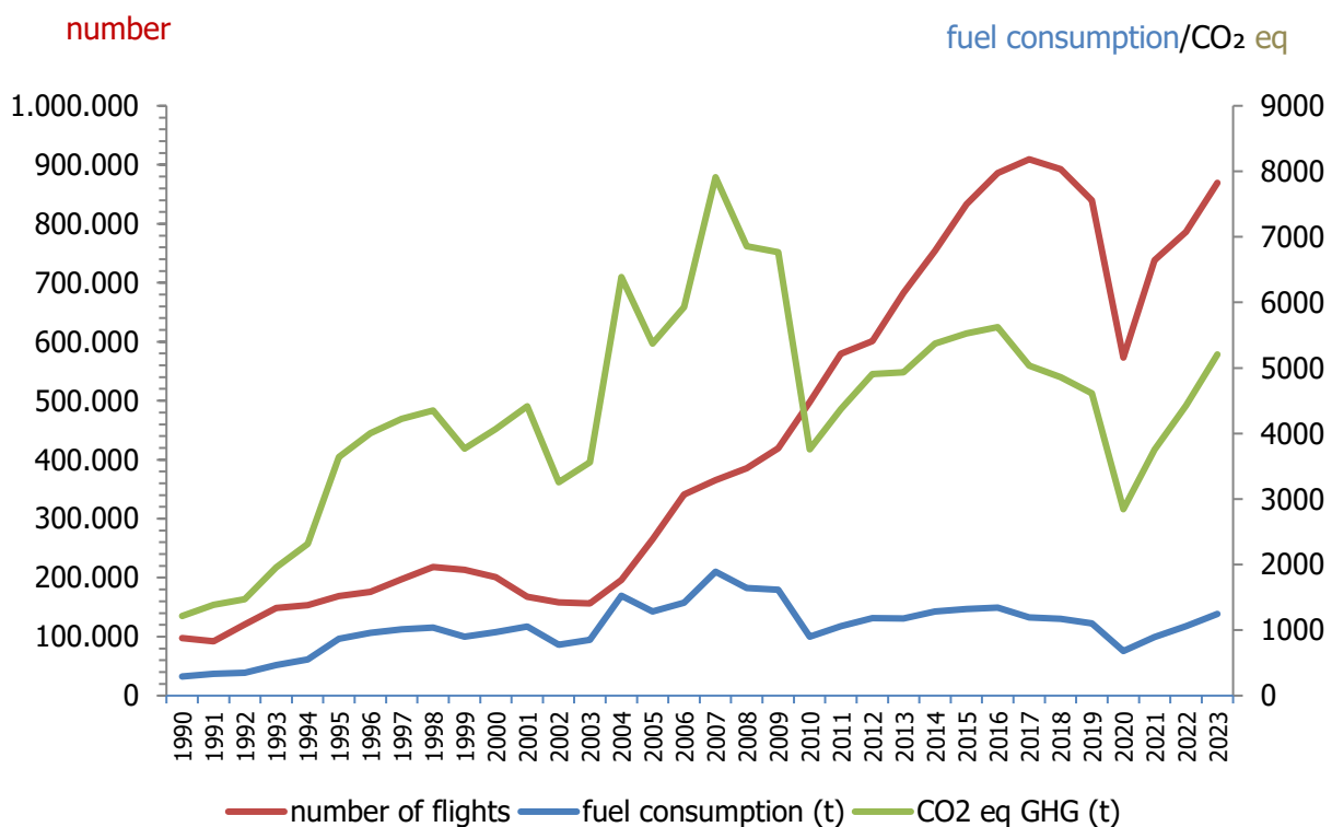
Figure 3.15 Comparison of number of flights, fuel consumption and GHG emissions of civil aviation, 1990-2023
