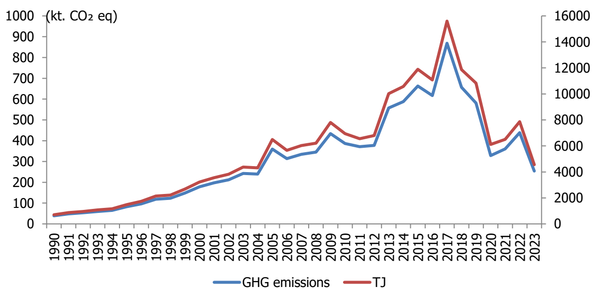
Figure 3.31 GHG emissions from pipeline transport, 1990-2023
