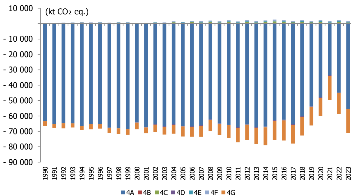
Figure 2.13 Trend of total emissions from the LULUCF sector, 1990-2023
