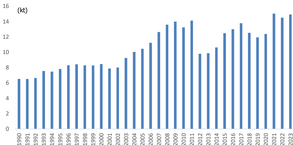
Figure 3.6 N 2 O emissions from fuel combustion, 1990-2023
