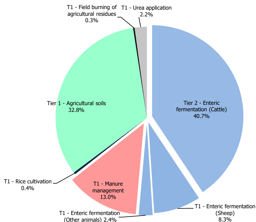
Figure 5.2 Category shares and methods used in the agriculture sector, 2023
