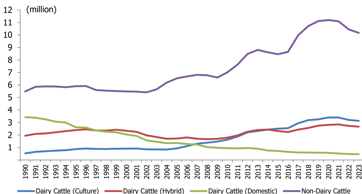
Figure 5.5 Population numbers for cattle categories, 1990–2023
