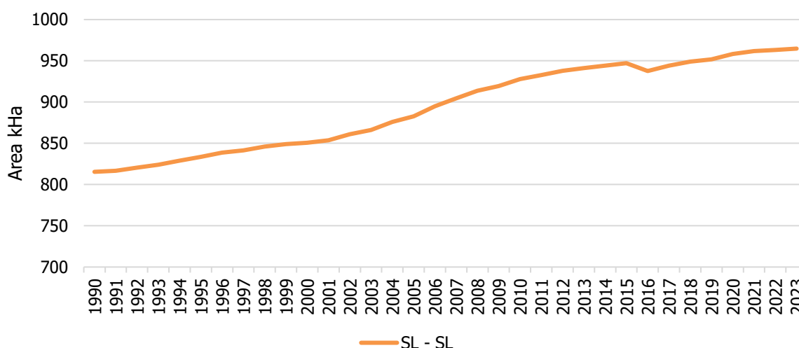
Figure 6.18 The change in area of settlements
