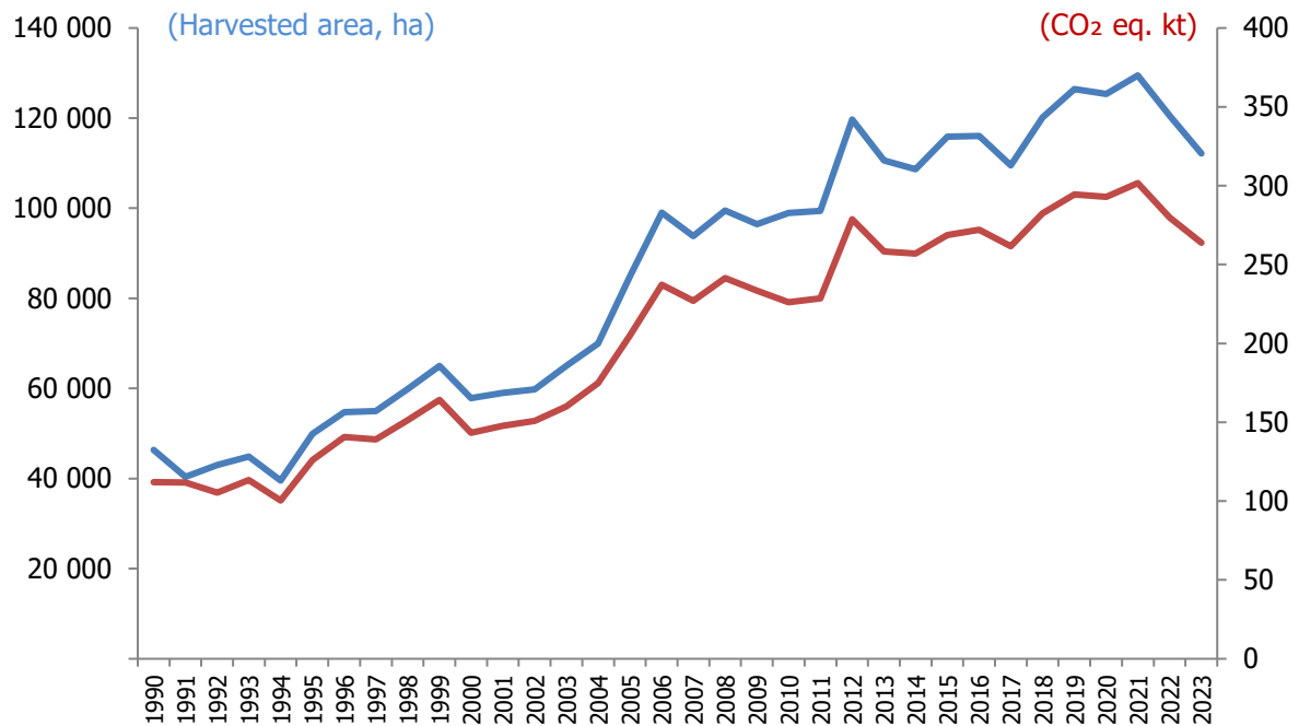
Figure 5.9 Harvested area and emitted CH 4 for rice cultivation, 1990–2023
