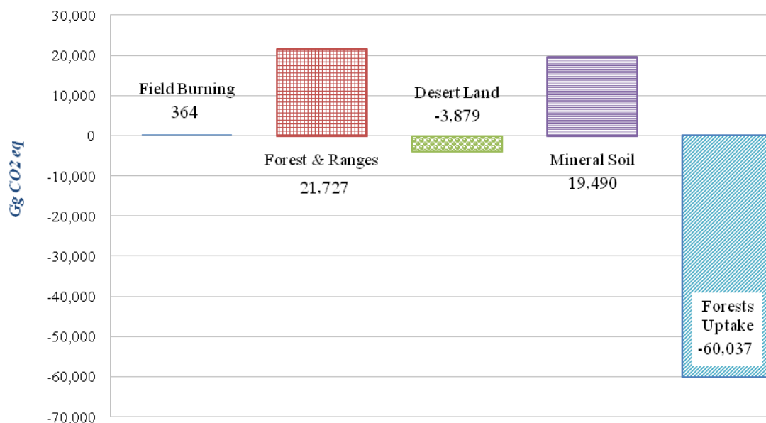
Fig. 2.19 GHG Emissions and Absorption (Sinks) /Retention by LUCF in 1994
