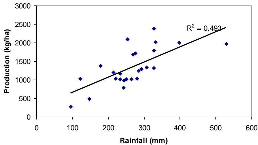
Fig. 3.20 The Relationship between Rainfall and Rainfed Wheat Production in the Hassakeh Governorate
