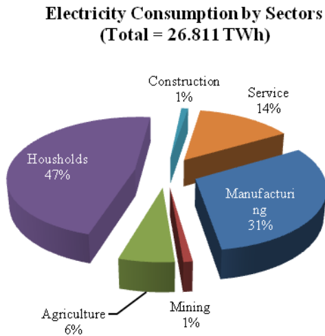
Fig. 3.27 Electricity Consumption by Sector
