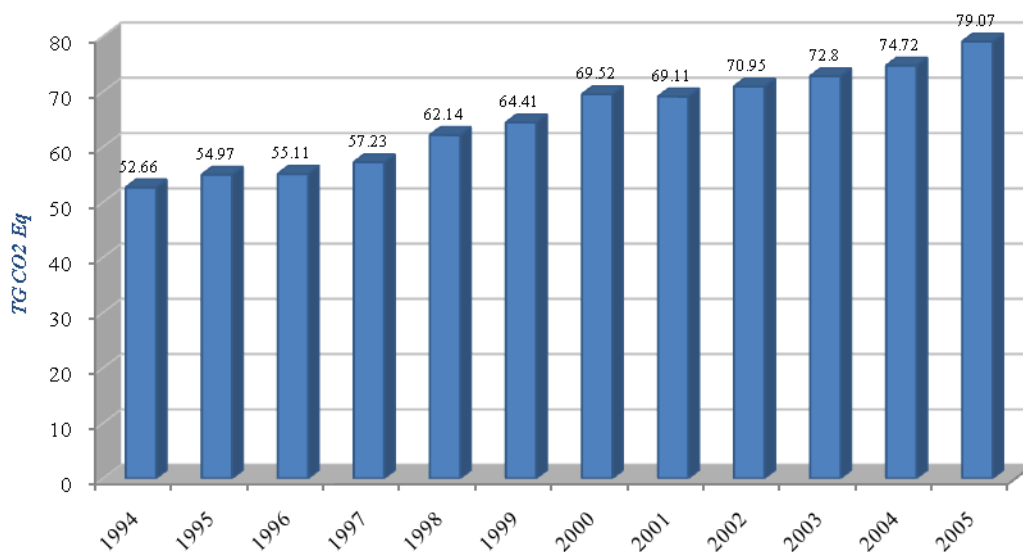
Fig. 2.1 Total Emissions of GHG from 1994 to 2005
