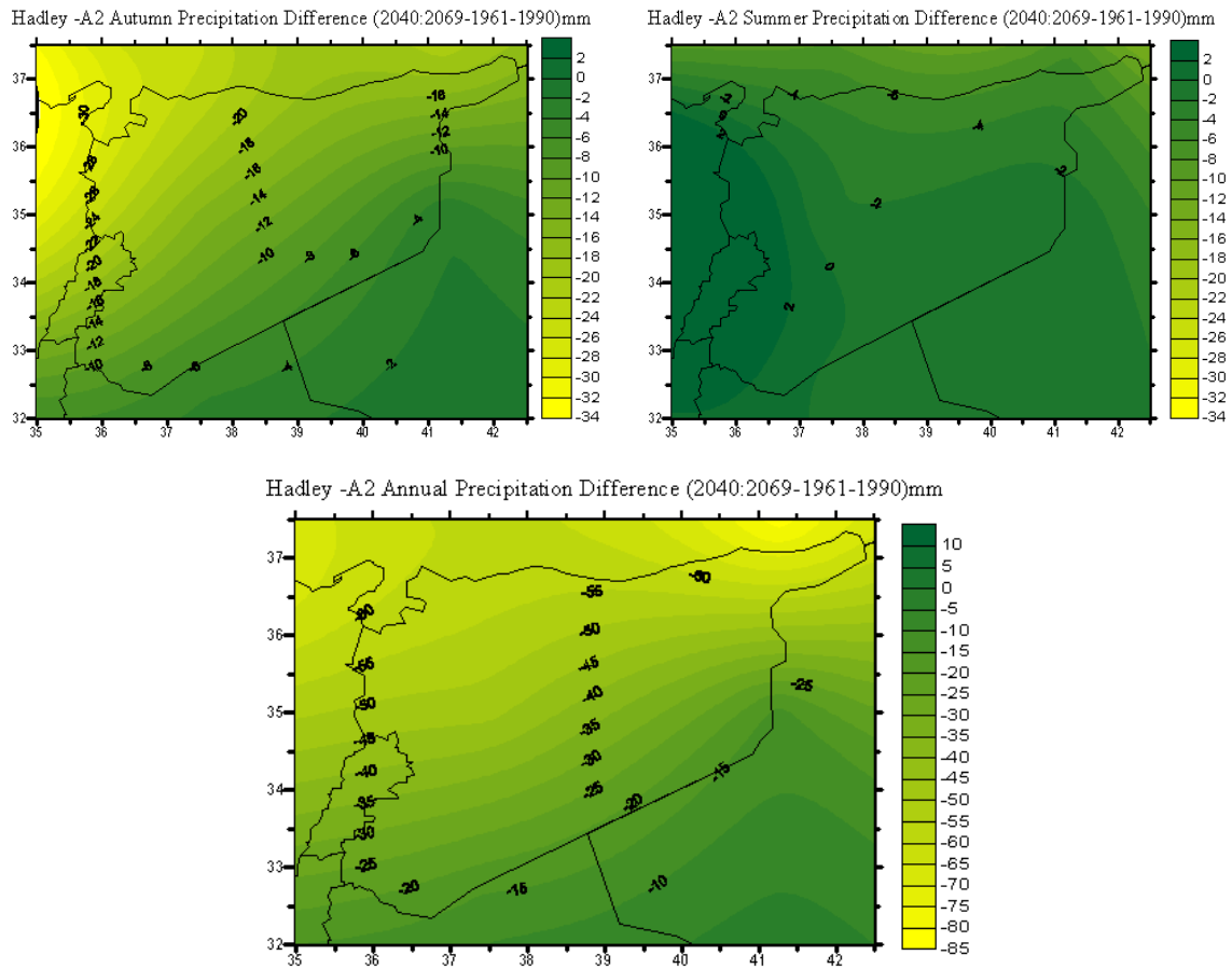
Fig. 3.6 Changes in Seasonal and Annual Precipitations in 2040-2069 (A2 scenario – Hadley Model-CM3)
