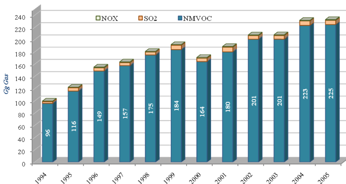
Fig. 2.21 Emissions of NMVOC, SO 2 (Sulfates) and NO x (Nitrates) from Industry
