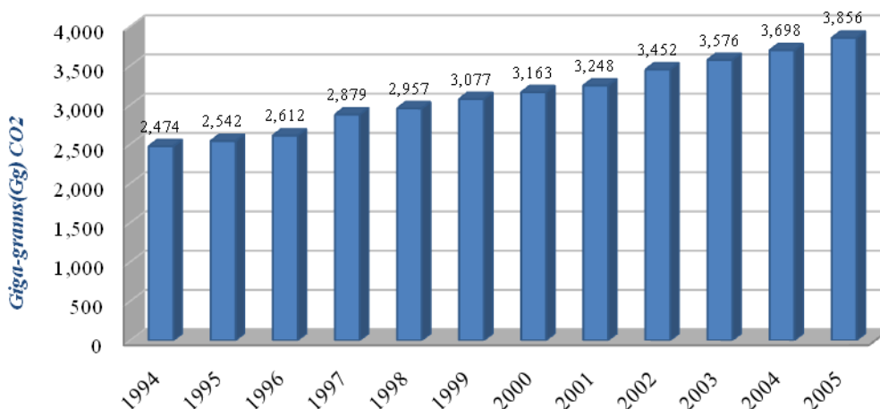
Fig. 2.12 Total GHG Emissions from the Waste Sector in CO 2 eq during the 1994-2005 Period
