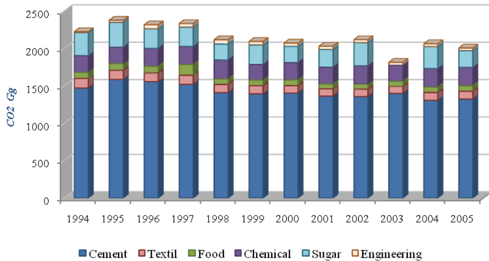
Fig. 4.8 Energy Consumed by Various Industries
