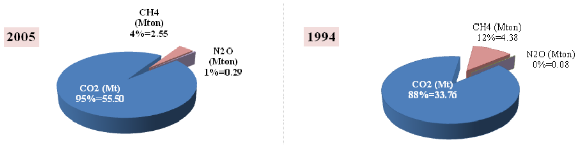
Fig. 2.7. GHG Emissions from the Energy Sector by Gas during the Years 1994 and 2005
