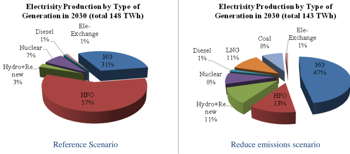
Fig. 4.3 Electricity produced in 2030 by Type of fuel: Comparison of Two Scenarios. (NG=natural gas, HFO=heavy fuel oil)
