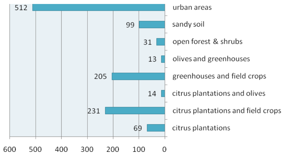
Fig. 3.24 Impact of RSL on Land Use/Cover (ha) 27
