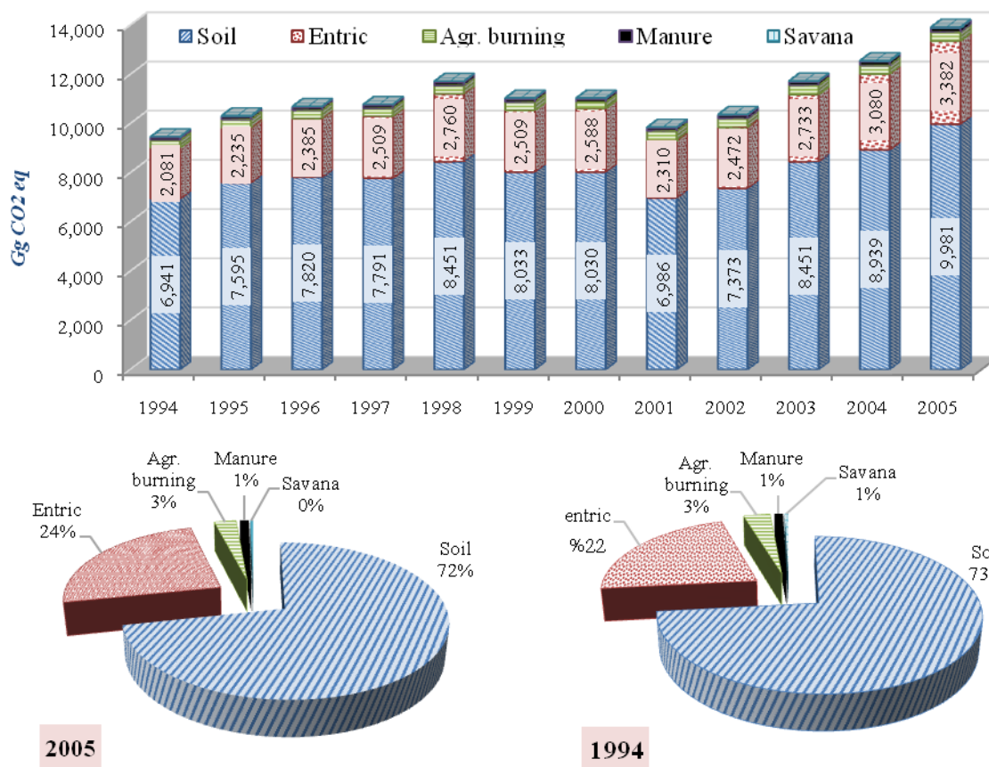
Fig. 2.17 GHG Emissions from Agriculture (by Sector)
