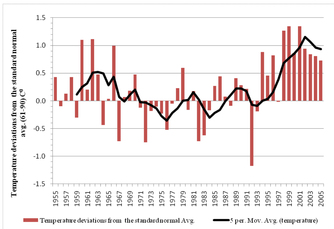
Fig. 1.6 Mean Annual Temperature Deviations from the Standard Average for Stations Representative of Syria's Climate Zones during the Years 1955–2005
