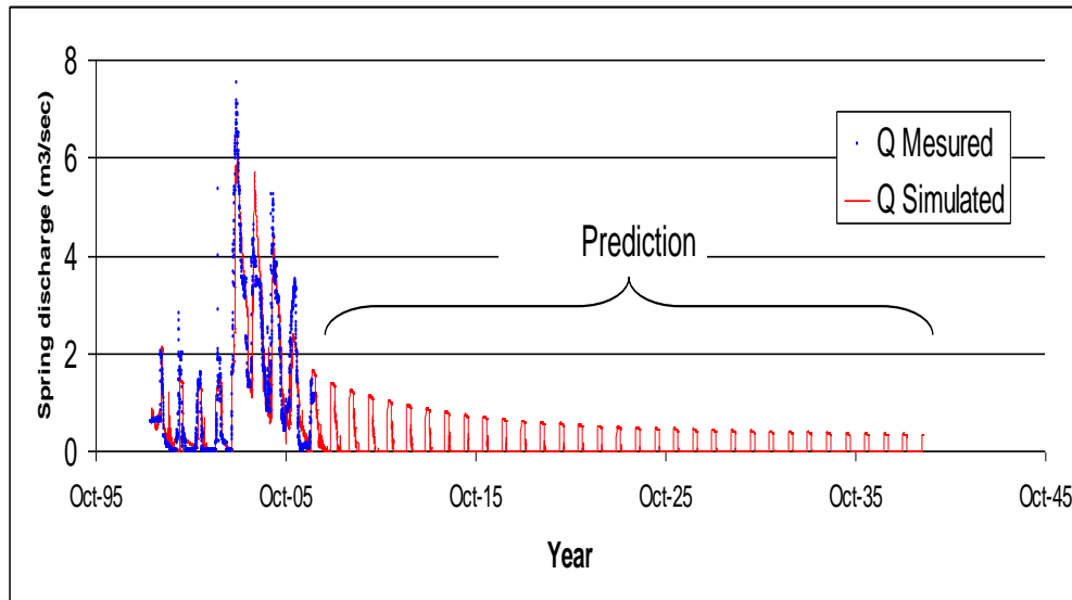
Fig. 3.19 Simulated Daily Spring Discharge after 2007
