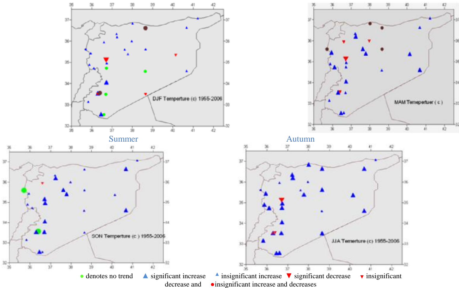
Fig. 3.3 Mann-Kendall Trend Analysis applied to Seasonal Average Annual Temperature Series between 1955 and 2006
