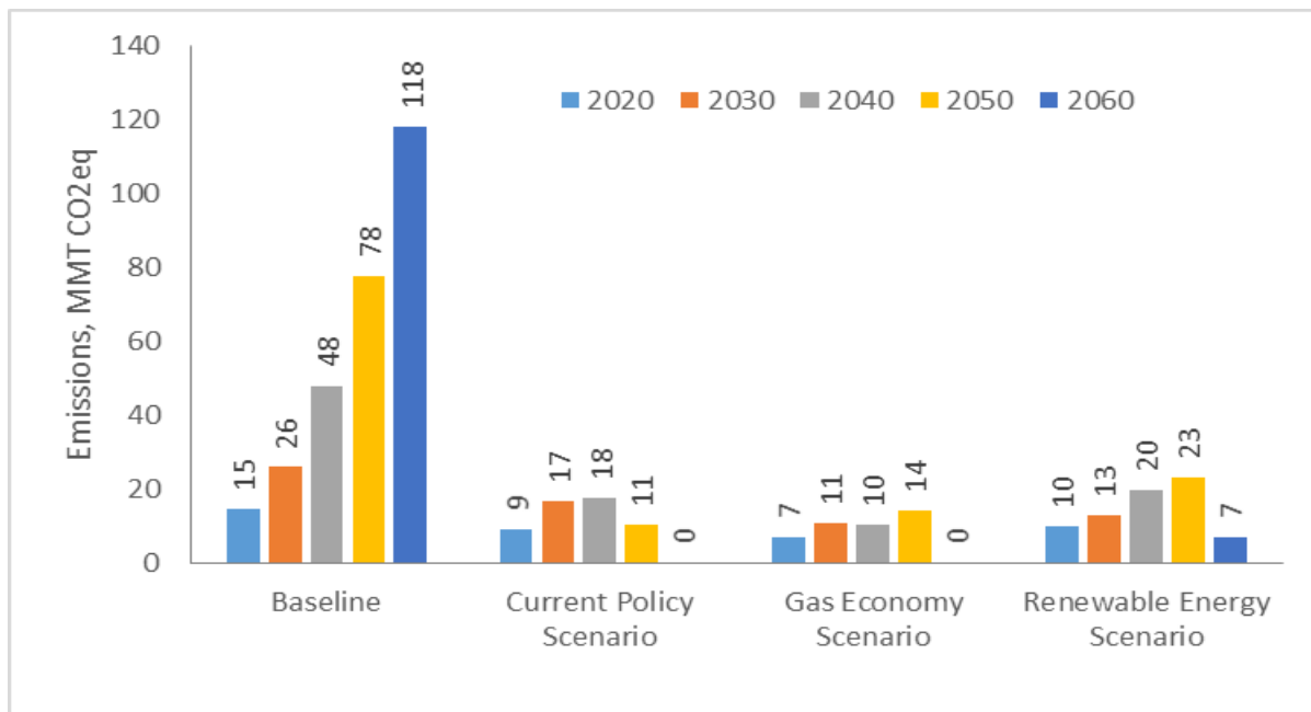
Figure 4.3: GHG emissions of power generation
