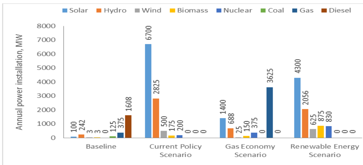
Figure 4.8: Annual power installation by scenarios
