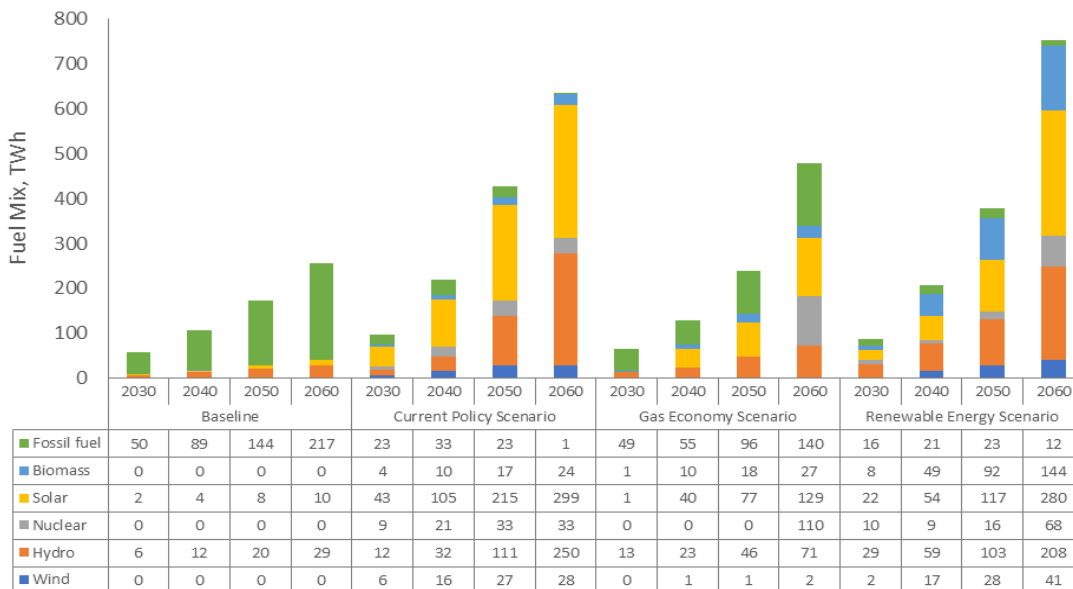
Figure 4.6: Electricity generation mix
