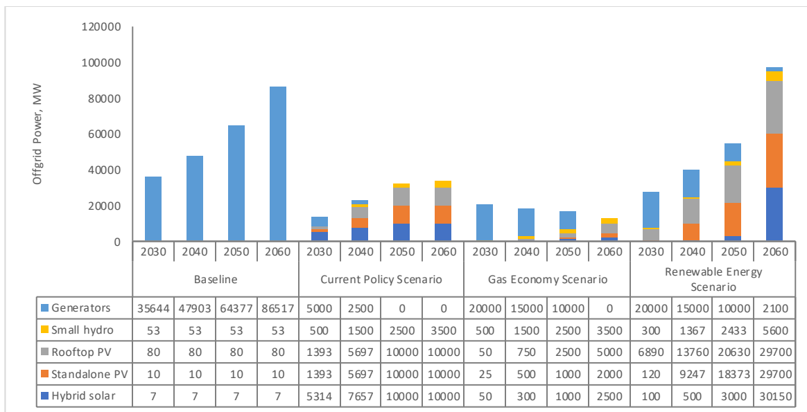
Figure 4.7b: Off-grid power generation capacity by technology
