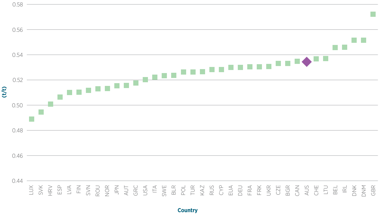
Figure 4.7 Cement production implied emission factors for Annex I countries (2023 submission) and Australia (2025 submission), tonnes of CO 2 per tonne of cement produced
