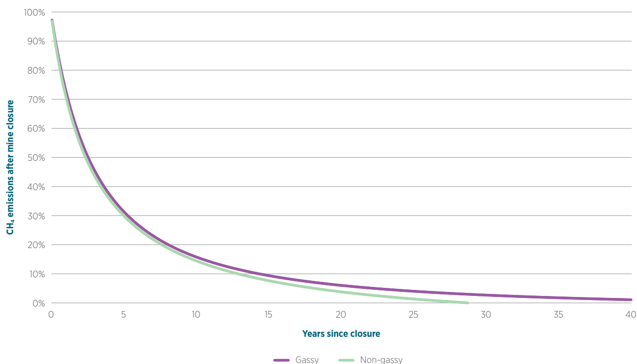
Figure 3.26 CH 4 decay curves for gassy and non-gassy Australian decommissioned coal mines
