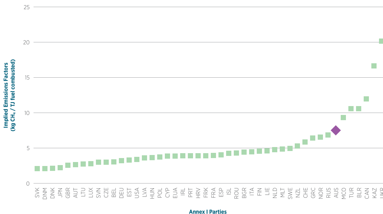
Figure 3.19 Implied emission factors from liquid fuel combustion for Annex I countries (2023 submission) and Australia (2025 submission), kg CH 4 per TJ combusted
