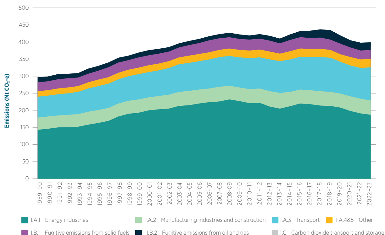
Figure 3.2 Energy emissions by subsector, 1989–90 to 2022–23
