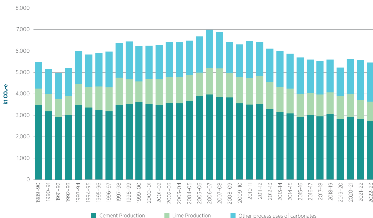
Figure 4.5 Emissions from the mineral industry, Australia, 1989-90 to 2022-23, kt CO 2 -e
