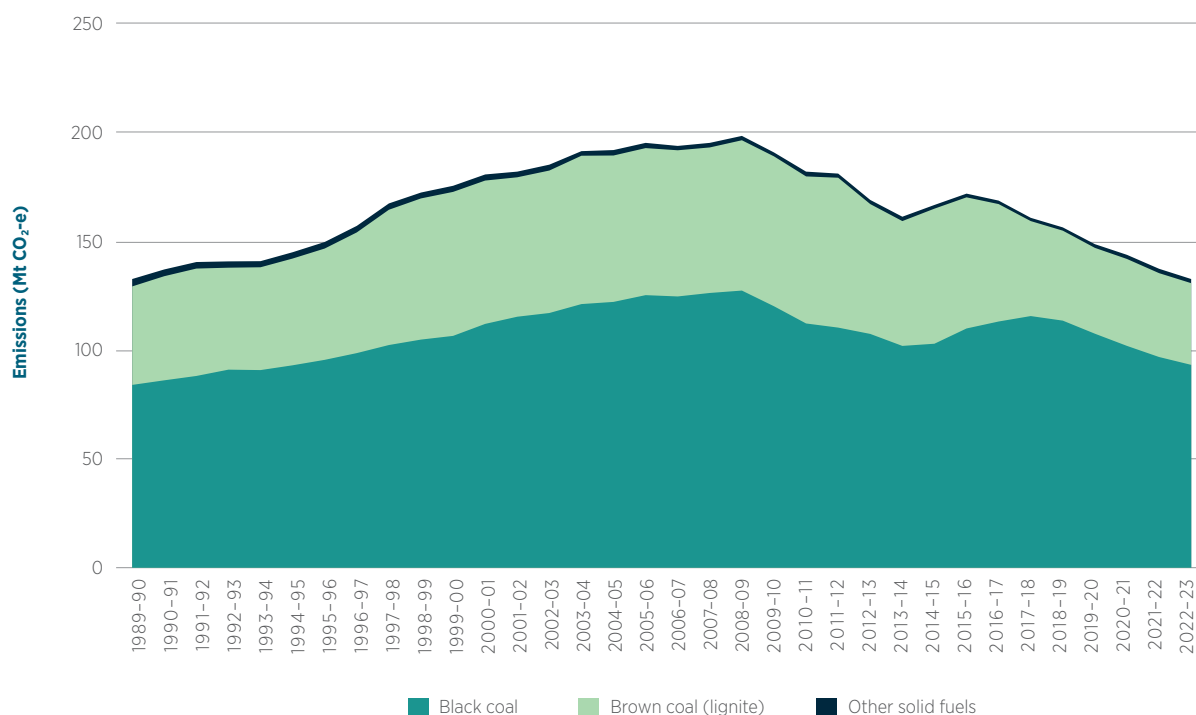
Figure 3.5 Emissions from solid fuel combustion, 1989–90 to 2022–23
