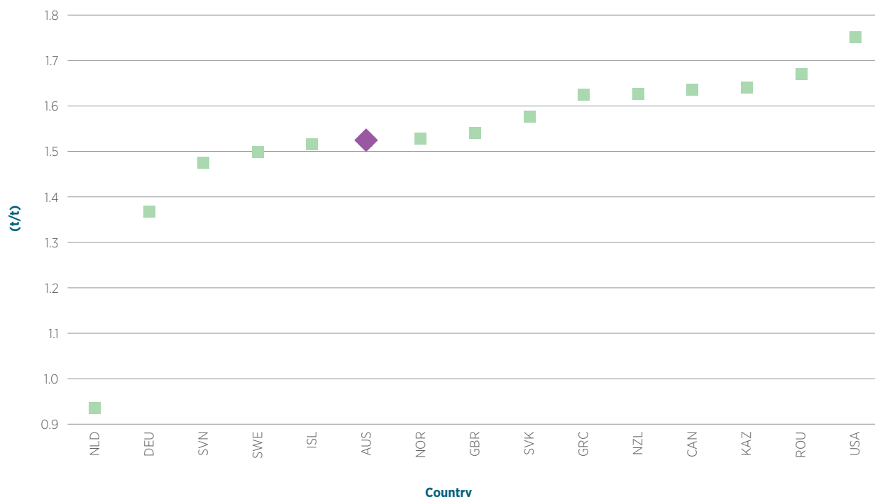
Figure 4.14 Aluminium production implied emission factors for Annex I countries (2023 submissions) and Australia (2025 submission), tonnes of CO 2 per tonne of aluminium produced
