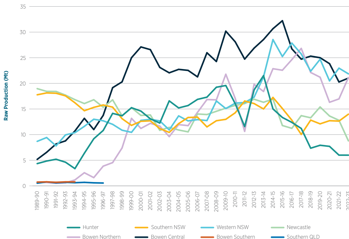
Figure 3.24 Underground black coal production by coal field since 1989–90
