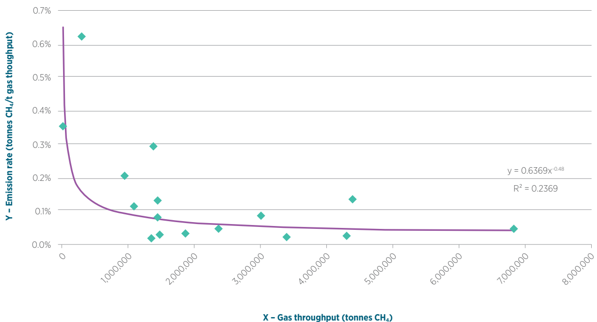
Figure 3.38 Gas processing plants with reported high emission rates are likely to have negligible gas throughputs
