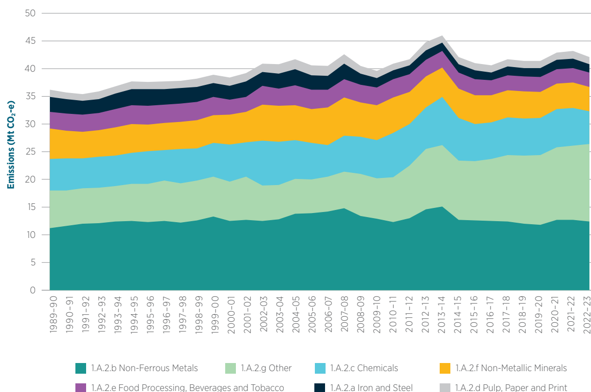
Figure 3.13 Emissions from the manufacturing and construction industries by subsector, 1989–90 to 2022–23
