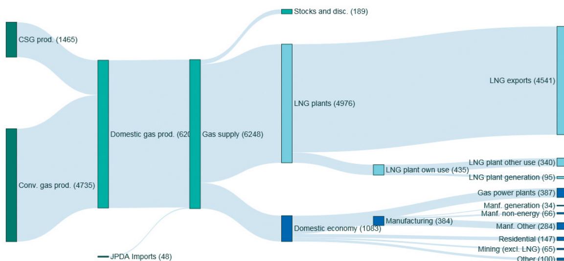
Figure 3.34 Australian natural gas energy flows, PJ, 2022–23
