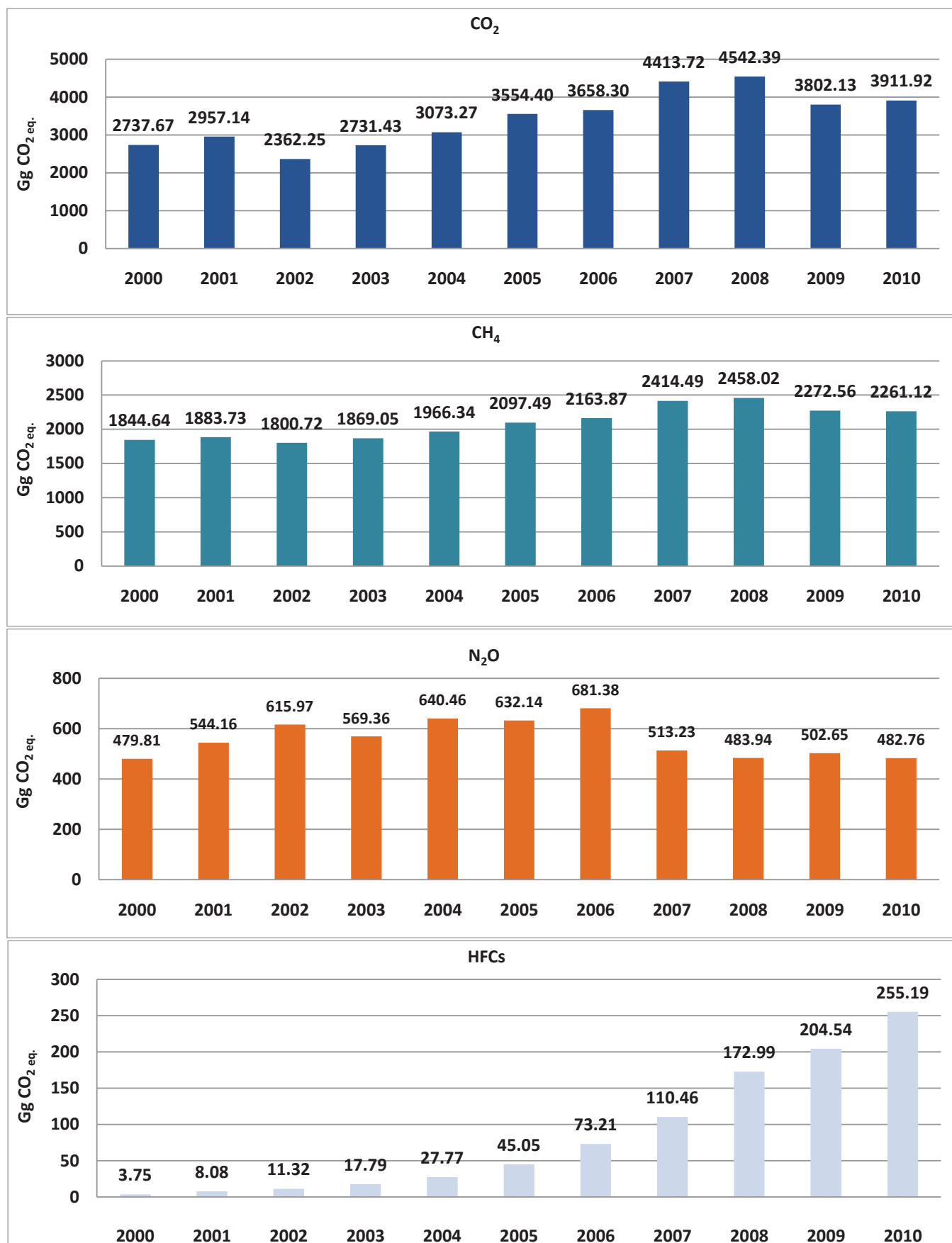
Figure 3.2 Emission Time Series by Gases, for 2000 - 2010 (Gg CO 2 eq.)
