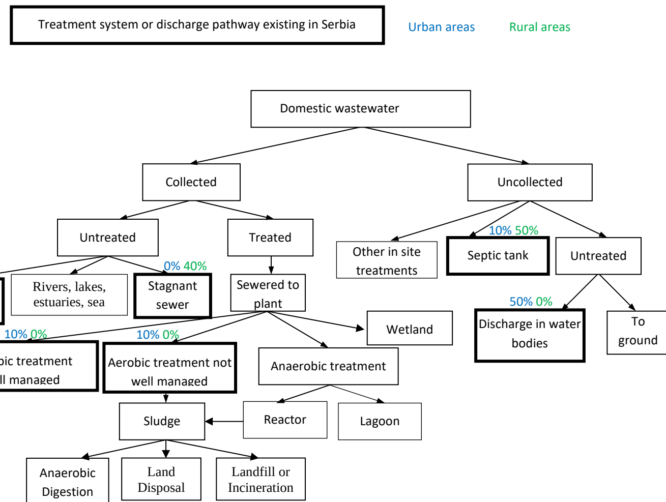
Figure 156: Serbian treatment systems and pathways for domestic wastewater
