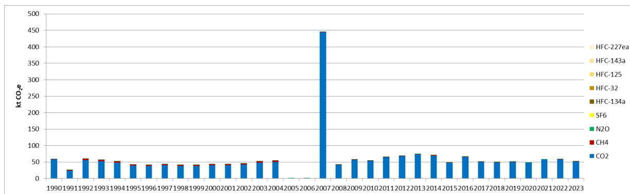
Figure 23 : GHG emissions for agriculture/forestry/fishing activities - stationary combustion (CRT 1A4ci), for the period 1990-2023 (in kt CO 2 e)
