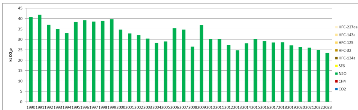
Figure 103 : N 2 O emissions for manure management of other livestock (CRT 3B24) (kt CO 2 e)
