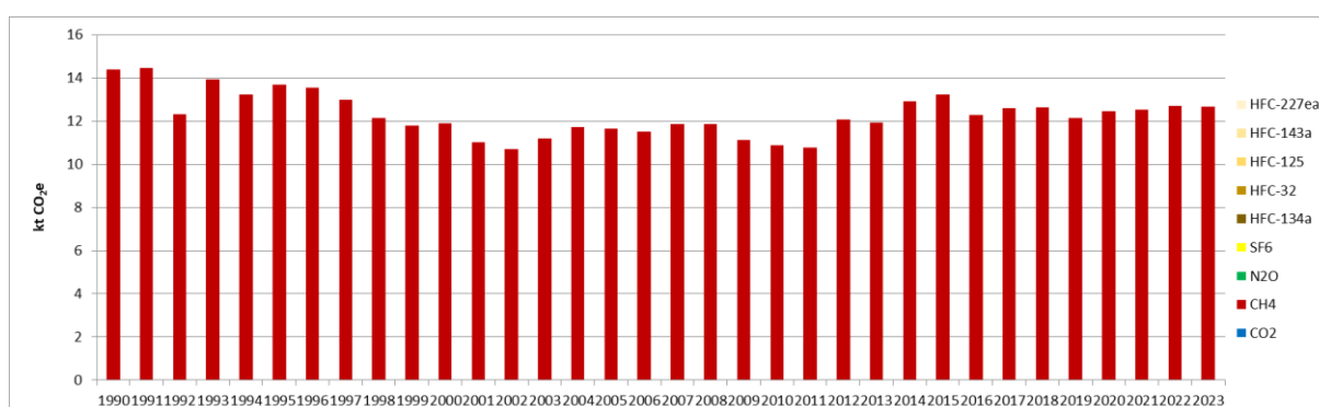
Figure 95 : CH 4 emissions for manure management of sheep (CRT 3B12) (kt CO 2 e)
