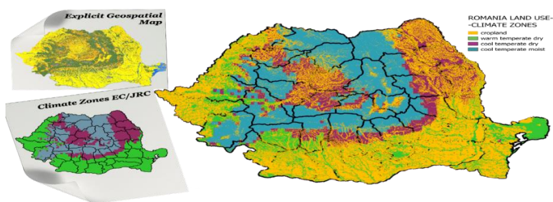
Figure 6.18 4.B land use category. EGM – explicit geospatial map
