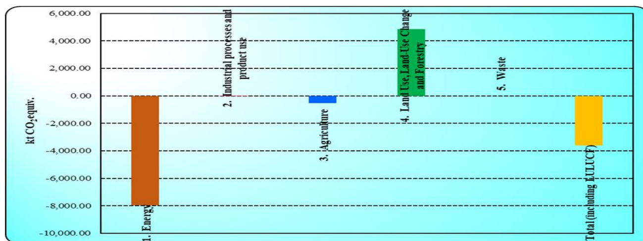
Figure 10.9 Changes of 2005 emissions/removals, in respect to the 2026 figures
