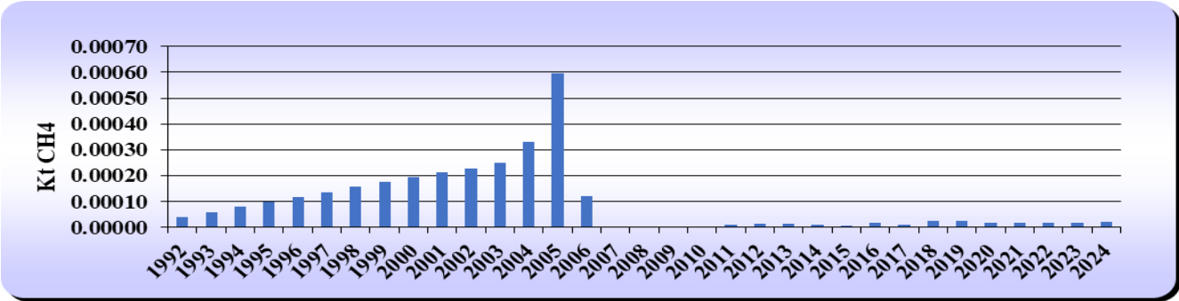
Figure 7.20 CH 4 emissions trend from biogenic waste incineration, for 2001–2024 period
