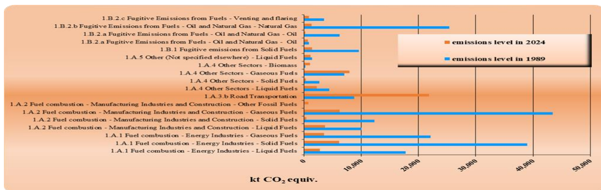
Figure 3.3 Key categories, both by level and trend criteria, overview – Energy Sector, 2024
