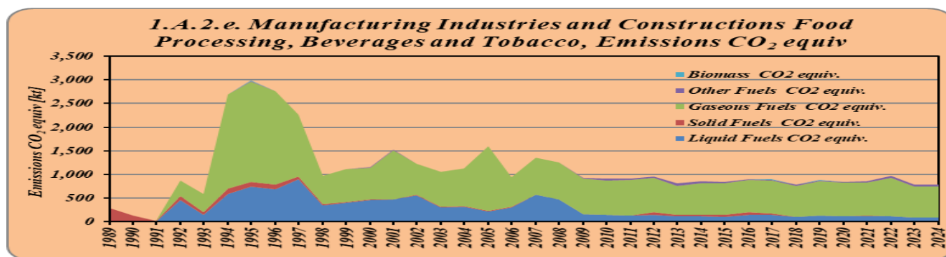
Figure 3.30 GHG emissions 1.A.2.e – Food Processing, Beverages and Tobacco, by fuels
