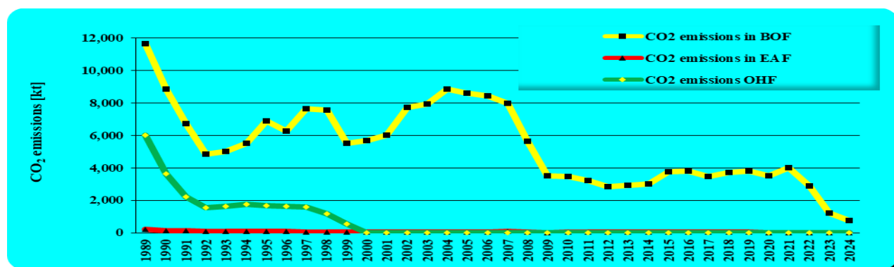
Figure 4.15 The trend of CO 2 emissions from Iron and Steel Production in the 1989–2024 period
