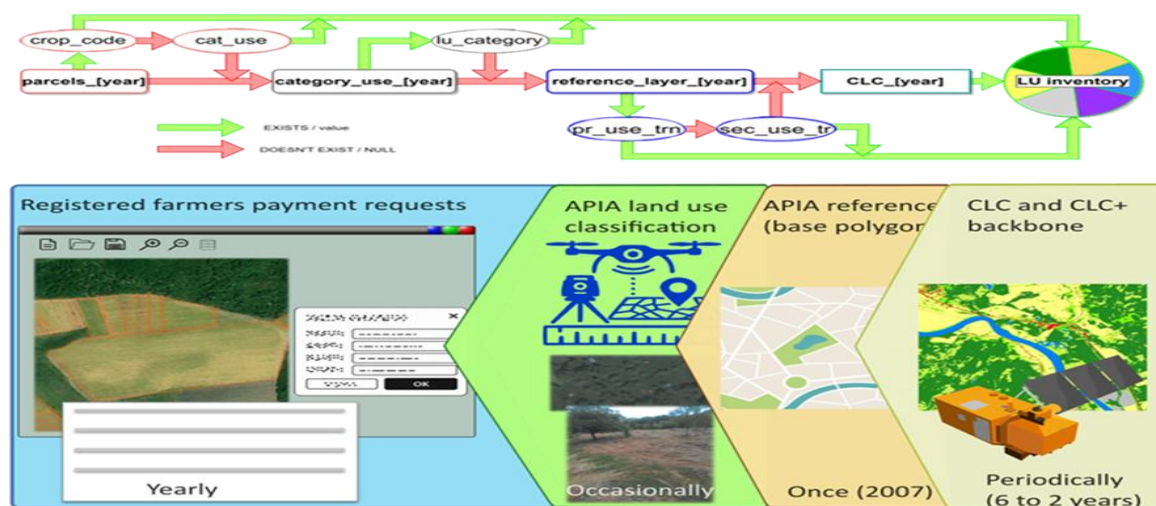
Figure 6.20 Graphical and alphanumeric data filtering algorithm that are used from the two combined sources, including illustrative examples of the land use identification process
