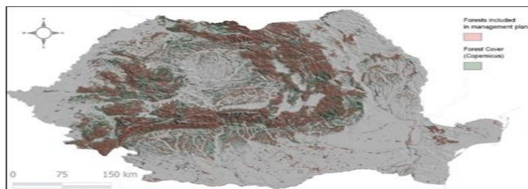
Figure 6.10 Area of forest land category stratified between included or not into forest management plans
