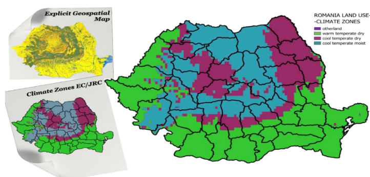
Figure 6.34 4.F land use category. EGM - explicit geospatial map
