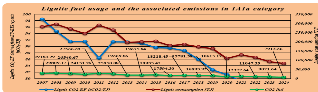
Figure 3.21 CO 2 emissions variation associated with the lignite usage in the 1.A.1.a – Public Electricity and Heat Production
