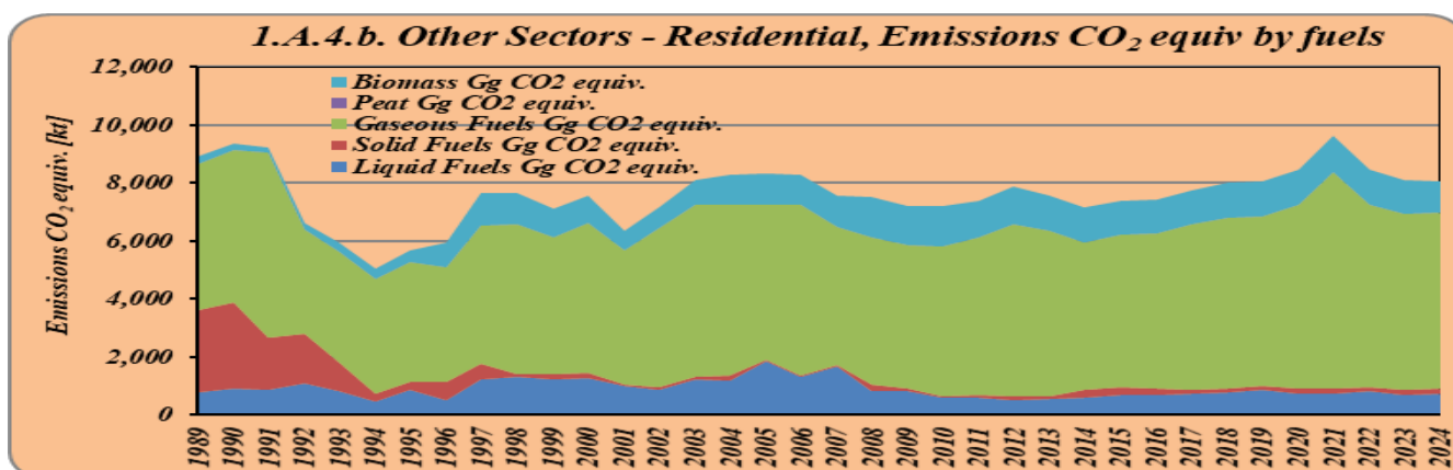
Figure 3.50 GHG emissions from 1.A.4.b – Residential, by fuels
