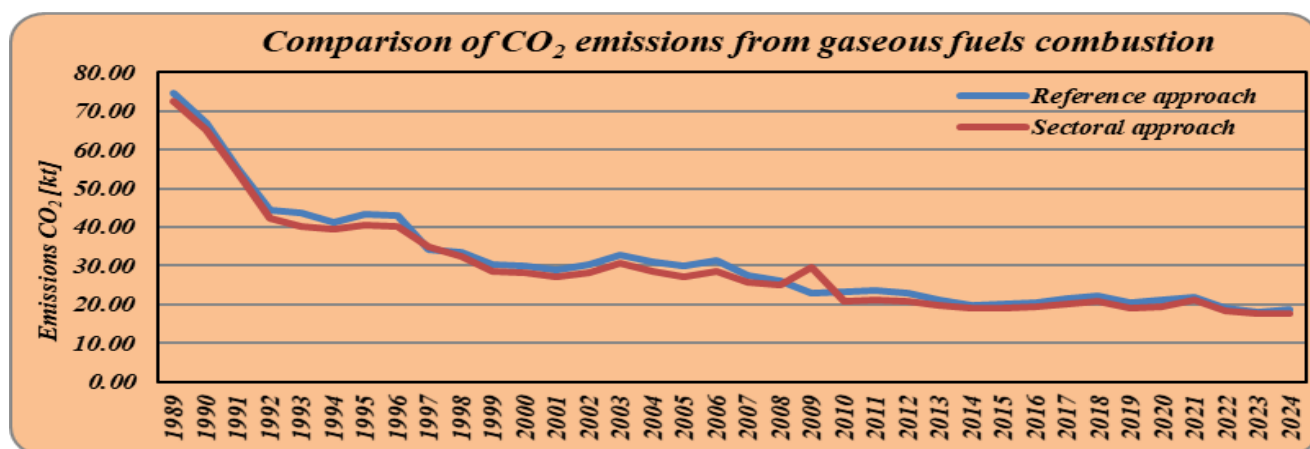
Figure 3.7 Comparison of the sectorial approach with the reference approach – gaseous fuels
