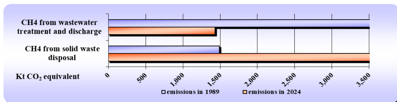
Figure 7.3 Key categories in in Waste Sector both by level and trend criteria, in 2024
