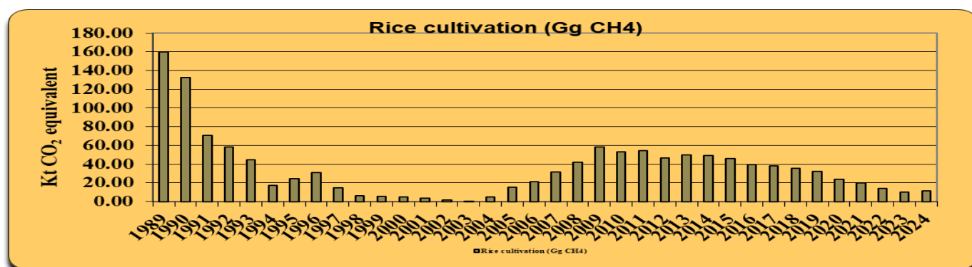
Figure 5.6 Methane emission trend due to the Rice Cultivation
