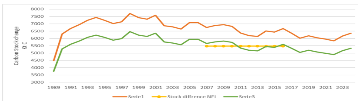
Figure 6.14 Comparison of Initial and Corrected Carbon Stock Change Estimates Using the Overlap Method.
