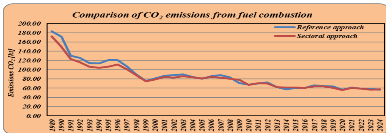
Figure 3.4 Comparison of the sectorial approach with the reference approach
