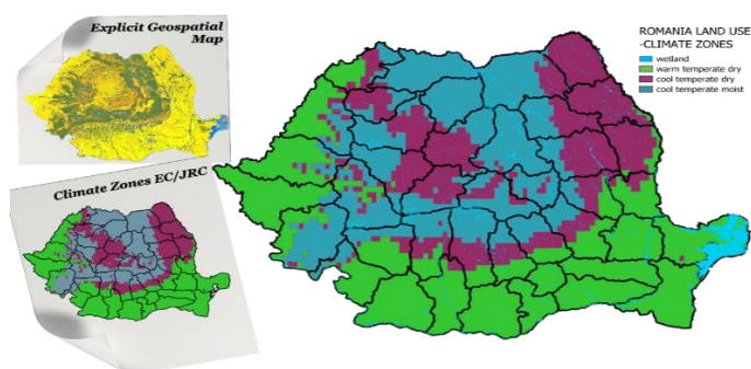
Figure 6.27 4.D land use category. EGM - explicit geospatial map
