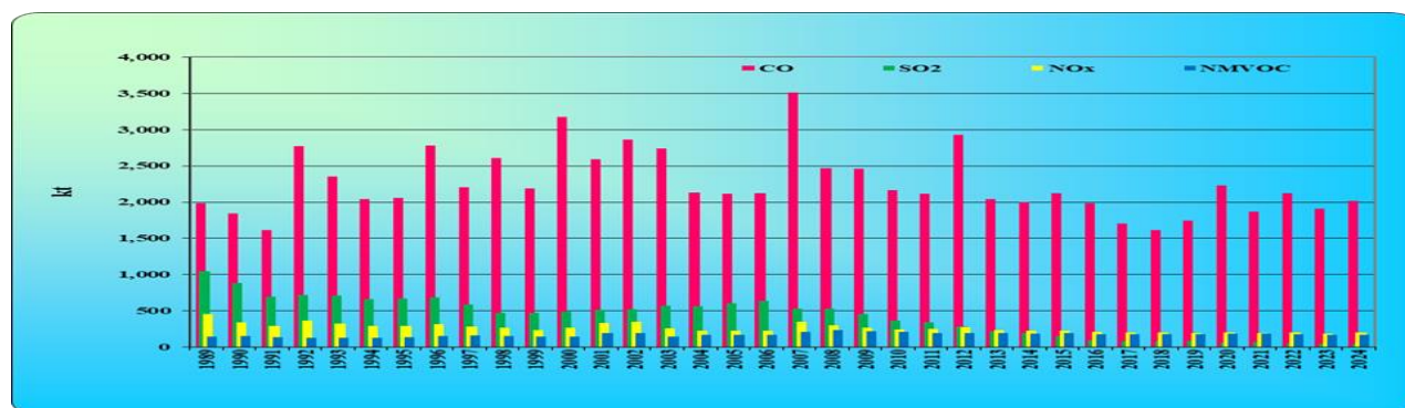
Figure 2.2 Indirect GHG emissions trends [kt]
