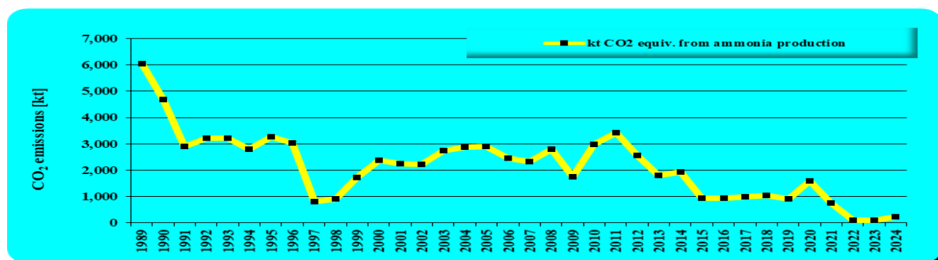
Figure 4.8 The trend of CO 2 emissions from ammonia production in the 1989–2024 period
