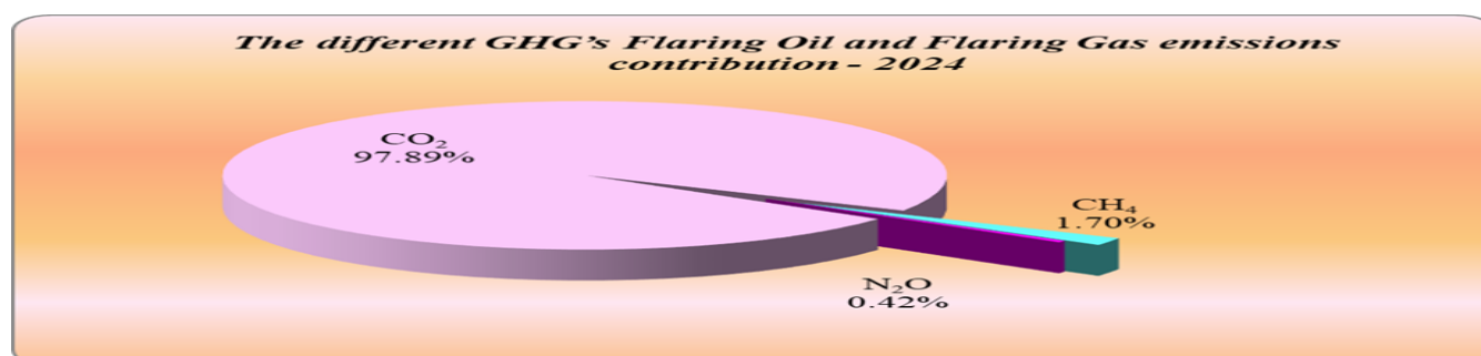
Figure 3.63 The different GHG's Flaring Oil and Flaring Gas emissions contribution
