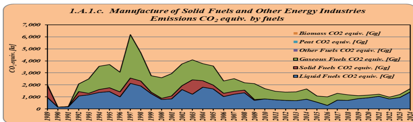
Figure 3.23 GHG emissions from 1.A.1.c Manufacture of Solid Fuels and Other Energy Industries
