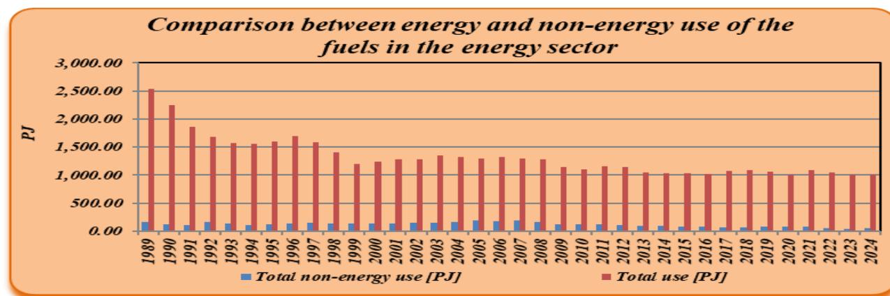
Figure 3.14 The most important non-energy consumption of the fuels
