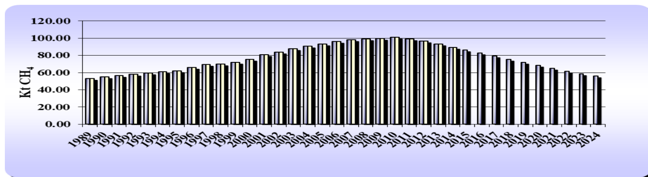
Figure 7.6 CH 4 emissions trend from waste disposed to unmanaged sites for 1989–2024 period
