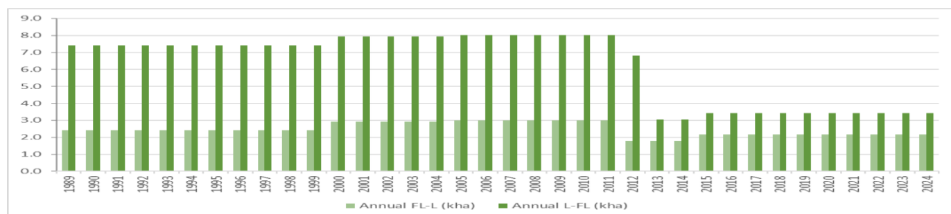
Figure 6.9 The area of forest-related land conversions
