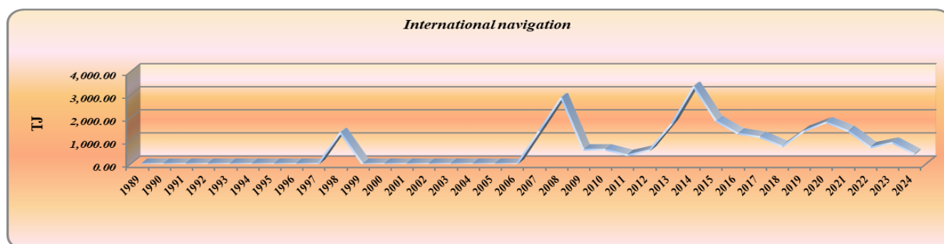
Figure 3.12 Total fuel consumption from International Navigation category for 1989–2024 period
