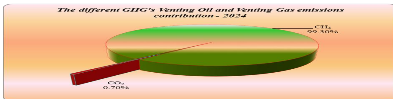
Figure 3.62 The different GHG's Venting oil and Venting Gas emissions contribution
