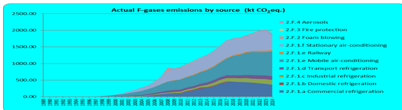
Figure 4.20 Actual F– gases emissions by source for 1989–2024 period
