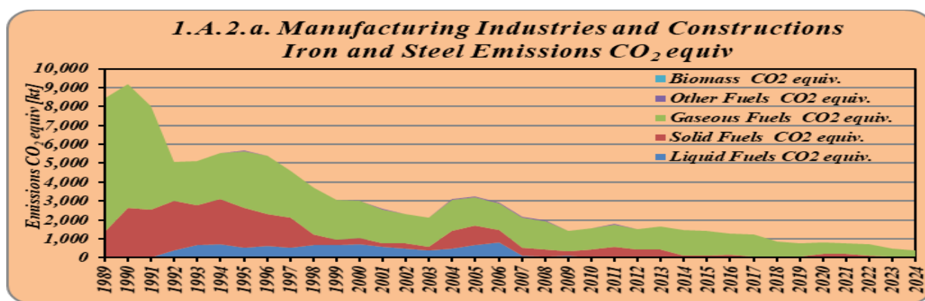
Figure 3.26 GHG emissions from 1.A.2.a – Iron and Steel, by fuels
