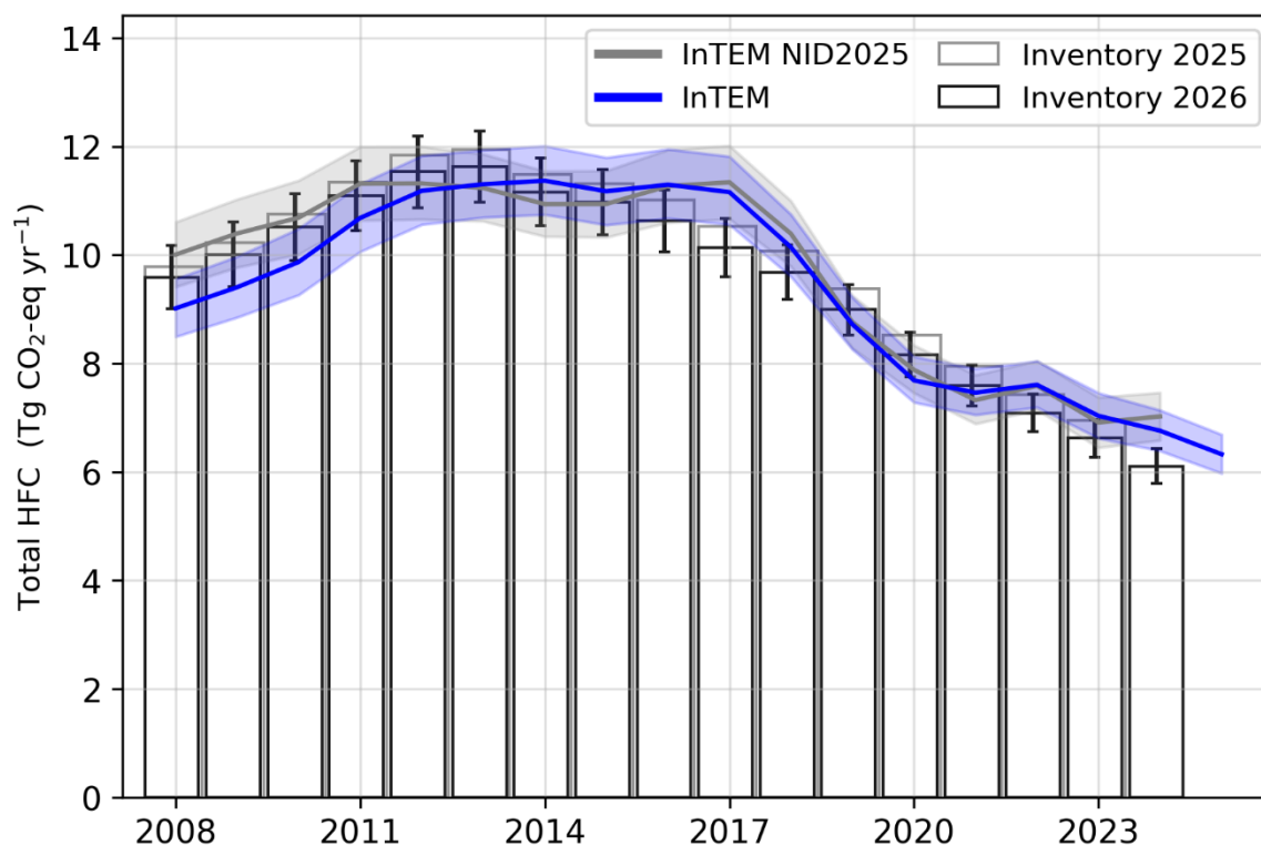
Figure A 6.4.1 Sum of UK HFC emission estimates (HFC-125, HFC-134a, HFC-143a, HFC-152a, HFC-23, HFC-32, HFC-227ea, HFC-245fa, HFC-365mfc HFC-43-10mee and HFC-236fa) in Tg CO 2 e yr -1 from the GHGI (black bar 2026, grey bar 2025) and InTEM, 1-year inversion, with a 3-year moving average applied, (blue line, grey line 2025). Note the very small contribution from HFC-43-10mee (< 0.2 TgCO 2 e yr -1 ) is only included from 2010 because of the lack of available observations. The uncertainty bars represent \pm 1\sigma .
