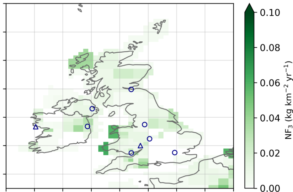
Figure A 6.7.2 Four-year average \text{NF}_3 InTEM emission estimates ( \text{kg km}^{-2} \text{yr}^{-1} ) 2022-2025. The observation stations are shown as blue triangles. Major cities are shown as blue circles.
