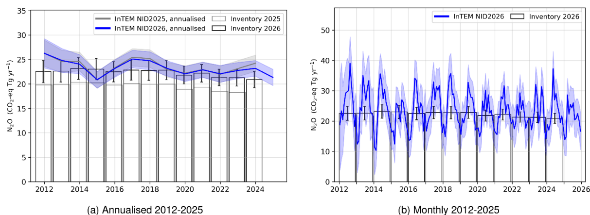
Figure A 6.3.2 Verification of the UK emission inventory estimates for N 2 O in Tg CO 2 e yr -1 from 2012. GHGI estimates are shown in black ( \pm 1\sigma ). InTEM 1-month estimates are shown in blue ( \pm 1\sigma ). (a) Annualised InTEM 1-month estimates compared to the InTEM estimates from last year (grey line) and GHGI estimates (black bar 2026, grey bar 2025) and (b) Monthly estimates.
