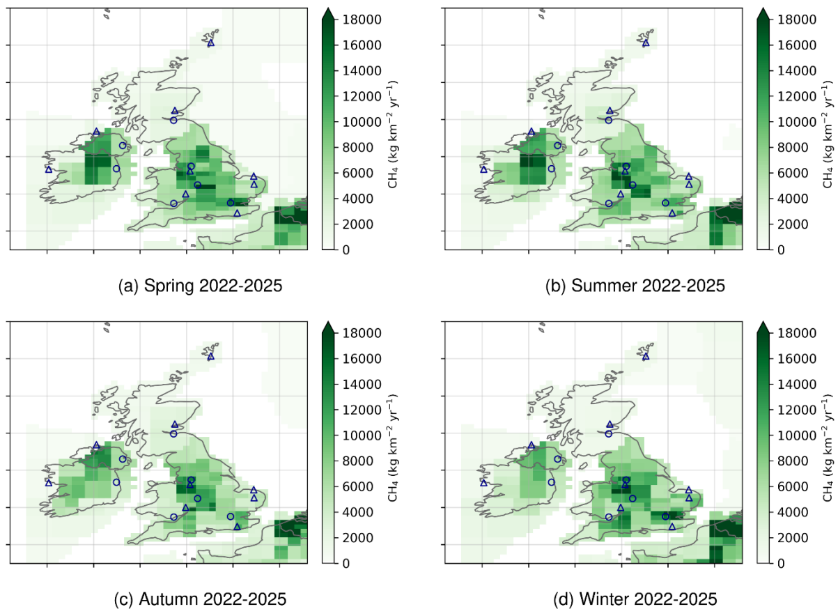
Figure A 6.2.4 Four-year average CH 4 InTEM emission estimates (kg km -2 yr -1 ) 2022-2025 by season: (a) Spring (b) Summer (c) Autumn and (d) Winter. The observation stations are shown as blue triangles. Major cities are shown as blue circles.
