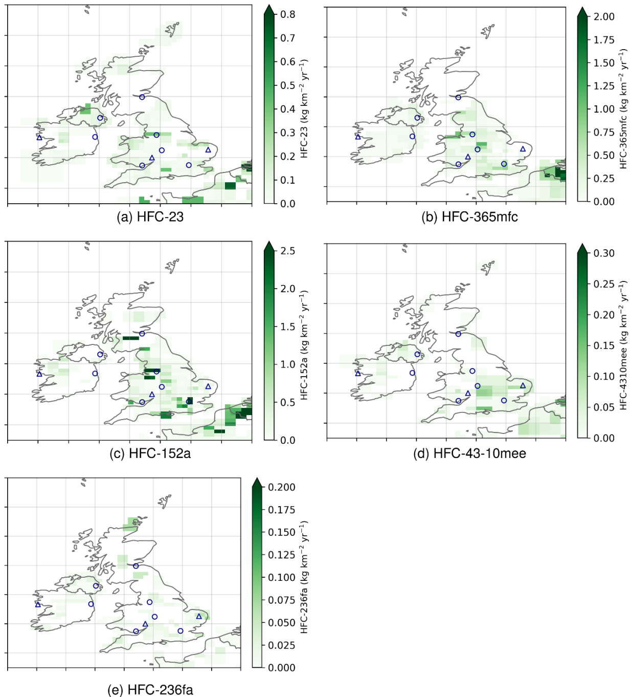
Figure A 6.4.7 Four-year average HFC InTEM emission estimates ( \text{kg km}^{-2} \text{yr}^{-1} ) 2022–2025. The observation stations are shown as blue triangles. Major cities are shown as blue circles.
