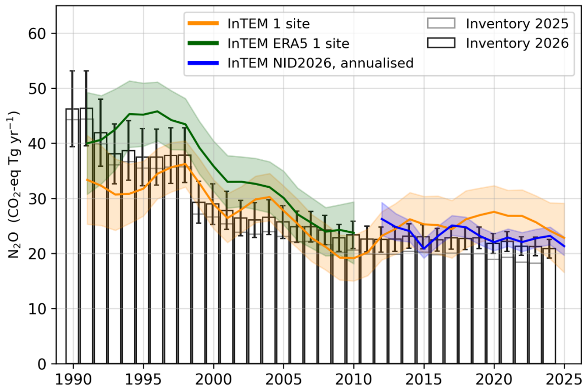
Figure A 6.3.1 Verification of the UK emission inventory estimates for N 2 O in Tg CO 2 e yr -1 from 1990. GHGI 2026 estimates are shown in black ( \pm 1\sigma ), the GHGI 2025 estimates are shown in grey. InTEM 1-site 3-year estimates, using the standard meteorology and the new ERA5 meteorology, are shown in orange and green respectively ( \pm 1\sigma ). InTEM full network, 1-month annualised, estimates are shown in blue ( \pm 1\sigma ).
