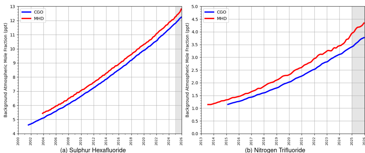
Figure A 6.6.1 (a) shows the hemispheric background atmospheric concentrations of sulphur hexafluoride (SF 6 ) from 2004 onwards. The background trend is monotonic and positive and in 2025 the Northern Hemispheric background concentration increased by 0.4 ppt.
