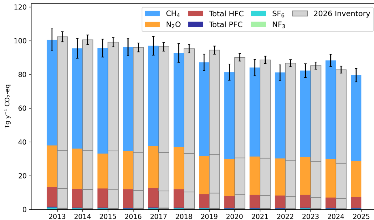
Figure A 6.1.1 Total emissions of GHGs (excluding CO 2 ) from 2013-2025. InTEM results are shown as coloured bars and the GHGI are shown as grey bars.
