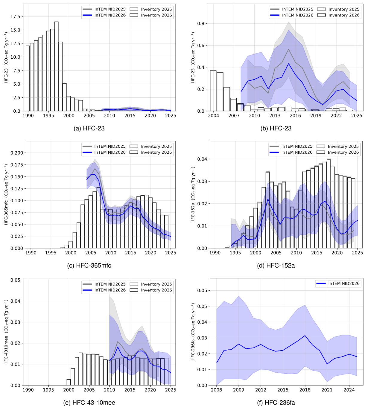
Figure A 6.4.5 Comparison of the UK emission inventory estimates for individual HFCs in Tg CO 2 e yr -1 from 1990. GHGI estimates are shown as black bars (GHGI 2025 as grey bars) (individual uncertainties by gas are not available). InTEM 1-year estimates, with a 3-year moving average applied, are shown as a blue line ( \pm 1\sigma ), (InTEM NID2025 result as a grey line).
