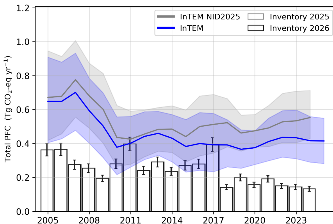
Figure A 6.5.1 Sum of UK PFC emission estimates (PFC-14, PFC-116, PFC-218, PFC-318) in Tg CO 2 e yr -1 from the GHGI (black bar 2026, grey bar 2025) and InTEM, 1-year inversion, with a 3-year moving average applied (blue line, grey line 2025). The uncertainty bounds represent 1- \sigma . Note the small contribution from PFC-318 (< 0.1 Tg CO 2 e yr -1 ) is only included from 2010 because of the lack of available observations.
