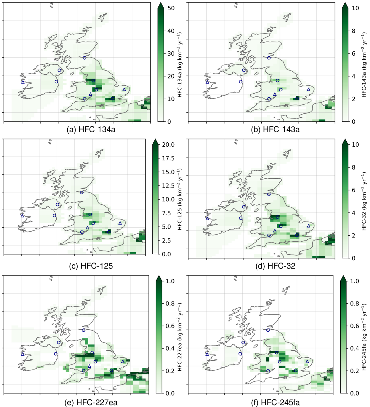
Figure A 6.4.6 Four-year average HFC InTEM emission estimates ( \text{kg km}^{-2} \text{yr}^{-1} ) 2022-2025. The observation stations are shown as blue triangles. Major cities are shown as blue circles.
