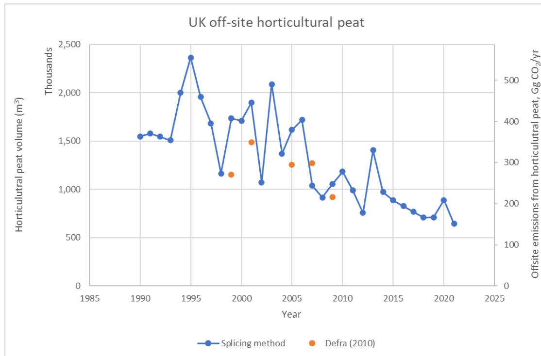
Figure A 5.1.24: Comparison of peat extraction volume for horticultural use and estimated off-site emissions in the UK using 1990-2021 GHG inventory data and the Northern Ireland spliced data, and UK-level peat volume data for 1999, 2001, 2005, 2007 and 2009 compiled in Defra report SP08020 (Defra 2010).
