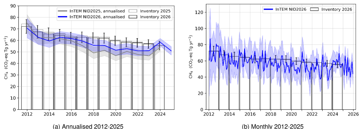
Figure A 6.2.3 Verification of the UK emission inventory estimates for CH 4 in Tg CO 2 e yr -1 from 2012. GHGI estimates are shown in black ( \pm 1\sigma ). InTEM 1-month estimates are shown in blue ( \pm 1\sigma ). (a) Annualised estimates compared to last year's InTEM and GHGI estimates and (b) Monthly estimates.
