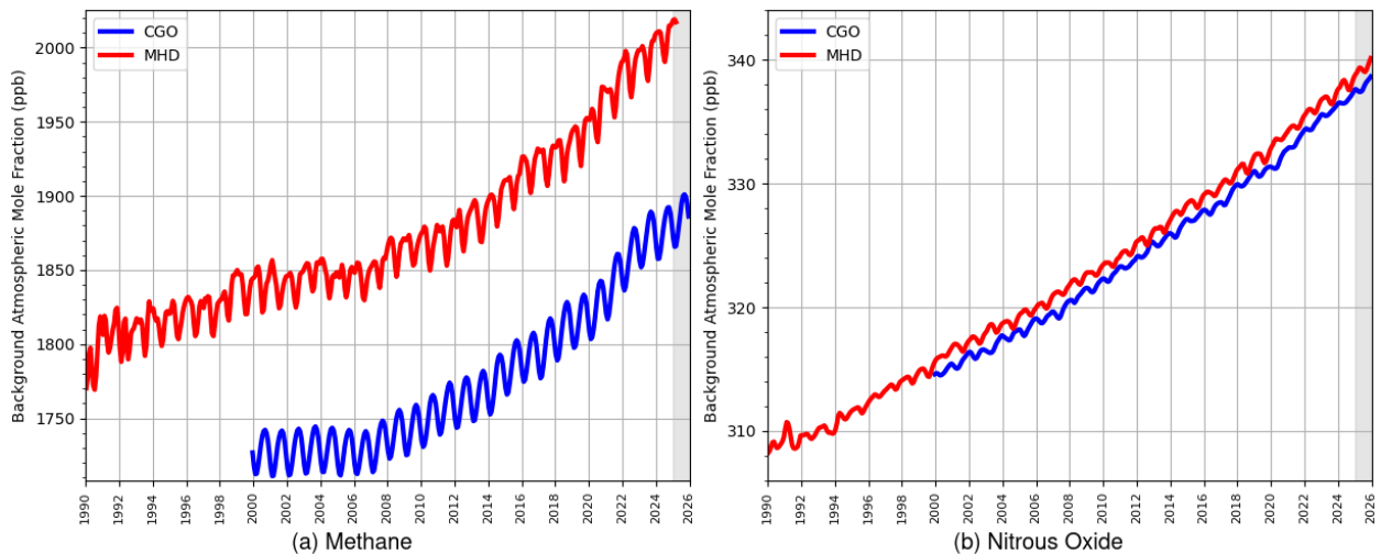
Figure A 6.2.1 Background Northern Hemisphere monthly concentrations of (a) CH 4 and (b) N 2 O estimated from MHD, Ireland, observations are shown in red, and background Southern Hemisphere monthly concentrations from CGO, Tasmania, are shown in blue. Grey shading represents unratiified data.
