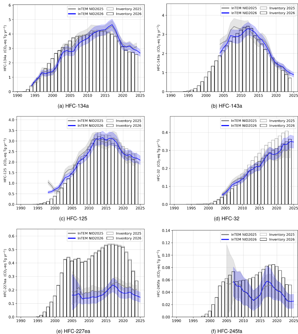
Figure A 6.4.4 Comparison of the UK emission inventory estimates for individual HFCs in Tg CO 2 e yr -1 from 1990. GHGI estimates are shown as black bars (GHGI 2025 as grey bars) (individual uncertainties by gas are not available). InTEM 1-year estimates, with a 3-year moving average applied, are shown as a blue line ( \pm 1\sigma ), (InTEM NID2025 result as a grey line).
