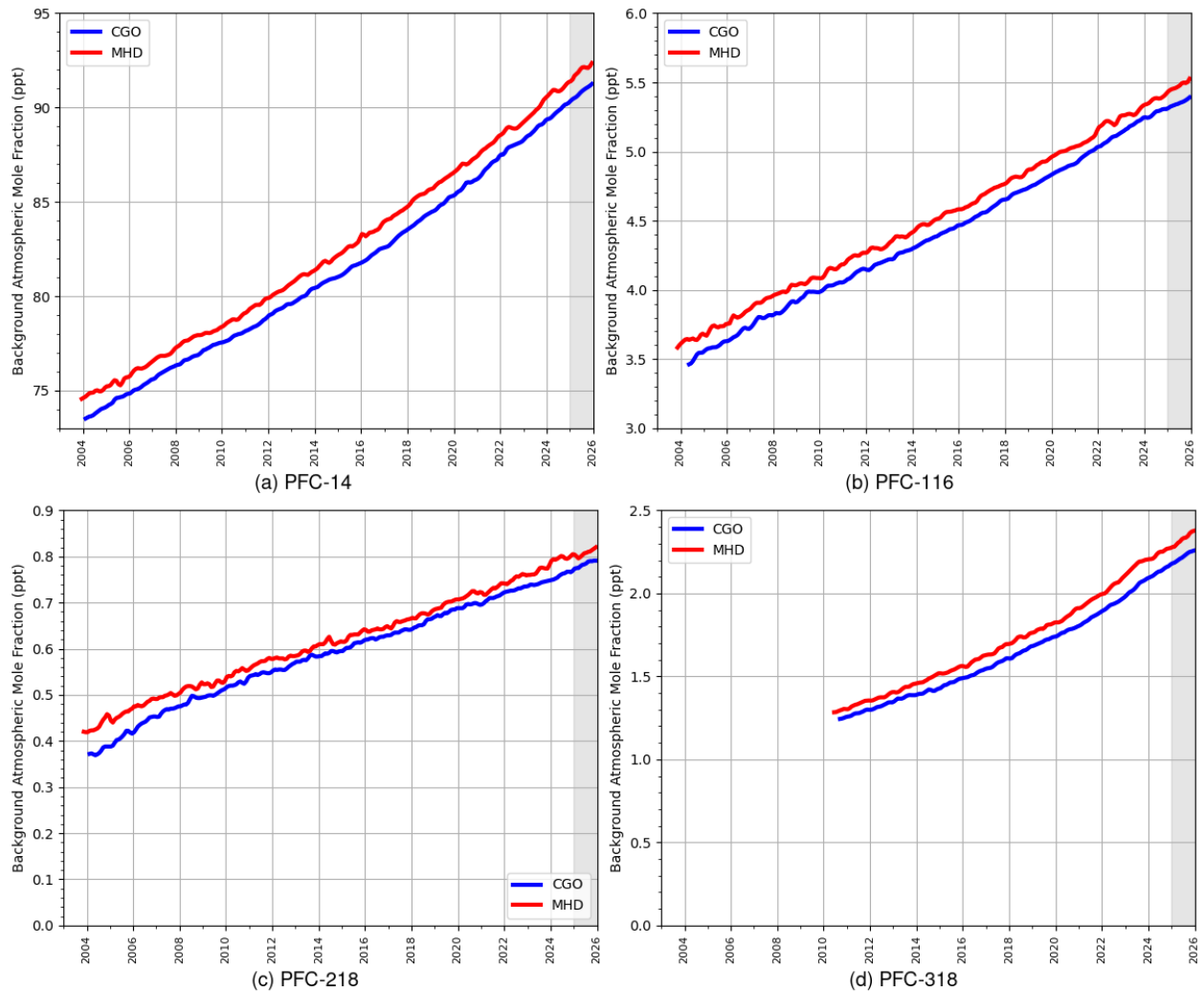
Figure A 6.5.2 Background Northern Hemisphere monthly concentrations of four PFCs estimated from MHD, Ireland observations are shown in red, and background Southern Hemisphere monthly concentrations from CGO, Tasmania are shown in blue. Grey shading represents unratified data.
