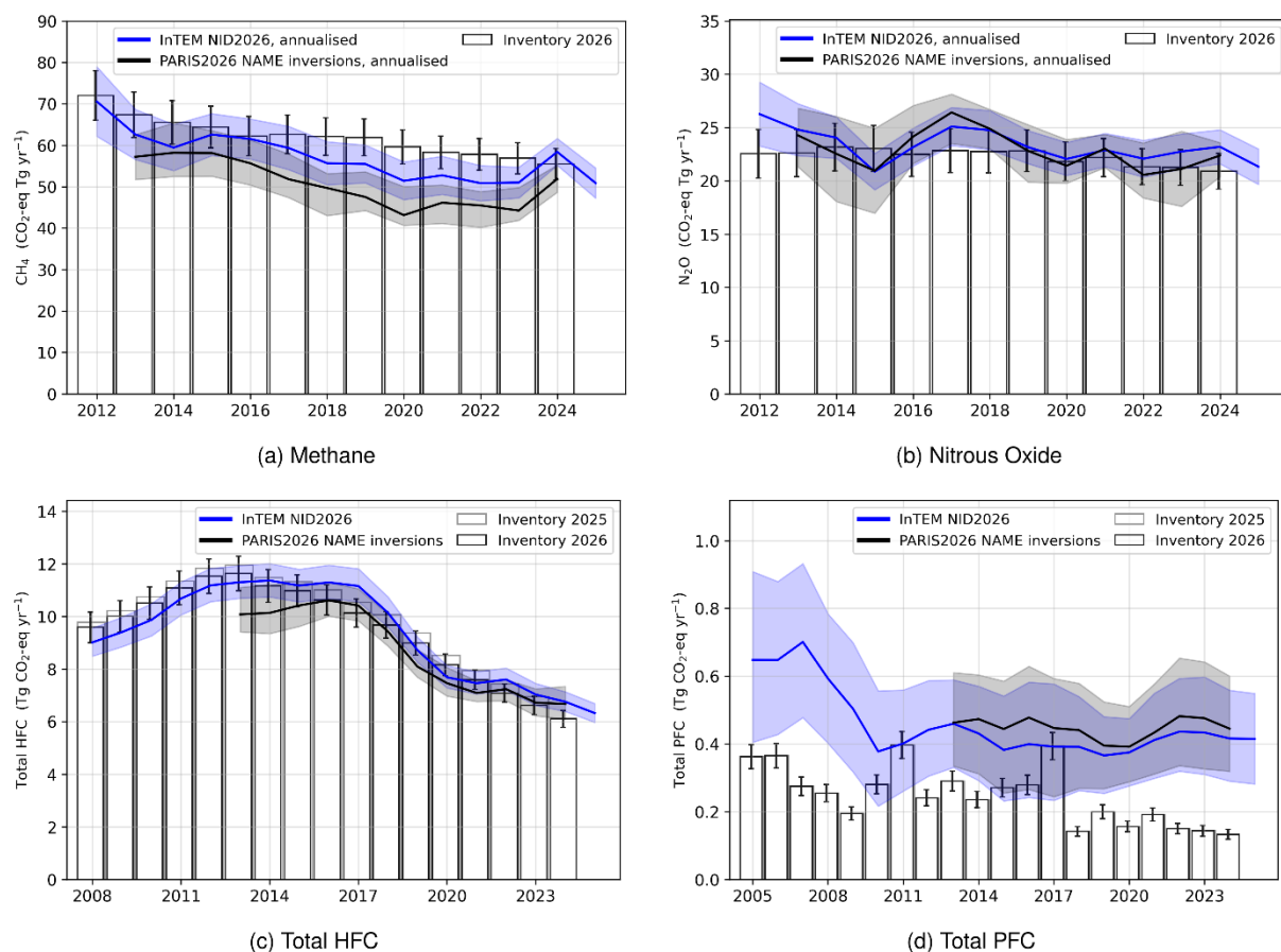
Figure A 6.9.1 InTEM model results (blue line), combined results from the PARIS project (black line) and GHGI (black bars) for (a) methane, (b) nitrous oxide, (c) total HFC and (d) total PFC. The HFC and PFC plots also show the GHGI 2025 values (grey bars).
