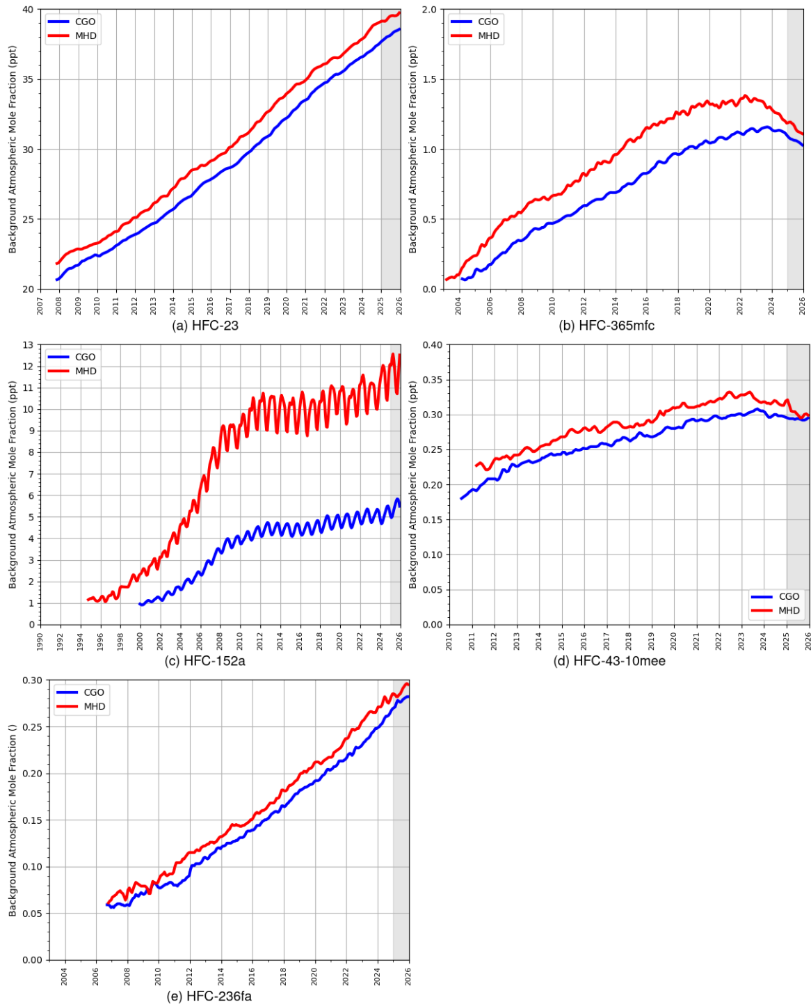
Figure A 6.4.3 Background Northern Hemisphere monthly concentrations of five HFCs estimated from MHD, Ireland observations are shown in red, and background Southern Hemisphere monthly concentrations from CGO, Tasmania are shown in blue. Grey shading represents unrated data.
