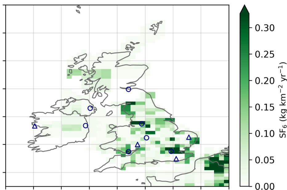
Figure A 6.6.4 Four-year average SF 6 InTEM emission estimates (kg km -2 yr -1 ) 2022-2025. The observation stations are shown as blue triangles. Major cities are shown as blue circles.
