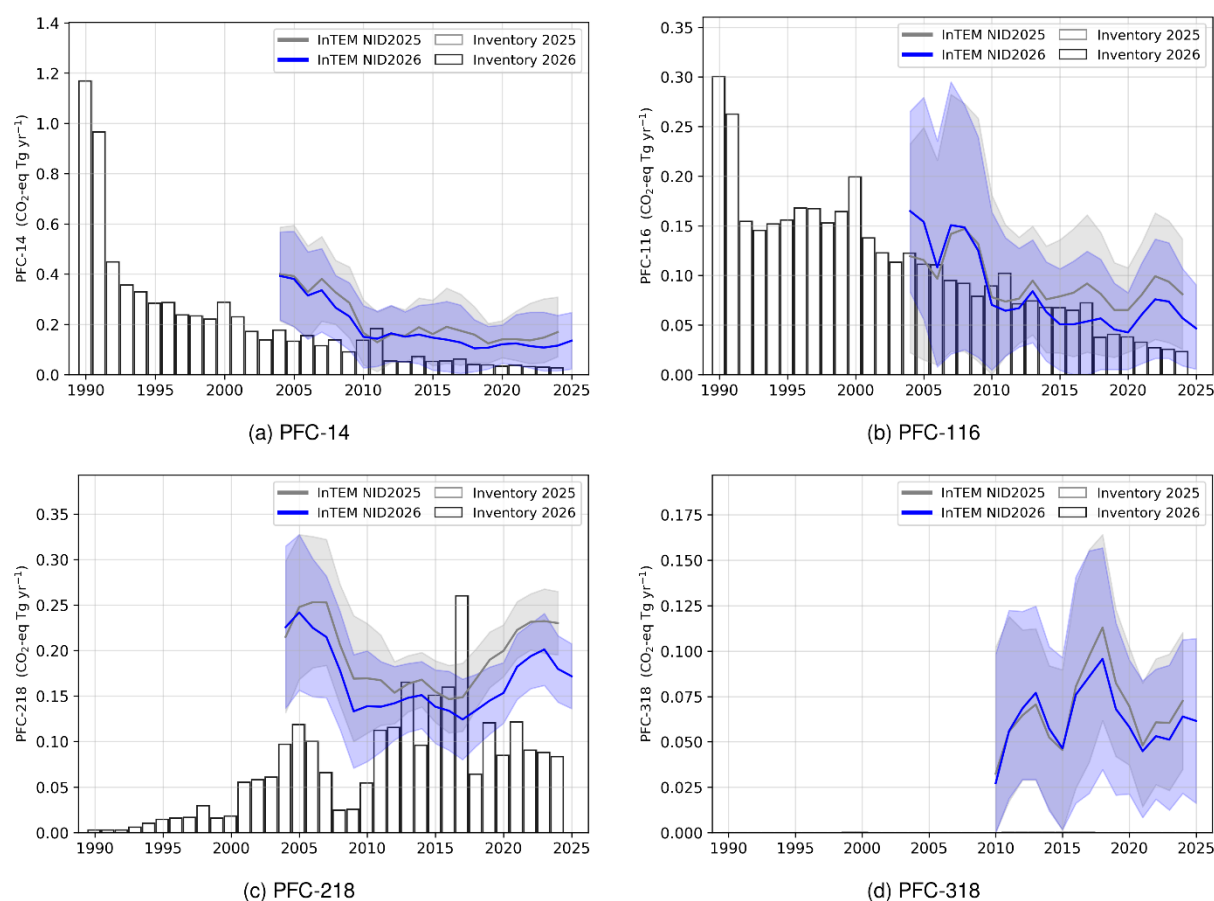
Figure A 6.5.3 Comparison of the UK emission inventory estimates for individual PFCs in Tg CO 2 e yr -1 from 1990. GHGI estimates are shown as black bars (GHGI 2025 as grey bars) (individual uncertainties by gas are not available). InTEM 1-year estimates, with a 3-year moving average applied, are shown as a blue line ( \pm 1\sigma ), (InTEM NID2025 result as a grey line). Note, for PFC-318 the inventory estimates are too small to be seen on the plot.
