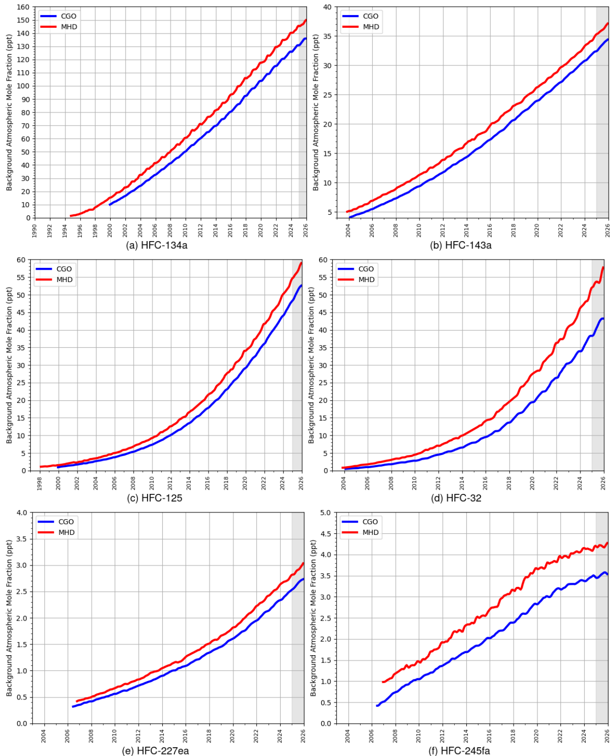
Figure A 6.4.2 Background Northern Hemisphere monthly concentrations of six HFCs estimated from MHD, Ireland observations are shown in red, and background Southern Hemisphere monthly concentrations from CGO, Tasmania are shown in blue. Grey shading represents unratified data.
