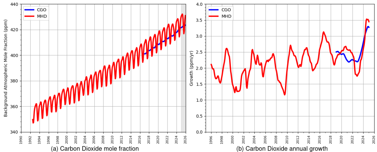
Figure A 6.8.1 Background Northern Hemisphere monthly concentrations and growth rates of CO 2 estimated from MHD, Ireland, observations are shown in red, and background Southern Hemisphere monthly concentrations and growth rates from CGO, Tasmania are shown in blue. Grey shading represents unratiified data.
