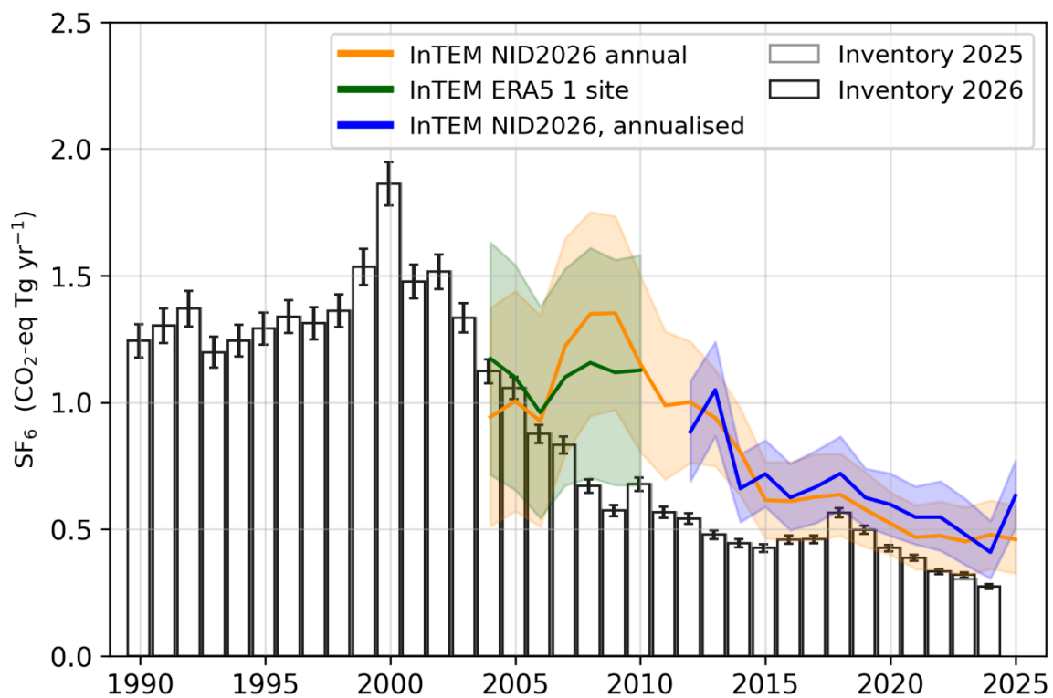
Figure A 6.6.2 Verification of the UK emission inventory estimates for SF 6 in Tg CO 2 e yr -1 from 1990. GHGI estimates are shown in black (2025 GHGI in grey). InTEM 1-year estimates, with a 3-year moving average applied, are shown in orange and InTEM annualised 1-month estimates are shown in blue. InTEM run for 1 site with ERA5 met data is shown in green. Uncertainties are given as \pm 1\sigma .
