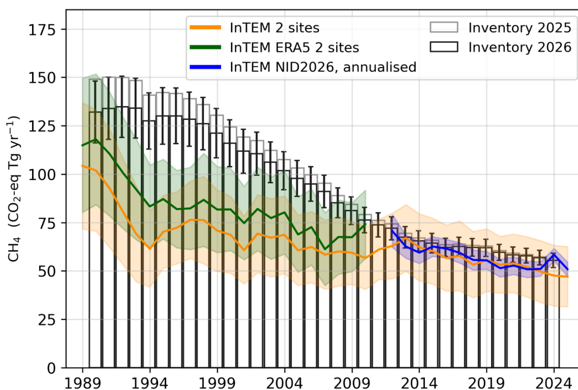
Figure A 6.2.2 Verification of the UK emission inventory estimates for CH 4 in Tg CO 2 e yr -1 from 1990. GHGI 2026 estimates are shown in black ( \pm 1\sigma ), the GHGI 2025 estimates are shown in grey. InTEM 2-sites 1-year estimates, using the standard meteorology and the new ERA5 meteorology, with a 3-year moving average applied, are shown in orange and green respectively ( \pm 1\sigma ). InTEM full network, 1-month annualised, estimates are shown in blue ( \pm 1\sigma ).
