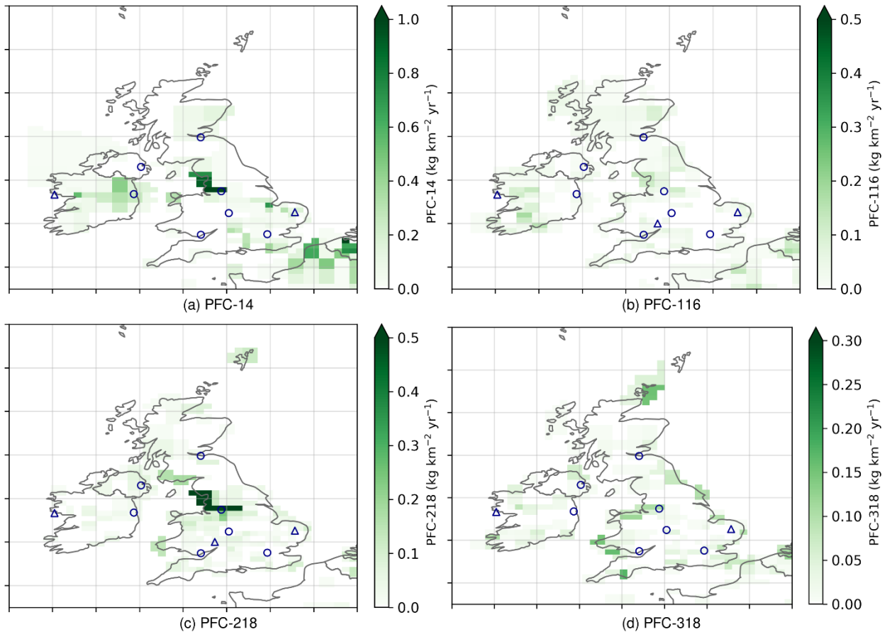
Figure A 6.5.4 Four-year average PFC InTEM emission estimates ( \text{kg km}^{-2} \text{yr}^{-1} ) 2022-2025. The observation stations are shown as blue triangles. Major cities are shown as blue circles.
