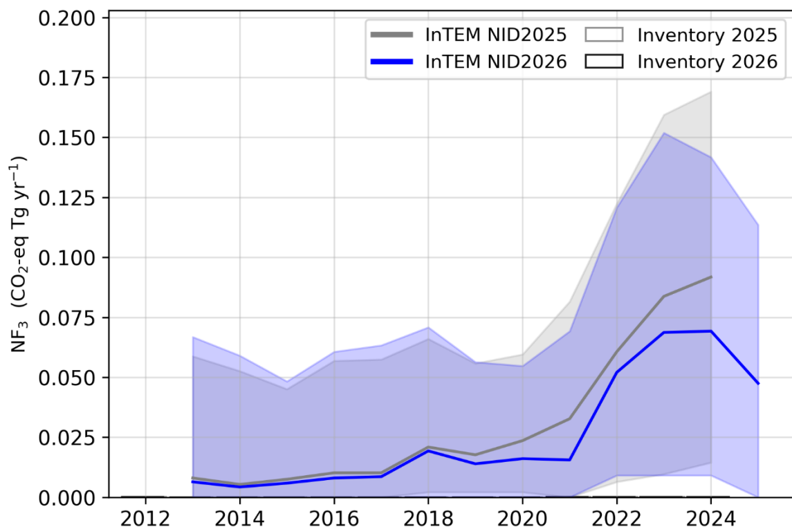
Figure A 6.7.1 Verification of the UK emission inventory estimates for NF 3 in Tg CO 2 e yr -1 from 2012. InTEM 1-year estimates, with a 3-year moving average applied, are shown in blue (±1σ) (2025 results in grey). Note, the inventory estimates are too small to be seen on the plot.
