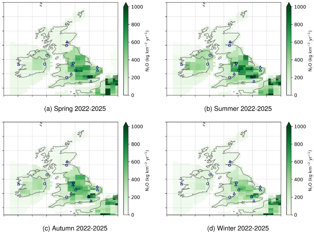
Figure A 6.3.3 Four-year average \text{N}_2\text{O} InTEM emission estimates ( \text{kg km}^{-2} \text{yr}^{-1} ) 2022-2025 by season: (a) Spring (b) Summer (c) Autumn and (d) Winter. The observation stations are shown as blue triangles. Major cities are shown as blue circles.
