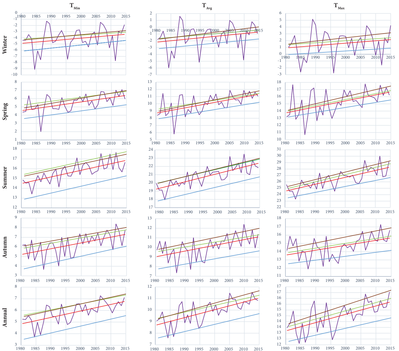
Figure 1-7: Trends in air temperature over period 1981-2015: Briceni – blue, Chisinau – green, Cahul – brown, the red linear trend – the average for the RM; the violet curve shows the inter-annual temperature variability for the Republic of Moldova.
