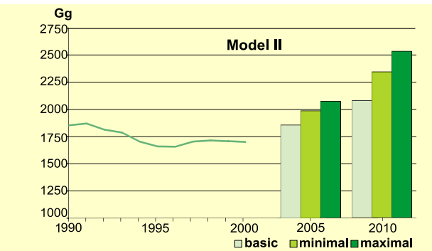
Figure 3.8. Prognosis of CO 2 reduction resulting from agricultural land use change and forestry, Gg
