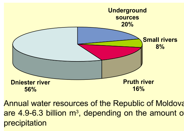
Figure 5.8. Water resources of the Republic of Moldova
