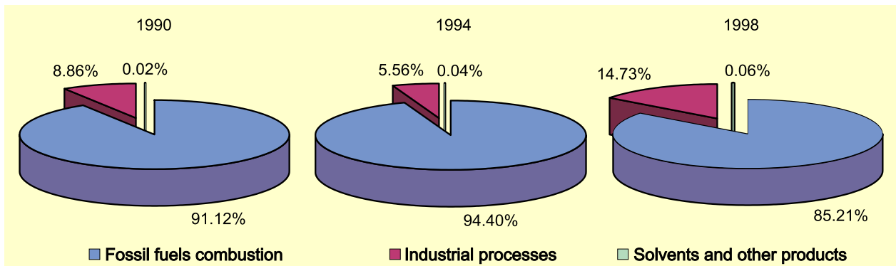
Figure 2.1. Structure of CO 2 emissions in 1990, 1994 and 1998
