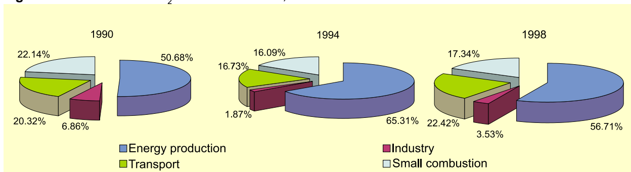
Figure 2.2 Structure of CO 2 emissions in the Energy sector in 1990, 1994 and in 1998
