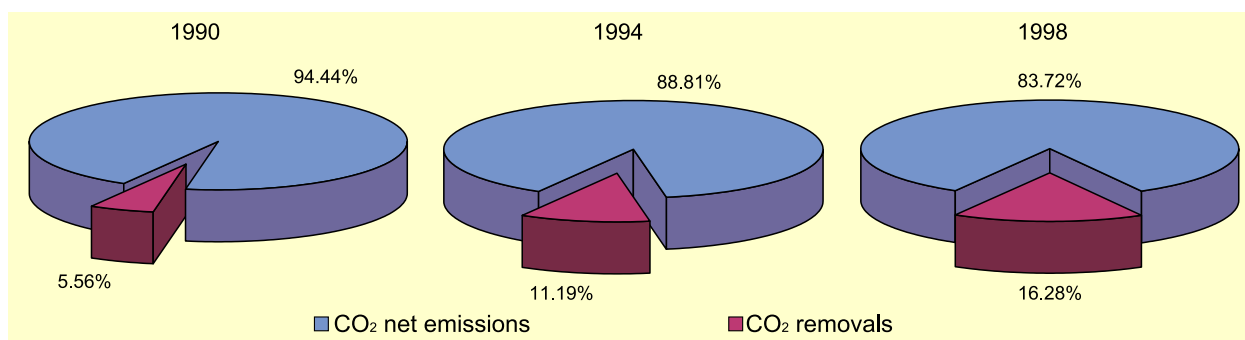
Figure 2.13. Storage potential of CO 2 emissions by forests in 1990, 1994 and 1998
