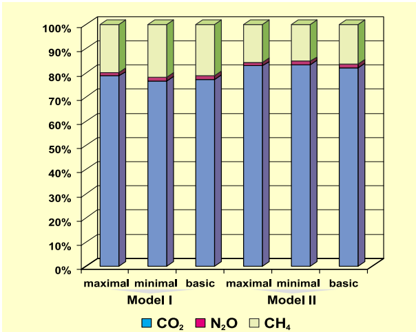
Figure 3.6 Prognoses of the structures of total direct GHG emissions expressed in CO 2 equivalents in 2010
