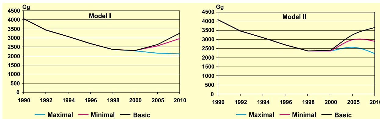
Figure 3.4 Prognoses of CH 4 emissions expressed in CO 2 equivalents until 2010
