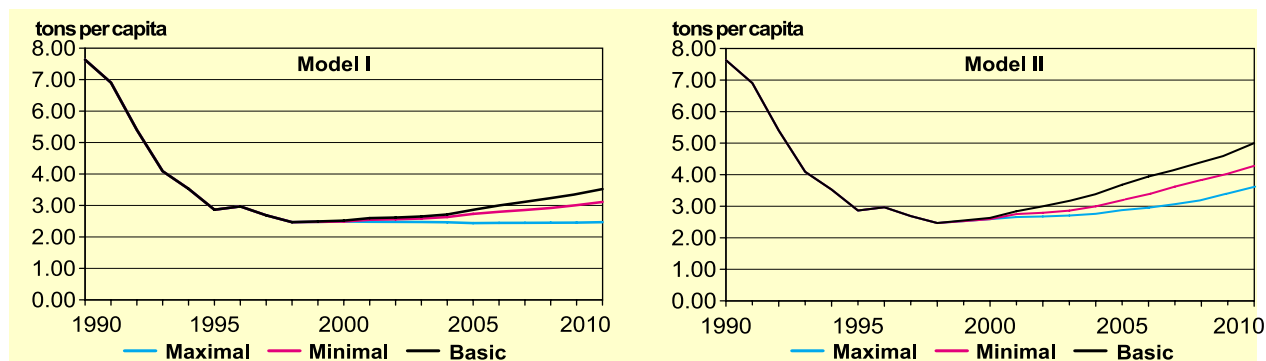
Figure 3.1. Progress of the total emissions of gases with direct greenhouse effect per capita
