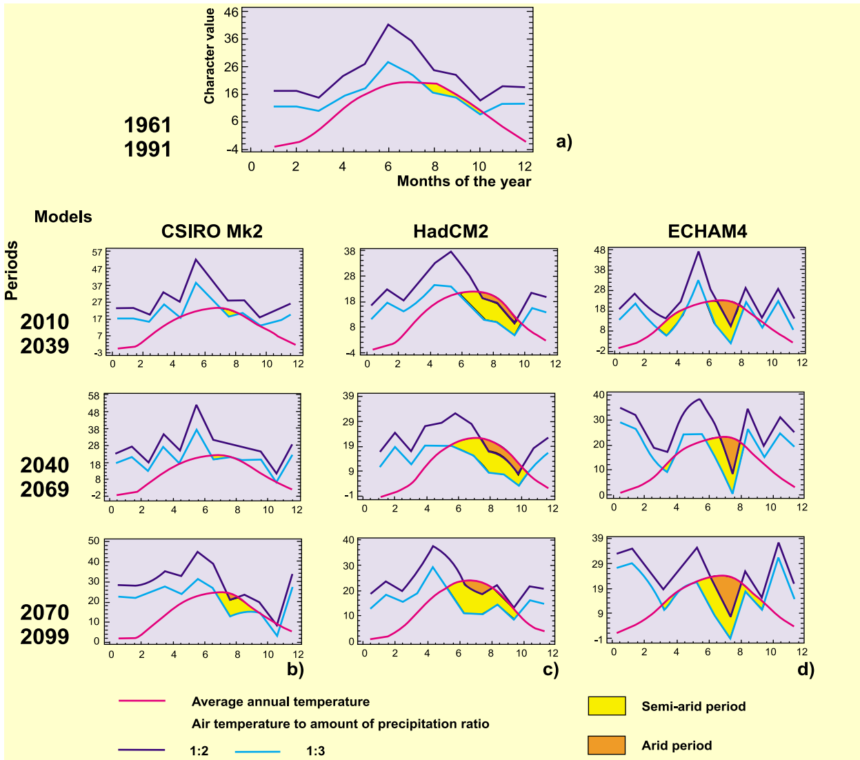
Figure 5.5 Climate diagrams for various climate change scenarios on the territory of the Republic of Moldova
