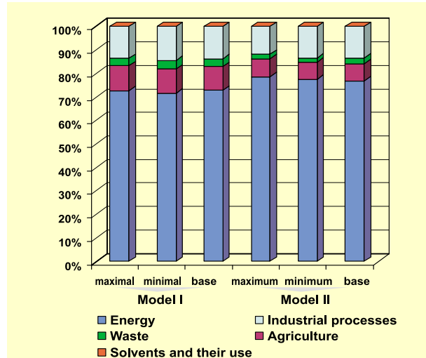
Figure 3.7 Prognoses of total direct GHG emissions expressed in CO 2 equivalents (depending on sources) in 2010
