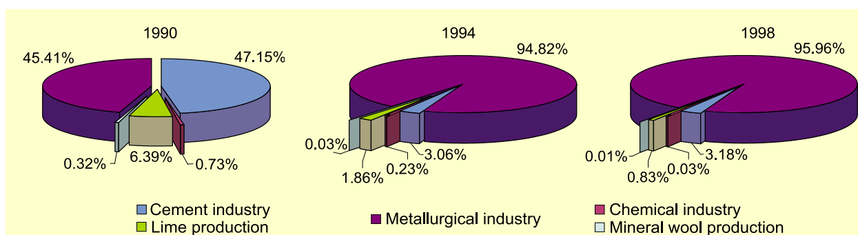
Figure 2.3 Structure of CO 2 emissions in the Industrial processes sector in the years 1990, 1994 and 1998
