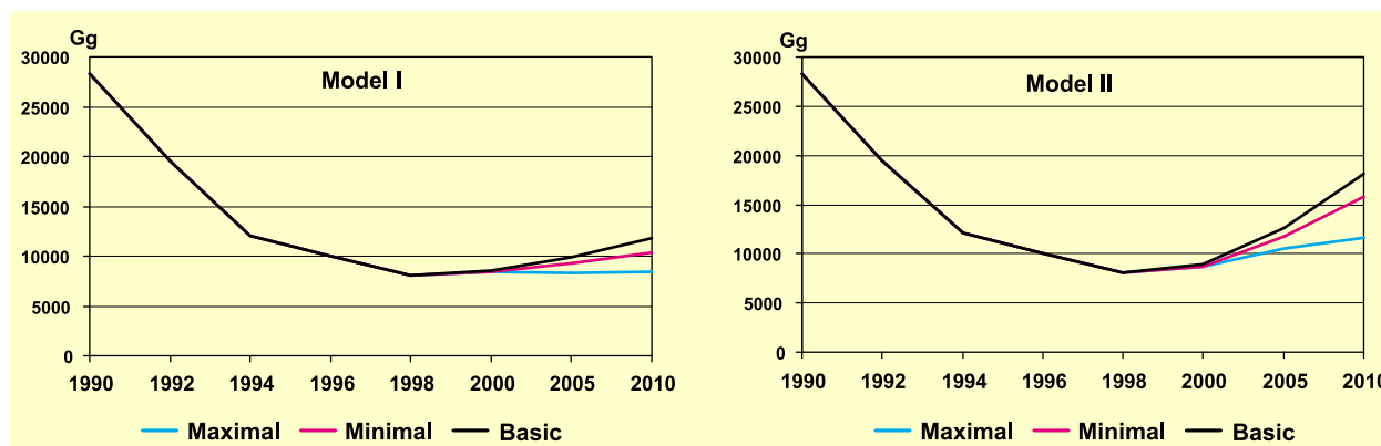
Figure 3.3 Prognoses of CO 2 emissions until 2010
