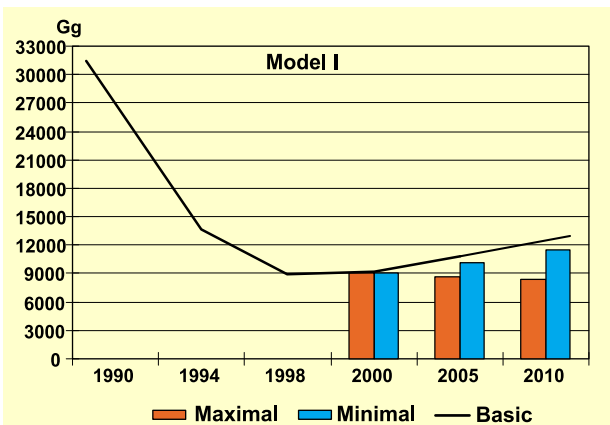
Figure 3.9. Prognosis of net direct greenhouse gas emissions expressed in CO 2 equivalents
