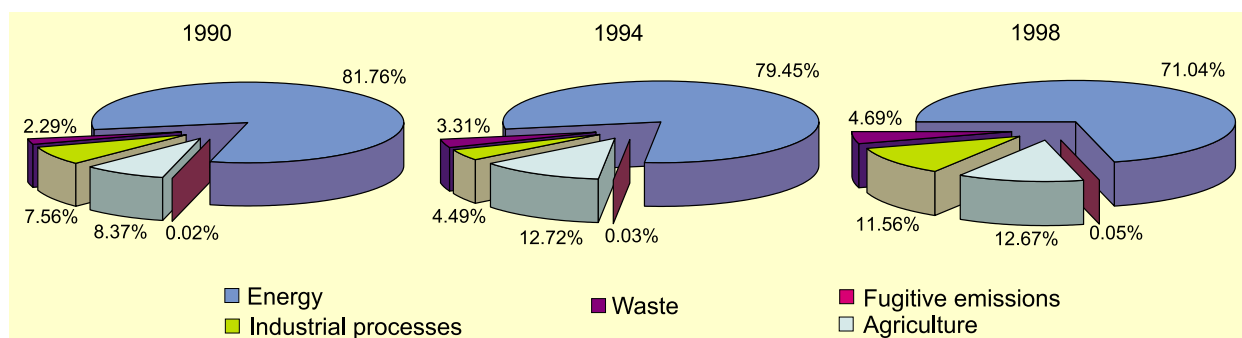
Figure 2.10 Total emissions expressed in CO 2 equivalents by sources
