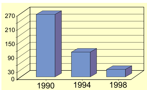
Figure 2.9 SO 2 emissions in 1990, 1994 and 1998
