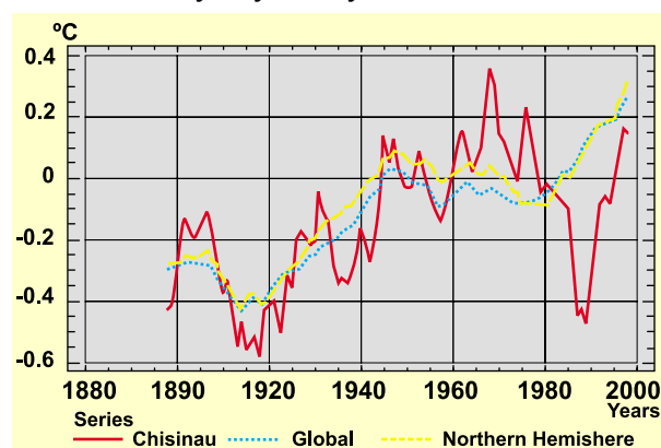
Figure 7.1. Average air temperature fluctuations as compared with the reference period, 1961-1990
