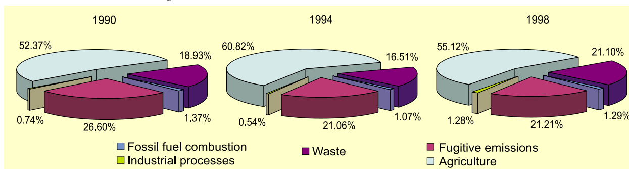
Figure 2.4 Structure of CH 4 emissions in the years 1990, 1994 and 1998
