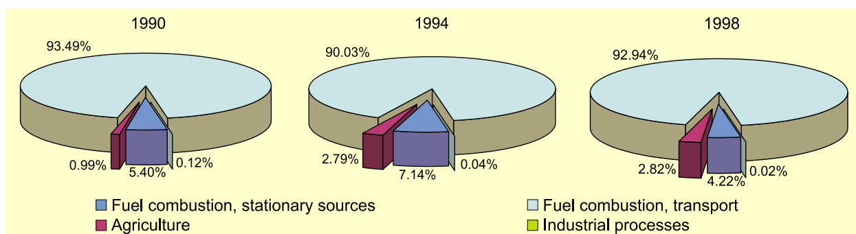
Figure 2.7 Structure of CO emissions in 1990, 1994 and 1998
