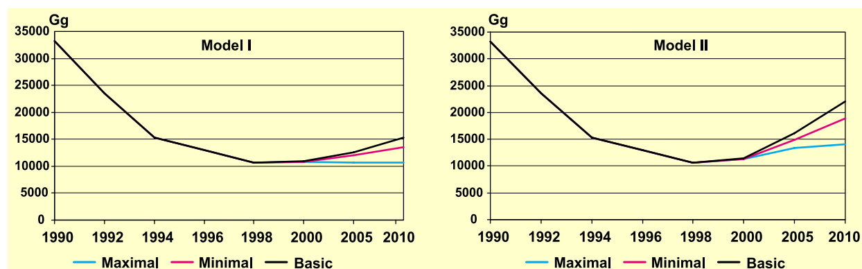
Figure 3.2 Prognoses of total direct greenhouse gas emissions expressed in CO 2 equivalents
