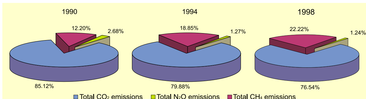
Figure 2.12 Total greenhouse gas emissions expressed in CO 2 equivalents in 1990, 1994 and 1998
