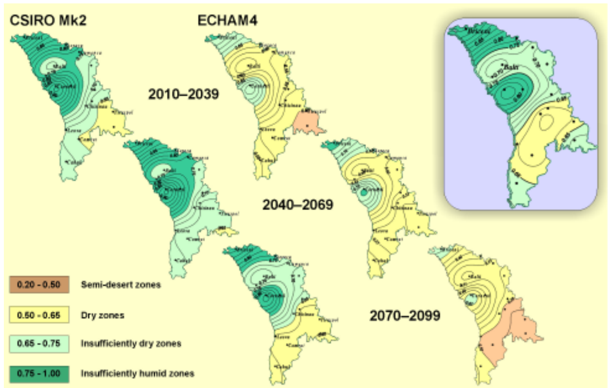
Figure 5.6. Change of Aridity Degree on the Territory of the Republic of Moldova according to CSIRO Mk2 and ECHAM4 Scenarios
