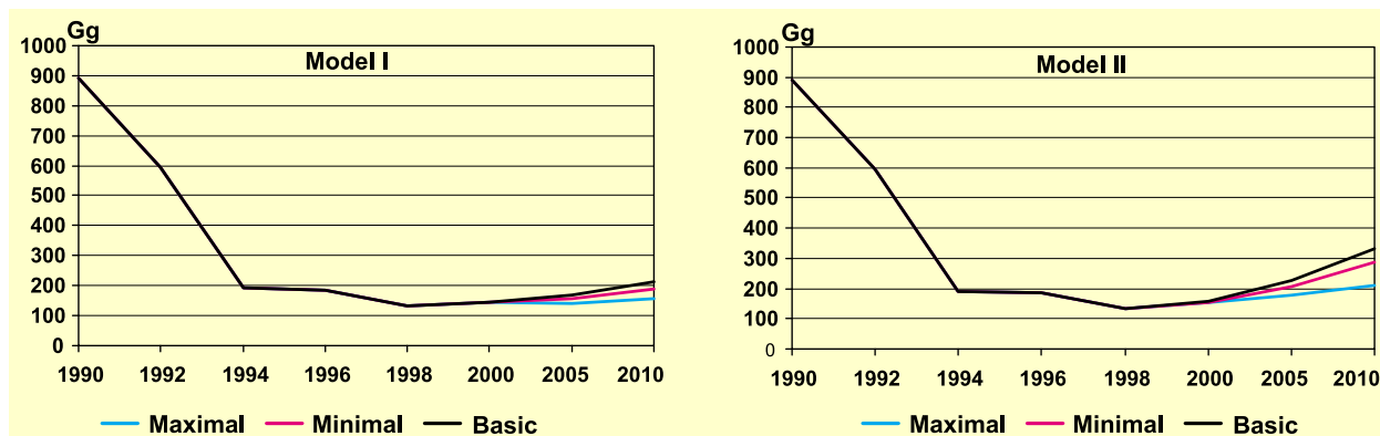
Figure 3.5 Prognoses of N 2 O emissions expressed in CO 2 equivalents until 2010
