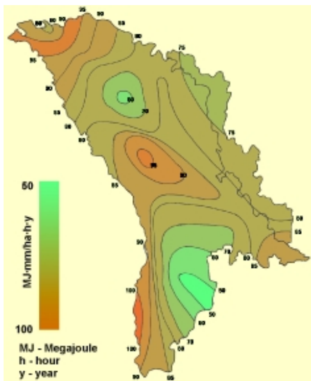
Figure 7.4. Soil erosion degree depending on erodibility index of rains intensity
