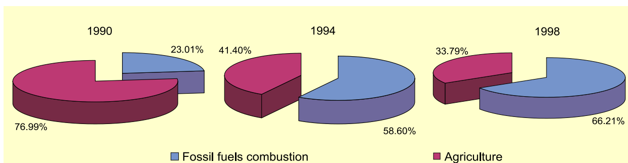
Figure 2.5 Structure of N 2 O emissions in the years 1990, 1994 and 1998
