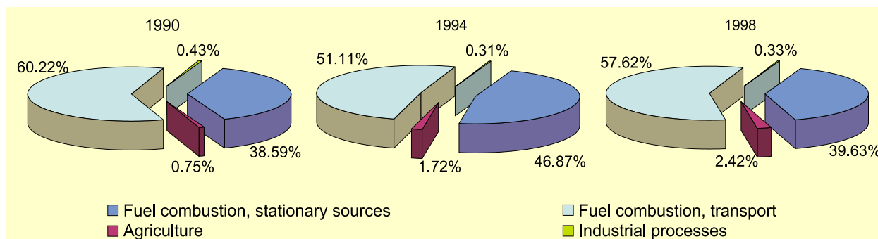
Figure 2.6 Structure of NO x emissions in 1990, 1994 and 1998
