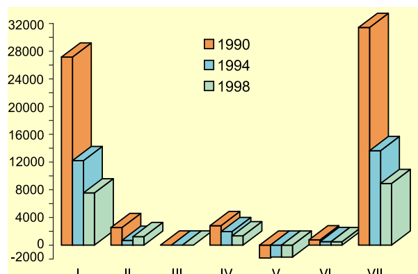
Figure 2.11 Total direct greenhouse gas emissions expressed in CO 2 equivalents
