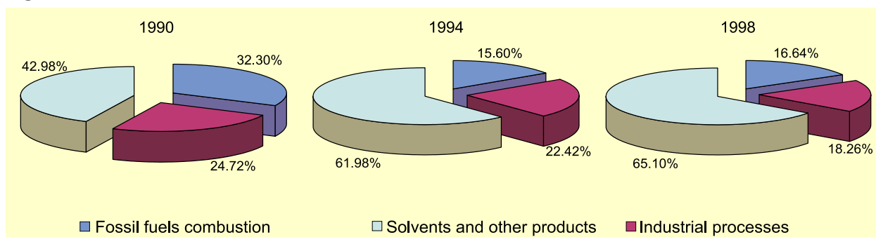
Figure 2.8 Structure of NMVOC emissions in 1990, 1994 and 1998
