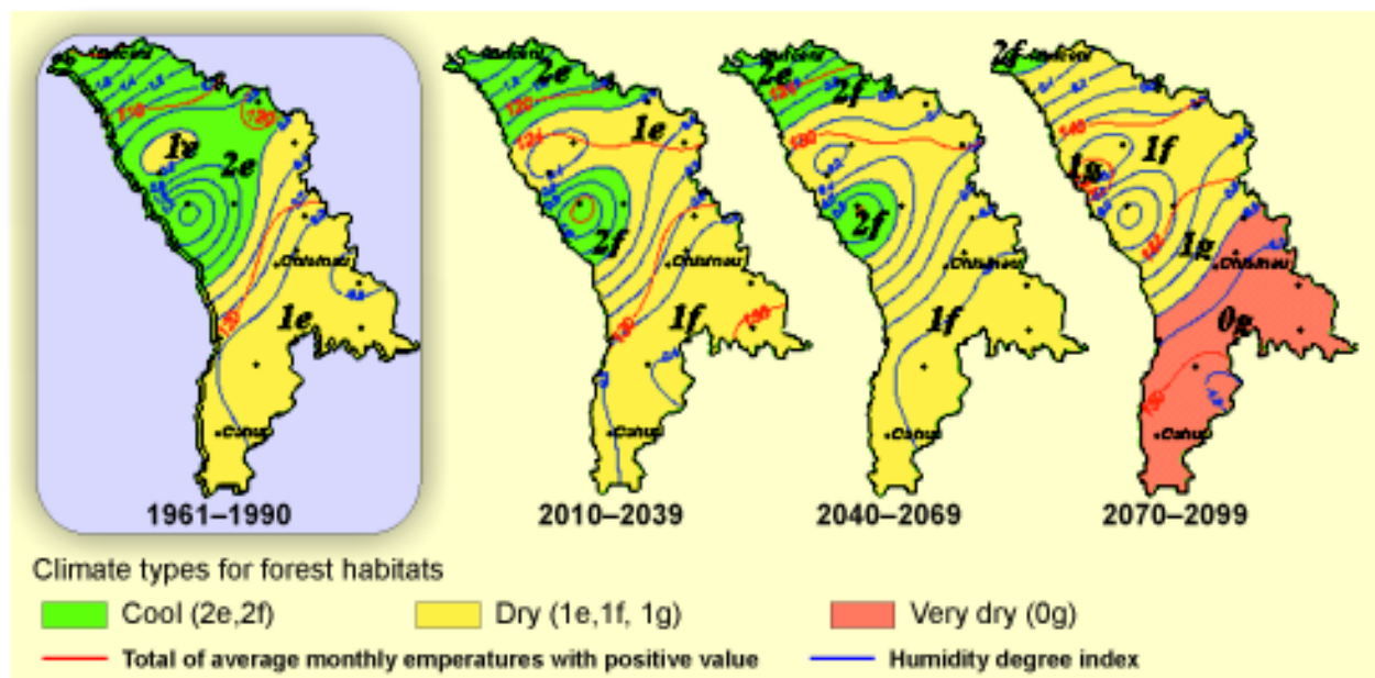
Figure 5.7. Climatic conditions evolution for the forest habitats of the Republic of Moldova according to CSIRO Mk2 scenario
