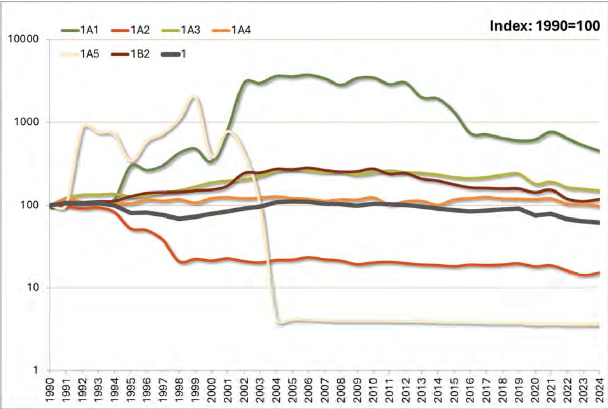
Figure 3-2 – GHG emission trend indexes for CRT Sector 1 – Energy: 1990-2024
