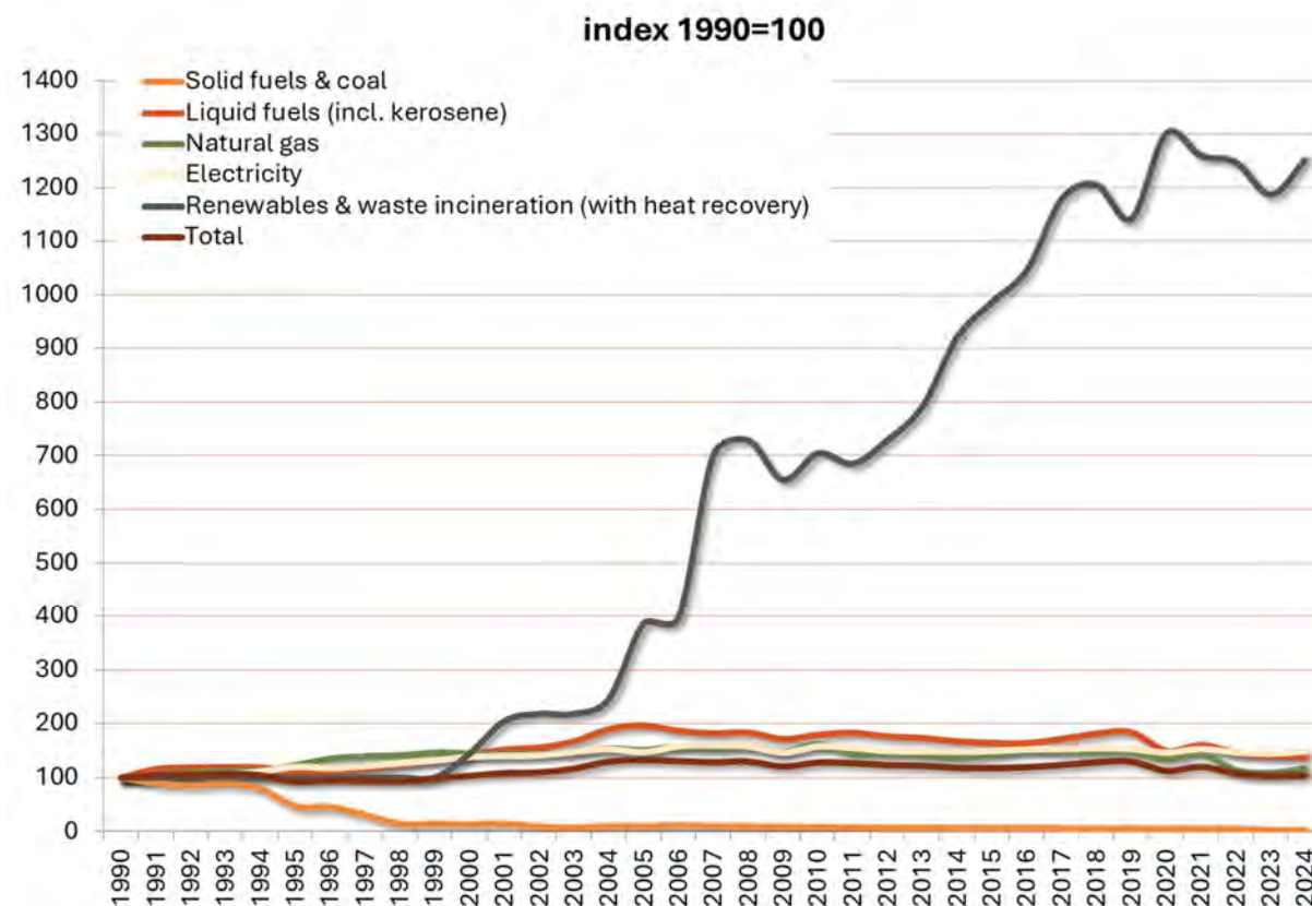
Figure 2-20 – Final energy consumption: 1990-2024
