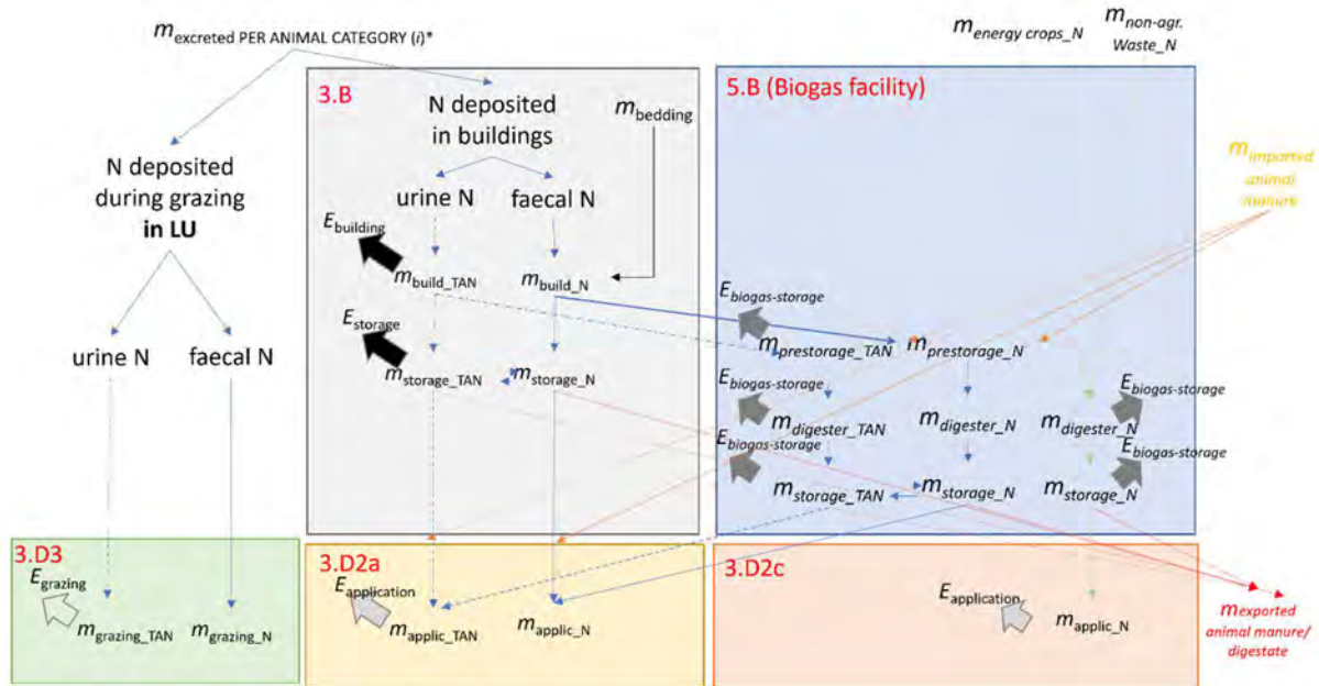
Figure 5-6 – N flow in the manure management system
