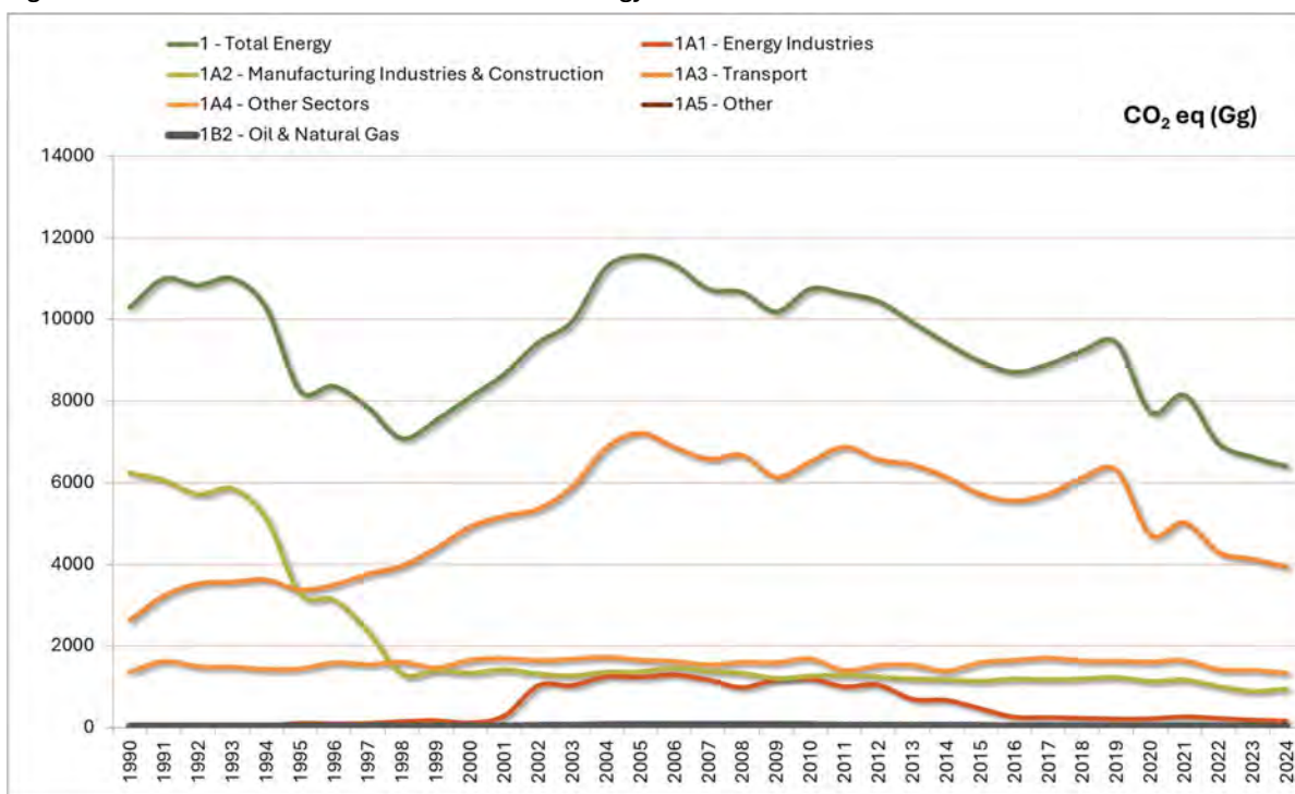
Figure 3-1 – GHG emission trends for CRT Sector 1-Energy: 1990-2024
