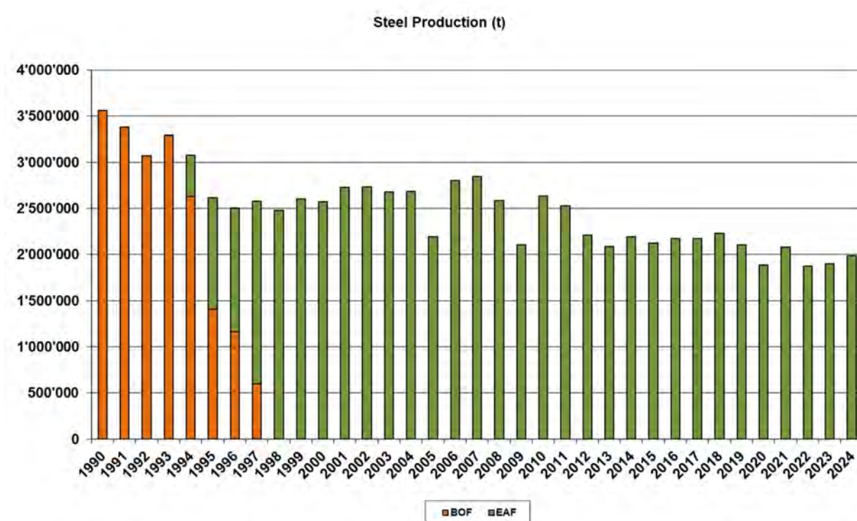
Figure 4-5 – Steel production according to BOF and EAF: 1990-2024
