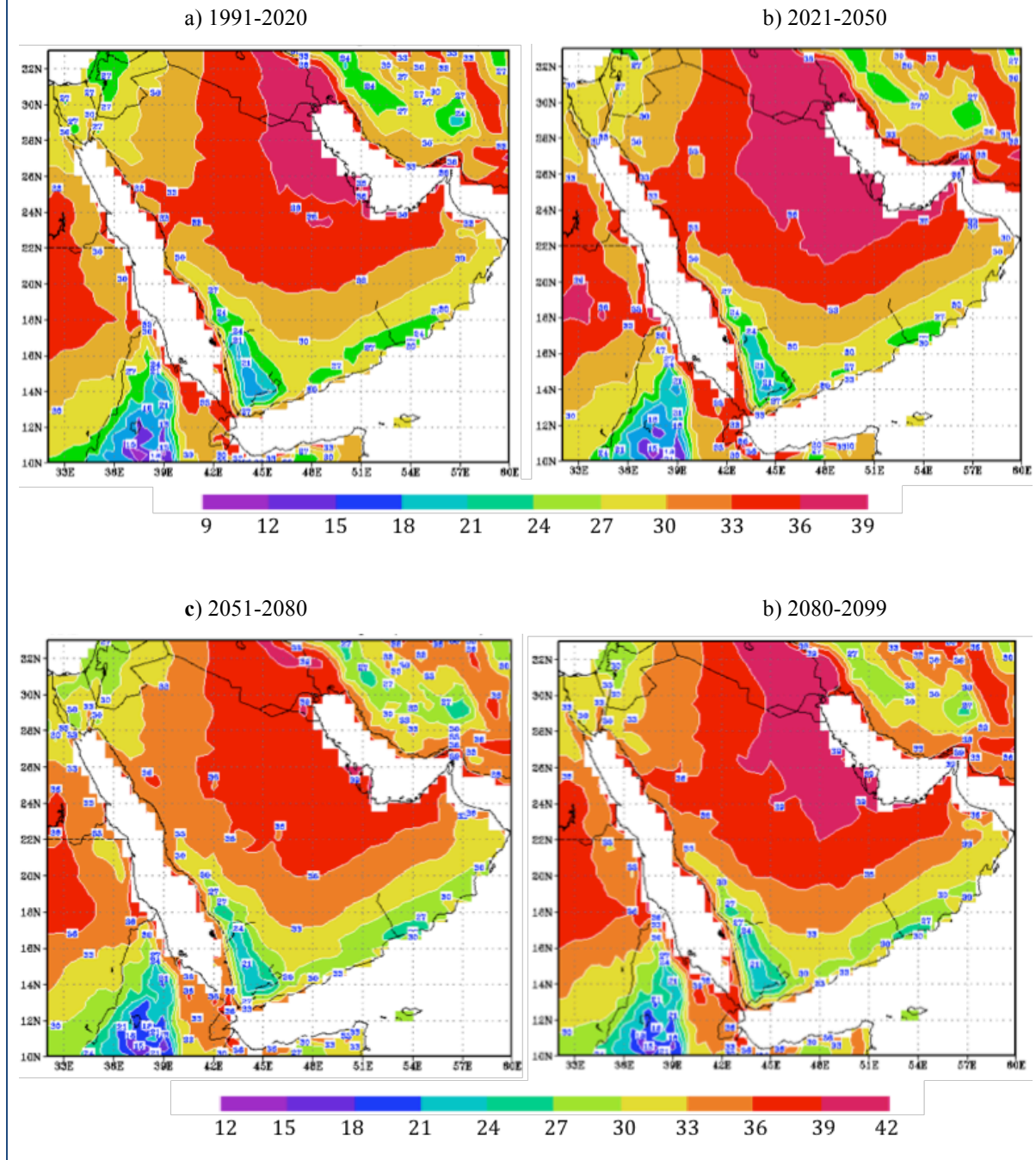
Figure 3-6: HadCM3 projected mean temperature in July at 2 meters above ground level
