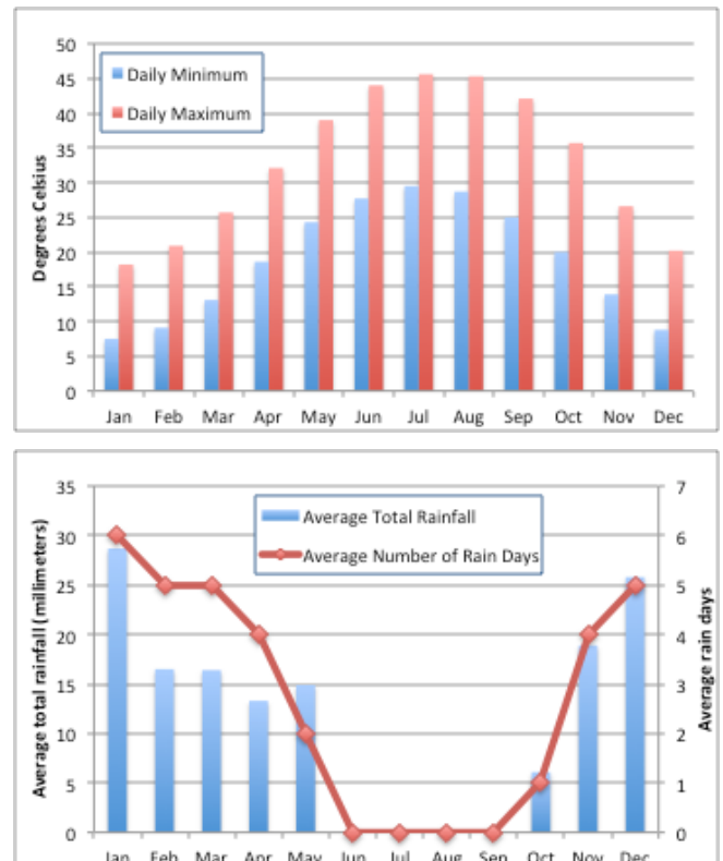
Figure 1-5: Kuwait average monthly temperature and rainfall, 1962-2008 (source: Kuwait Meteorology Department)
