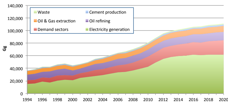
Figure 4-2: Baseline Scenario CO 2 e emissions in Kuwait, 1994-2020
