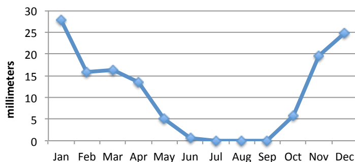
Figure 3-3: Average monthly rainfall in Kuwait, 1957-2010
