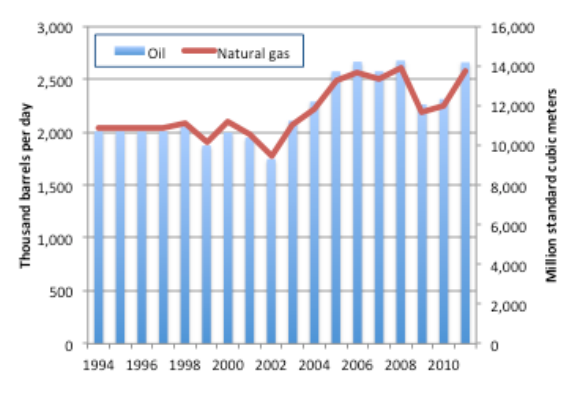
Figure 1-10: Kuwait gross production of oil and natural gas, 1994-2010 (source: OPEC Annual Statistical Bulletins)
