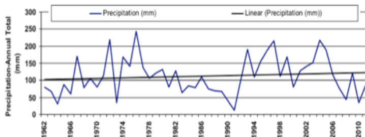
Figure 3-4: Average annual rainfall in Kuwait, 1962-2010
