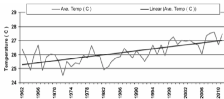
Figure 3-2: Average annual temperature trend in Kuwait, 1962-2010
