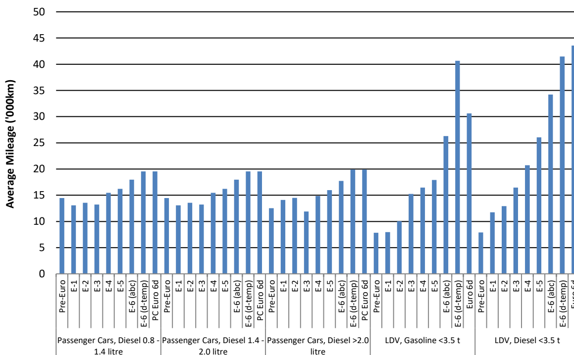
Figure 3.10.5 Average Balanced Vehicle mileage for Diesel Passenger car and LDV (2023)
