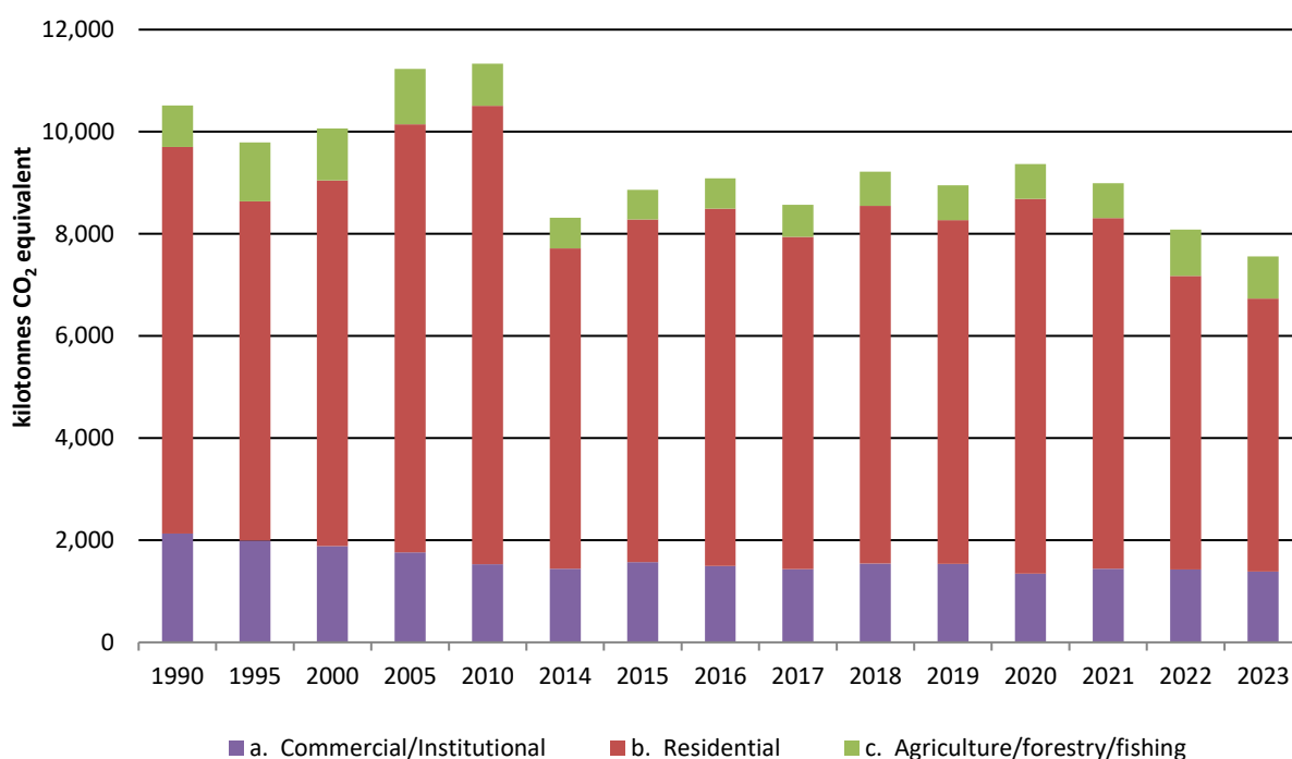
Figure 3.11 Emissions from 1.A.4 Other Sectors 1990-2023
