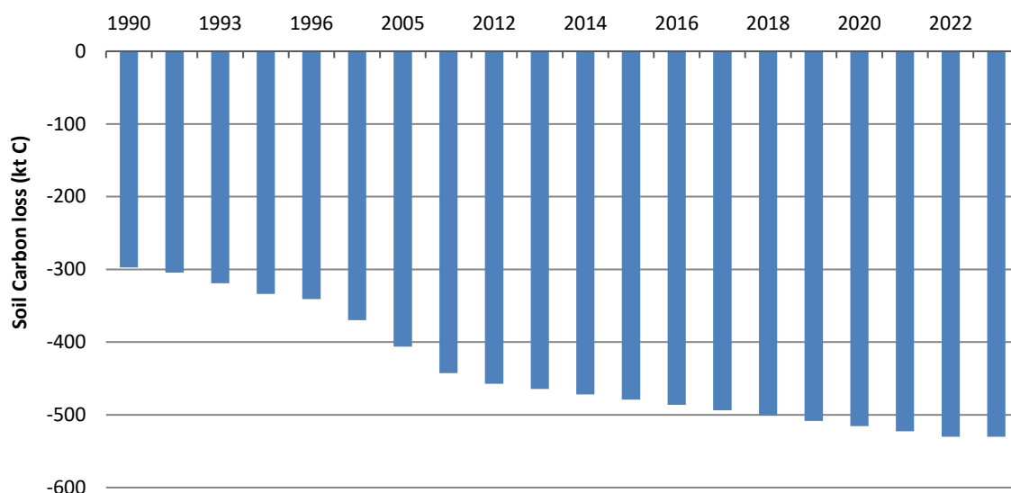
Figure 6.30 Time series of carbon loss from drained organic soils under grassland Rewetting of previously drained organic soils under grassland area
