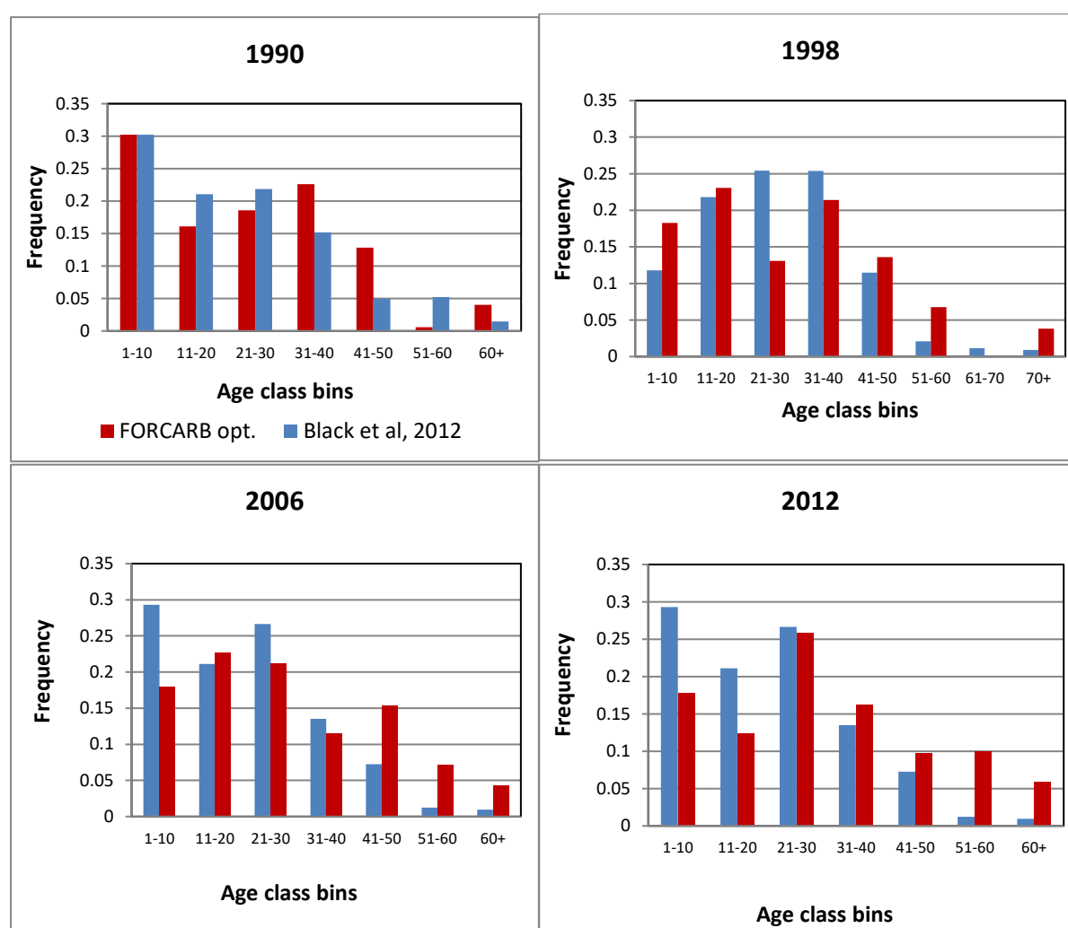
Figure 3.4.C-1 Validation of optimised age-class distributions
