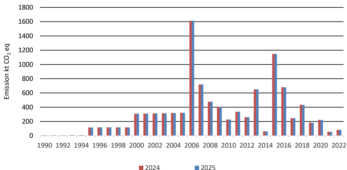
Figure 6.15 Comparison of deforestation emissions for the 2024 and 2025 submissions
