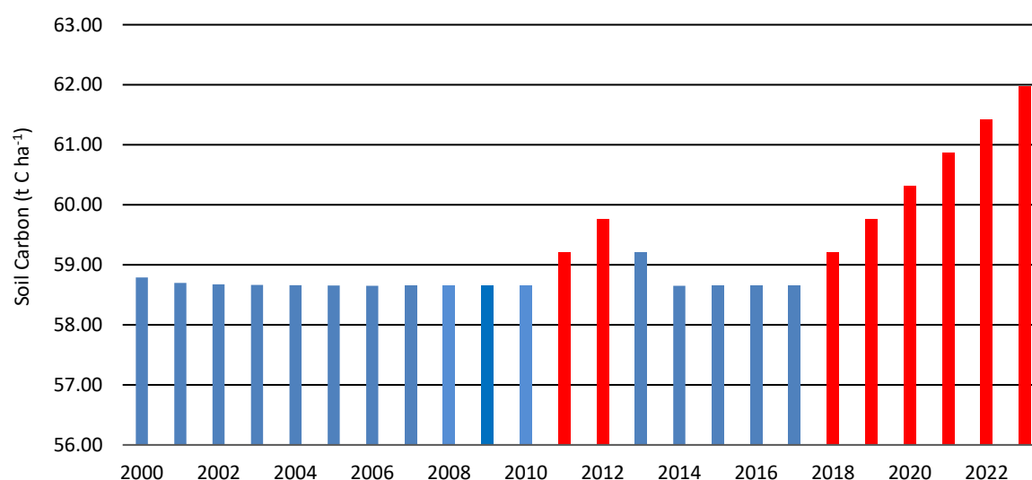
Figure 6.23 Estimated Soil Carbon per hectare based on the crop rotation pattern outlined in Table 6.30 for the period 2000-2023
