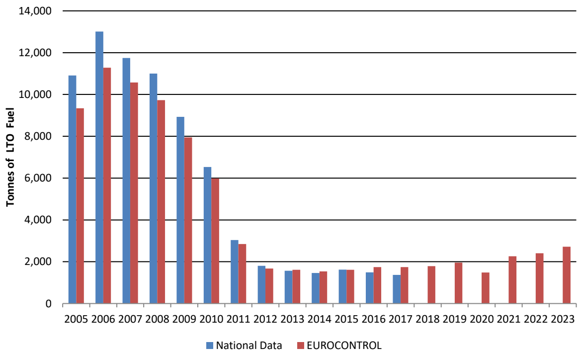
Figure 3.8 National LTO fuel data and EUROCONTROL LTO fuel data for 2005-2023
