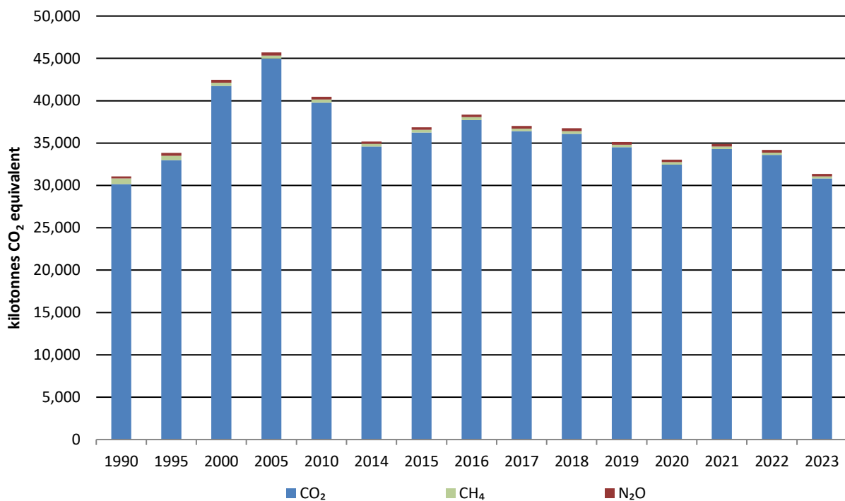
Figure 3.2 Total Emissions from Energy by Gas, 1990-2023
