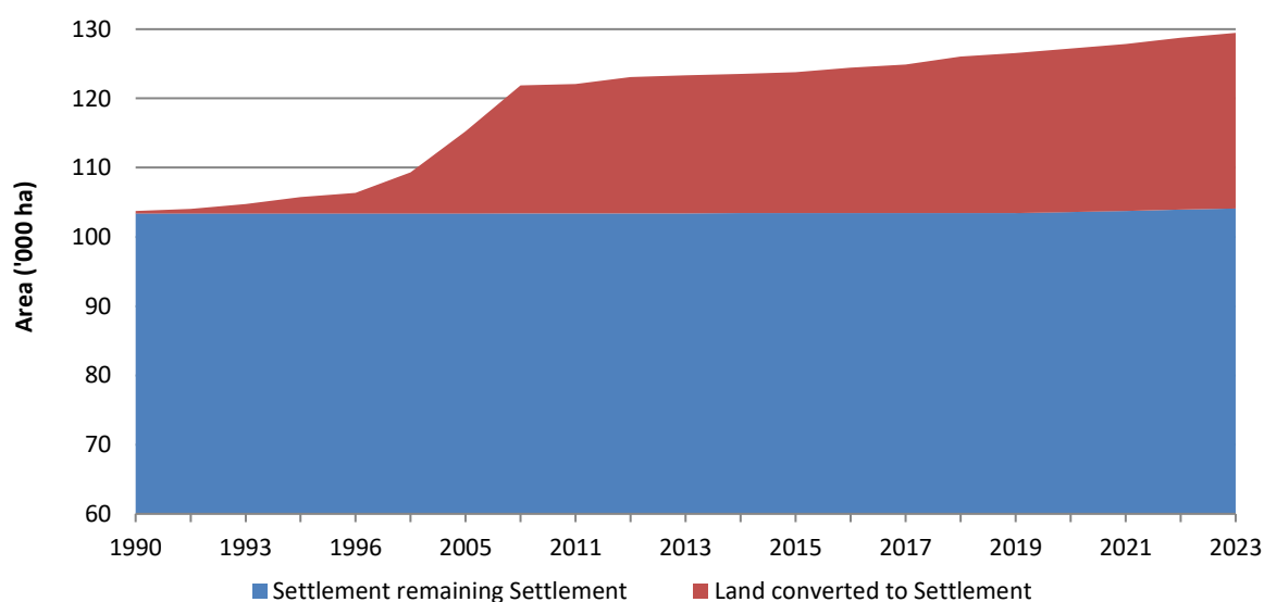
Figure 6.37 Estimated area of Settlements 1990 to 2023
