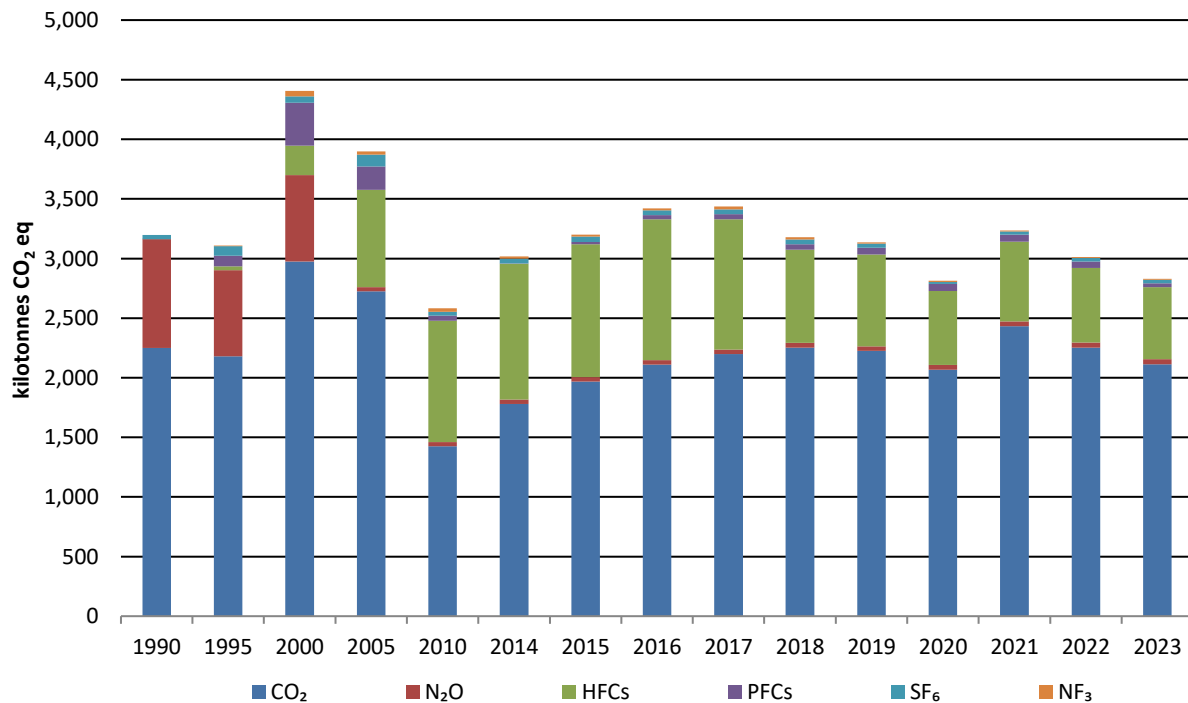
Figure 4.2 Total Emissions from IPPU by Gas, 1990-2023
