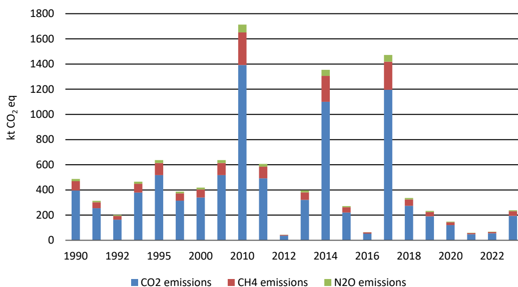
Figure 6.35 Estimate emissions (kt CO 2 eq) due to biomass burning on wetlands
