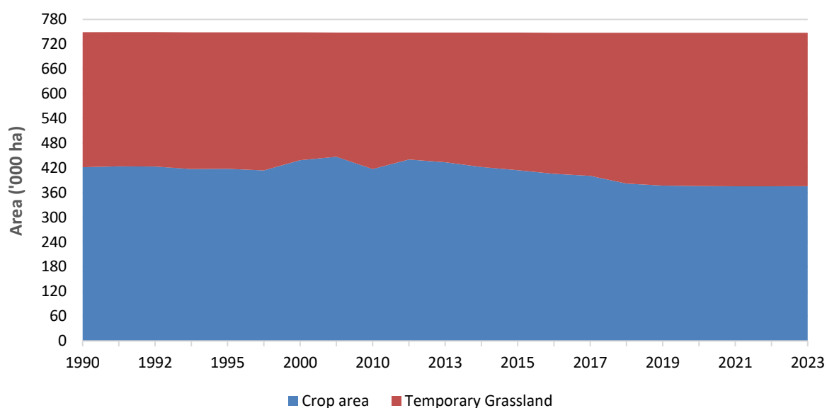
Figure 6.22 Time series of Cropland 1990 to 2023
