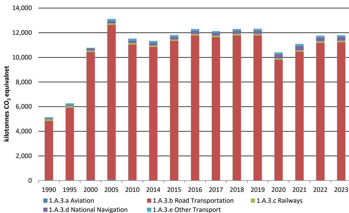
Figure 3.5 Emissions from 1.A.3 Transport 1990-2023
