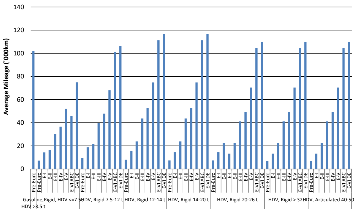
Figure 3.10.6 Average Balanced Vehicle mileage for HD Vehicle categories (2023)
