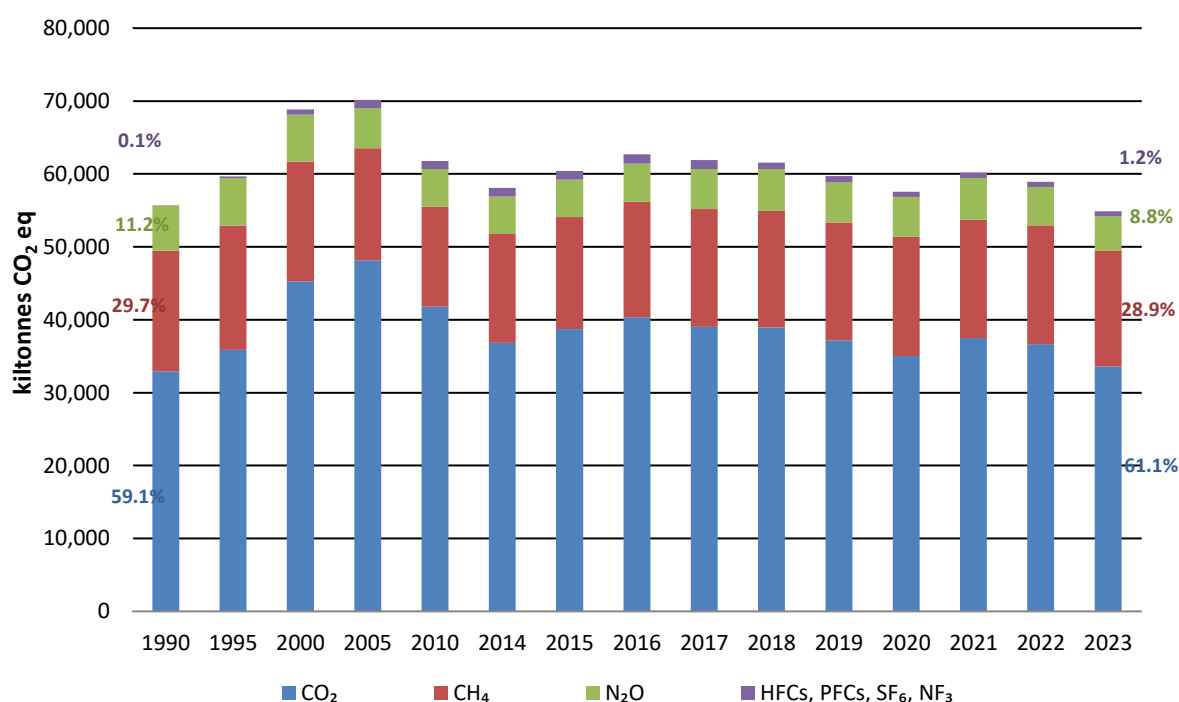
Figure 2.3 Greenhouse Gas emissions-by Gas (excluding LULUCF) 1990-2023
