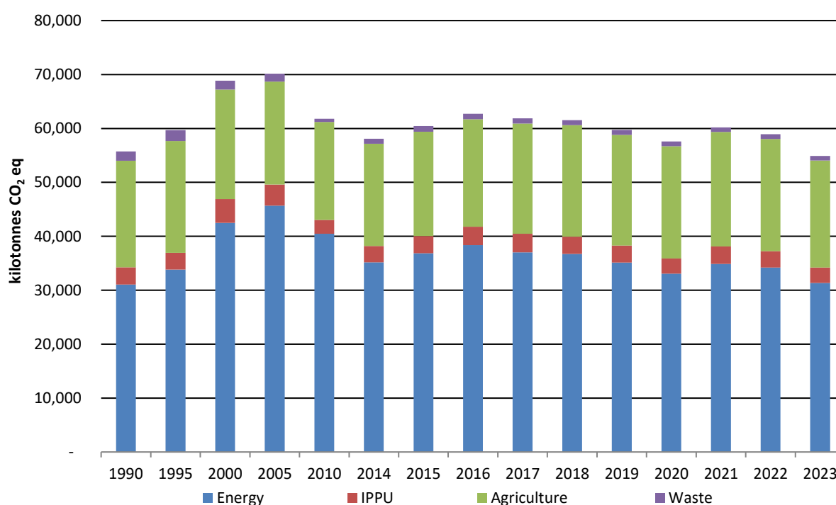
Figure 2.1 National total Greenhouse Gas emissions (excluding LULUCF) 1990-2023
