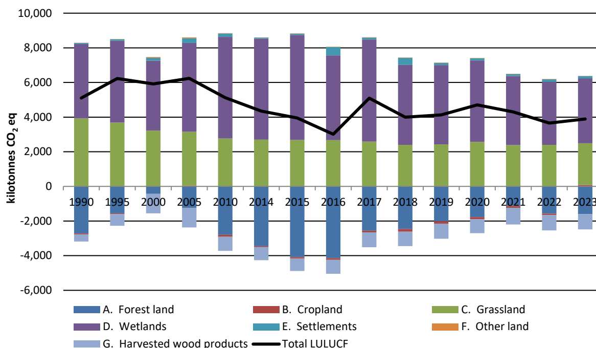
Figure 2.10 Trend in Emissions and Removals from Land Use Land-Use Change and Forestry 1990-2023
