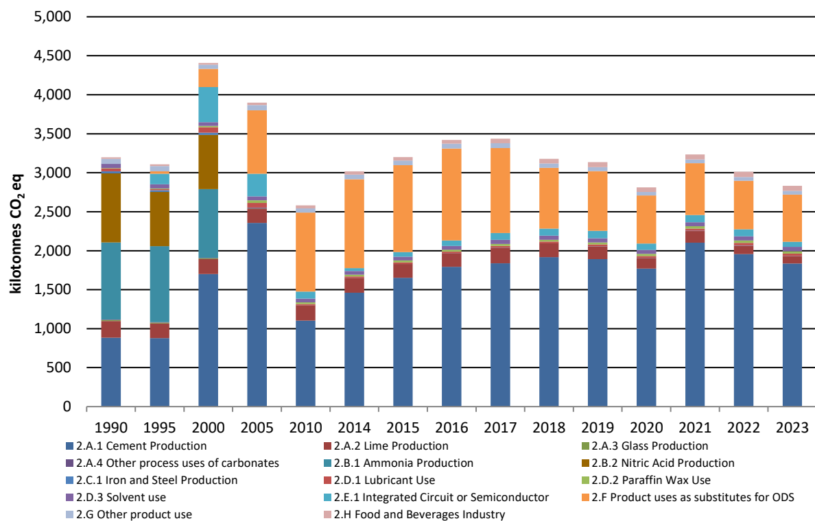
Figure 4.1 Total Emissions from IPPU by Category, 1990-2023
