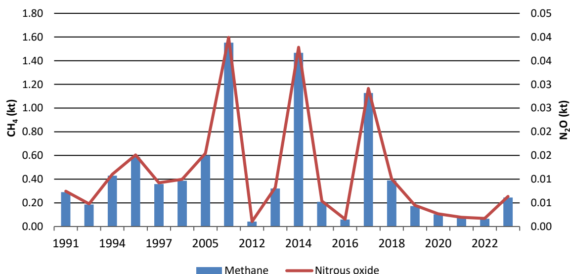
Figure 6.32 Estimated CH 4 and N 2 O emissions from biomass burning on Grassland
