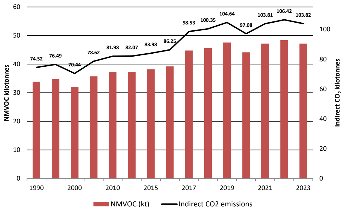
Figure 9.1 Total Indirect CO 2 emissions 1990-2023
