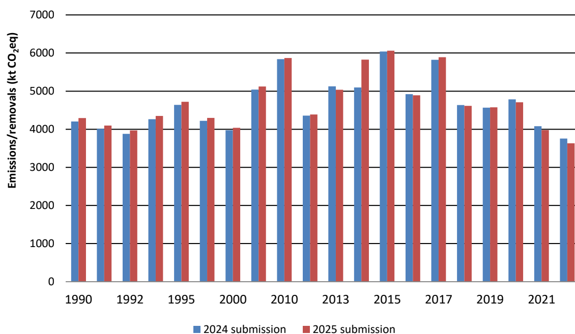
Figure 6.36 Comparison between the 2024 and 2025 submissions of estimated total emissions associated with the Wetlands category
