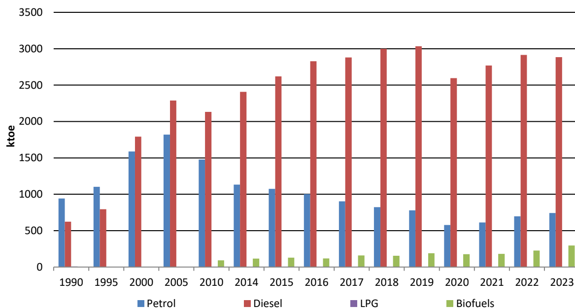
Figure 2.6 Fuel use in Road Transport 1990-2023
