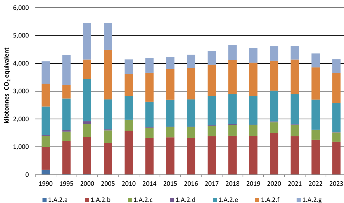
Figure 3.4 Emissions from 1.A.2 Manufacturing Industries and Construction 1990-2023
