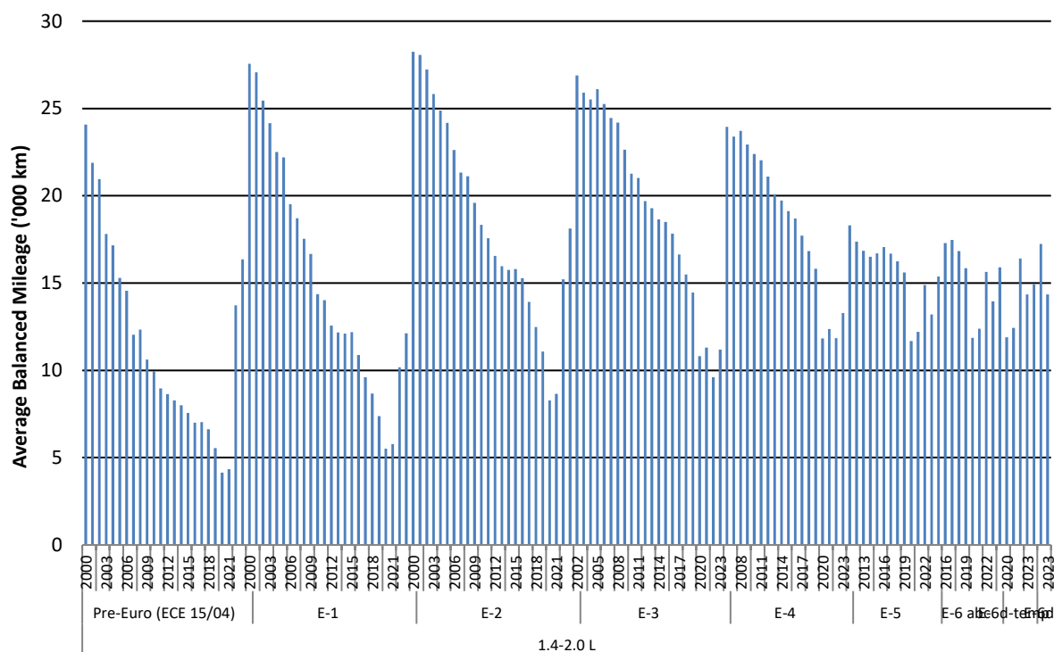
Figure 3.10.4 Average Balanced Vehicle mileage for Petrol PC 1.4-2L (2000-2023)
