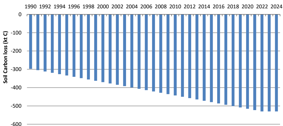
Figure 6.30 Time series of carbon loss from drained organic soils under grassland
