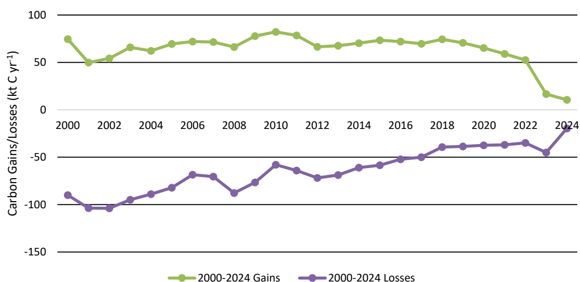
Figure 6.26 Time Series of estimated soil carbon gains and losses associated with rotational patterns of crop production and temporary grassland
