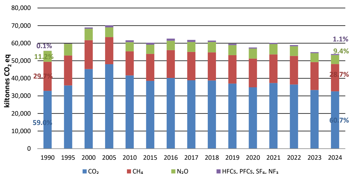
Figure 2.3 Greenhouse Gas emissions-by Gas (excluding LULUCF) 1990-2024
