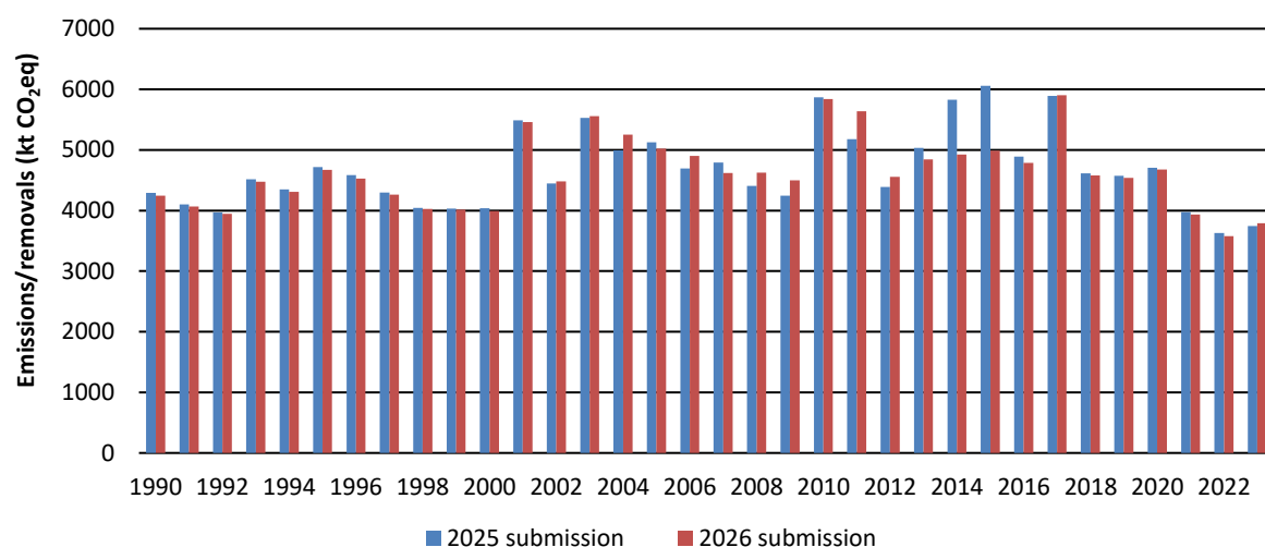
Figure 6.36 Comparison between the 2025 and 2026 submissions of estimated total emissions associated with the Wetlands category
