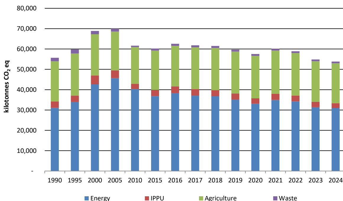
Figure ES.1 National total Greenhouse Gas emissions (excluding LULUCF) 1990-2024
