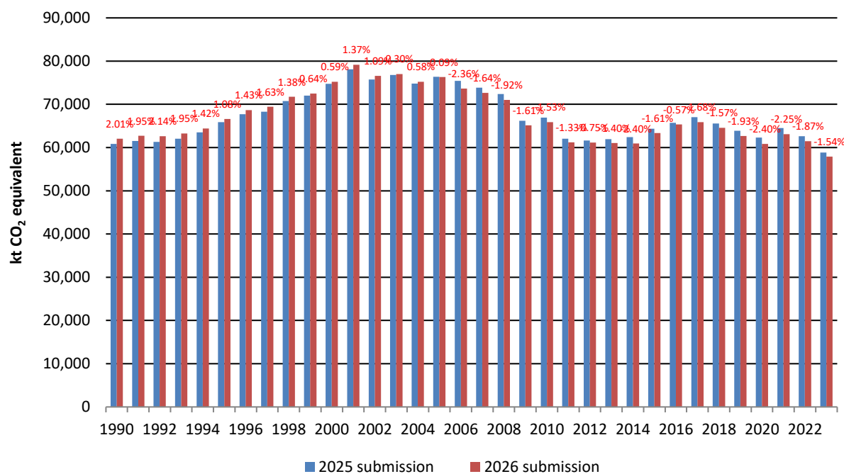
Figure 10.7 Total Impact of Recalculations between annual Submissions (with LULUCF) 1990-2023
