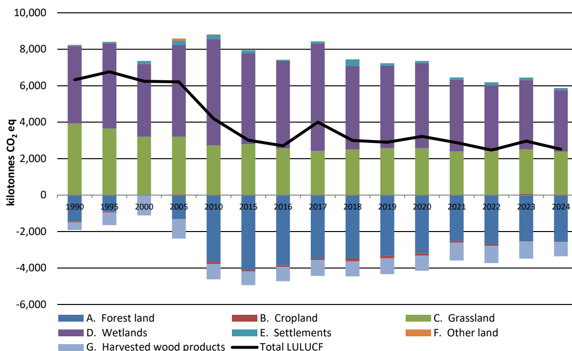
Figure 2.10 Trend in Emissions and Removals from Land Use Land-Use Change and Forestry 1990-2024
