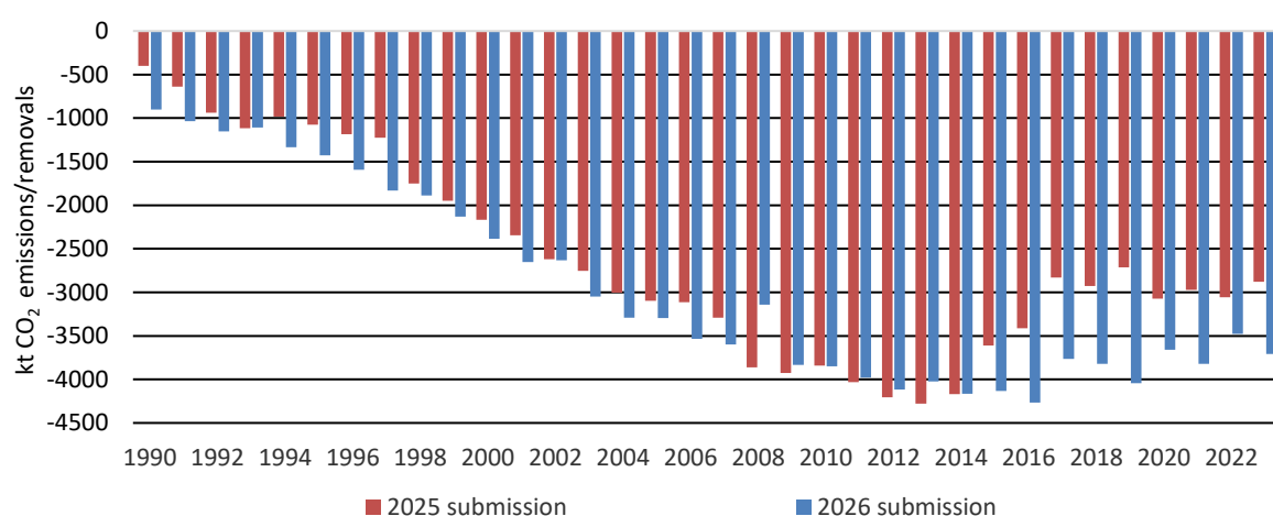
Figure 6.14 Comparison of category 4.A.2 emissions/removals for the 2025 and 2026 submissions
