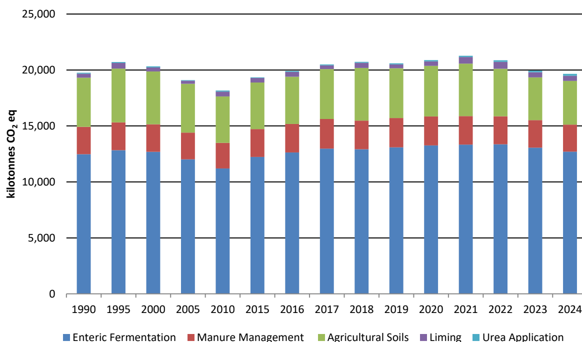
Figure 5.1 Total Emissions from Agriculture by Sector 1990-2024
