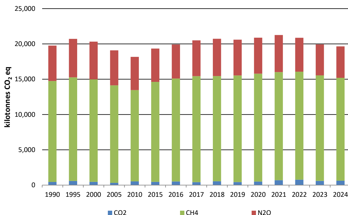
Figure 5.2 Total Emissions from Agriculture by Gas 1990-2024
