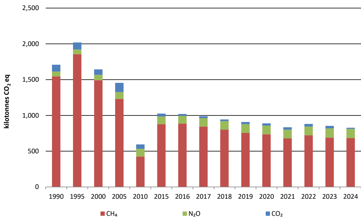
Figure 7.2 Total Emissions from Waste by Gas, 1990-2024
