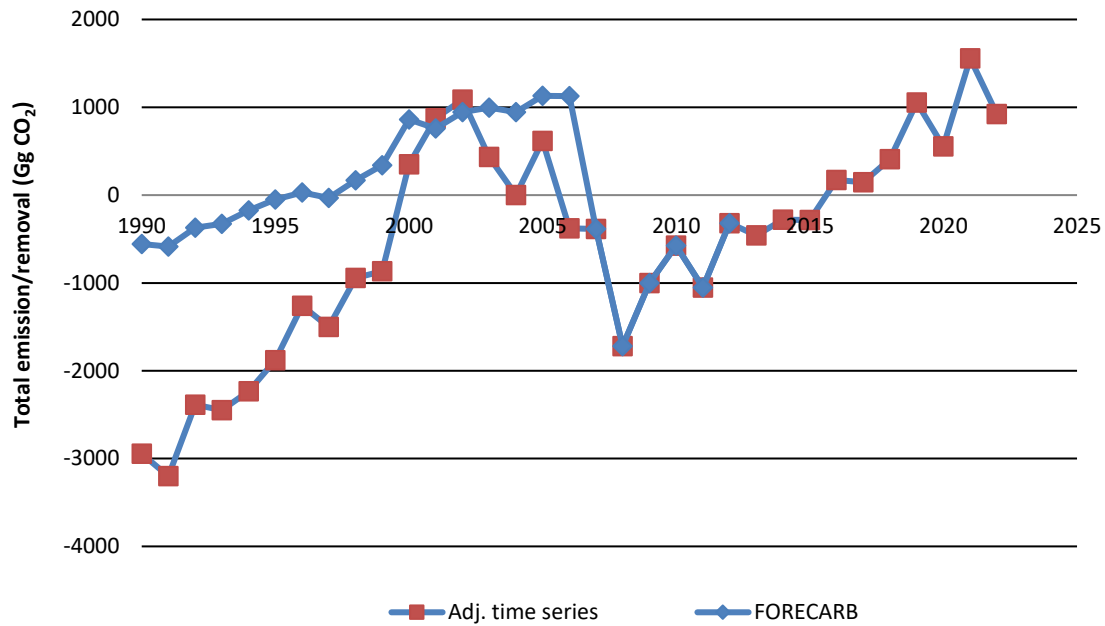
Figure 3.4.C.1-1 Adjusted time series for forest category afforested before 1990 (FM)
