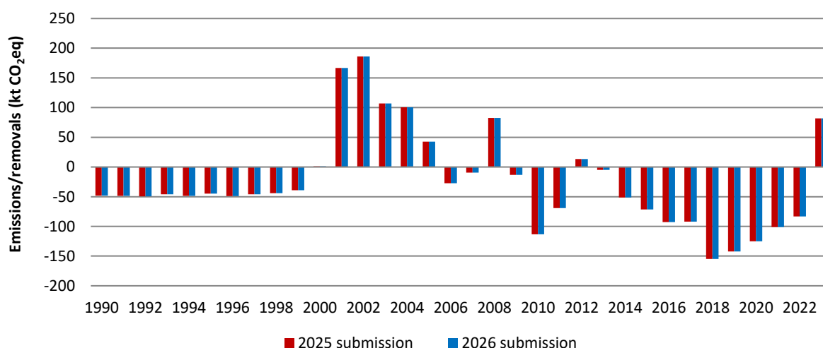
Figure 6.27 Comparison between the 2025 and 2026 submissions of estimated total emissions and removals associated with Cropland
