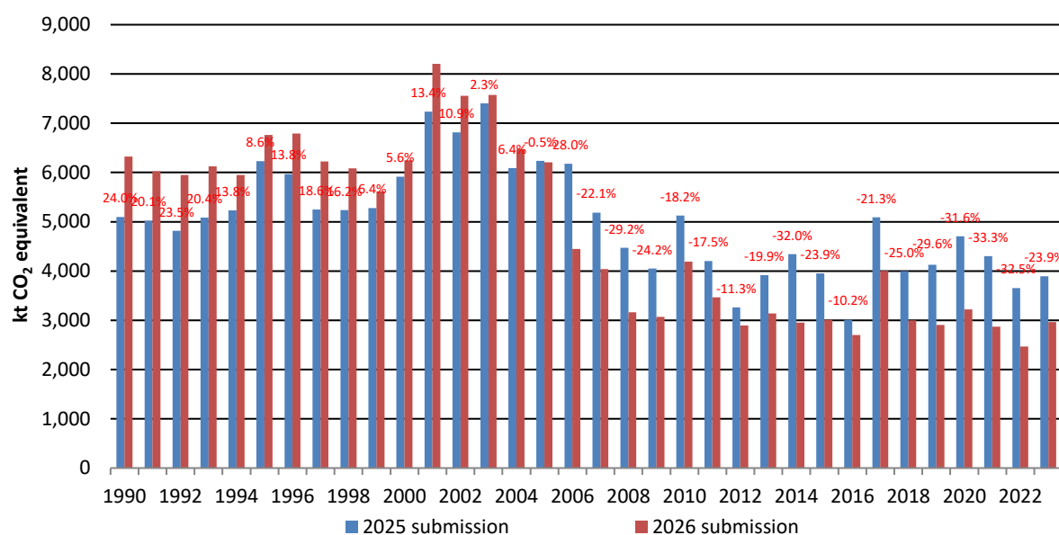
Figure 10.4 Impact of Recalculations in LULUCF between annual Submissions 1990-2023
