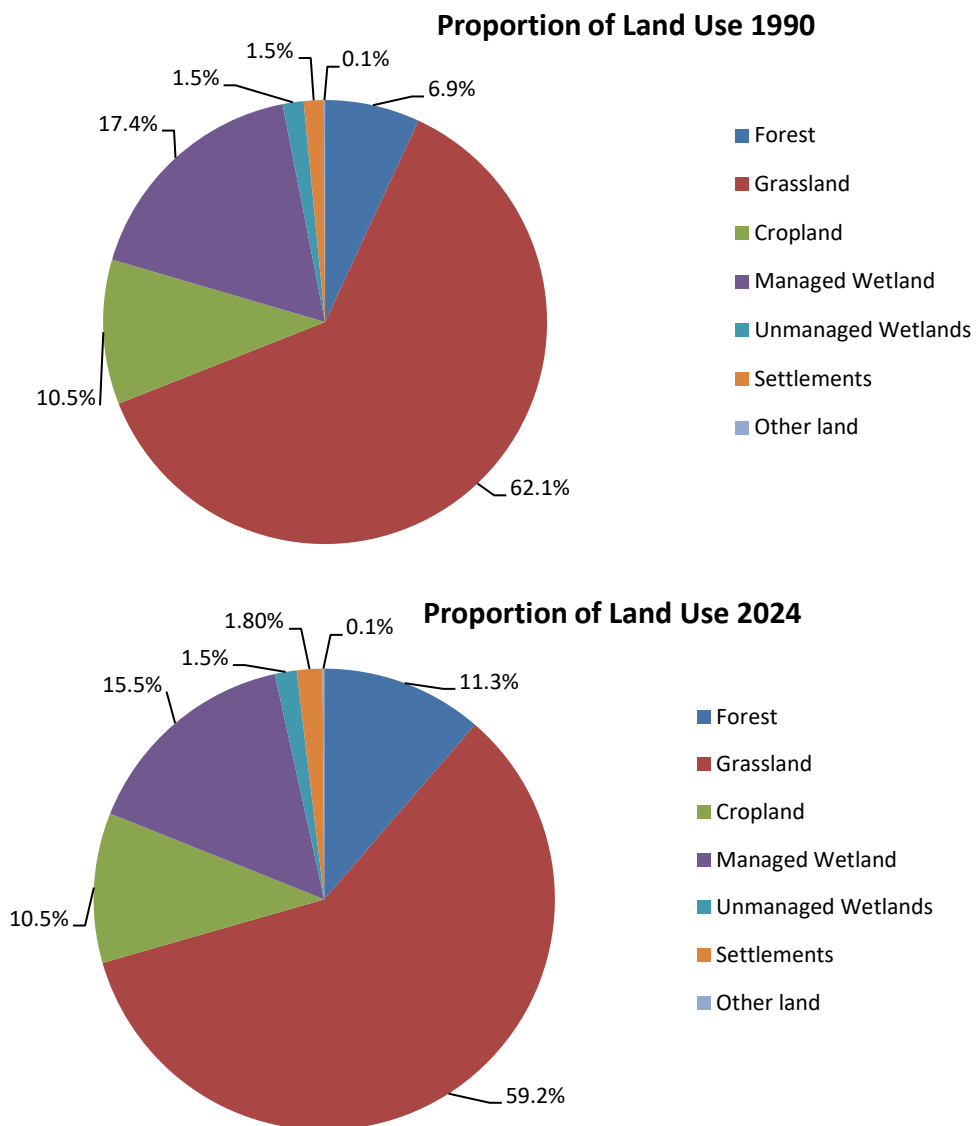
Figure 6.2 Overview of land use change between 1990 and 2024
