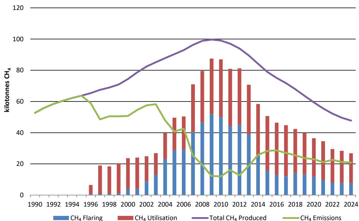
Figure 7.3 Methane Emissions from Solid Waste Disposal 1990-2024
