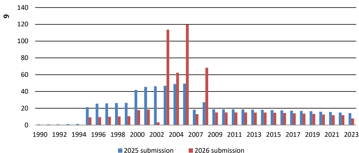
Figure 6.39 Comparison between the 2025 and 2026 submissions of estimated total emissions for Other Land
