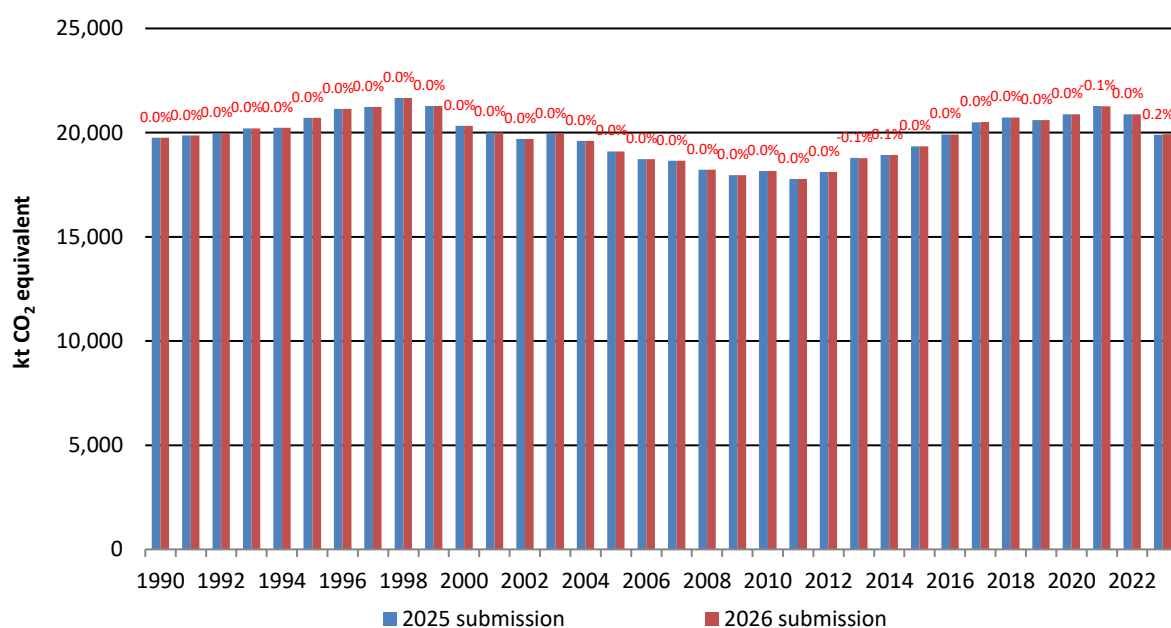
Figure 10.3 Impact of Recalculations in Agriculture between annual Submissions 1990-2023
