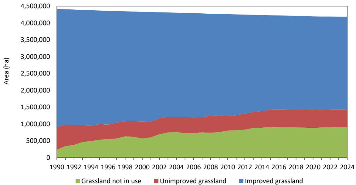
Figure 6.29 Trends in Grassland use 1990-2024
