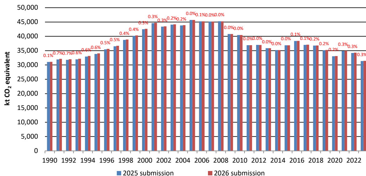
Figure 10.1 Impact of Recalculations in Energy between annual Submissions 1990-2023
