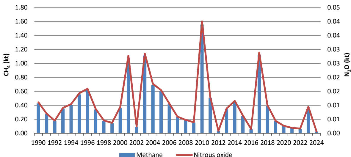
Figure 6.32 Estimated CH 4 and N 2 O emissions from biomass burning on Grassland
