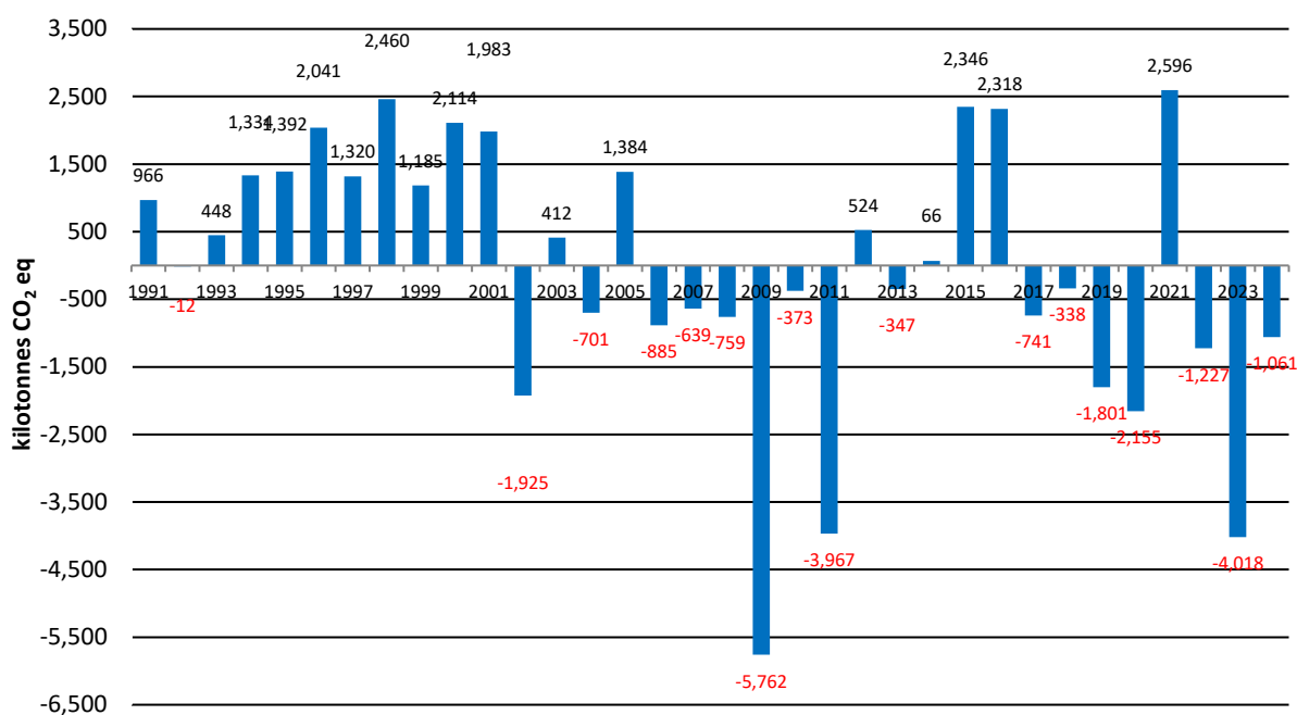
Figure 2.2 Inter annual changes
