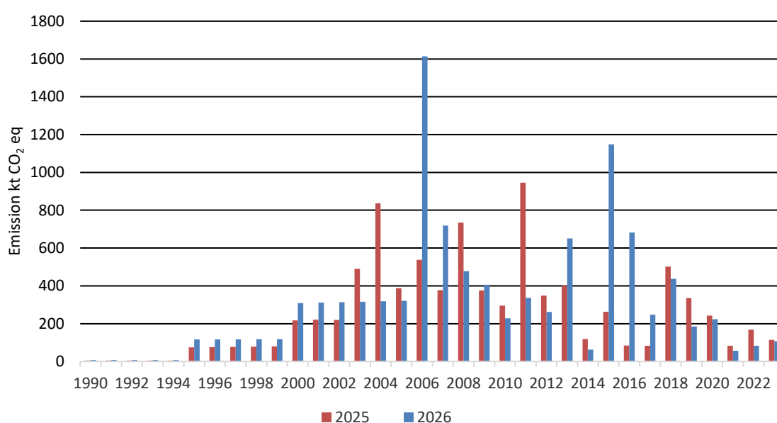
Figure 6.15 Comparison of deforestation emissions for the 2025 and 2026 submissions
