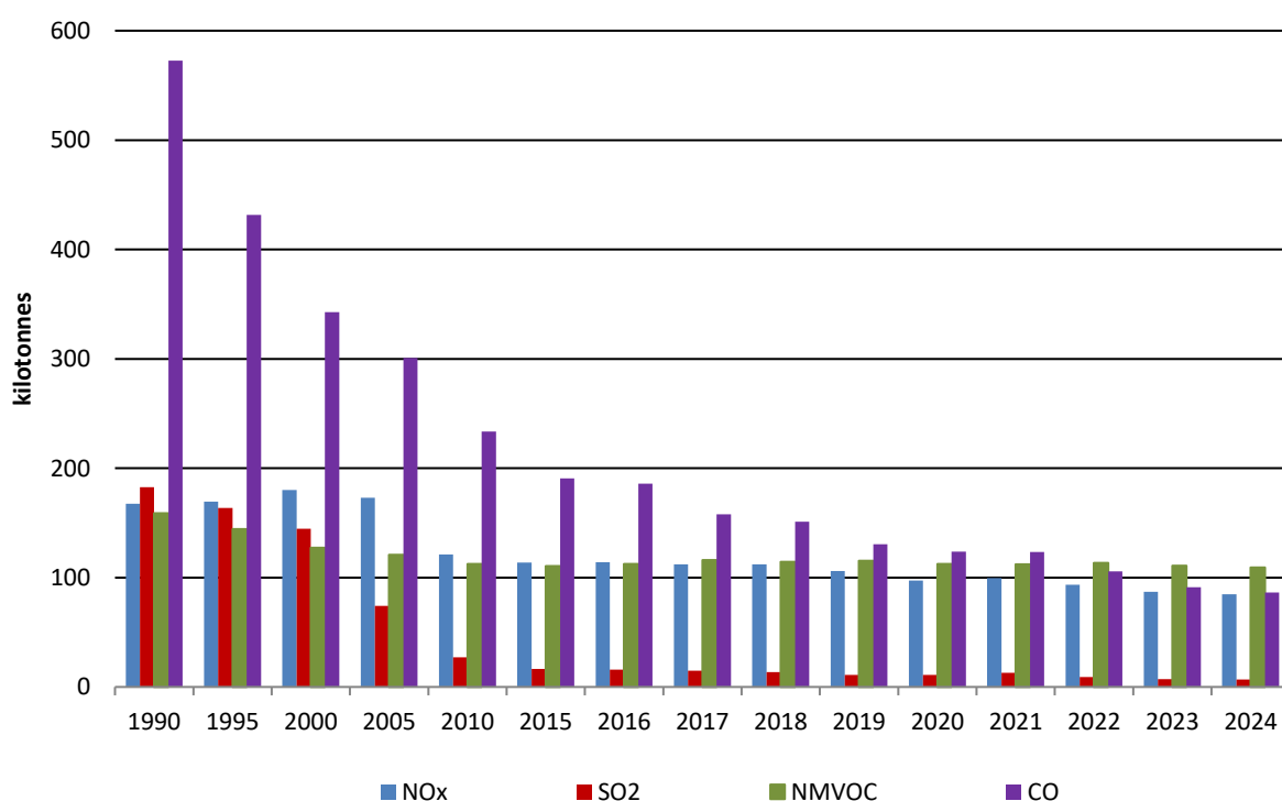
Figure 2.12 Trend in Indirect Greenhouse Gases 1990-2024
