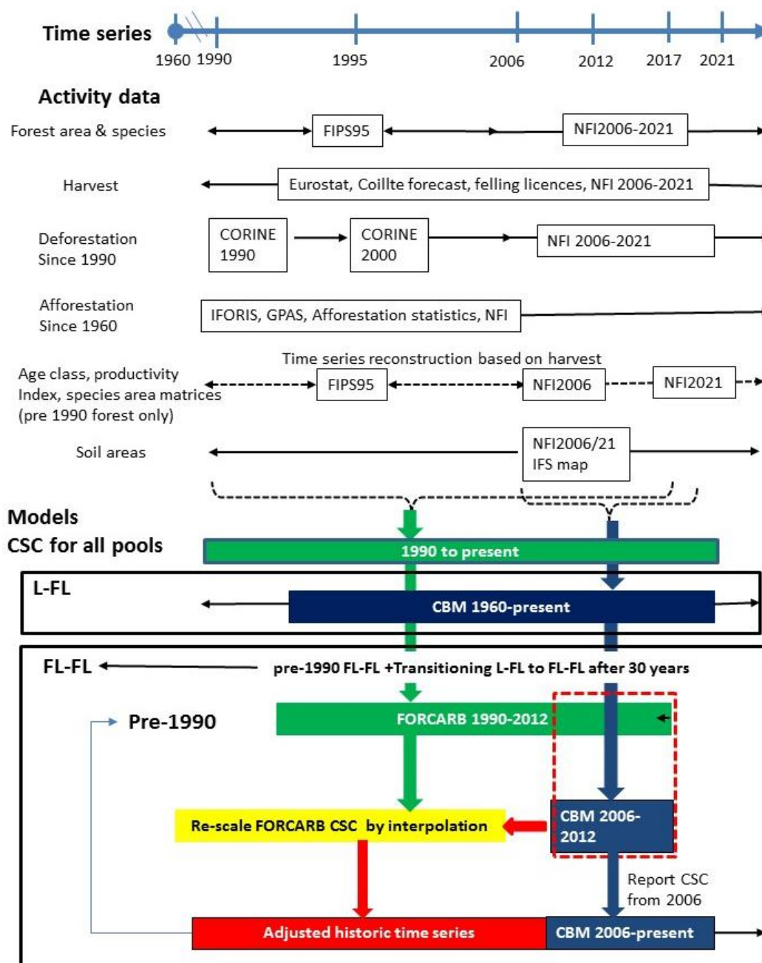
Figure 6.3 Activity data and models used to derive carbon stock changes for forest land
