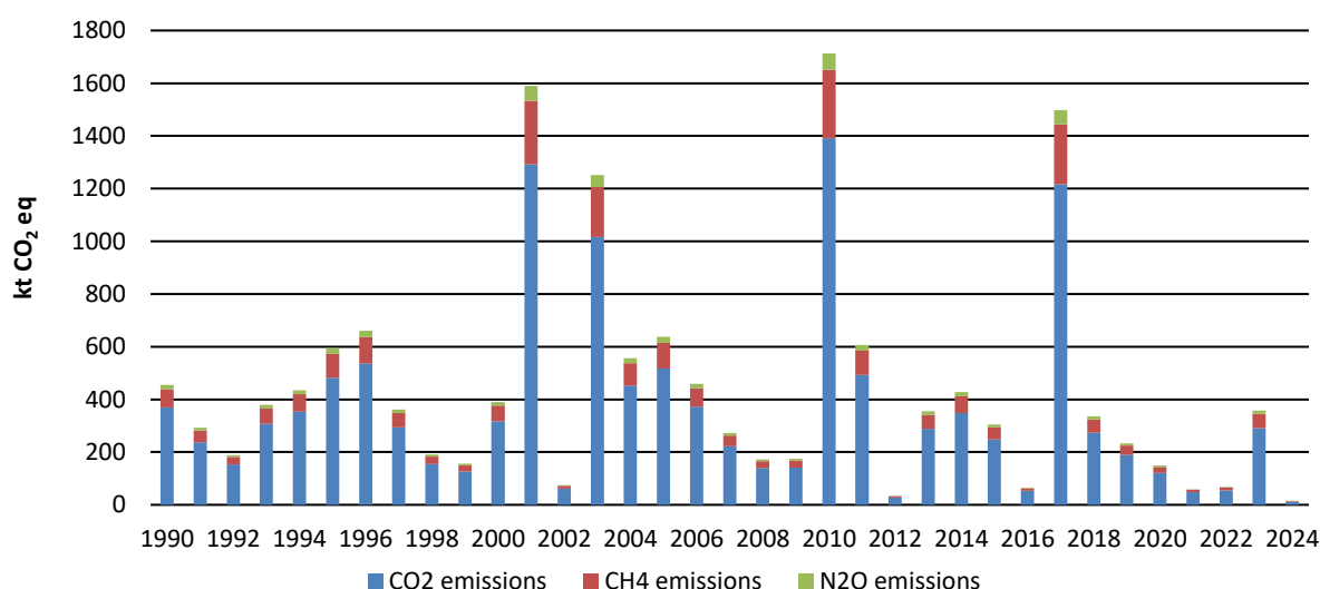
Figure 6.35 Estimate emissions (kt CO 2 eq) due to biomass burning on wetlands
