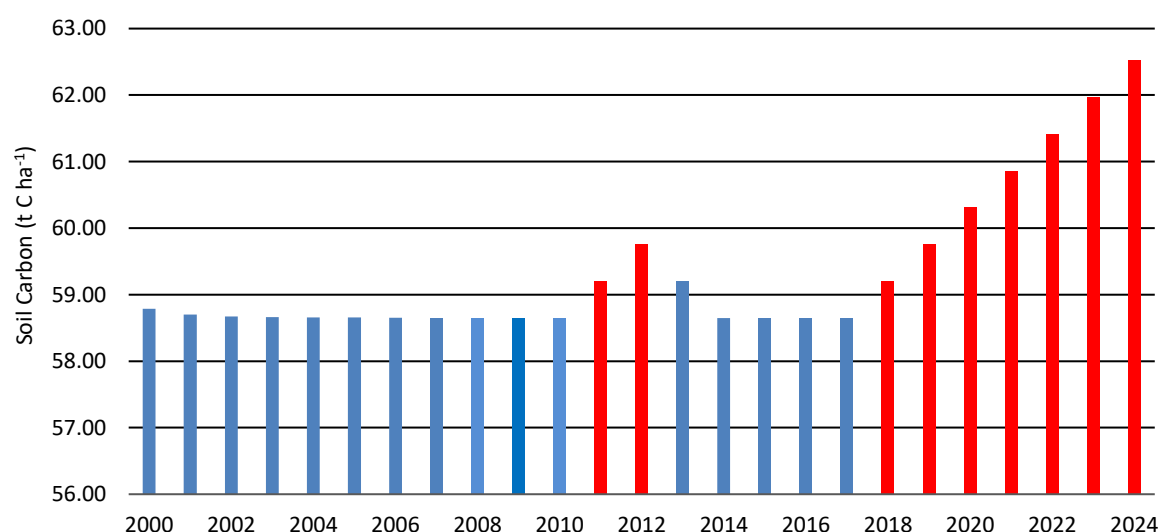
Figure 6.23 Estimated Soil Carbon per hectare based on the crop rotation pattern outlined in Table 6.30 for the period 2000-2024
