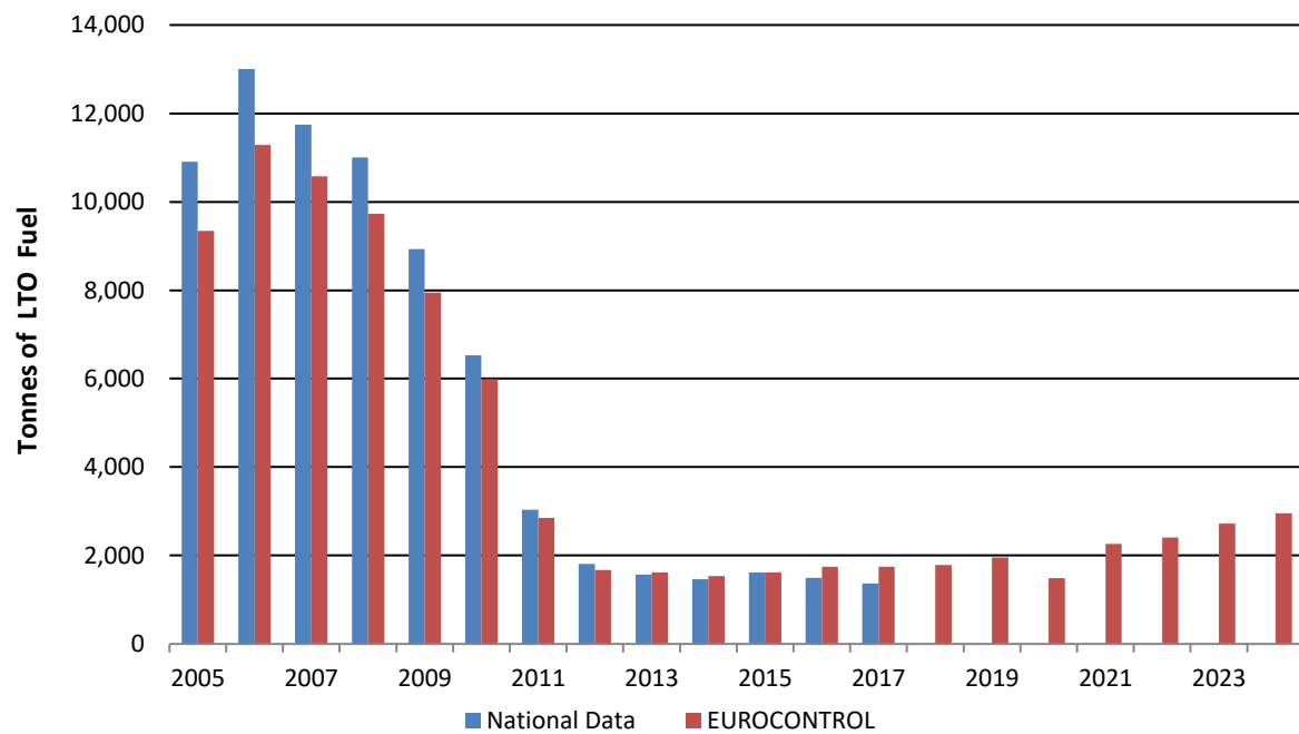
Figure 3.8 National LTO fuel data and EUROCONTROL LTO fuel data for 2005-2024
