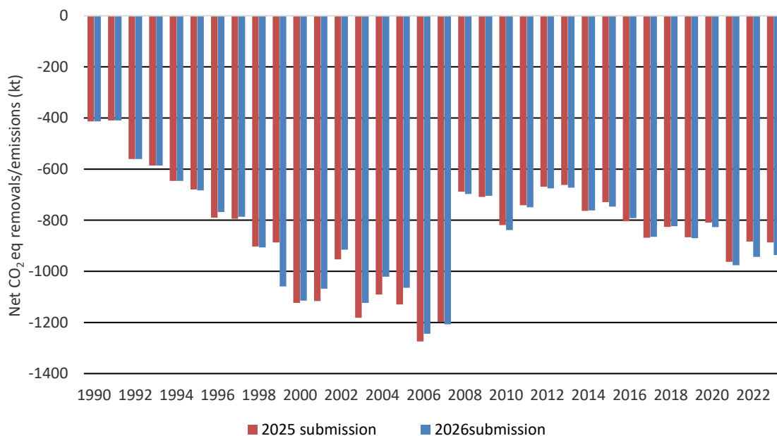
Figure 6.16 Comparison of HWP removals for the 2025 and 2026 submissions
