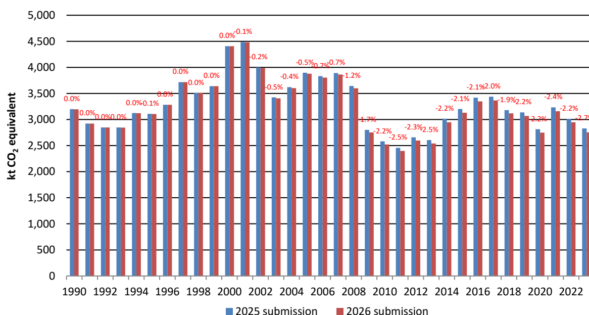
Figure 10.2 Impact of Recalculations in IPPU between annual Submissions 1990-2023
