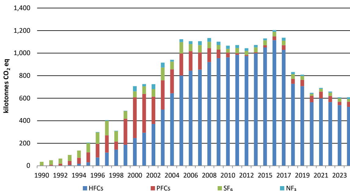
Figure 4.3 Emissions of HFC, PFC, SF 6 and NF 3 , 1990-2024
