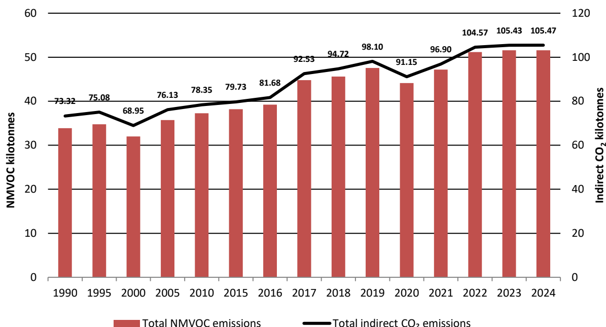
Figure 9.1 Total Indirect CO 2 emissions 1990-2024
