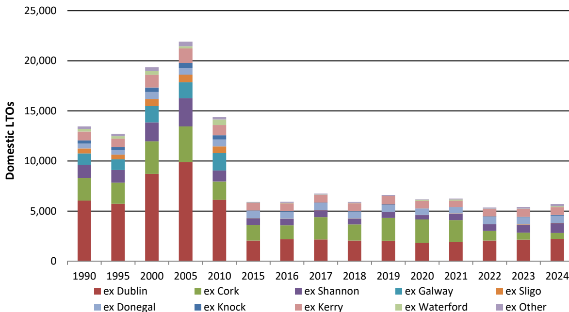
Figure 3.6 Number of LTOs from Irish airports 1990-2024
