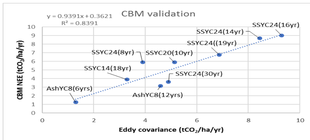
Figure 6.40 Validation of NEE estimated from CBM-CFS3 and eddy covariance data for different aged a Sitka spruce (SS) and Ash stands
