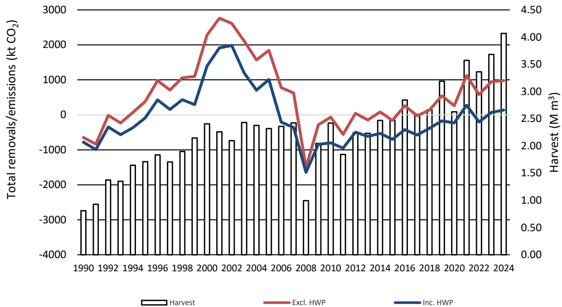
Figure 6.11 Time series of carbon stock changes (including and excluding Harvested Wood Products) and annual harvest rates for FL-FL, category 4.A.1.
