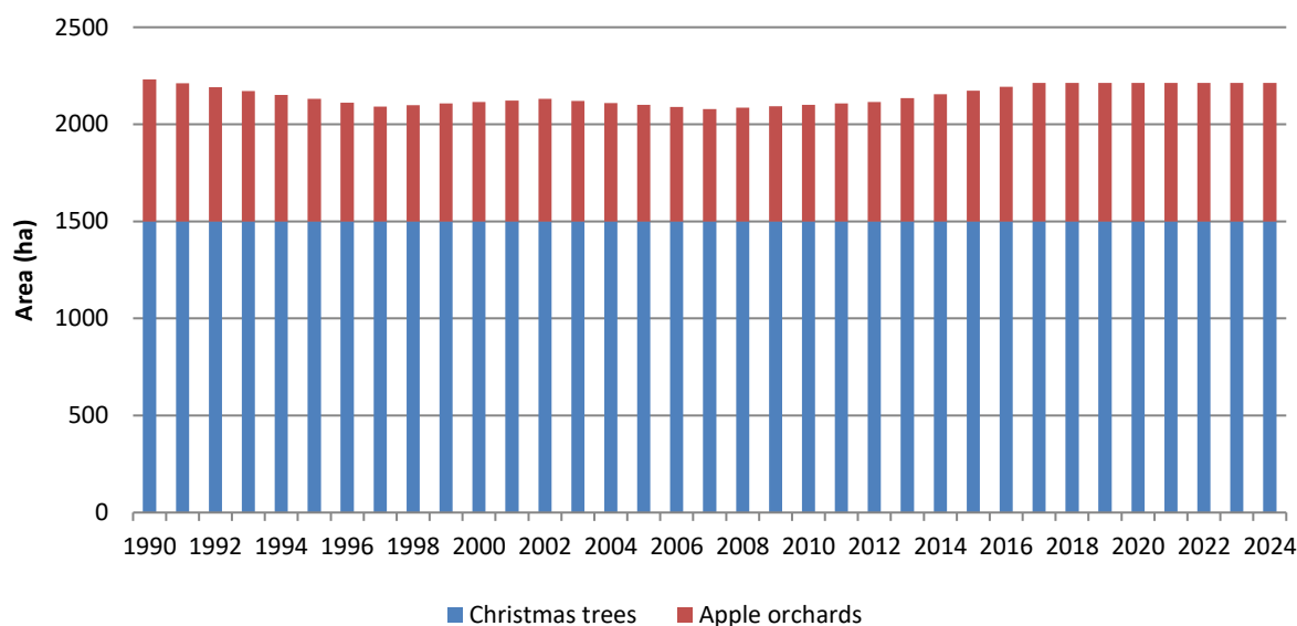
Figure 6.24 Estimated area under Perennial crops 1990-2024
