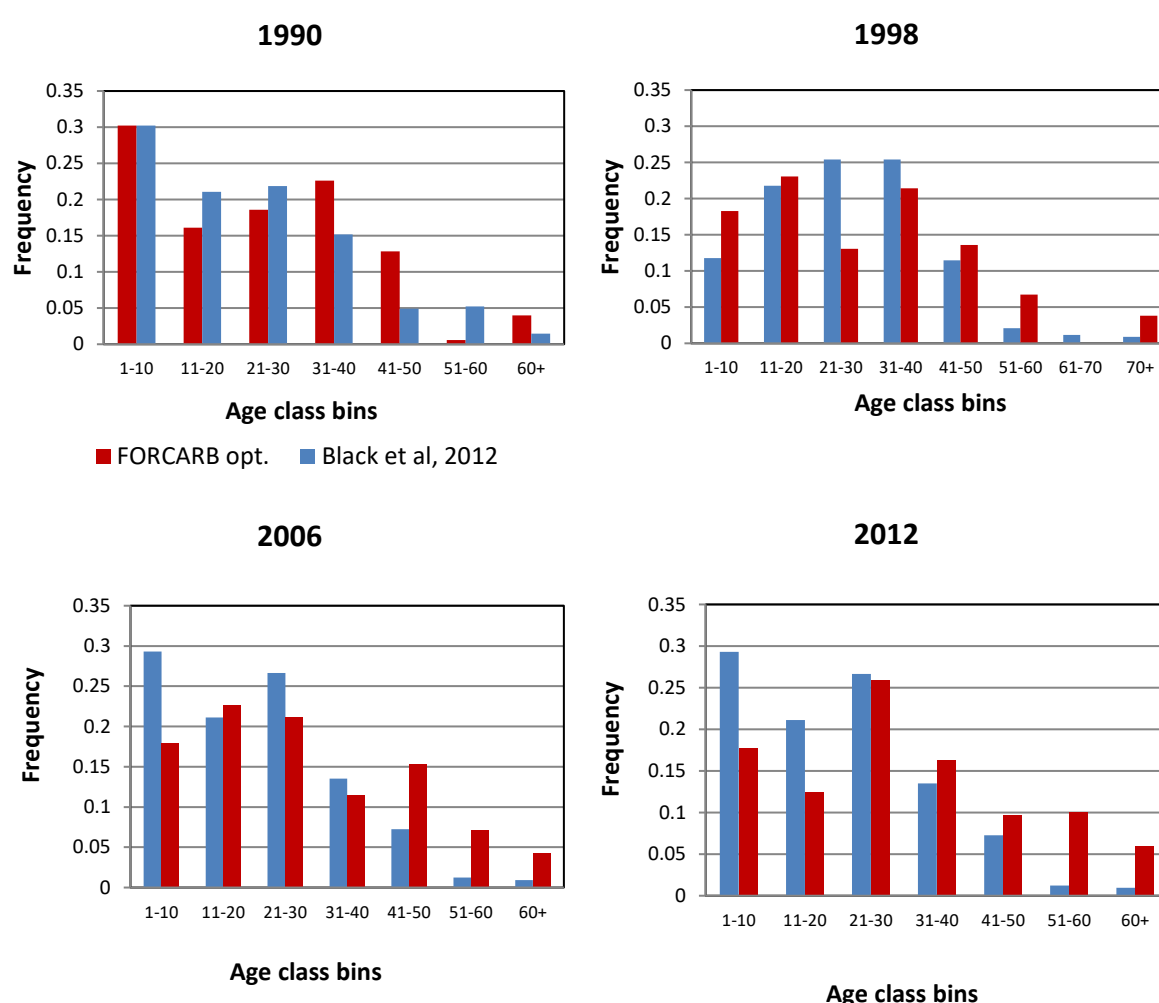
Figure 3.4.C-1 Validation of optimised age-class distributions
