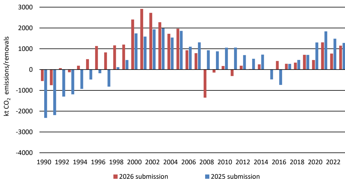
Figure 6.12 Comparison of category 4.A.1 emissions/removals for 2025 and 2026 submissions
