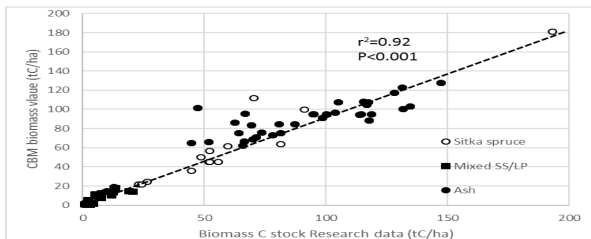
Figure 6.41 Validation of total biomass estimates from CBM-CFS3 and research data plots for different aged Sitka spruce, mixed Sitka spruce and Lodgepole pine (SS/LP) and Ash stands.
