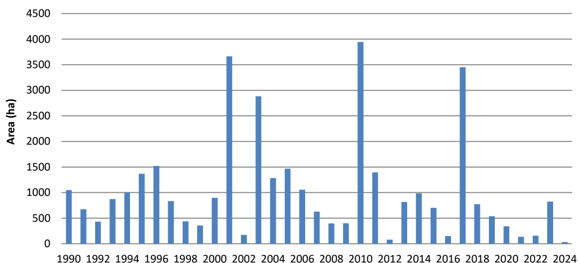
Figure 6.34 Estimate of the area of wetland subject to biomass burning
