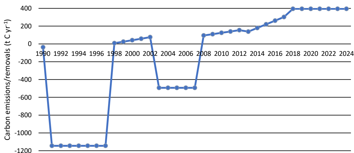
Figure 6.25 Carbon Stock Change in Biomass in Perennial Crops
