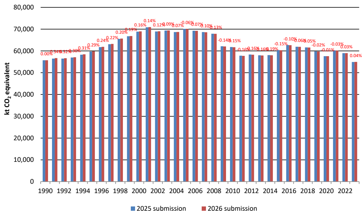
Figure 10.6 Total Impact of Recalculations between annual Submissions (without LULUCF) 1990-2023
