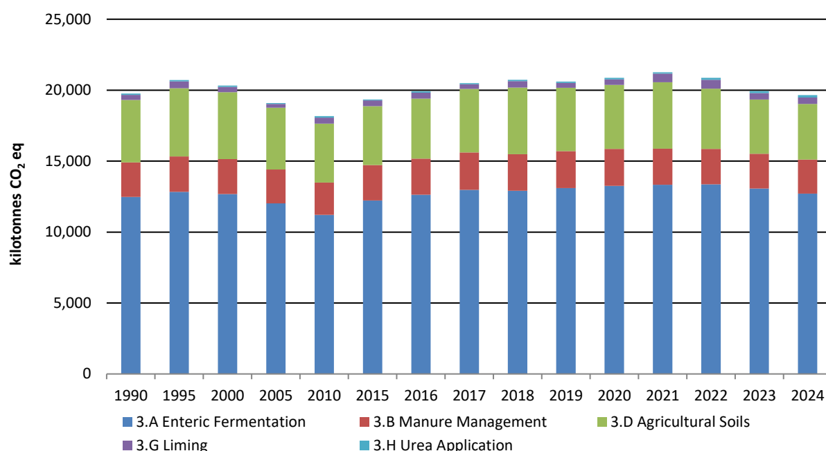
Figure 2.9 Trend in Emissions from Agriculture 1990-2024
