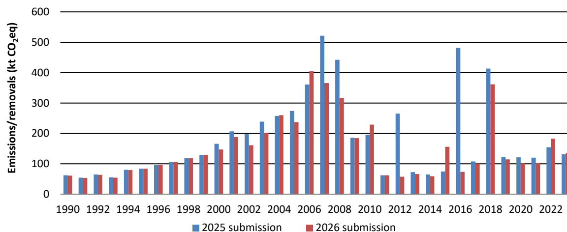
Figure 6.38 Comparison between the 2025 and 2026 submissions of estimated total emissions associated with Settlements
