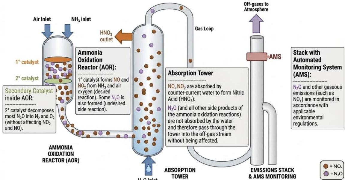
Figure 1. Project Activity boundary for an Article 6.4 activity with secondary N 2 O abatement only
