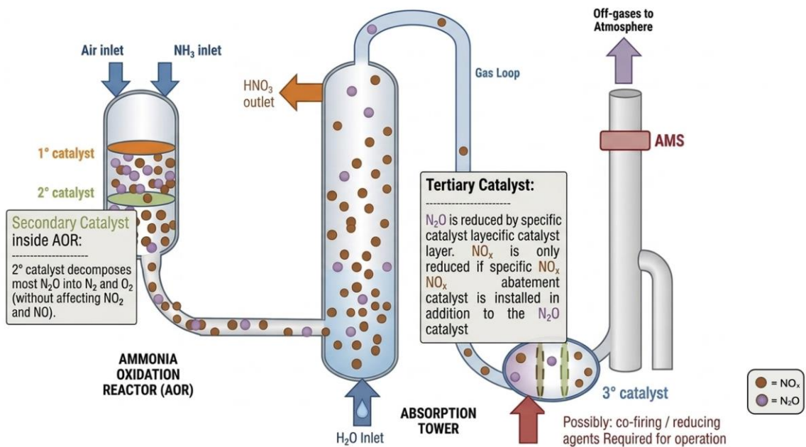
Figure 3. Project Activity boundary for an Article 6.4 activity with a combination of secondary and tertiary N 2 O abatement
