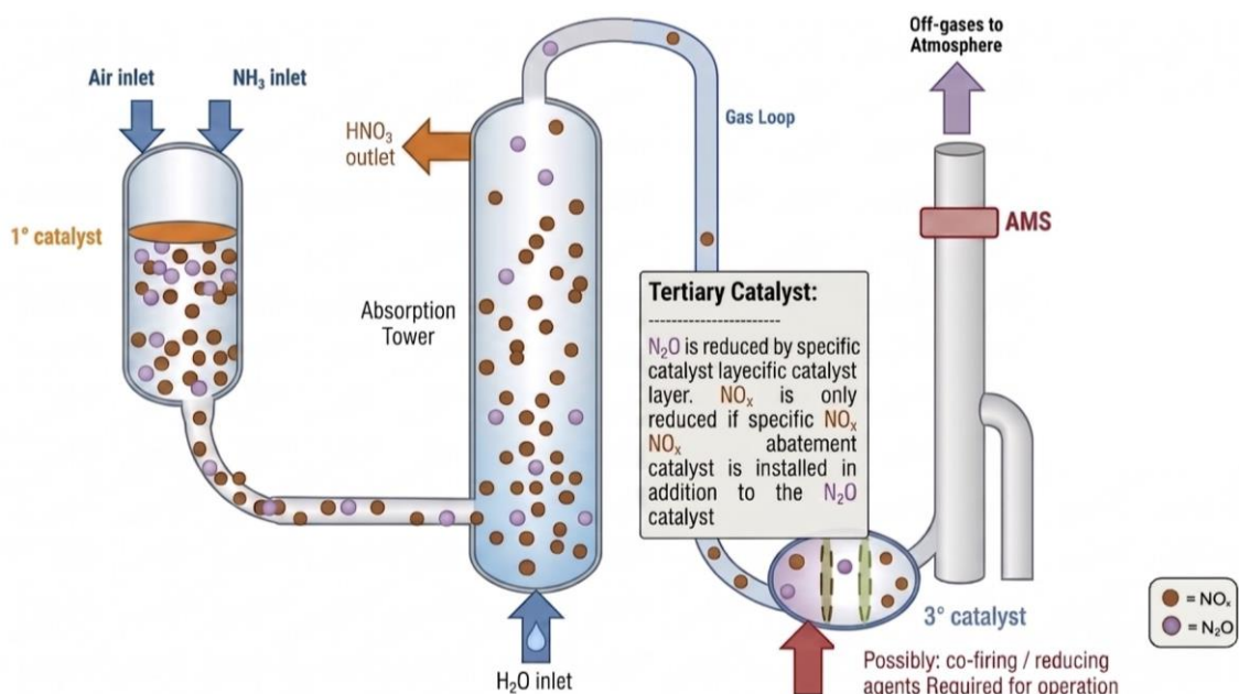
Figure 2. Project Activity boundary for an Article 6.4 activity with tertiary N 2 O abatement only
