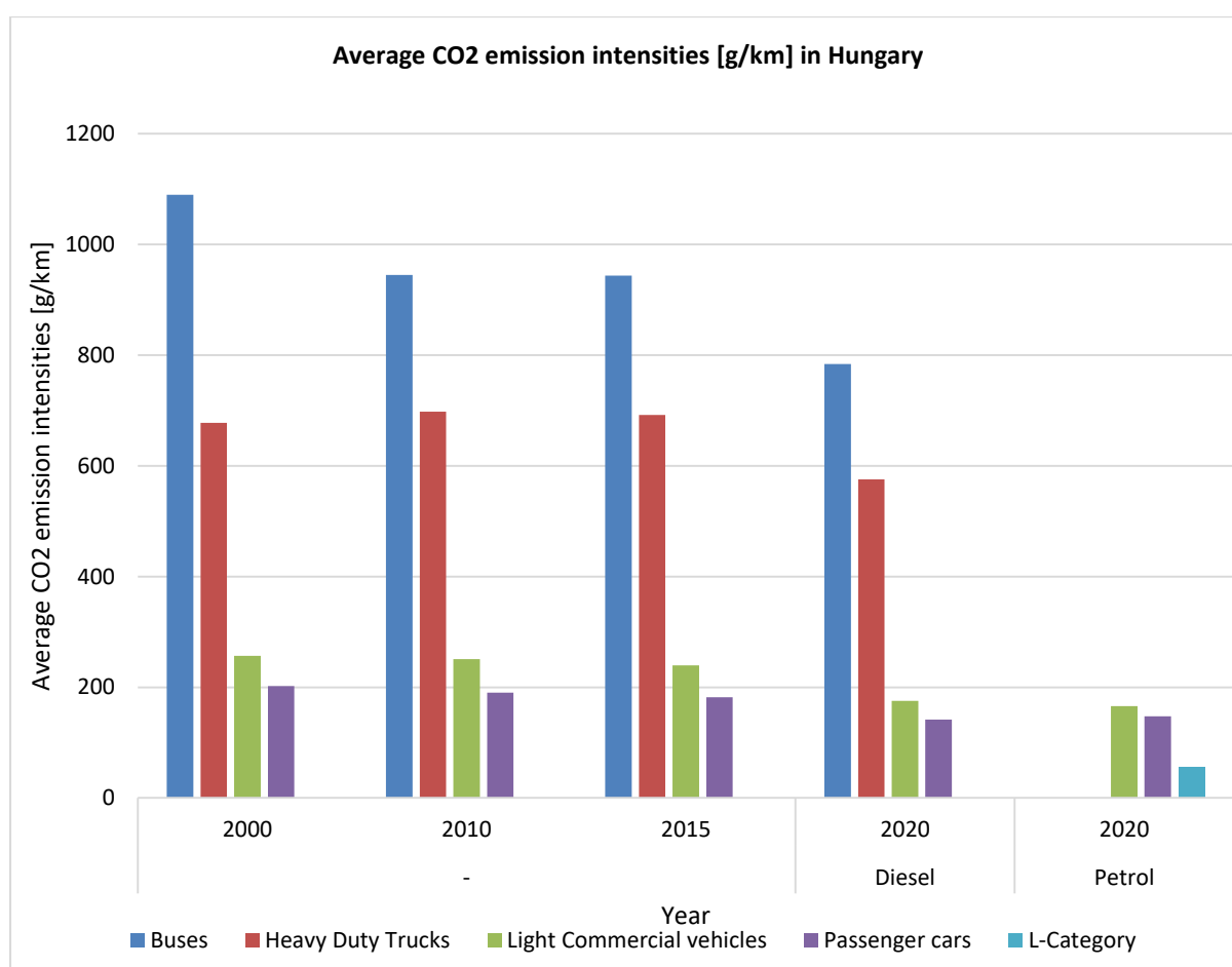
Figure 2.26. Average CO 2 emission intensities (g/km) in 2000, 2010, 2015 and 2020
