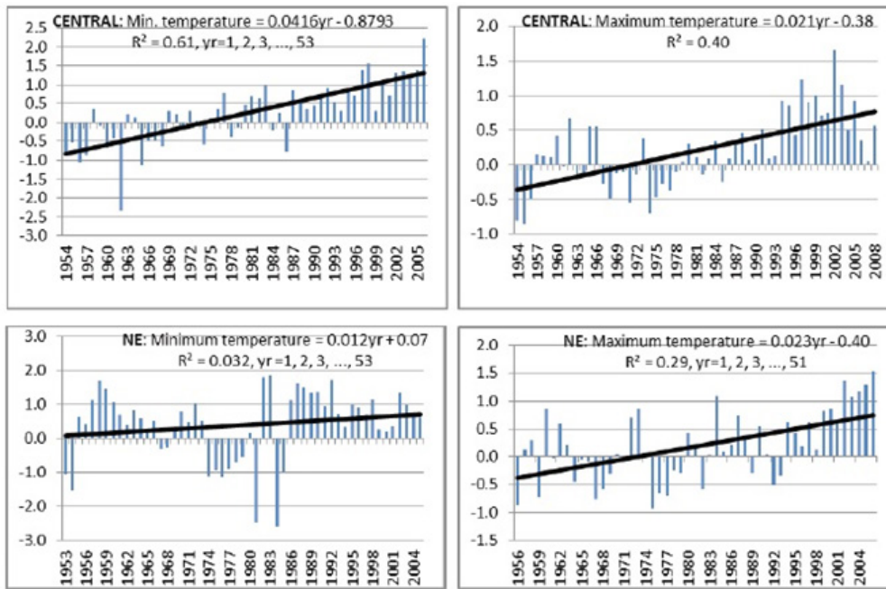
Figure 10. Inter-annual variation of the mean minimum (Left) and maximum temperature (Right) for Central Ethiopia (Top Row) and North Eastern Ethiopia (Bottom Row)
