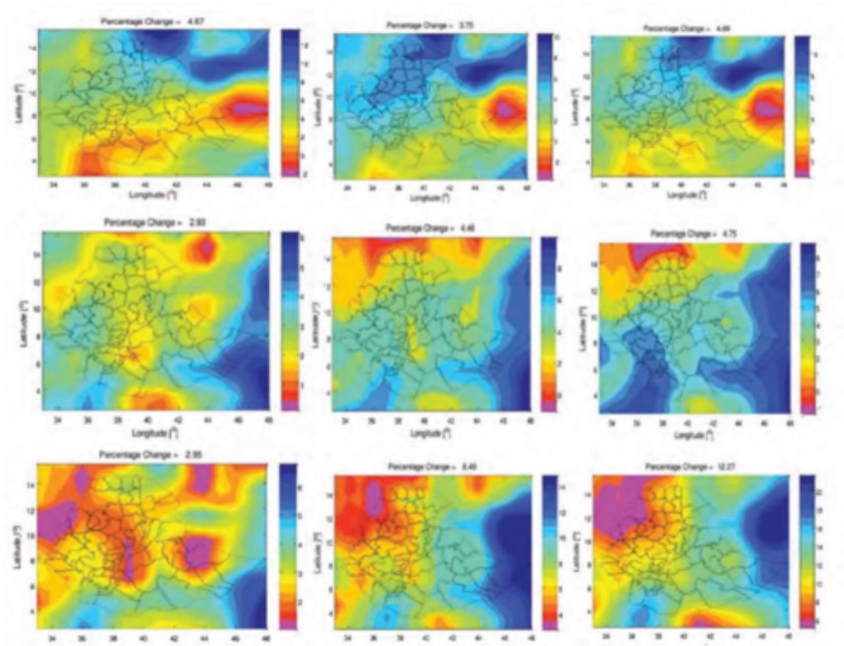
Figure 7. Percentage change in rainfall over Ethiopia under 3 regional climate scenarios for three future time periods relative to the baseline period (1975-2005) and mean rainfall for the three regional climate scenarios
