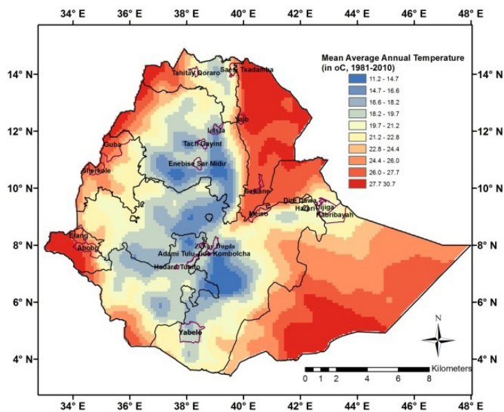
Figure 9. Mean annual surface temperature in °C
