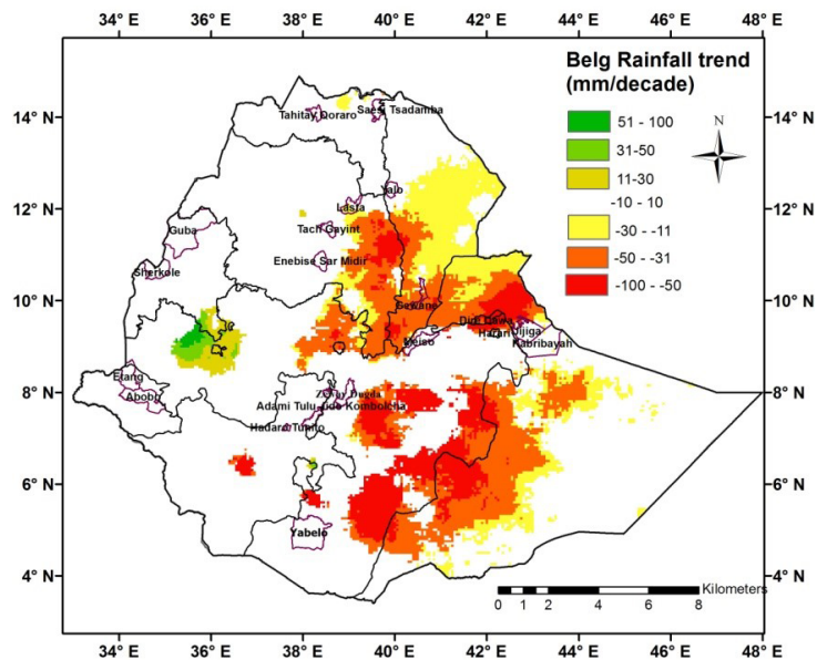
Figure 5. Rainfall trend over Ethiopia (1981-2014)
