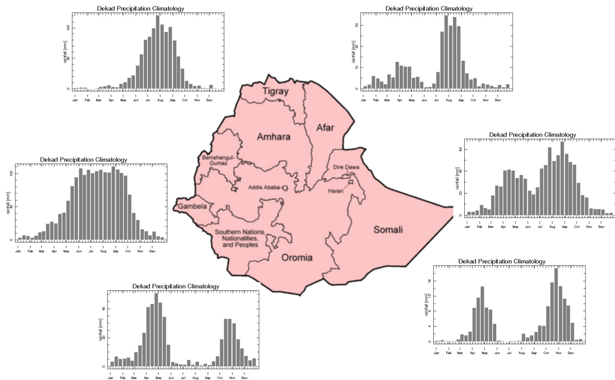
Figure 1. Rainfall regime of Ethiopia showing sample Woredas to demonstrate the rainfall regimes
