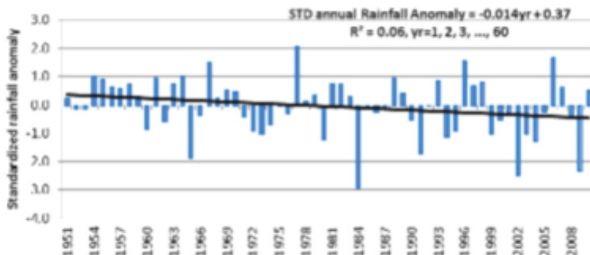
Figure 4. Standardized annual rainfall anomaly - 1951-2010 in relation to 1961-1990 average
