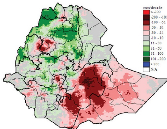
Figure 6. Change in average rainfall over the March-September season, comparing averages for 1997-2013 with 1981-1996
