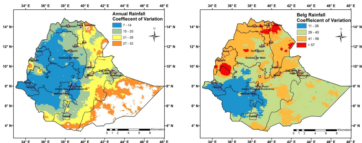
Figure 3. Annual and Belg rainfall coefficient of variation
