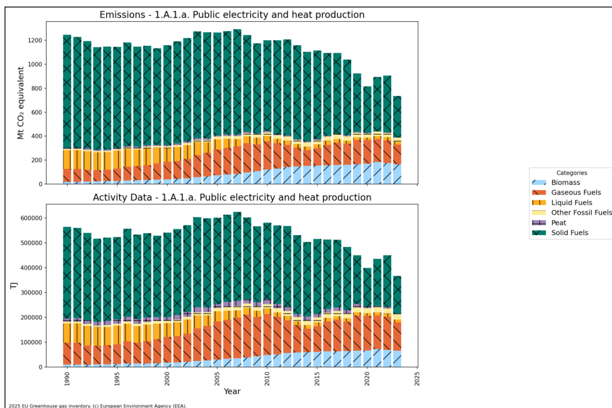
Figure 3.13 1.A.1.a Public Electricity and Heat Production: Total emission and activity data trends
