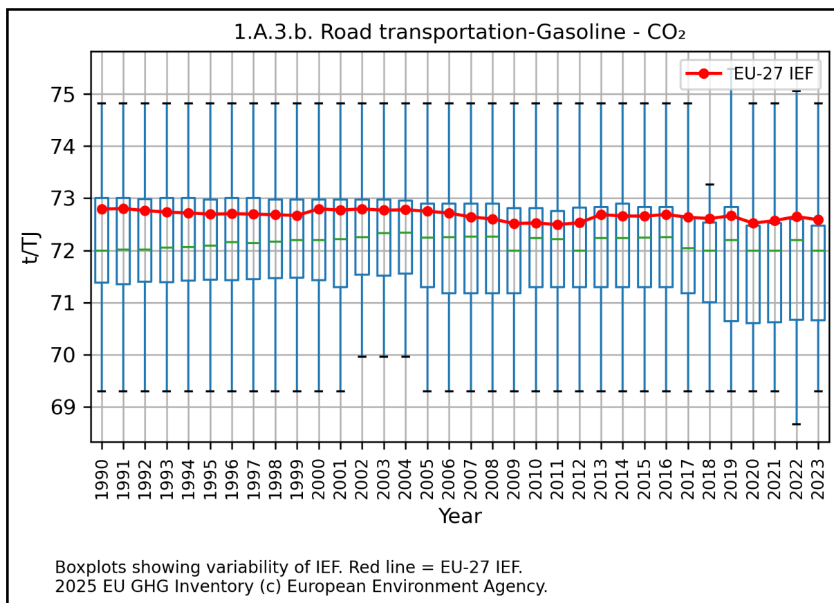
Figure 3.98 1A3b Road Transportation – Gasoline: CO 2 Implied Emission Factor (IEF) in EU (in t/TJ)
