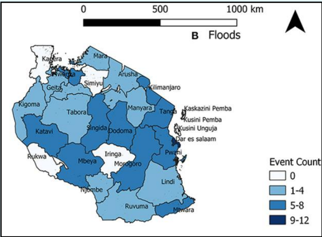
Figure 1:Distribution of flood events in Tanzania (2000–2019) (Msemo et al, 2021)
