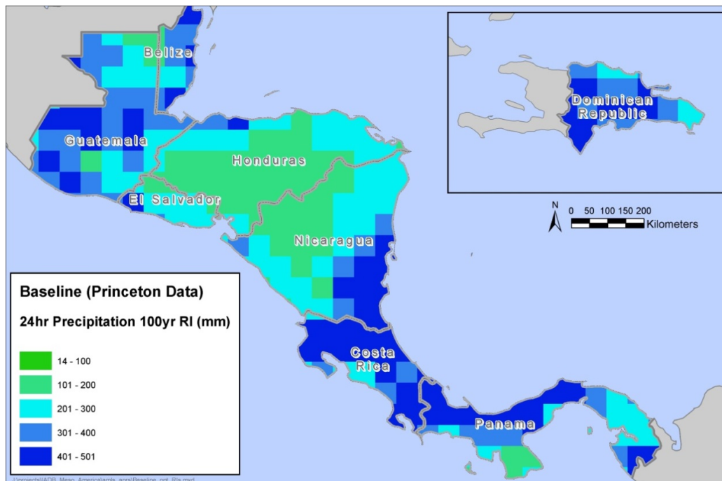
Figure 4-2 Gridded observed precipitation data from Princeton dataset based on 1948–2008 data
