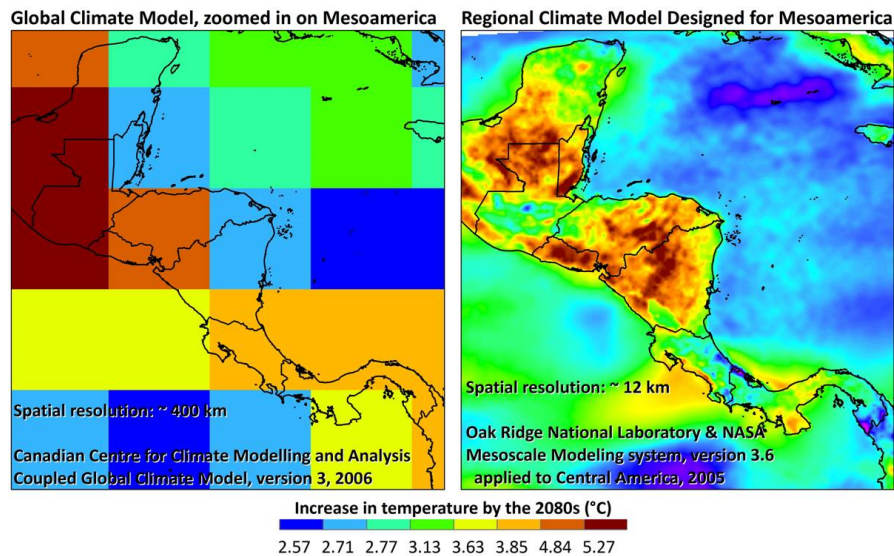
Figure 4-4 The issue of spatial resolution: Global versus regional analysis
