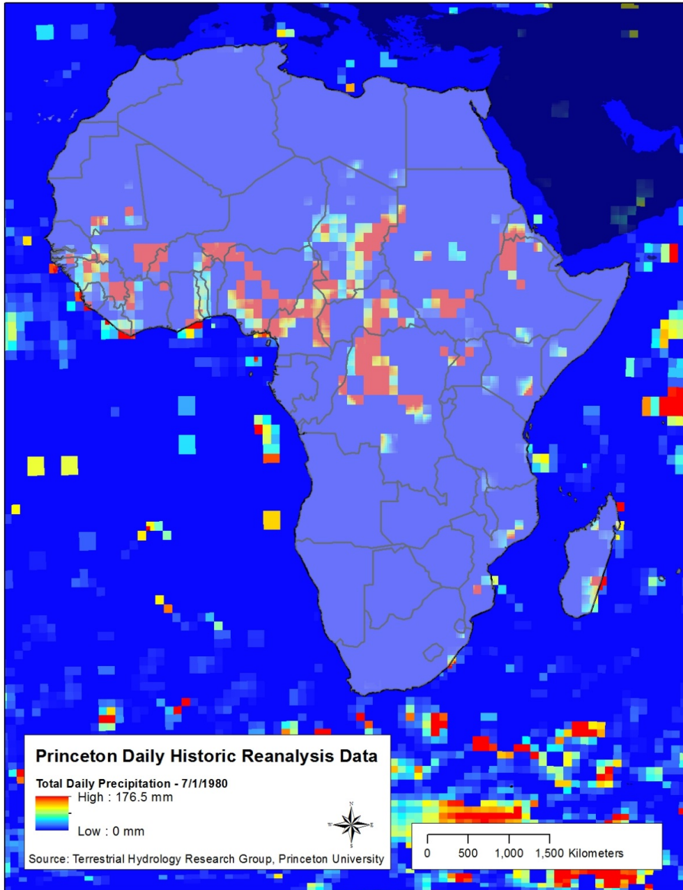
Figure 4-3 Gridded observed precipitation data from Princeton dataset
