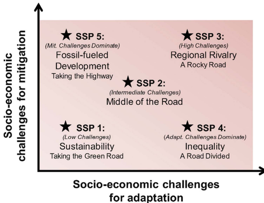
Figure 3-1 Five shared socioeconomic pathways
