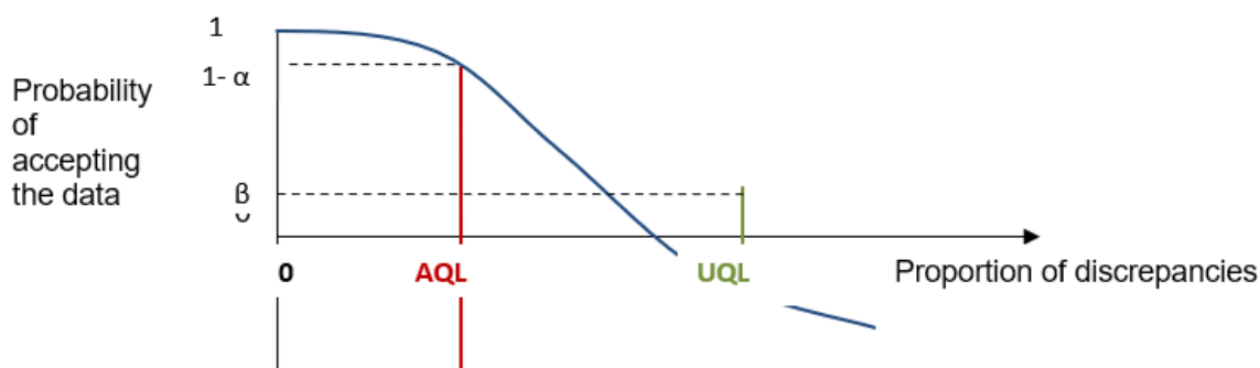
Figure. Acceptance sampling operating characteristic curve
