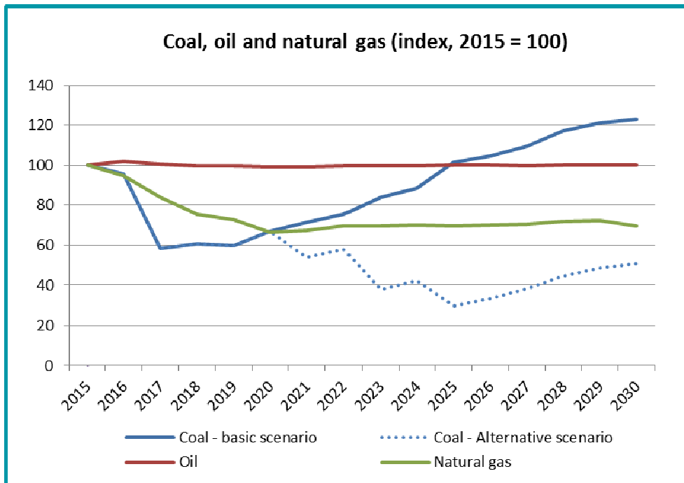
FIGURE 5.8 COAL, OIL AND NATURAL GAS (INDEX, 2015 = 100) 2015-2030, 2015 IS OBSERVED Source: Danish Energy Agency
