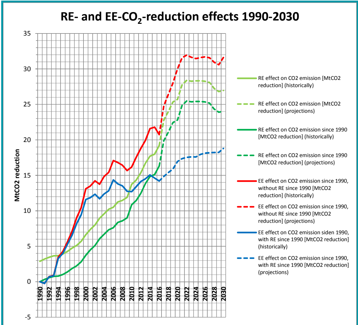
FIGURE B4.1: TOTAL EFFECT OF THE GROUP OF POLICIES AND MEASURES THAT PROMOTE THE USE OF RENEWABLE ENERGY (RE-PAMs) AND OF THE TOTAL EFFECT OF THE GROUP OF POLICIES AND MEASURES THAT PROMOTE ENERGY EFFICIENCY (EE-PAMs) - 1990-2016 EX-POST ESTIMATES BASED ON ENERGY STATISTICS AND 2017-2030 EX-ANTE ESTIMATES BASED ON THE 2017 ENERGY PROJECTION
