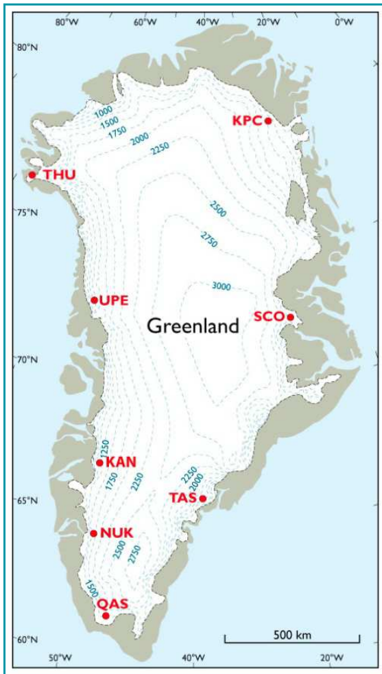
FIGURE 8.1 LOCATION AND IDENTIFICATION CODES OF PROMICE AUTOMATIC WEATHER STATIONS. DOTTED LINES ARE ELEVATION CONTOURS IN M ABOVE SEA LEVEL. Source: Geological Survey of Denmark and Greenland
