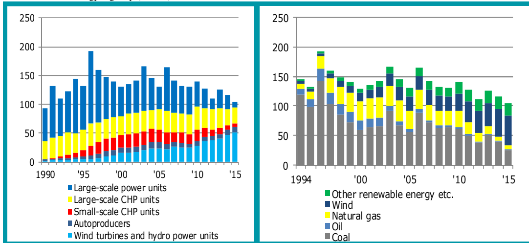
FIGURE 2.8 ELECTRICITY PRODUCTION BY TYPE OF PRODUCER AND BY FUEL, PJ Source: Danish Energy Agency (E2015)
