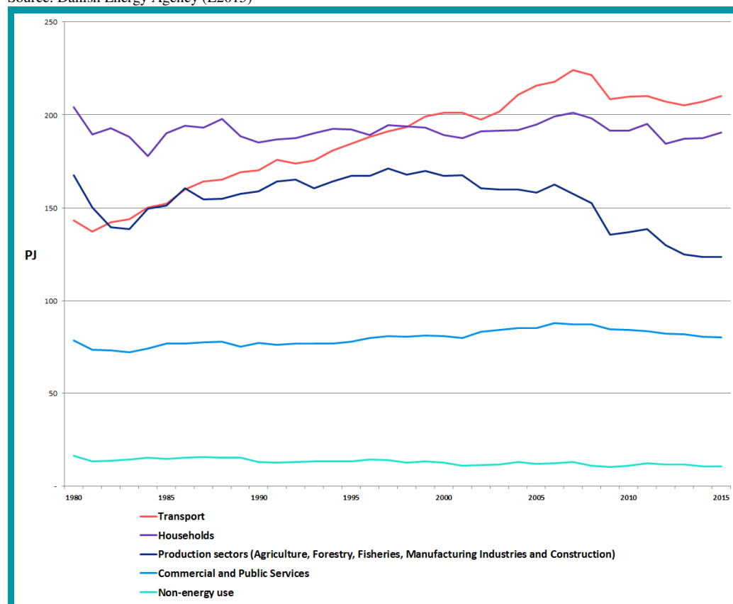
FIGURE 2.6 ADJUSTED GROSS ENERGY CONSUMPTION, BREAKDOWN BY SECTOR
