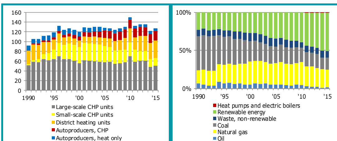
FIGURE 2.10 DISTRICT HEATING PRODUCTION BY TYPE OF PRODUCER [PJ] AND BY FUEL [SHARE IN %] Source: Danish Energy Agency (E2015)
