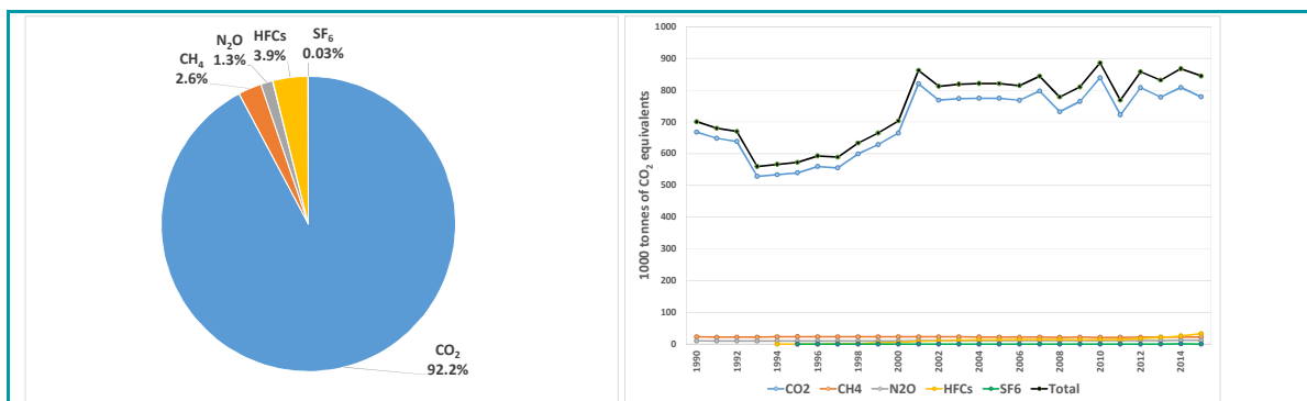
FIGURE VII.C.2 EMISSIONS OF GHG BY GAS IN 2015 AND DEVELOPMENT 1990-2015.
