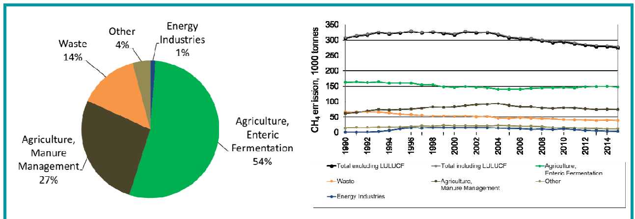
FIGURE 3.2 CH 4 EMISSIONS BY SECTOR (2015) AND DEVELOPMENT IN 1990-2015
