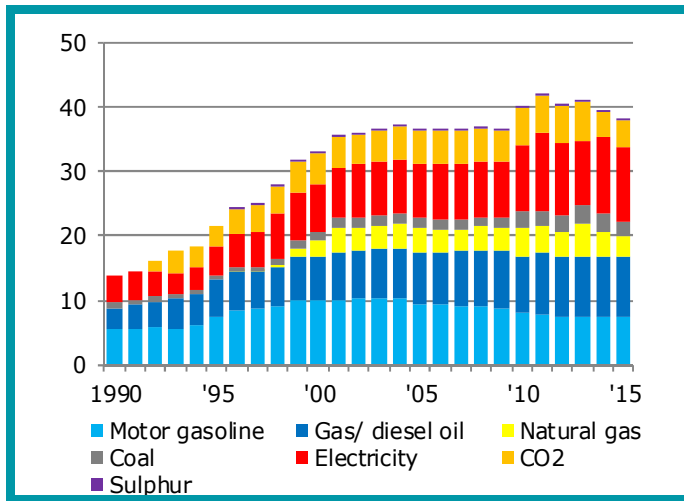
FIGURE 2.12 REVENUES FROM ENERGY, CO 2 AND SULPHUR TAXES. CURRENT PRICES IN BILLION DKK Source: Danish Energy Agency (E2015) and Statistics Denmark
