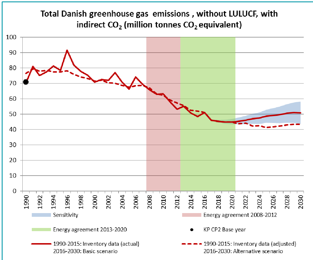
FIGURE 5.1 TOTAL DANISH GREENHOUSE GAS EMISSIONS, WITHOUT LULUCF, WITH INDIRECT CO 2 IN THE BASIC SCENARIO (WEM) AND THE ALTERNATIVE SCENARIO UNTIL 2030, 1990-2015 ARE INVENTORY DATA WITHOUT AND WITH ADJUSTMENTS FOR INTERANNUAL VARIATIONS IN ELECTRICITY TRADE AND TEMPERATURE
