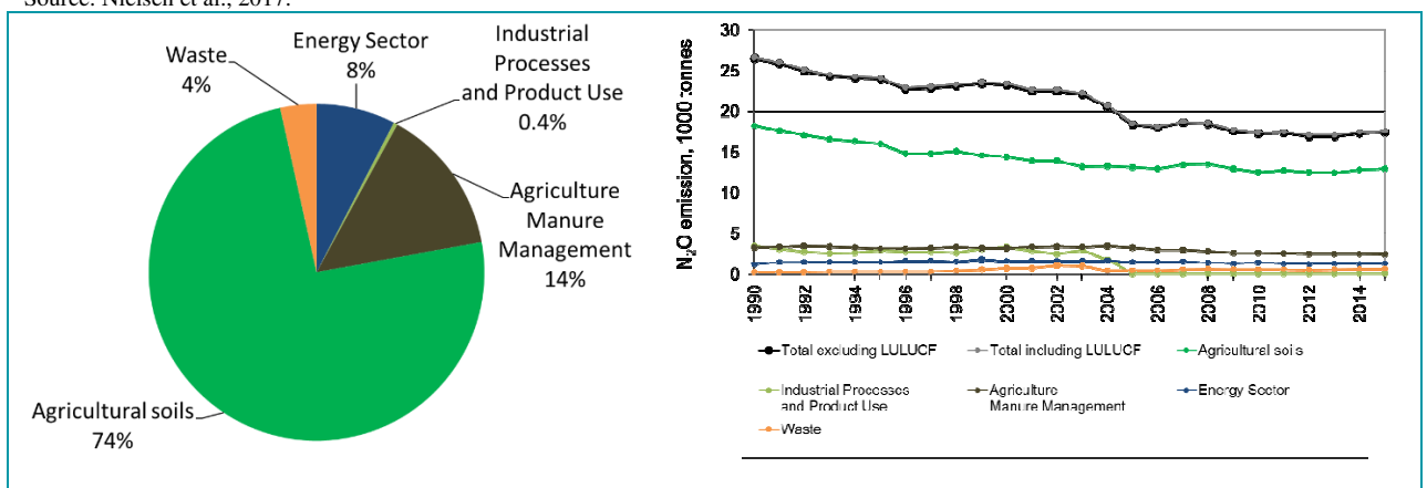
FIGURE II.3 N 2 O EMISSIONS BY SECTOR AND DEVELOPMENT IN 1990-2015 IN KT N 2 O Source: Nielsen et al., 2017.
