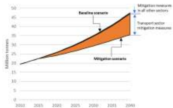
Figure ES.1: GHG emission trajectories, with and without GHG mitigation
