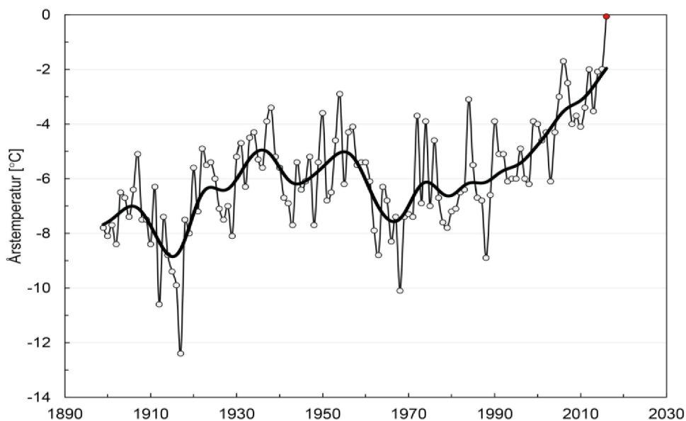
Figure 6.6 Annual mean temperatures for Svalbard Airport (Longyearbyen) during 1898-2016. The bold black curve illustrates smoothed variations on a decadal scale
