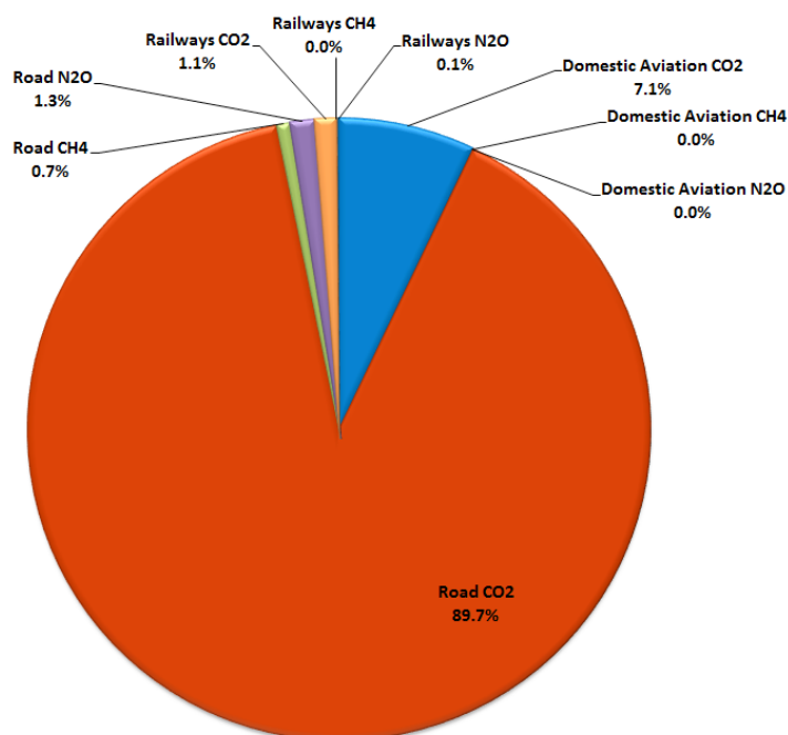
Figure 3.9: Sector I Energy: Percentage contribution of CO 2 , CH 4 and N 2 O from the transport sector, average over 2000 – 2012 period.
