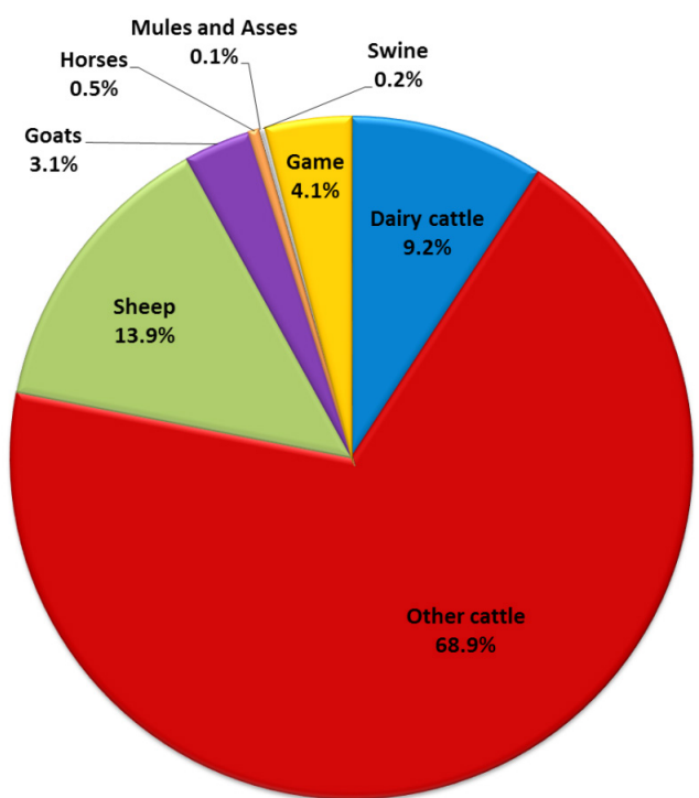
Figure 5.6: Sector 3 AFOLU – Livestock: Contribution of the livestock categories to the enteric fermentation emissions in 2012.
