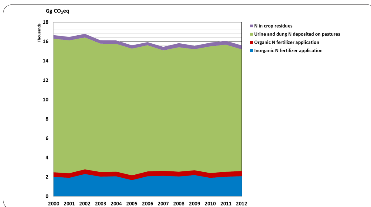
Figure 5.22: Sector 3 AFOLU – Aggregated and non- \text{CO}_2 sources: Trend and emission levels of direct \text{N}_2\text{O} from managed soils, 2000 – 2012
