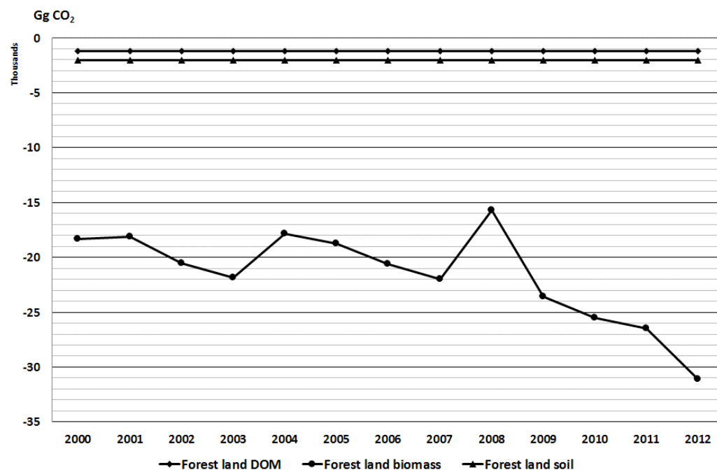
Figure 5.14: Sector 3 AFOLU – Land: Trend in emissions and sinks (in Gg CO 2 ) in the forest land between 2000 and 2012, differentiated by source category.
