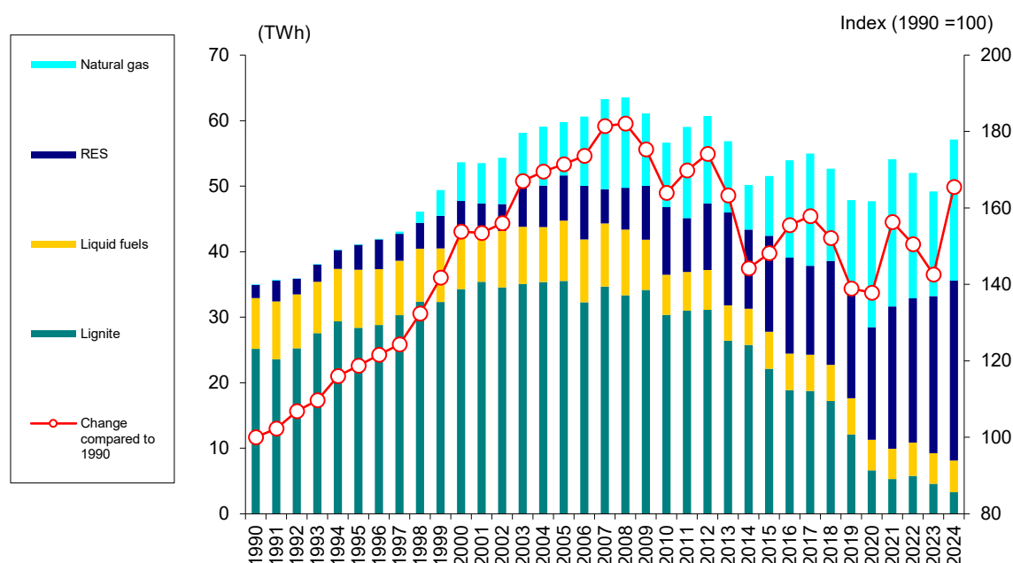
Figure 3.6 Electricity production (in TWh) by energy type for the period 1990 – 2024
