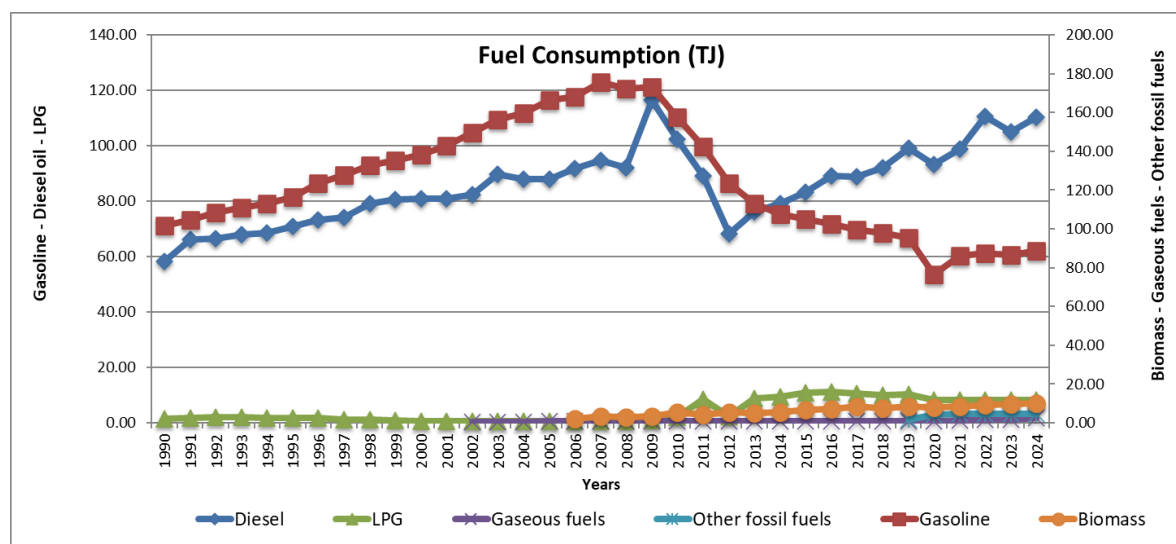
Figure 3.10a Fuel consumption per fuel category during whole time period 1990-2024
