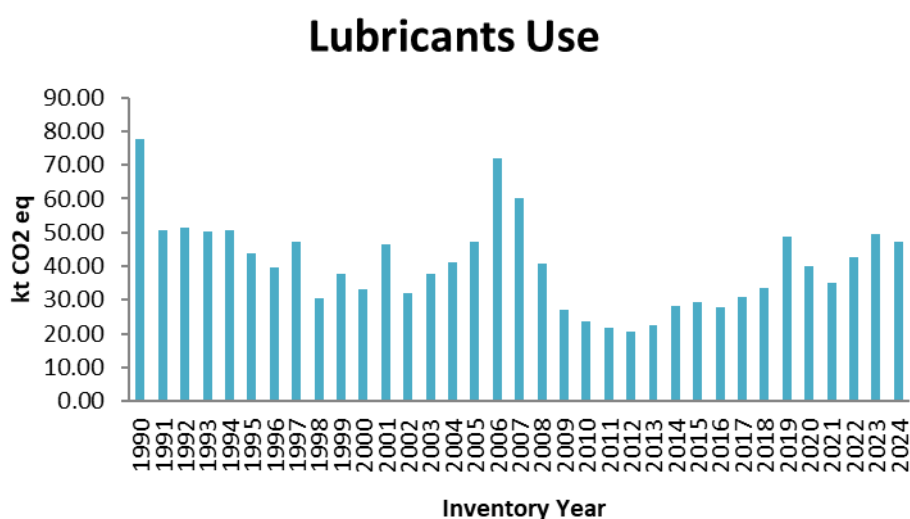
Figure 4.16 CO 2 emissions (in kt) from Lubricant Use for the period 1990 – 2024.
