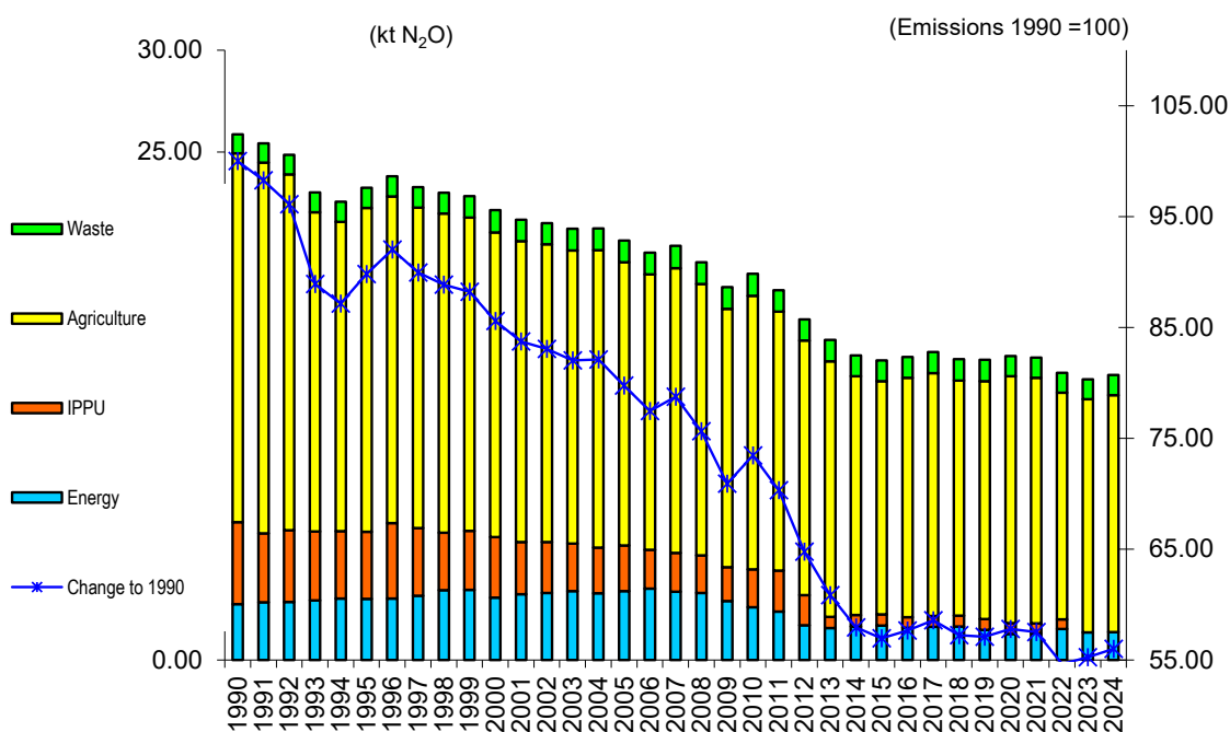
Figure 2.4 N 2 O emissions by sector (in kt) for the period 1990 – 2024 (without LULUCF)
