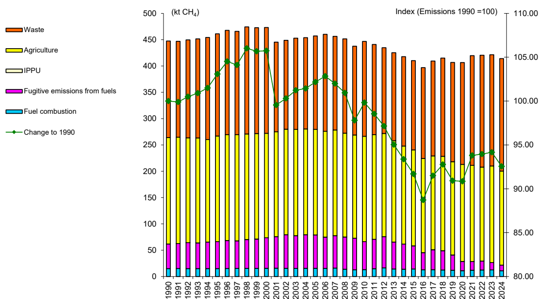
Figure 2.3 CH 4 emissions by sector (in kt) for the period 1990 – 2024 (without LULUCF)
