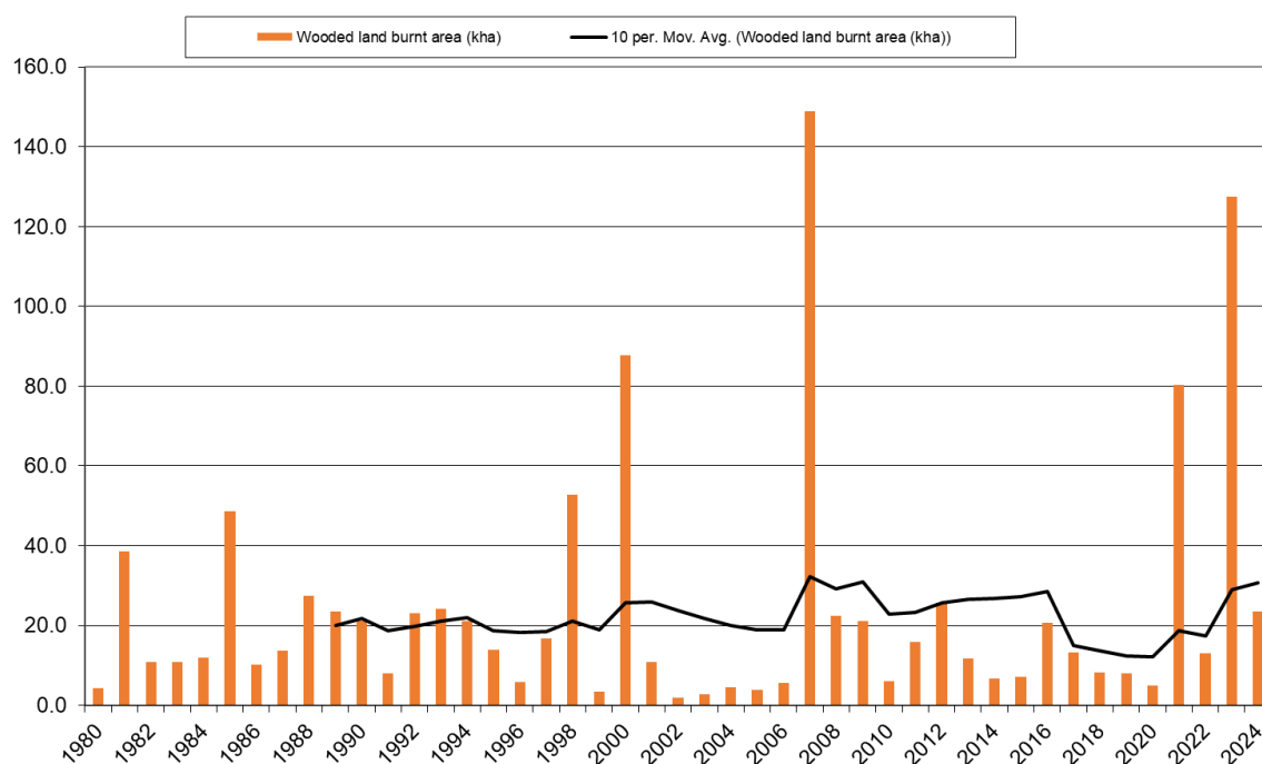
Figure 6.4 Areas of Forest Land burnt since 1980
