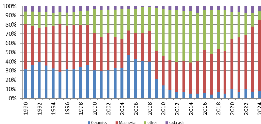
Figure 4.6 Contribution of each subcategory of the Other Process Uses of Carbonates category for the period 1990 – 2024
