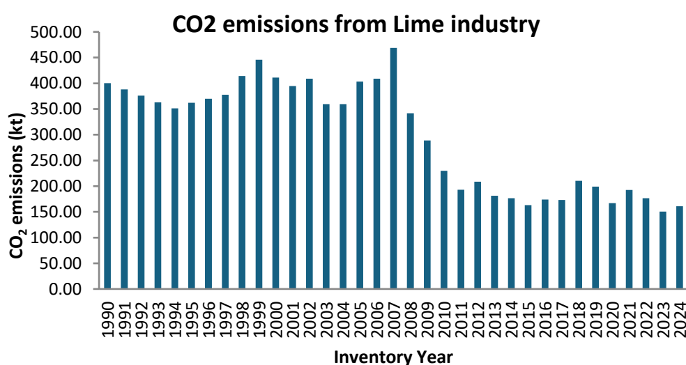
Figure 4.4 CO 2 emissions for lime production for the period 1990 – 2024
