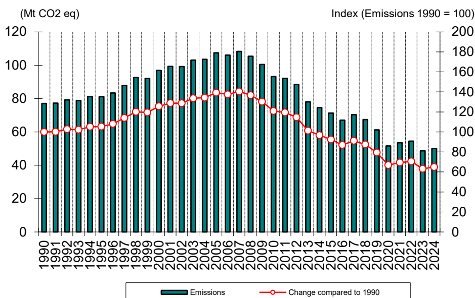
Figure 3.2 Total GHG emissions from Energy (in Mt CO 2 eq) for the period 1990 – 2024
