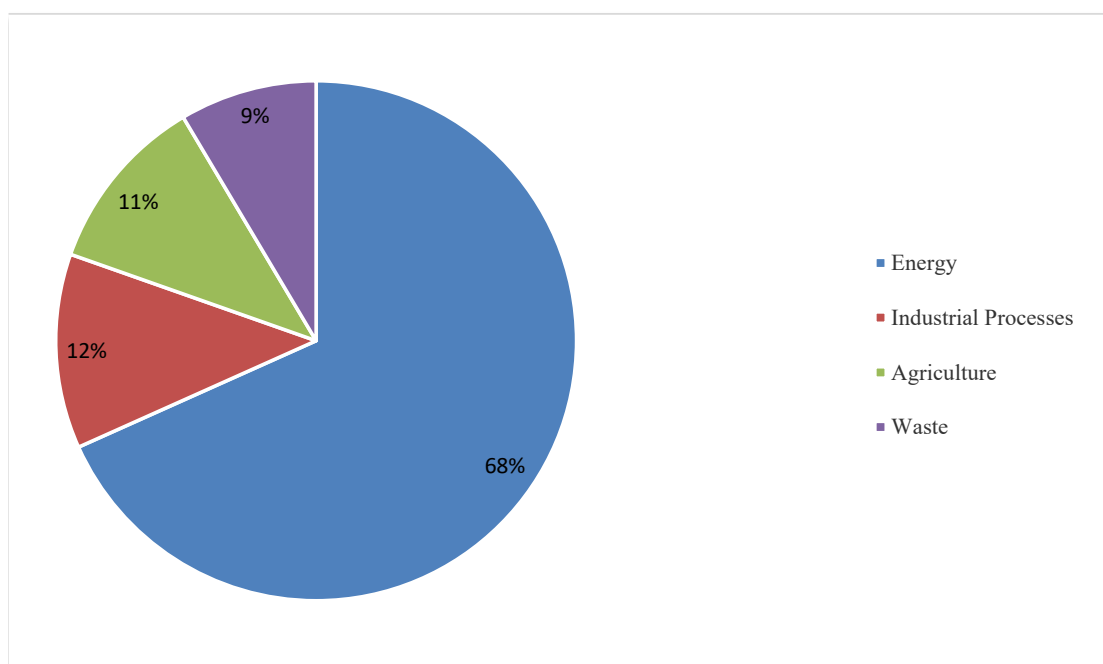
Figure 2.1 Relative contribution of activity sectors to total GHG emissions (without LULUCF) in 2024
