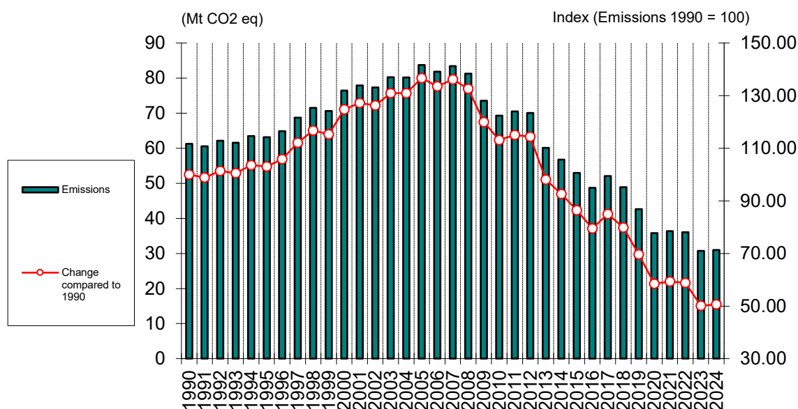
Figure 3.4 GHG emissions (in Mt CO 2 eq) from stationary combustion for the period 1990 – 2024
