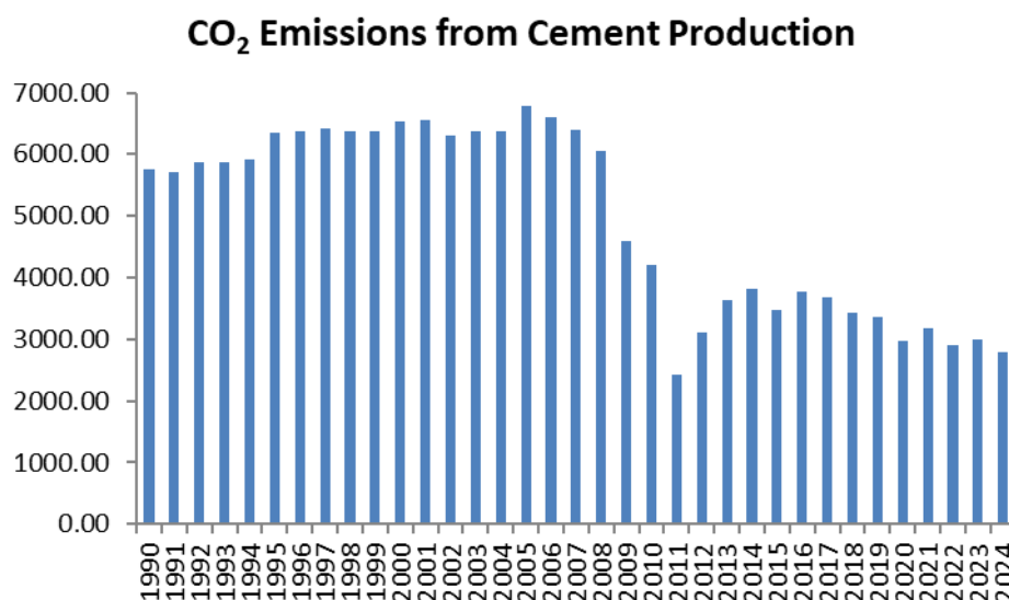
Figure 4.3 CO 2 emissions (in kt) from Cement Production for the period 1990 – 2024
