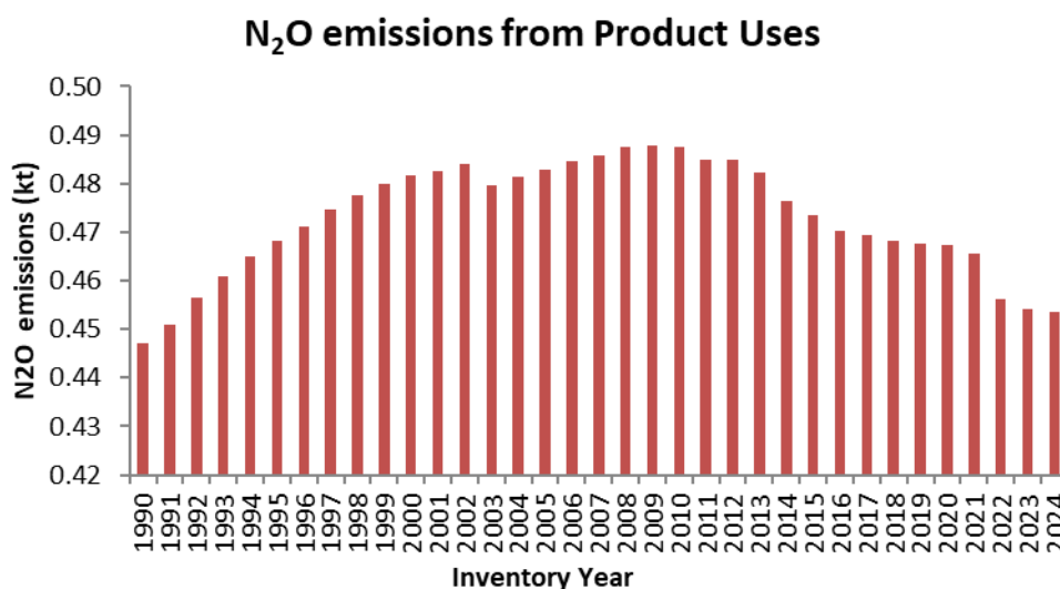
Figure 4.25 N 2 O emissions (in kt) from Product Uses for the period 1990 – 2024.
