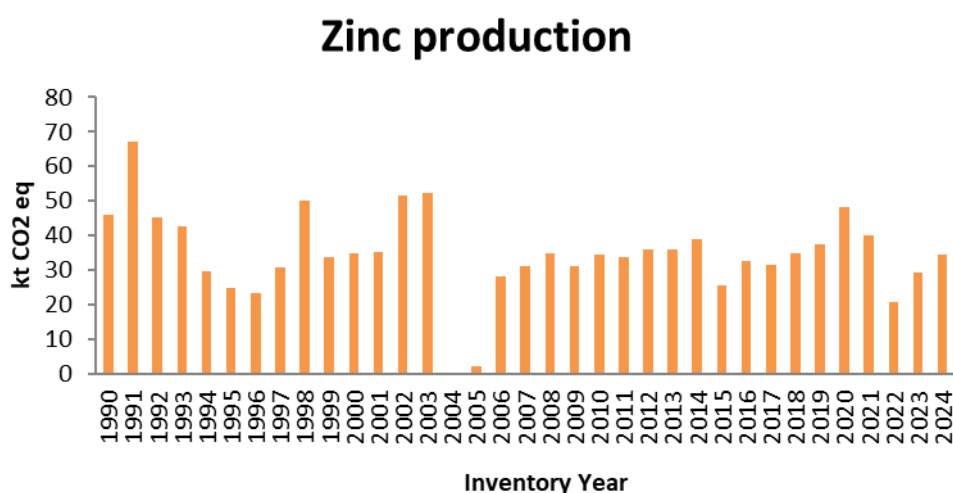
Figure 4.15 CO 2 emissions (in kt) from Zinc Production for the period 1990 – 2024.
