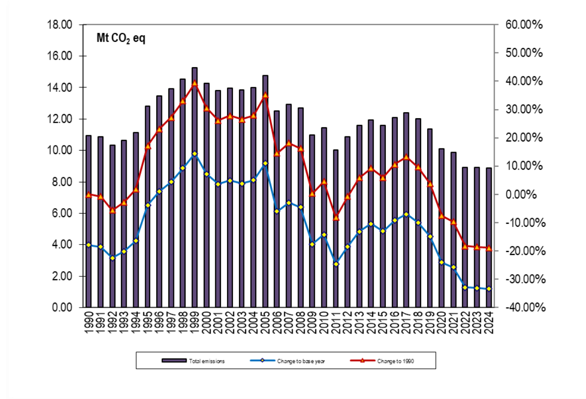
Figure 4.1 Total GHG emissions (in Mt CO 2 eq) from Industrial Processes for the period 1990 – 2024
