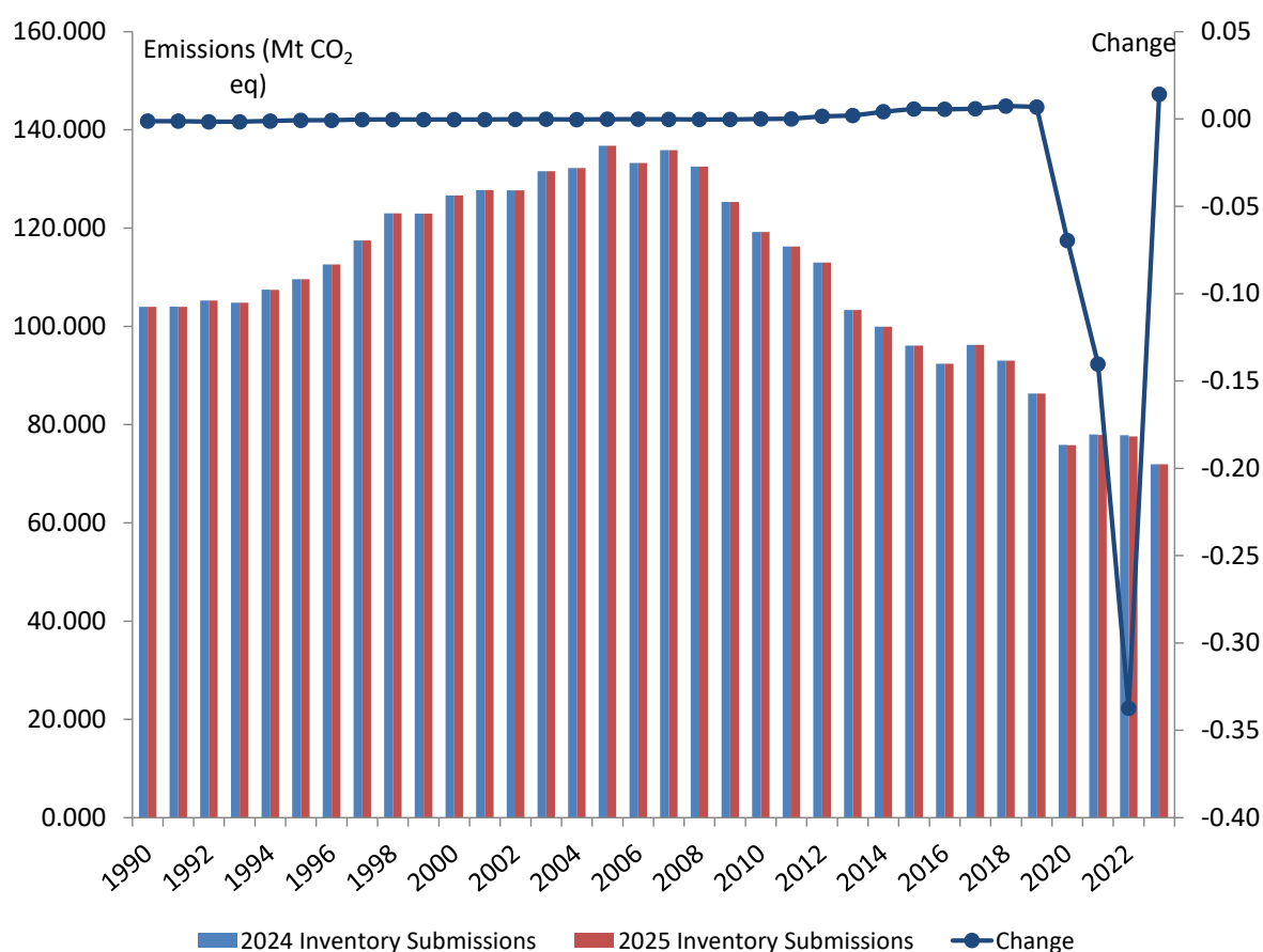
Figure 8.1 GHG emissions trends in Greece for the period 1990 – 2023 (without LULUCF) according to the inventories submitted in 2025 & 2026
