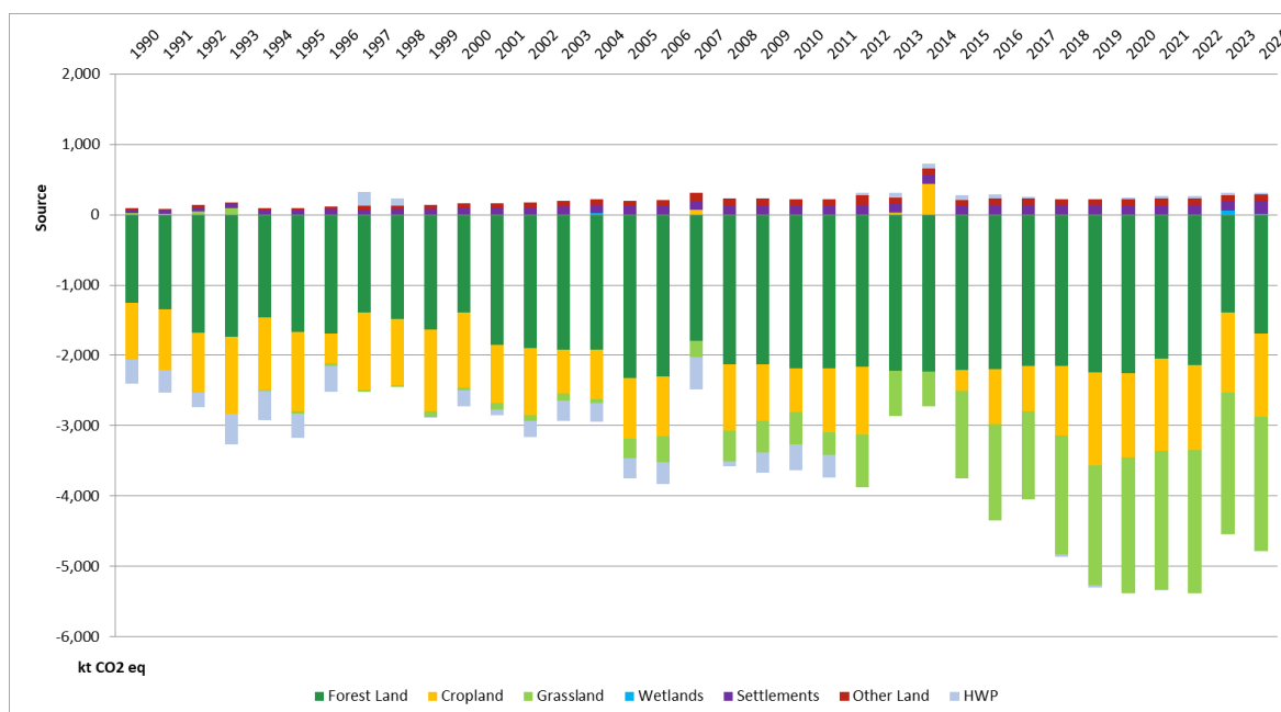
Figure 6.1 Net GHG emissions / removals (in kt CO 2 eq) from the Land Use, Land Use Change and Forestry sector by category for the period 1990 – 2024
