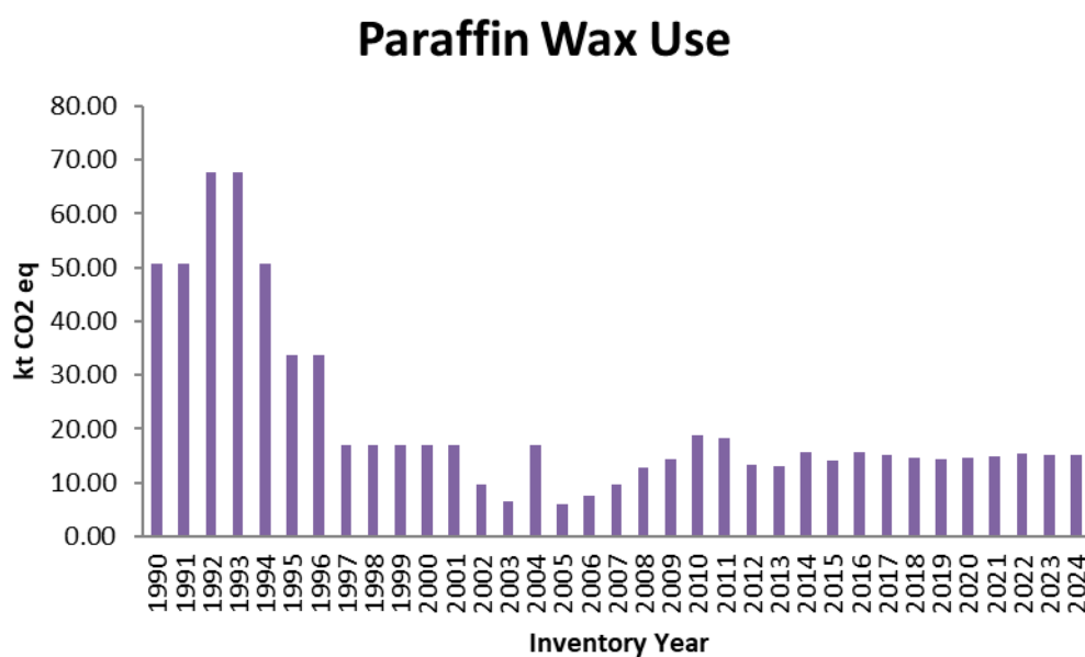
Figure 4.17 CO 2 emissions (in kt) from Paraffin Wax Use for the period 1990 – 2024.
