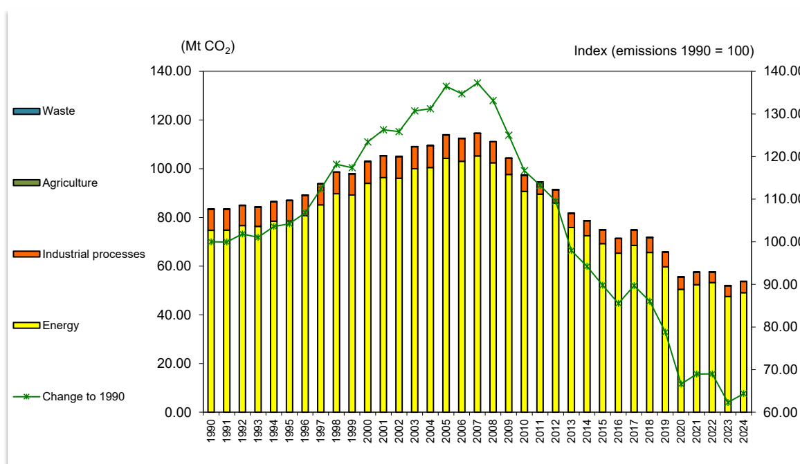
Figure 2.2 CO 2 emissions by sector (in Mt) for the years 1990 – 2024 (without LULUCF)
