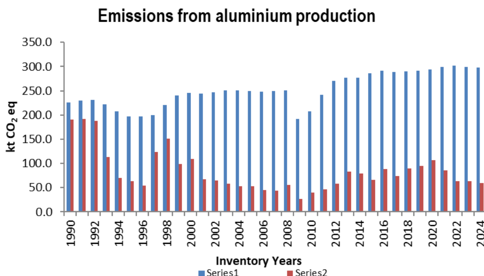
Figure 4.13 CO 2 and PFCs emissions (in ktCO 2 eq) from aluminium production for the period 1990 – 2024
