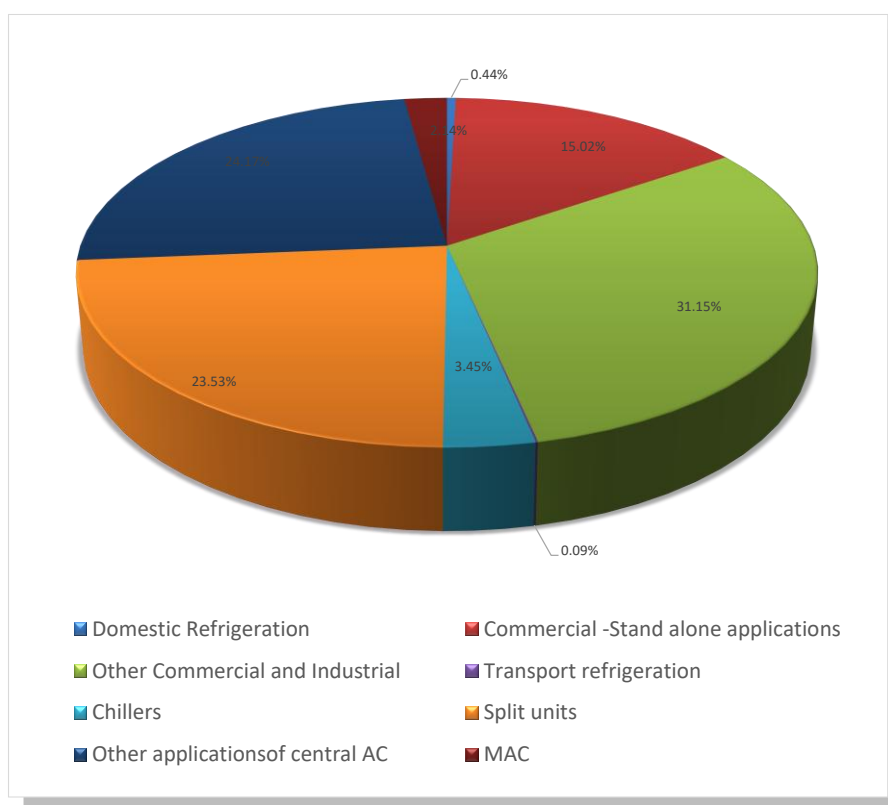
Figure 4.20 Contribution of each sub-source for 2.F.1 for 2024
