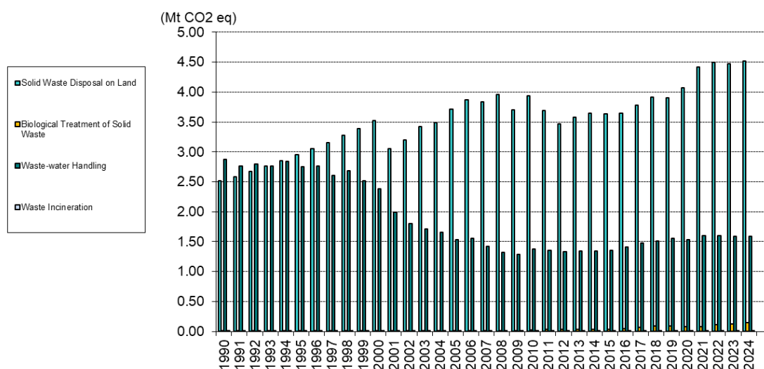
Figure 7.2 Greenhouse gases emissions (in kt CO 2 eq) from Waste per source category for the period 1990 – 2024
