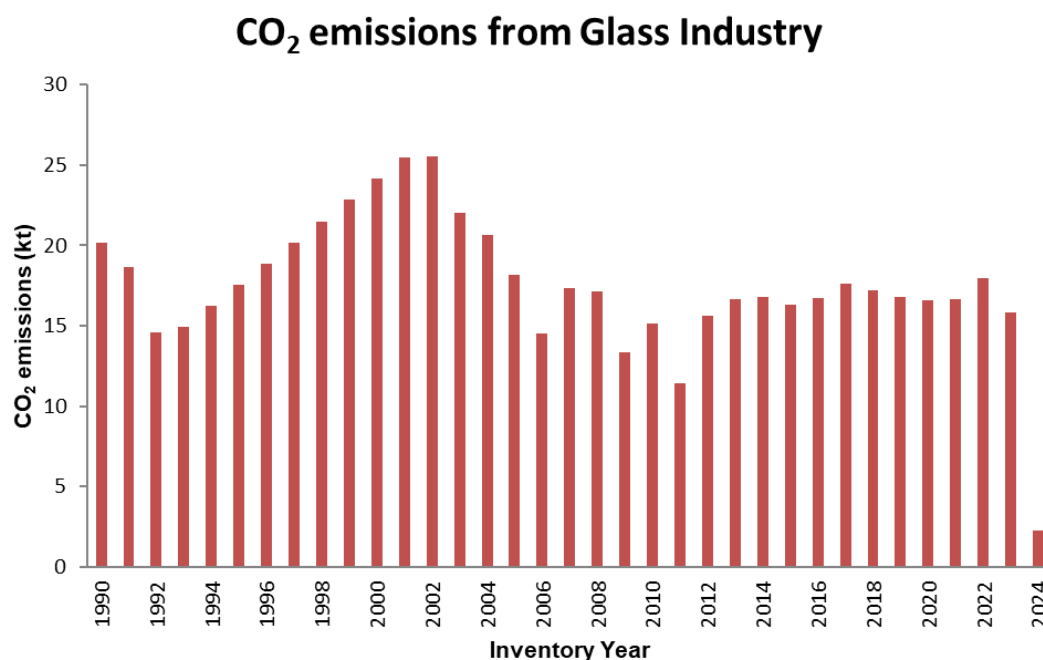
Figure 4.5 CO 2 emissions (in kt) from Glass Production for the period 1990 – 2024
