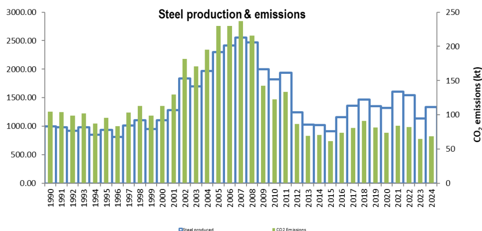
Figure 4.11 Steel production and CO 2 emissions (in kt) for the period 1990 – 2024
