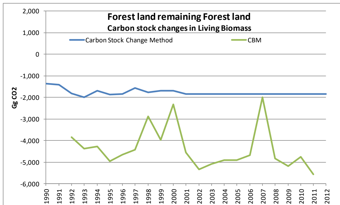
Figure 6.3 Comparison of the carbon stock changes in Living biomass in Forest land remaining Forest land, with the application of Carbon Stock Change Method and the CBM 7
