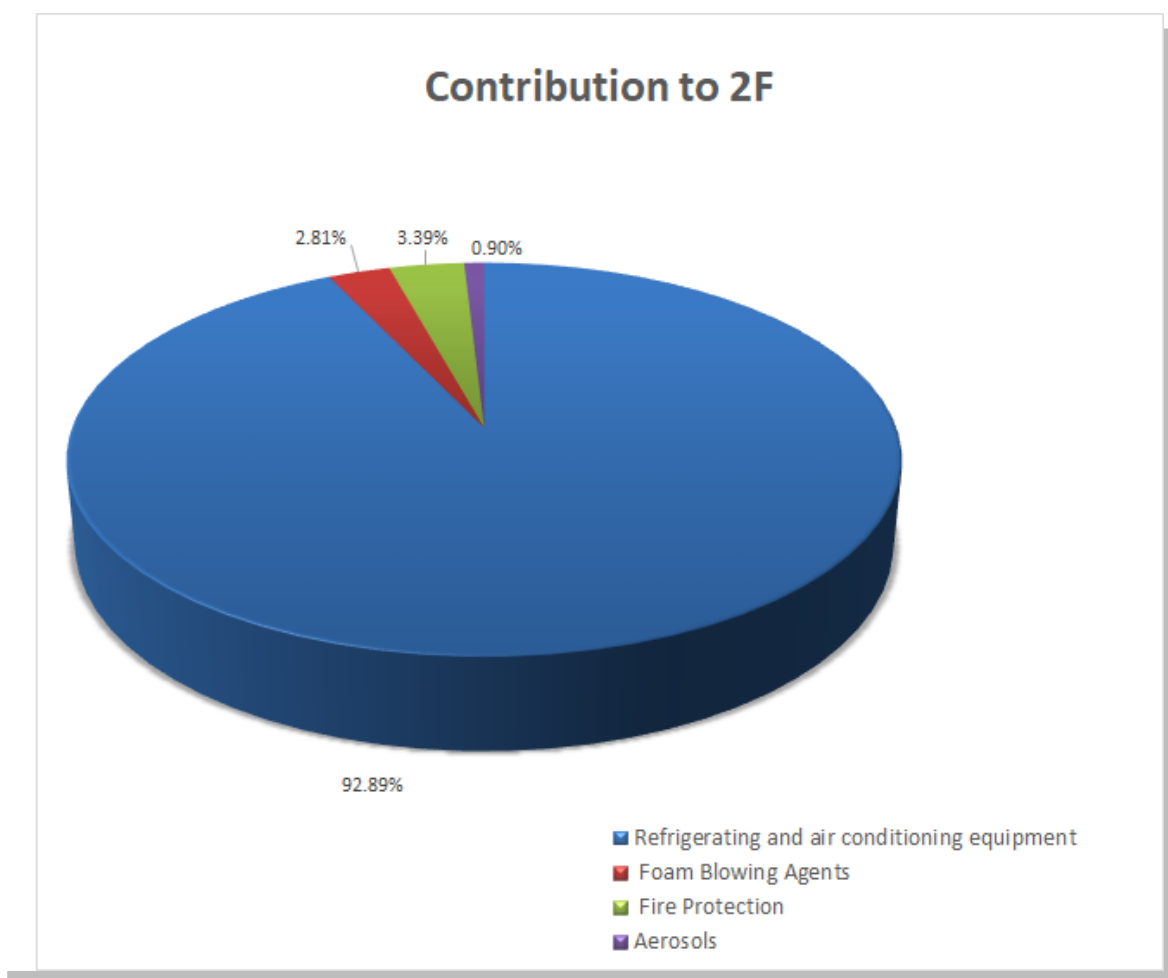
Figure 4.19 F Gases emissions distribution from ODS substitutes in 2023
