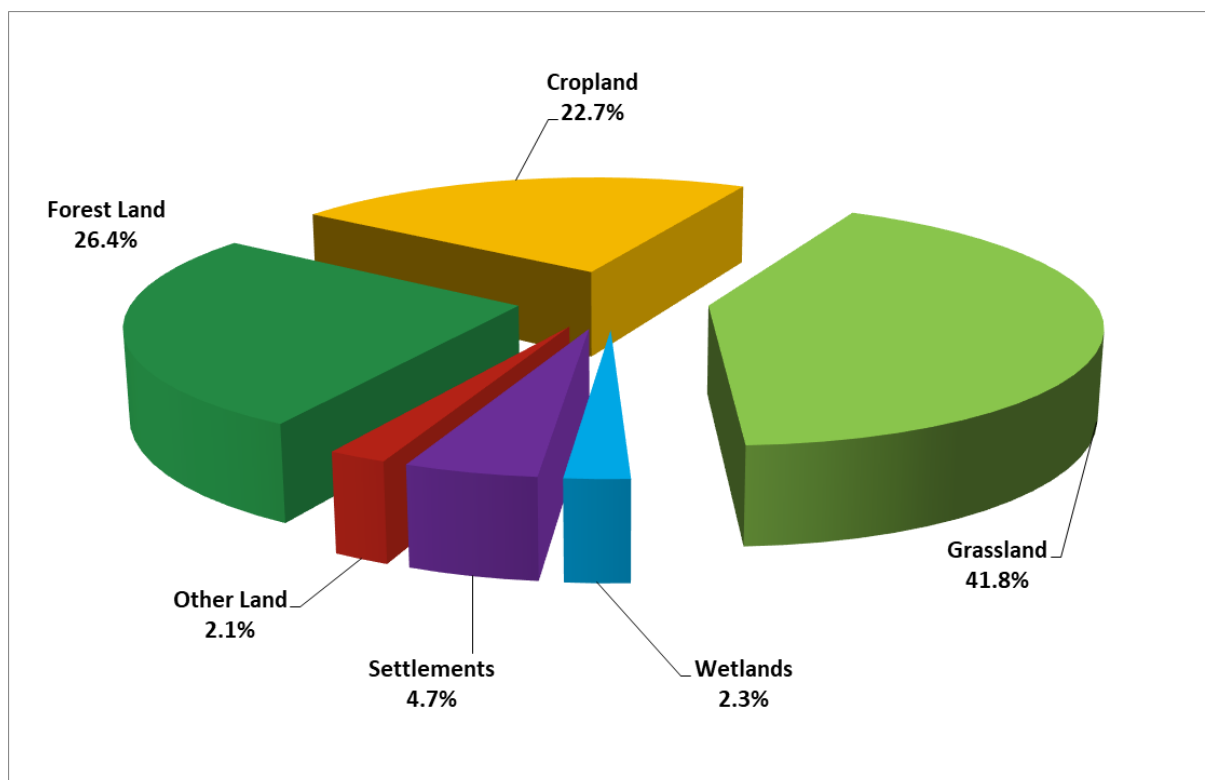
Figure 6.2 Distribution of the area of Greece in 2023 by land-use category
