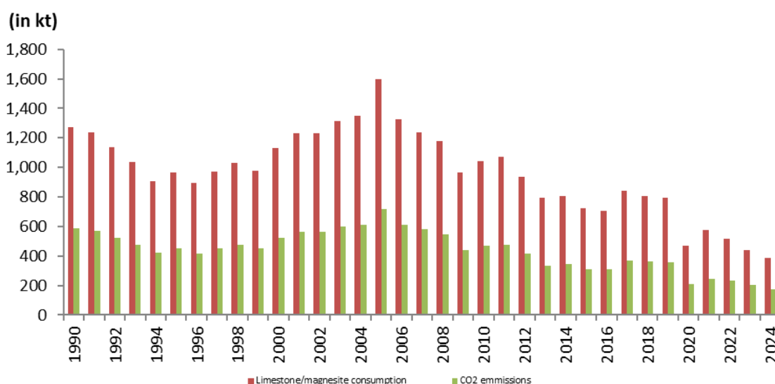
Figure 4.7 CO 2 emissions (in kt) and Limestone/ magnesite consumption (in kt) from Other Process Uses of Carbonates for the period 1990 – 2024
