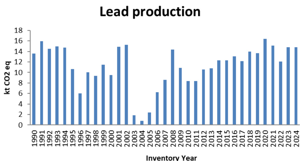
Figure 4.14 CO 2 emissions (in kt) from Lead Production for the period 1990 – 2024.
