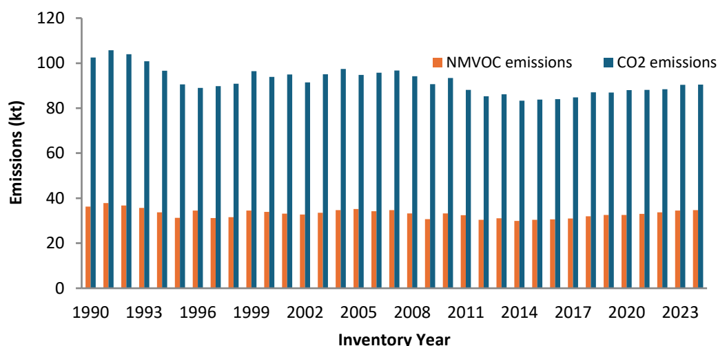
Figure 4.26 CO2 and NMVOC emissions (in kt) from other uses of solvents for the period 1990 – 2024.
