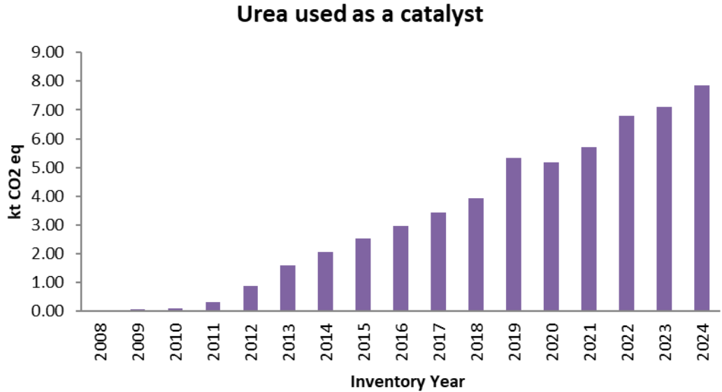
Figure 4.18 CO 2 emissions (in kt) from urea-based additives in catalytic converters for the period 2008– 2024.
