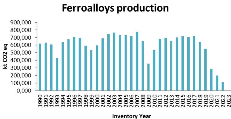
Figure 4.12 CO 2 emissions (in kt) from Ferroalloys Production for the period 1990 – 2023
