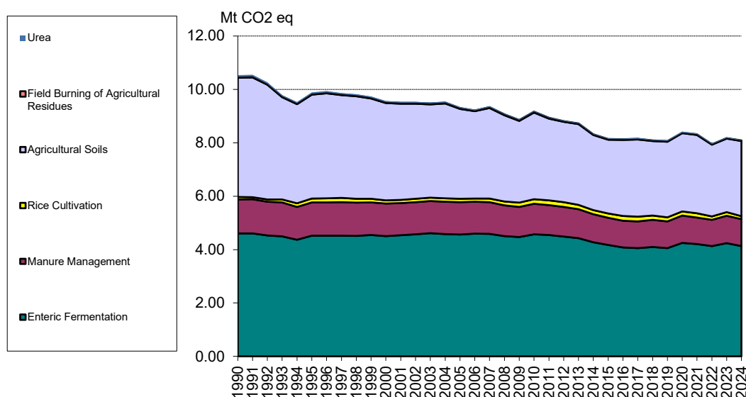
Figure 5.2 GHG emissions (in kt CO 2 eq) from Agriculture per source category
