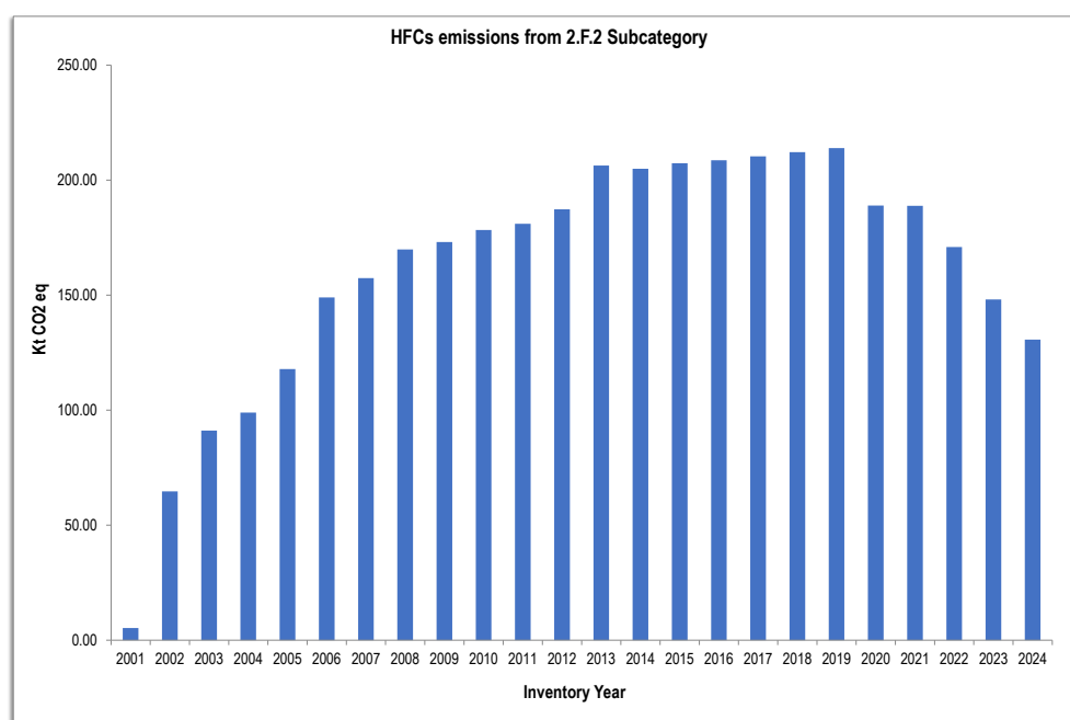
Figure 4.21 HFCs emissions from 2.F.2 Subcategory for the period 1990 – 2024.
