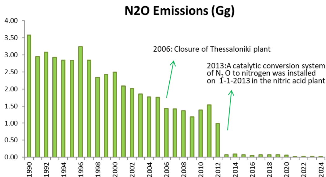
Figure 4.9 N 2 O emissions (in kt) from Nitric Acid Production for the period 1990 – 2024
