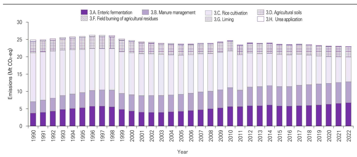
| Figure 2–15 | Trends in Agriculture Sector Greenhouse Gas Emissions (1990–2022)
