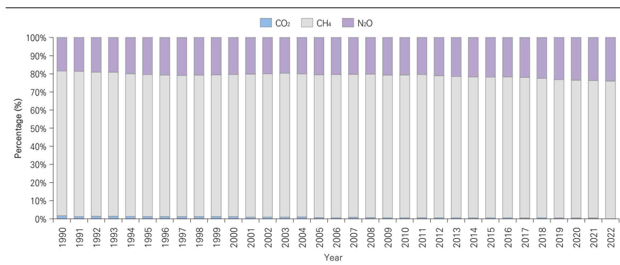
| Figure 2-17 | Percentage of Gas in Agriculture Sector Emissions (1990-2022)
