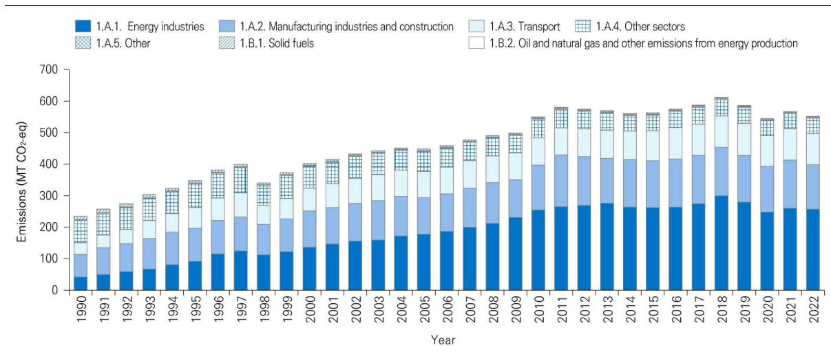
| Figure 2–9 | Trends in Energy Sector Greenhouse Gas Emissions (1990–2022)
