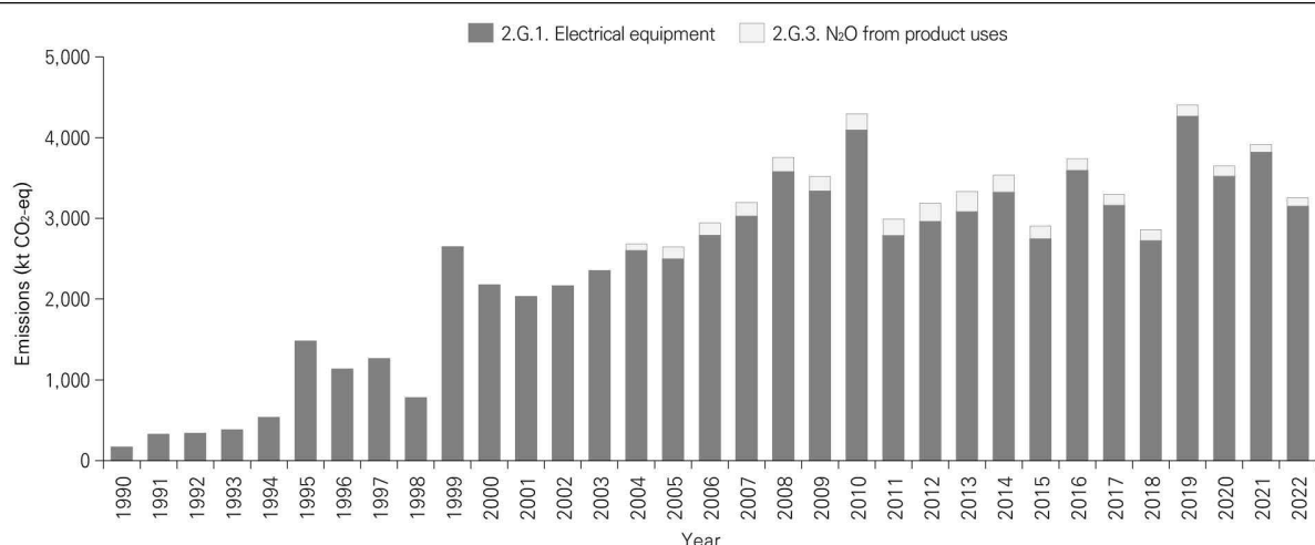
Figure 4-9 | Trends in Emissions from Other Product Manufacture and Use (1990–2022)
