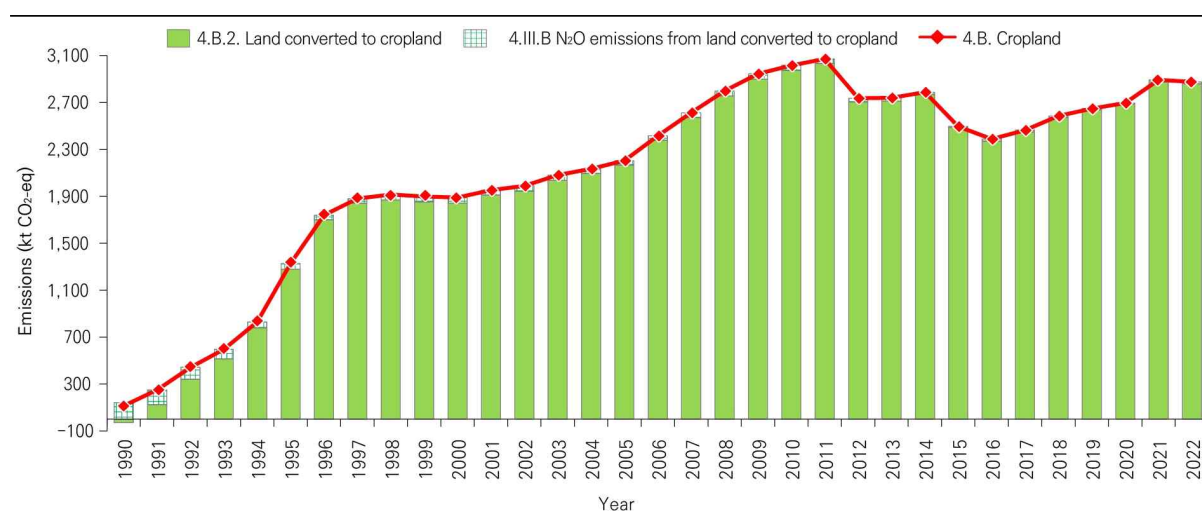
| Figure 6-4 | Trends in Cropland Emissions and Removal (1990–2022)
