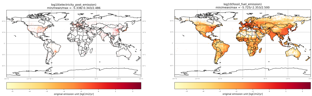
Figure 5 – 2021 fossil fuel and biofuel emissions inferred by CCFDAS in kgC m -2 yr -1 on a logarithmic scale for the energy generation sector (left) and for the total over all sectors (right).
