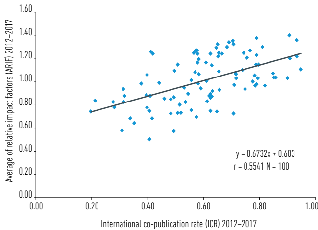
Figure ES.10. Comparison of ICR and average of relative impact factors (ARIF) of the ocean science community and ocean practitioners.
