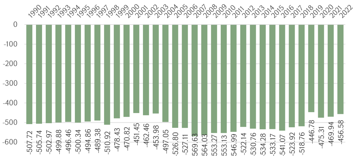
Figure 7.4 Carbon dioxide removals in Forest Land Remaining Forest Land sub-category, kt
