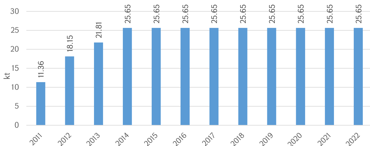
Figure 7.8 Carbon dioxide emissions in Land Converted to Grassland sub-category in 2011-2022, kt
