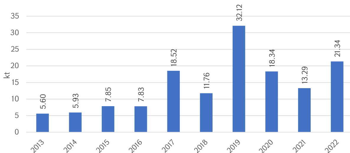
Figure 7.9 Annual emissions of CO 2 from Wetlands , kt CO 2
