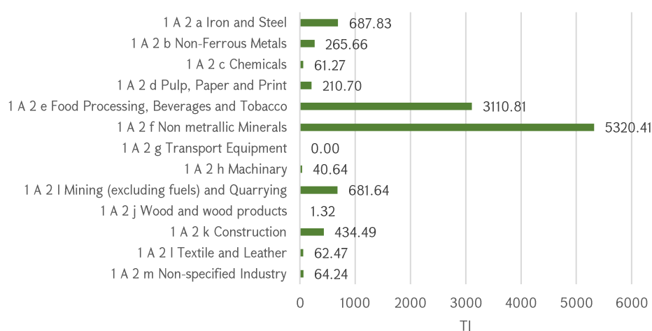
Figure 4.11 Natural gas, diesel fuel, LPG and total energy consumption by sub-categories, 2022
