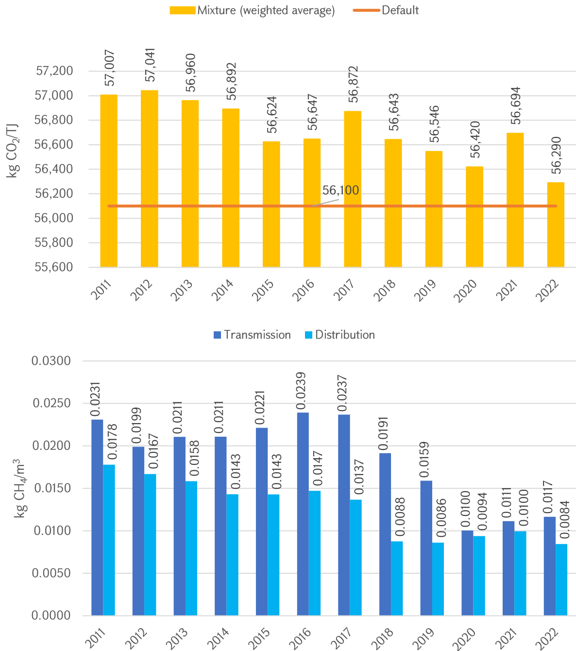
Figure 4.7 CO 2 country-specific emission factors for natural gas mixture (kg CO 2 /TJ) and country-specific CH 4 fugitive emission factors (kg CH 4 /m 3 ), 2011-2022
