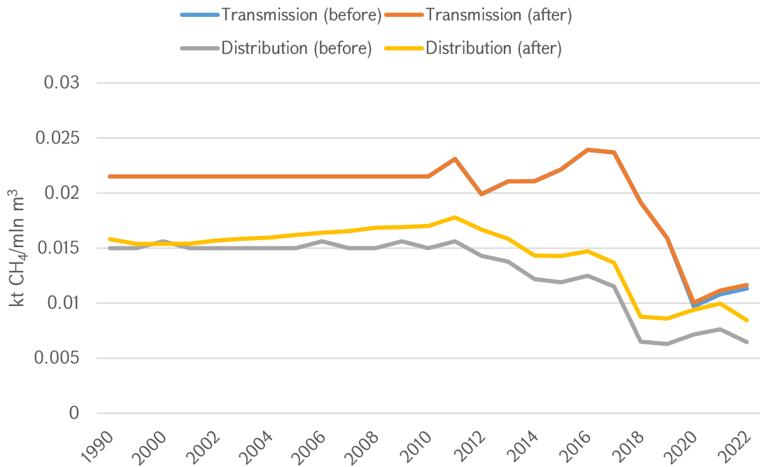
Figure 4.25 Methane country-specific fugitive emission factors (transmission and distribution), before and after recalculation, 1990-2022 (kt CH 4 /mln. m 3 )
