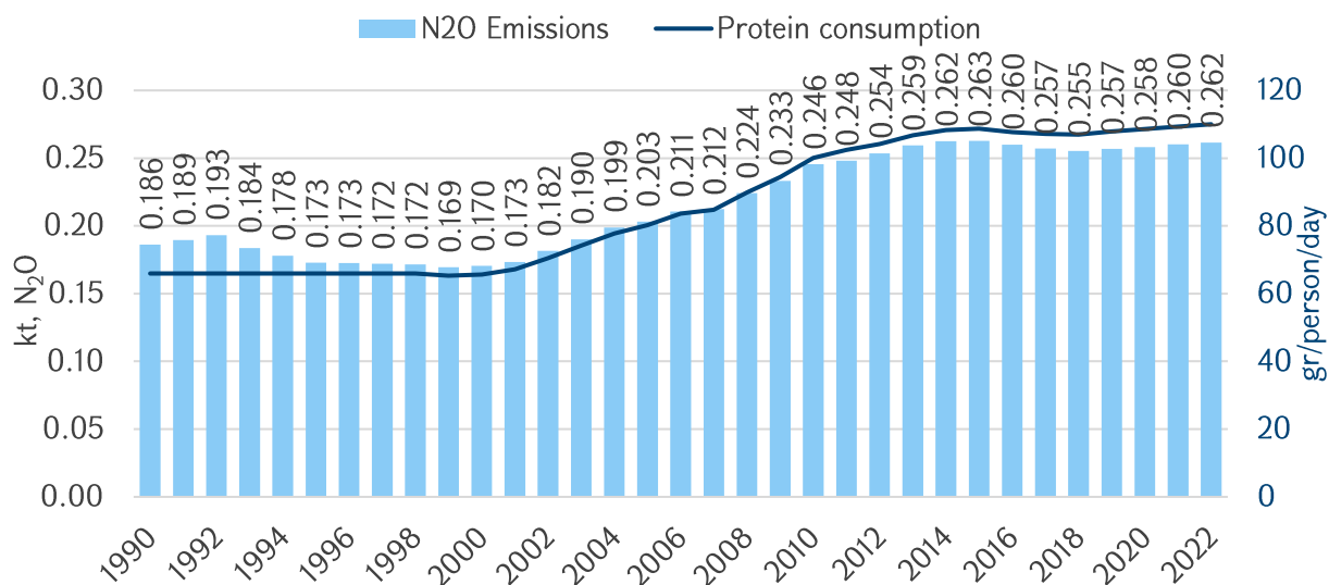
Figure 8.7 Nitrogen oxide emissions from wastewater (kt) and protein consumption
