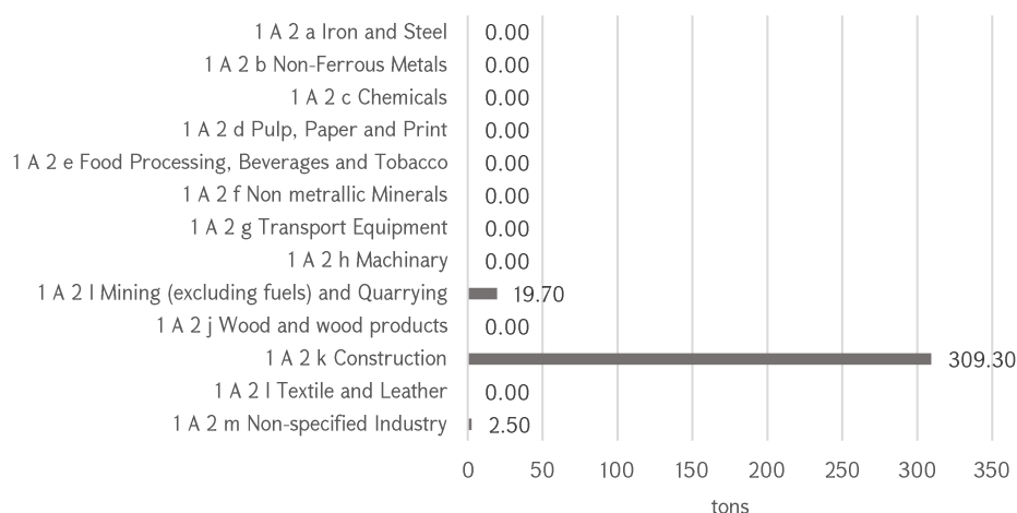
LPG Consumption in Industry and Construction sub-category 2022
