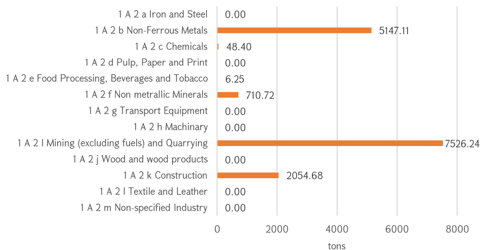
Diesel fuel consumption in Industry and Construction sub-category 2022
