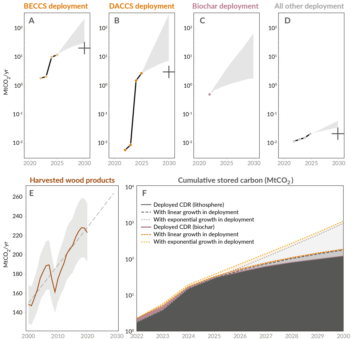
Figure 6.4. (A-D) Deployment of various methods for generating carbon sinks, measured in \text{MtCO}_2 per year. Grey projections indicate a lower (linear) and upper (exponential) extrapolation of 2020-2025 deployment data. The grey crosses indicate 2030 deployment if only currently in-development projects are completed. (E) Harvested wood product production, measured in \text{MtCO}_2 per year, with a linear projection to 2030, with 9-95% uncertainty in grey. (F) Cumulative stored carbon by storage reservoir/pool, given observed deployment, continued linear deployment and continued exponential deployment, measured in \text{MtCO}_2 . Definitions: Bioenergy with Carbon Capture and Storage (BECCS); Carbon Dioxide Removal (CDR); Direct Air Carbon Capture and Storage (DACCS).
