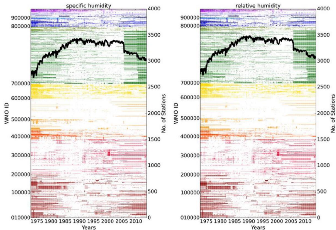
Figure 82: Number of stations (black lines; right-hand scale) from which data are selected for use to construct gridded products for specific (left) and relative (right) humidity, as a function of year. Also shown in colour are missing station months as a function of WMO ID (left scale). The colour coding denotes different geographical regions. Source: Willett et al. (2014a).
