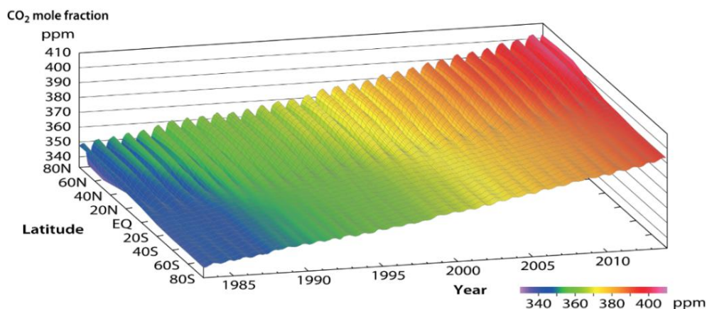
Figure 33: Variation with latitude and time of zonally averaged monthly-mean CO 2 mole fractions, from an analysis of data submitted to the World Data Centre from Greenhouse Gases (WDCGG), Japan Meteorological Agency. The zonally averaged mole fractions were calculated for 20° latitude bands based on station data shown later in Figure 93. Source: Plate 3.1 of the annual issue of the Data Summary published in March 2015 (WDCGG, 2015).
