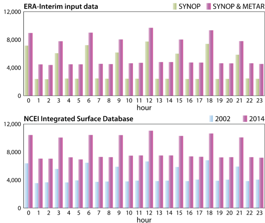
Figure 8: Average counts of surface air temperature observations over land for each hour of the day for October 2014 from ECMWF’s operational receipt of data, as processed in ERA-Interim following basic quality-control checks (upper), and for October 2002 and 2014 from the NOAA NCEI Integrated Surface Database after duplicate removal and elimination of sub-hourly data (lower). ERA-Interim counts are shown for SYNOP reports alone, and as supplemented by METAR reports. NCEI data were downloaded from the ISD-Lite data stream on 22 January 2015.
