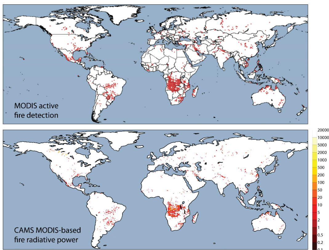
Figure 69: MODIS active-fire detection (upper) and Copernicus Atmosphere Monitoring Service (CAMS) fire radiative power (FRP) areal density ( \text{mW}/\text{m}^2 ; lower) based on assimilation of MODIS FRP data, for 8 June 2015. Sources: the NASA MODIS product was visualised at https://firms.modaps.eosdis.nasa.gov/firemap/ ; the CAMS map was downloaded from http://www.copernicus-atmosphere.eu/catalogue .
