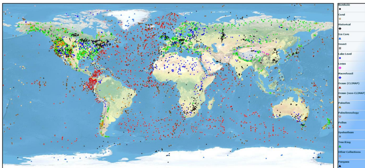
Figure 74: locations of data records (excluding reconstructions) held at the World Data Centre for Paleoclimatology. Source: NOAA, map generated at http://gis.ncdc.noaa.gov/map/viewer/#app=cdo&cfg=paleo&theme=paleo .
