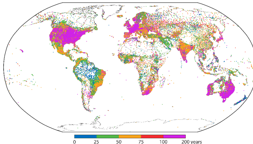
Figure 18: Locations of 75631 stations and lengths of their precipitation records held in the monthly database of the GPCP at DWD. Only stations with records longer than 10 years, covering periods beginning no earlier than 1814, are shown. Figure reproduced with permission of DWD.
