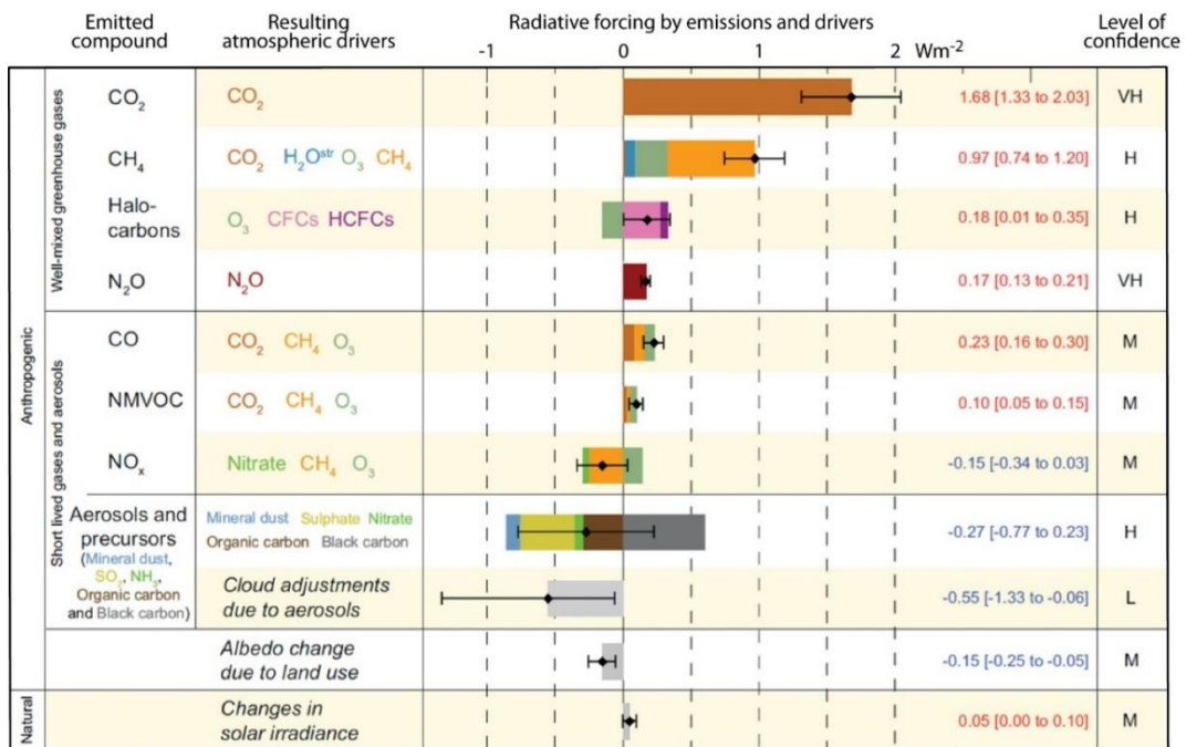
Figure 30: Radiative forcing (Wm -2 ) of climate change partitioned according to emitted compounds and resulting atmospheric drivers. Source: IPCC (2013; Figure SPM.5).
