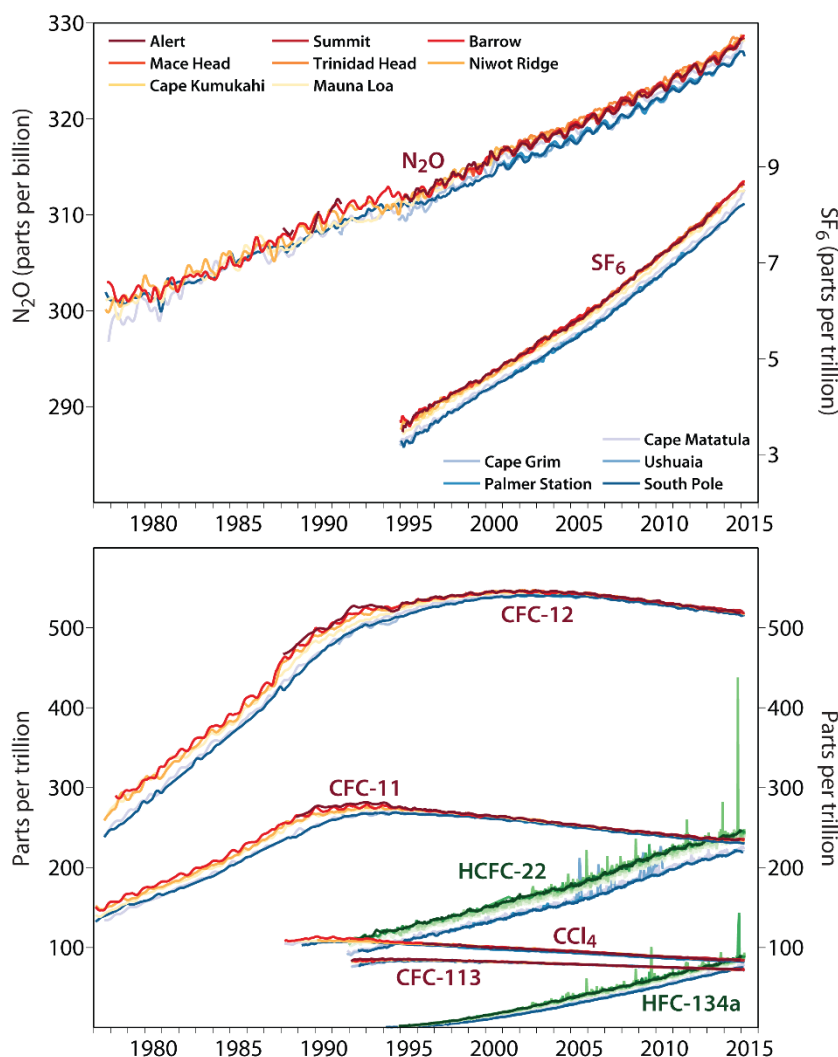
Figure 36: Mole fractions of N 2 O (upper panel, left scale; ppb) and SF 6 (upper panel, right scale; ppt) and of six halocarbons (lower panel; ppt) from measurements at a set of thirteen stations in the northern (upper legend) and southern (lower legend) hemispheres. Green colouring is used for the northern hemispheric values of HCFC-22 and HFC-134a, which are plotted using flask data for specific dates. Data for the other variables are monthly values combined from two or more measurement programmes. Data were downloaded from http://www.esrl.noaa.gov/gmd/hats/flask/flasks.html on 17 April 2015.
