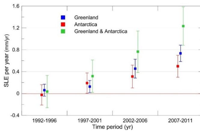
Figure 60: Rate of ice sheet loss in sea level equivalent (SLE) averaged over five-year periods between 1992 and 2011. Source: IPCC (2013; Figure 4.17).
