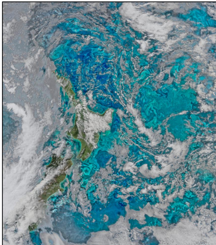
Figure 51: Image from VIIRS collected 29 September 2015 showing fine-scale structure in ocean colour near New Zealand. Source: NASA, downloaded from http://oceancolor.gsfc.nasa.gov/cms/ .
