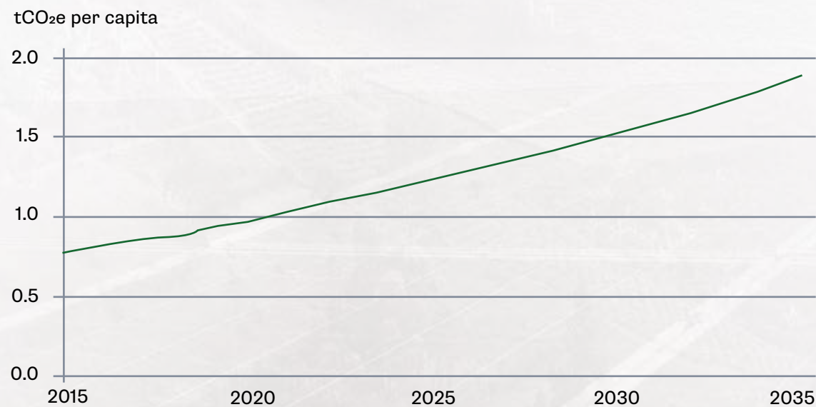
Figure 5.4 Rwanda per capita emissions, BAU scenario 2015-2035
