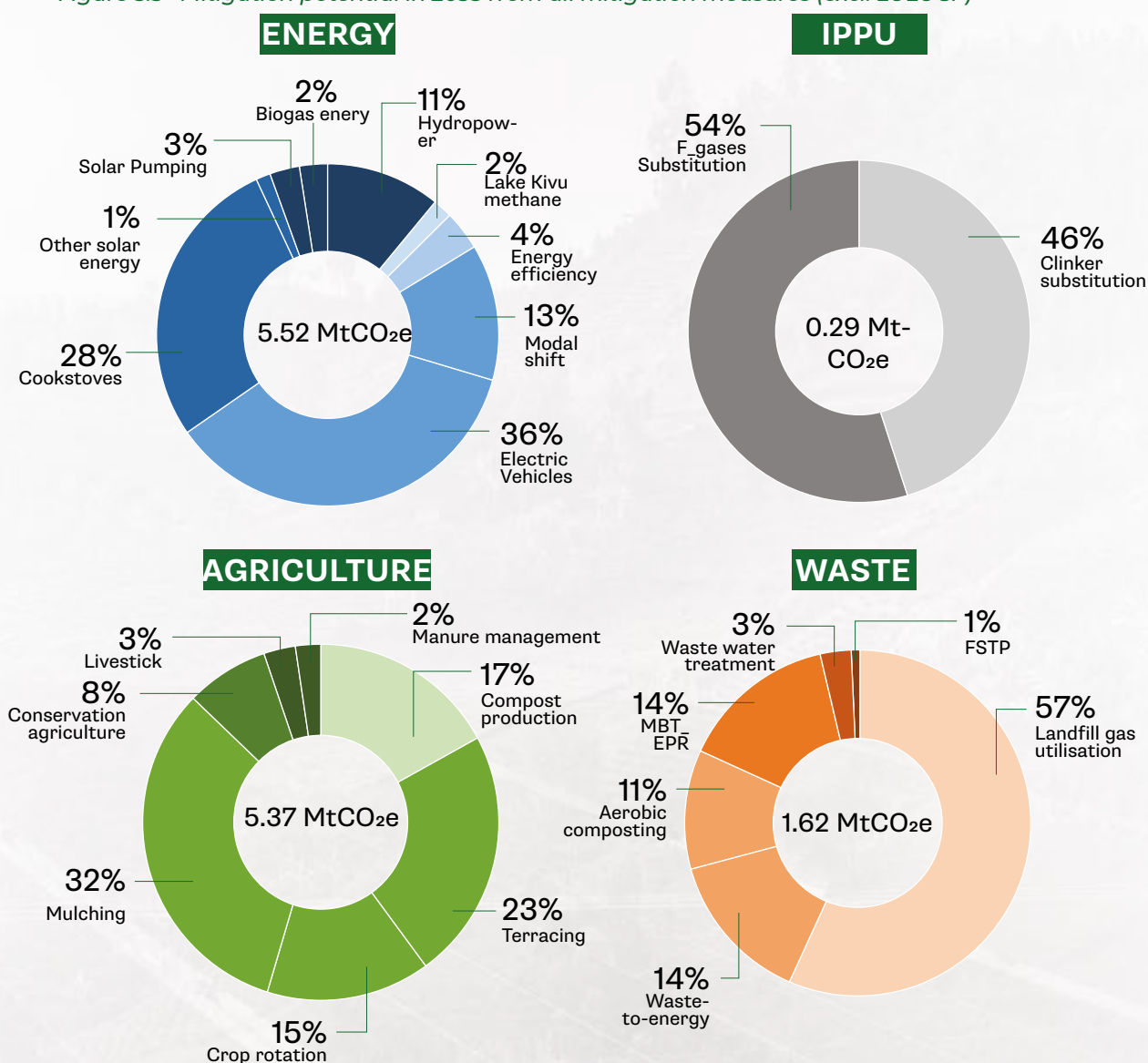
Figure 5.5 Mitigation potential in 2035 from all mitigation measures (excl. LULUCF)
