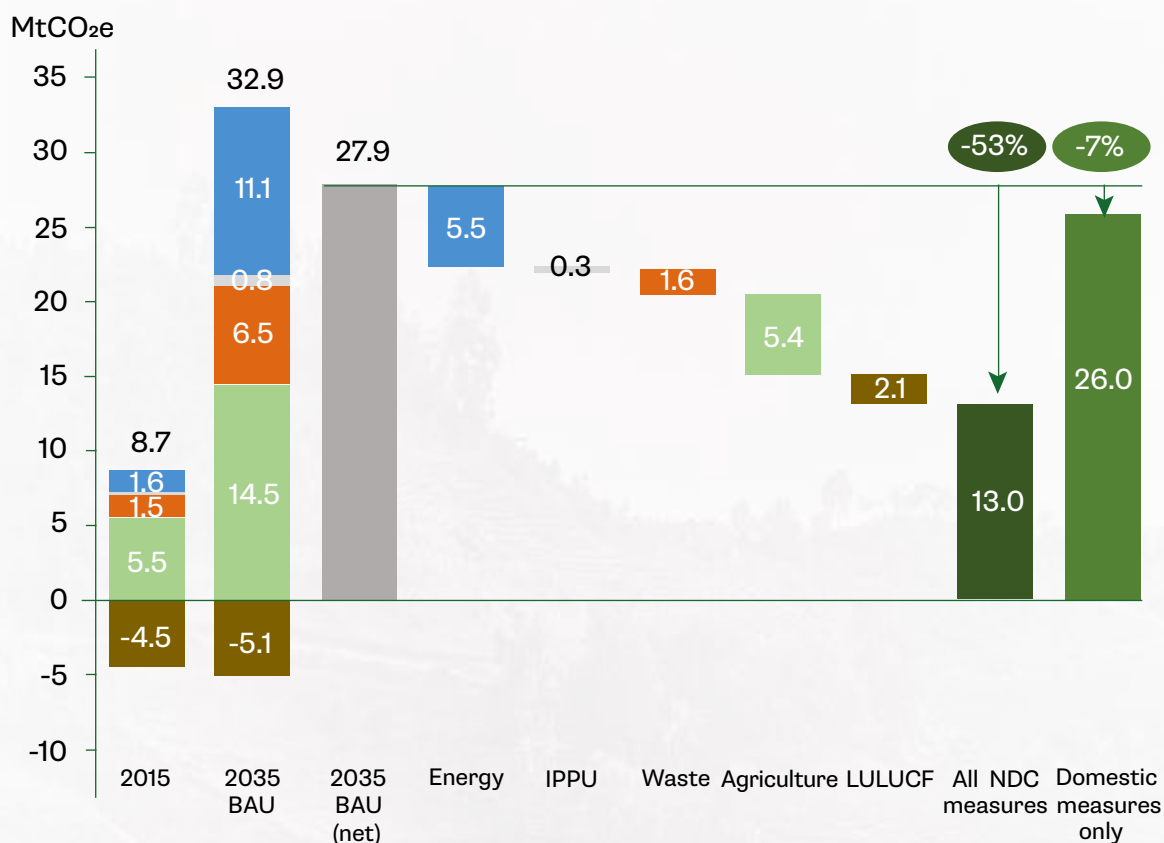
Figure 5.9 Mitigation contributions against BAU baseline (including LULUCF), 2035
