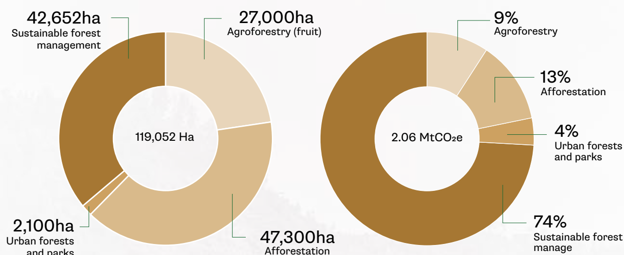
Figure 5.7 NDC forestry measure targets and associated mitigation potential in 2035
