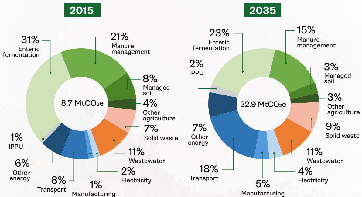
Figure 5.3 BAU scenario emissions in 2015 and 2035
