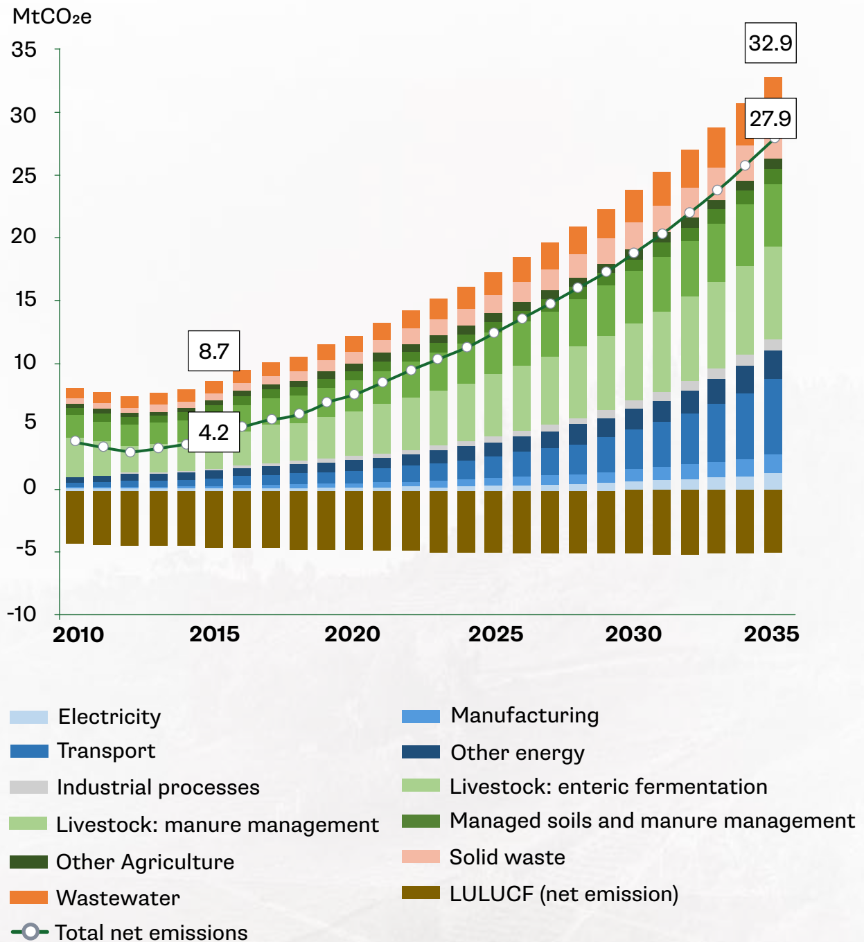
Figure 5.2 BAU GHG emissions projection, all sectors
