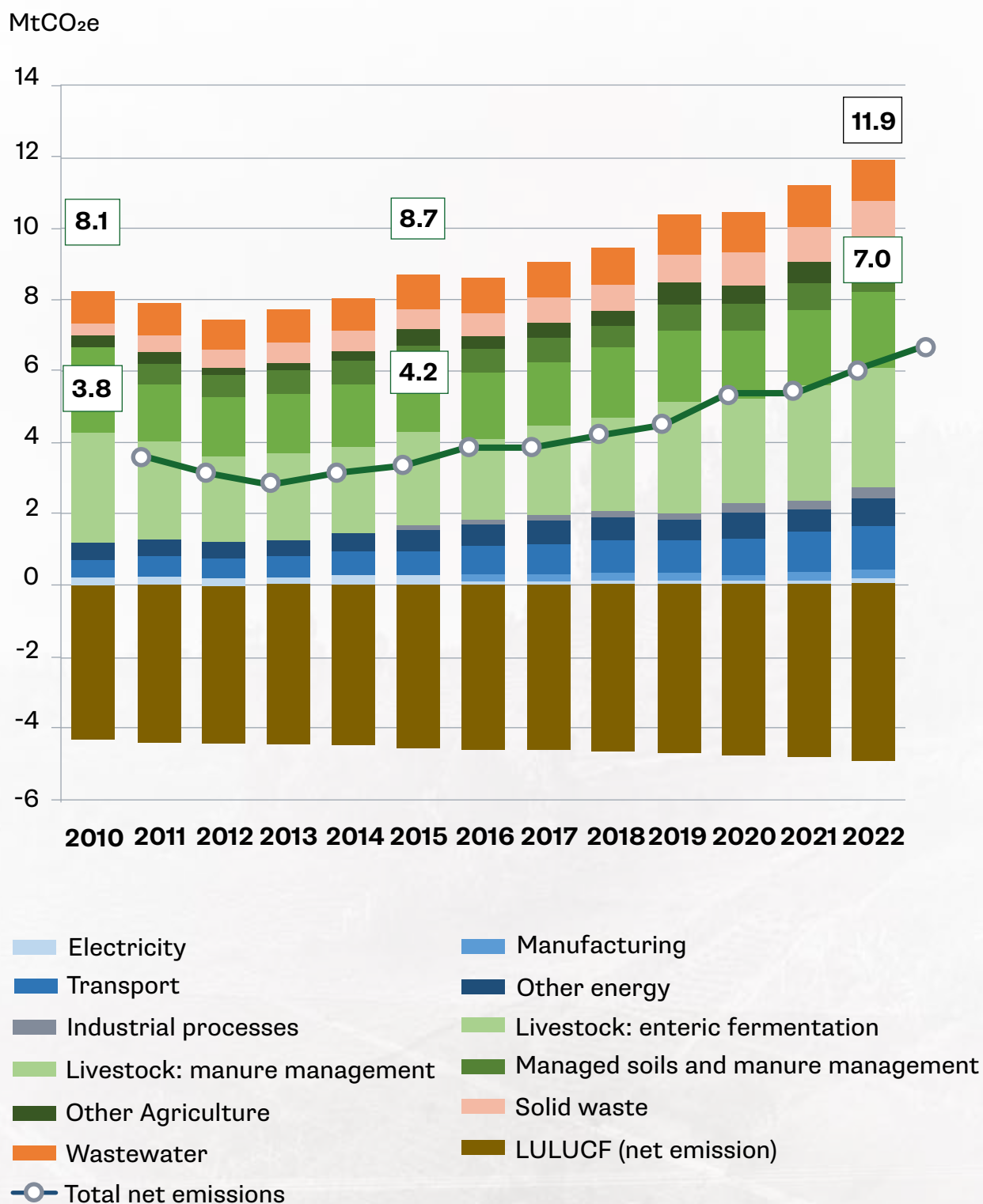
Figure 5.1 Rwanda's GHG emissions and removals by source 2010 to 2022, MtCO 2 e
