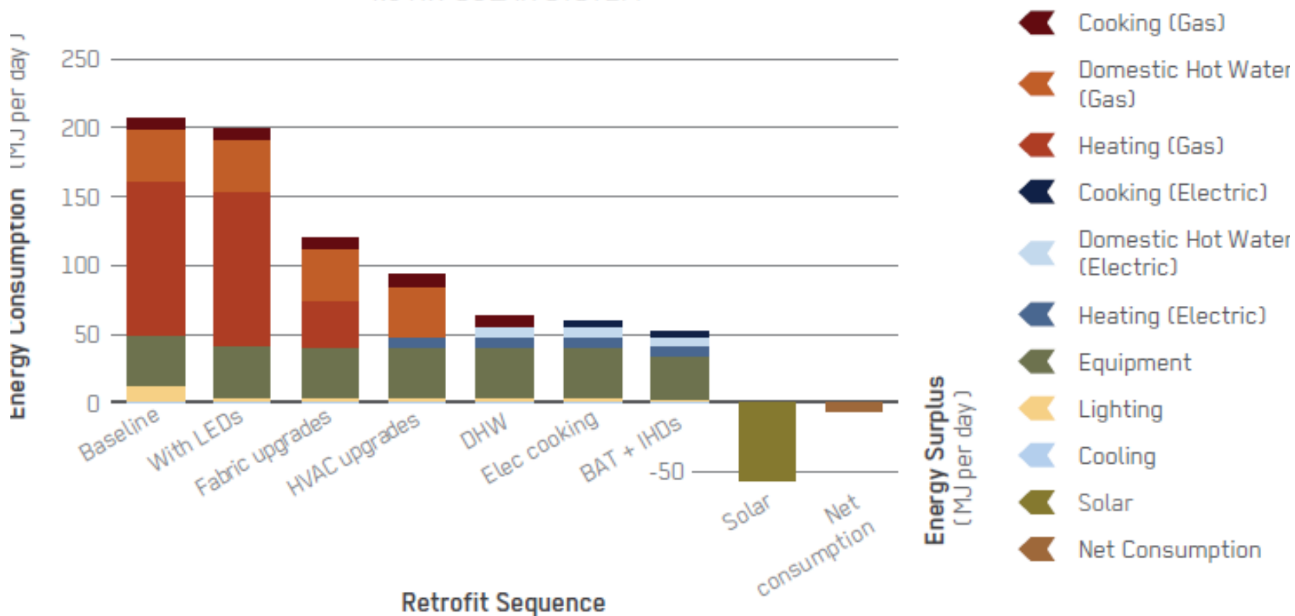
REDUCTION IN ENERGY CONSUMPTION RESULTING FROM RETROFIT 4.5 KW SOLAR SYSTEM
