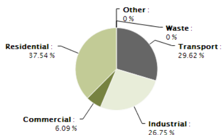
Community GHG Emissions Total ( 2007 ) : 1,534,552 tCO 2 e
