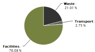
Government GHG Emissions Total ( 2007 ) : 121,185 tCO 2 e
